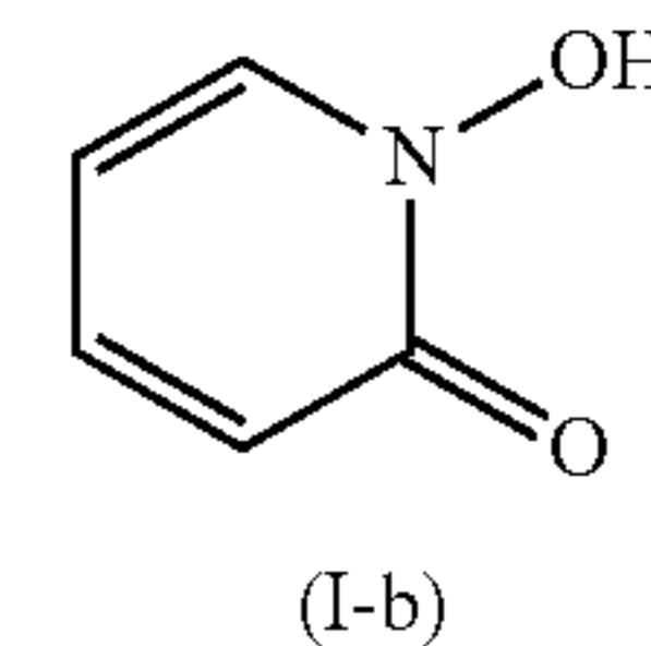
1-hydroxy-2-pyridinone (I-b) (CAS 822-89-9)
