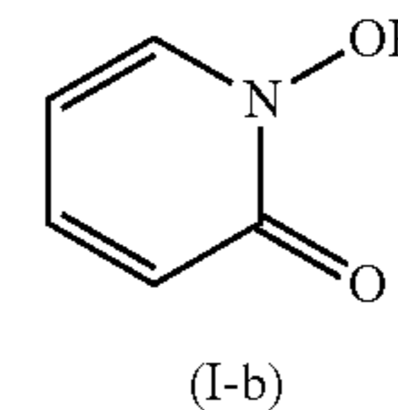
1-hydroxy-2-pyridinone (I-b) (CAS 822-89-9)
