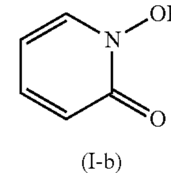
1-hydroxy-2-pyridinone (I-b) (CAS 822-89-9)
