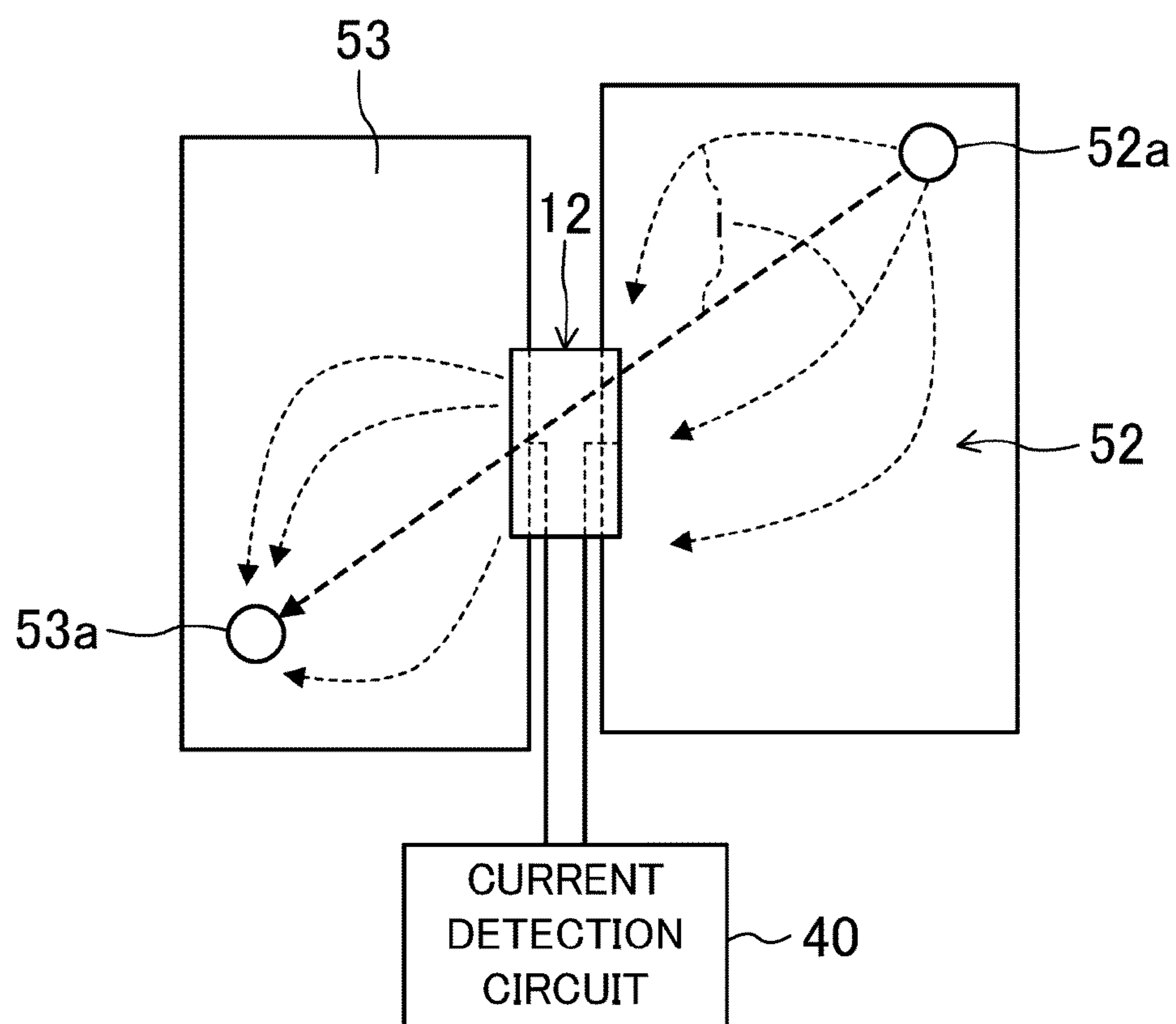
FIG. 13 PRIOR ART
