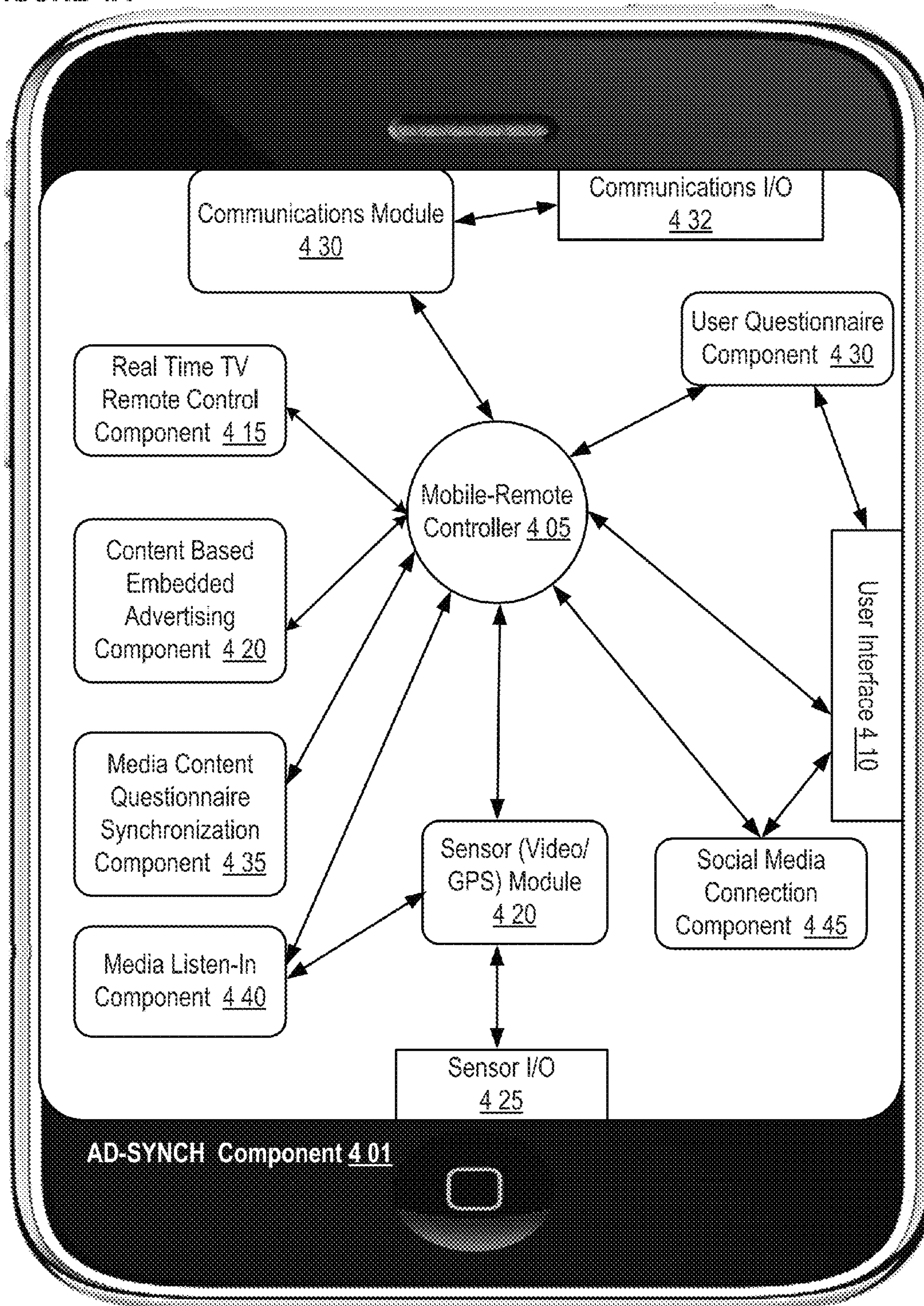
AD-SYNCH Example Client Mobile App Block View
