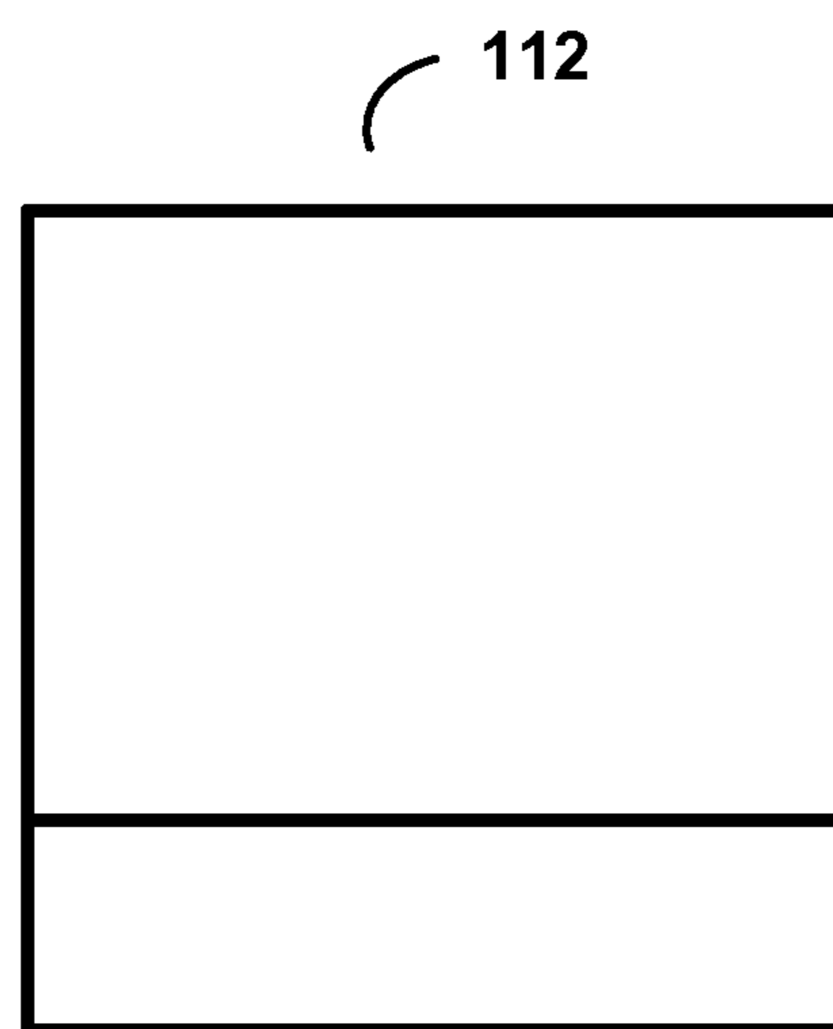
2NxnD (Inter-Prediction)
