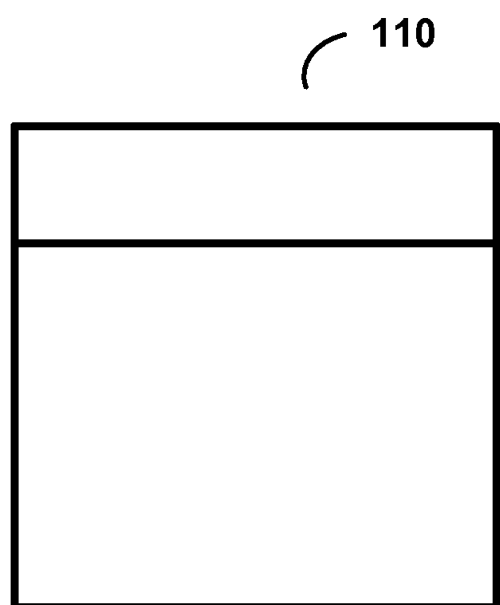
2NxnU (Inter-Prediction)
