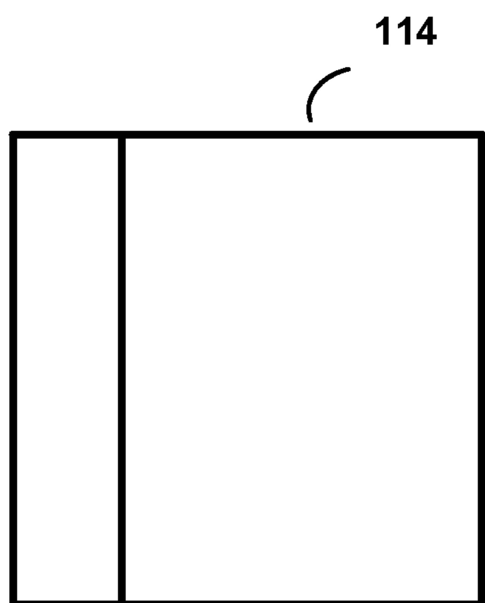
nLx2N (Inter-Prediction)
