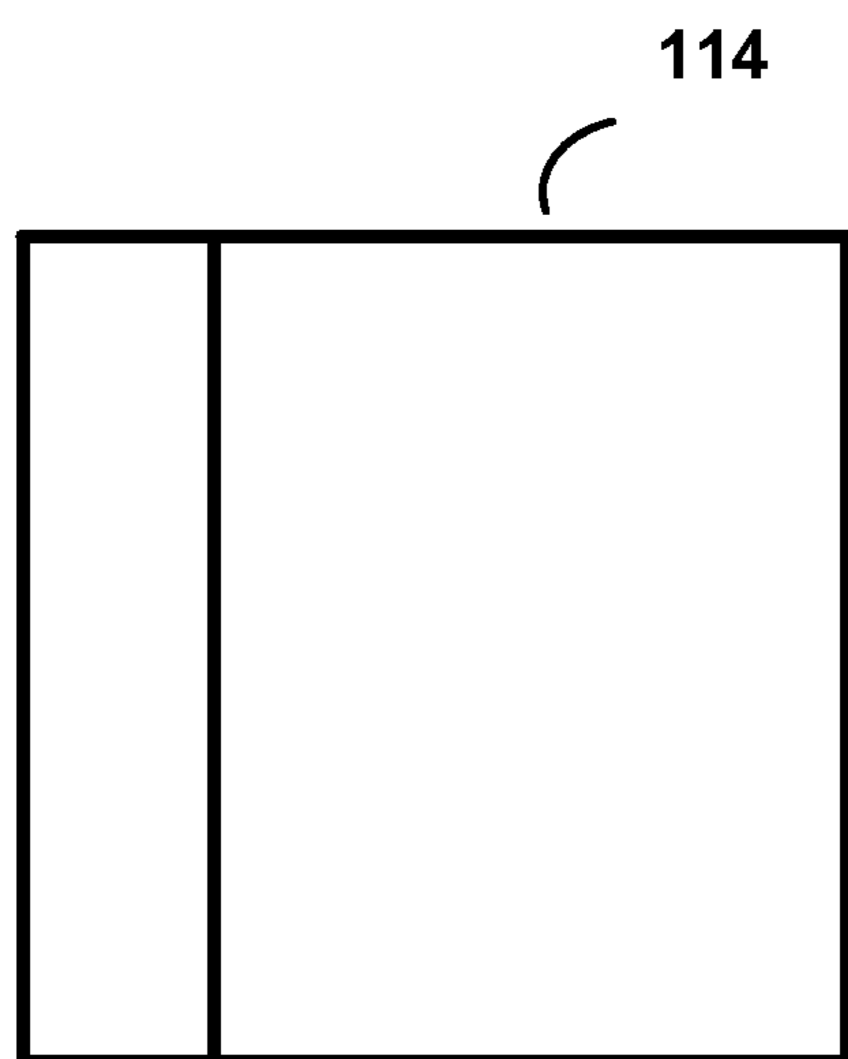
nLx2N (Inter-Prediction)
