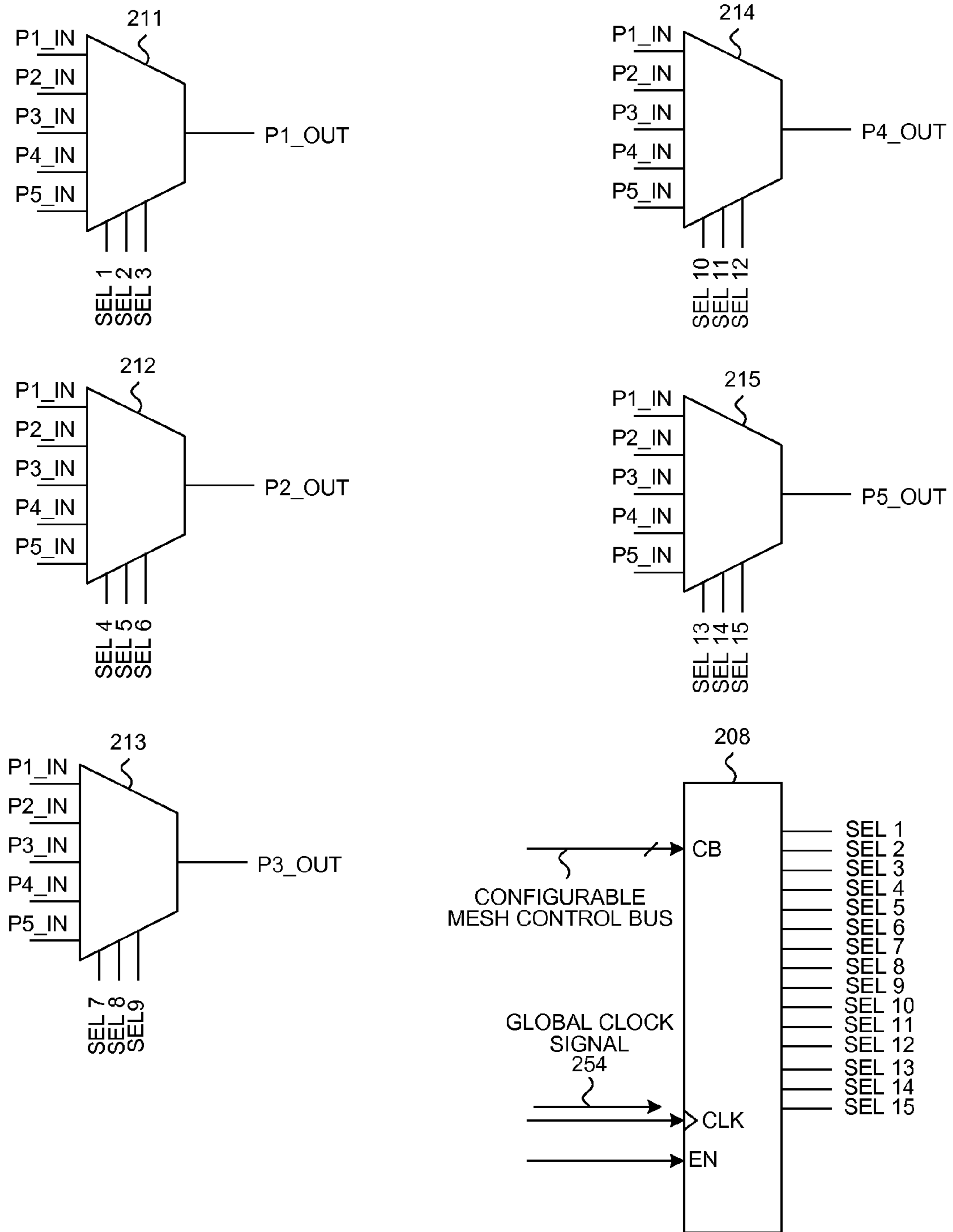
RUN TIME CONFIGURABLE SWITCH CIRCUIT
