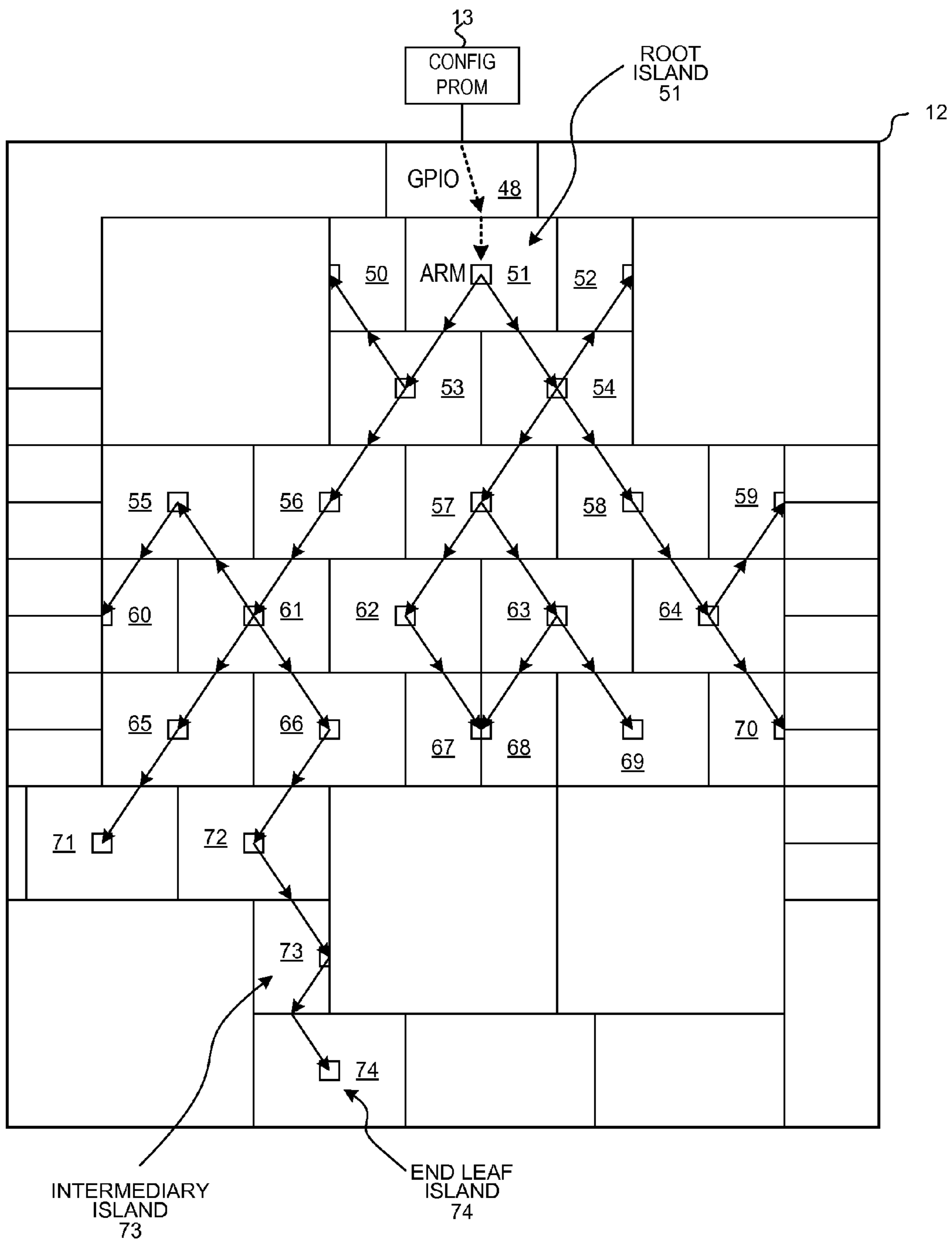
CONFIGURED CONFIGURABLE MESH CONTROL BUS
