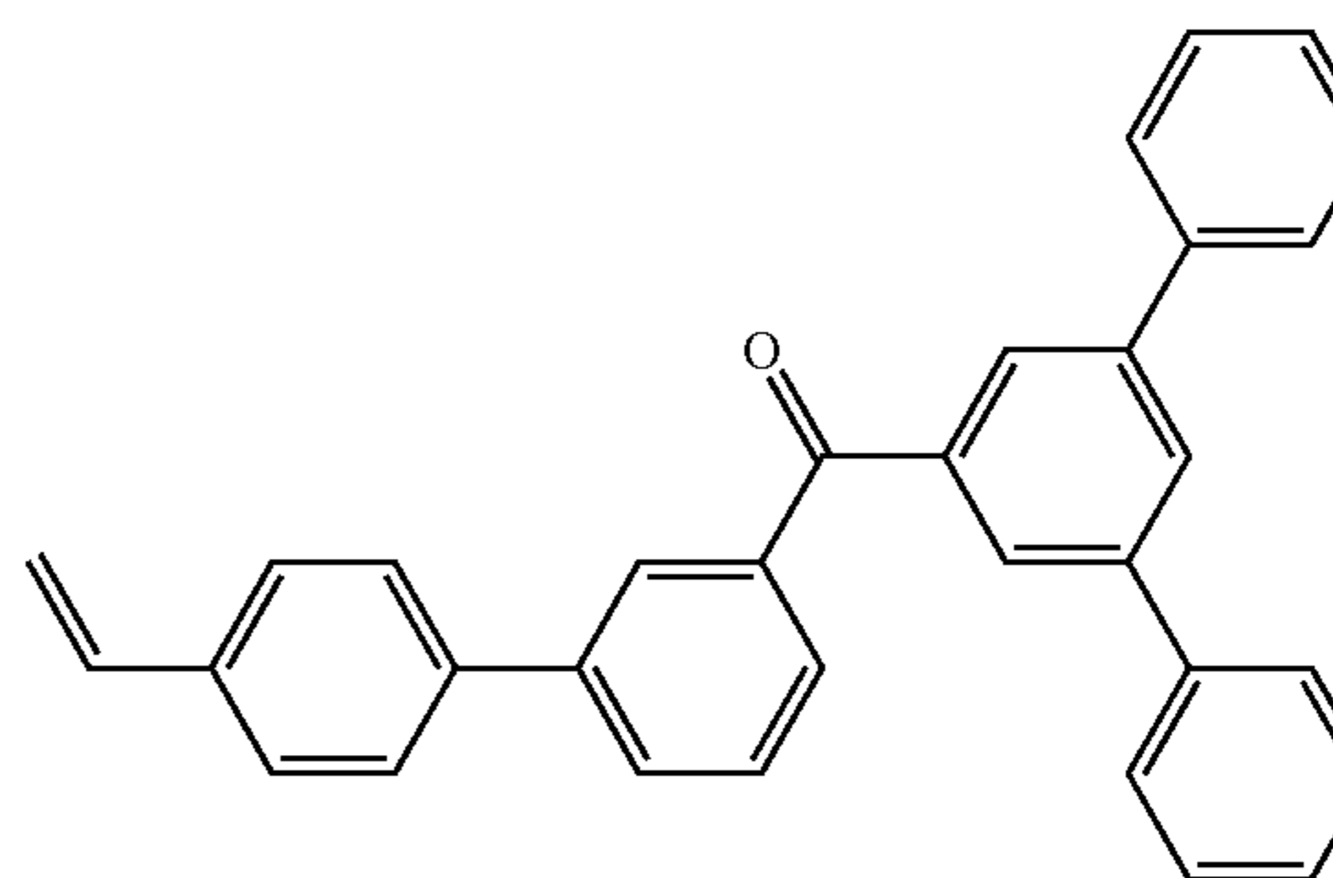
[1,1';3',1'']Terphenyl-5'-yl 4'-vinylbiphenyl-3-yl ketone (M4)
