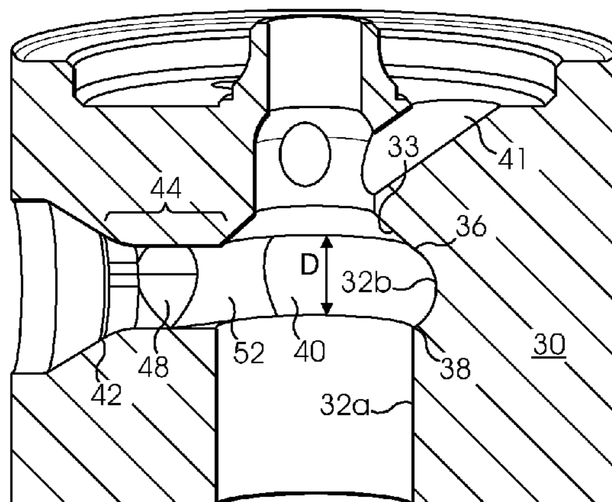
Section B-B
