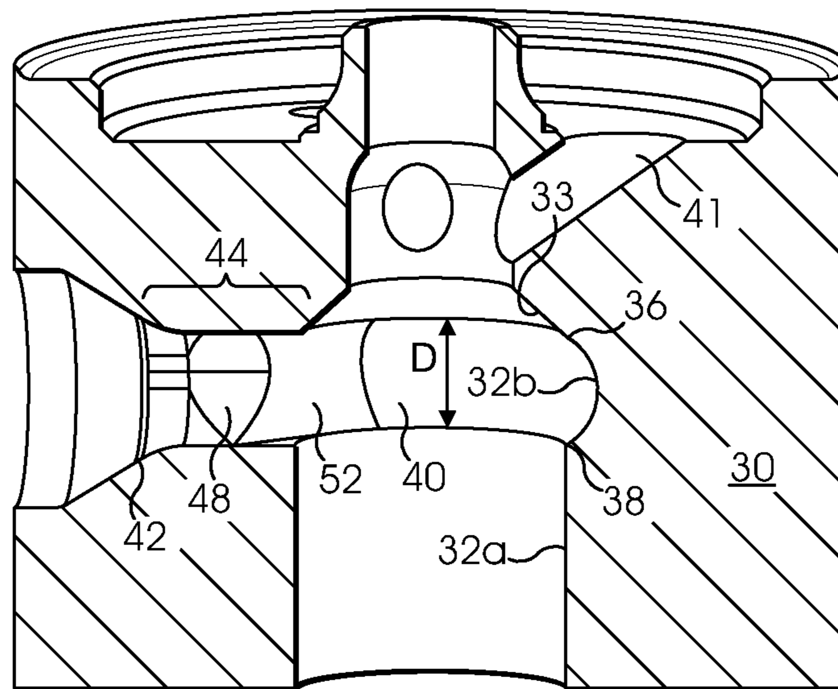
Section B-B
