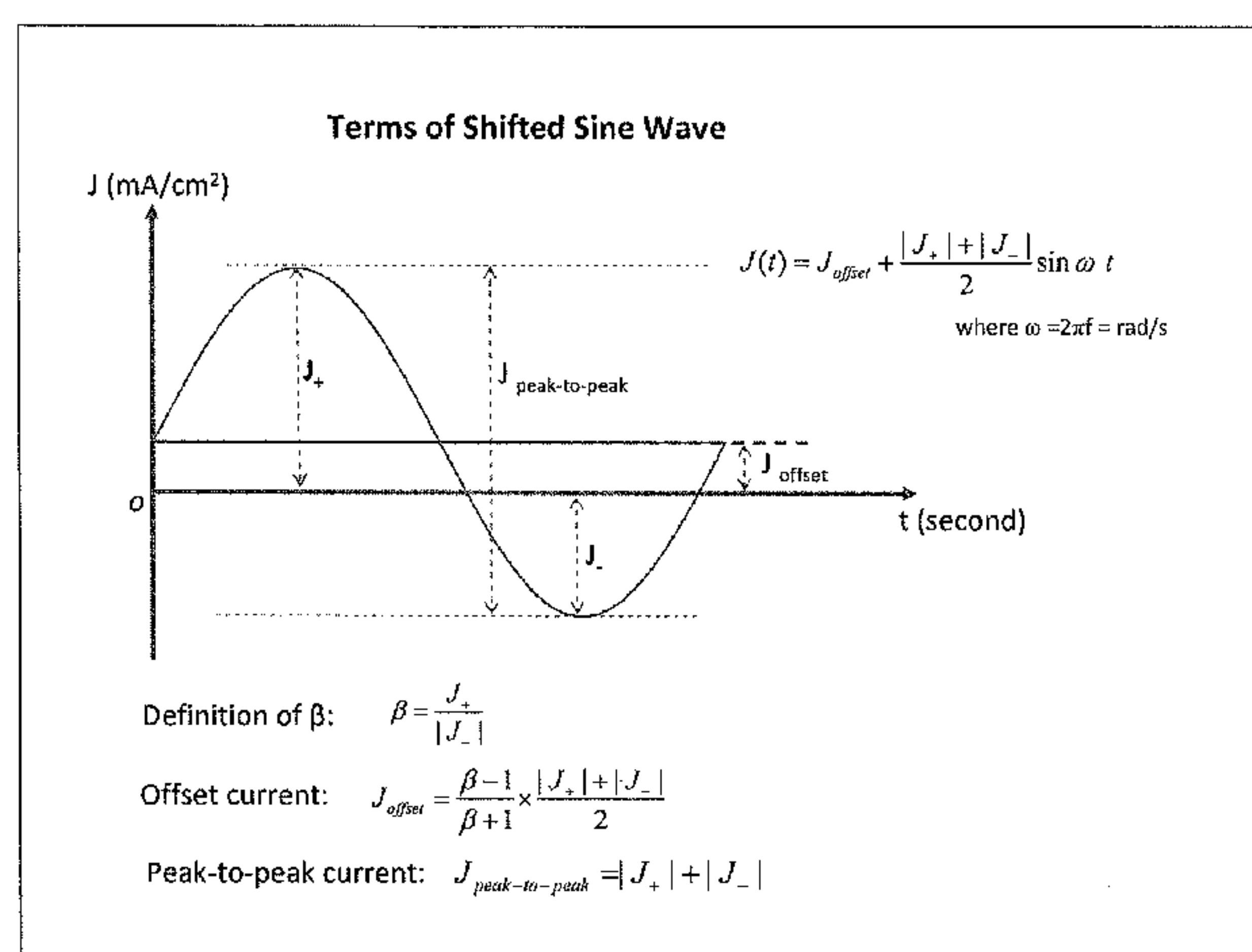
illustration of terminology used to describe shifted sine wave.
