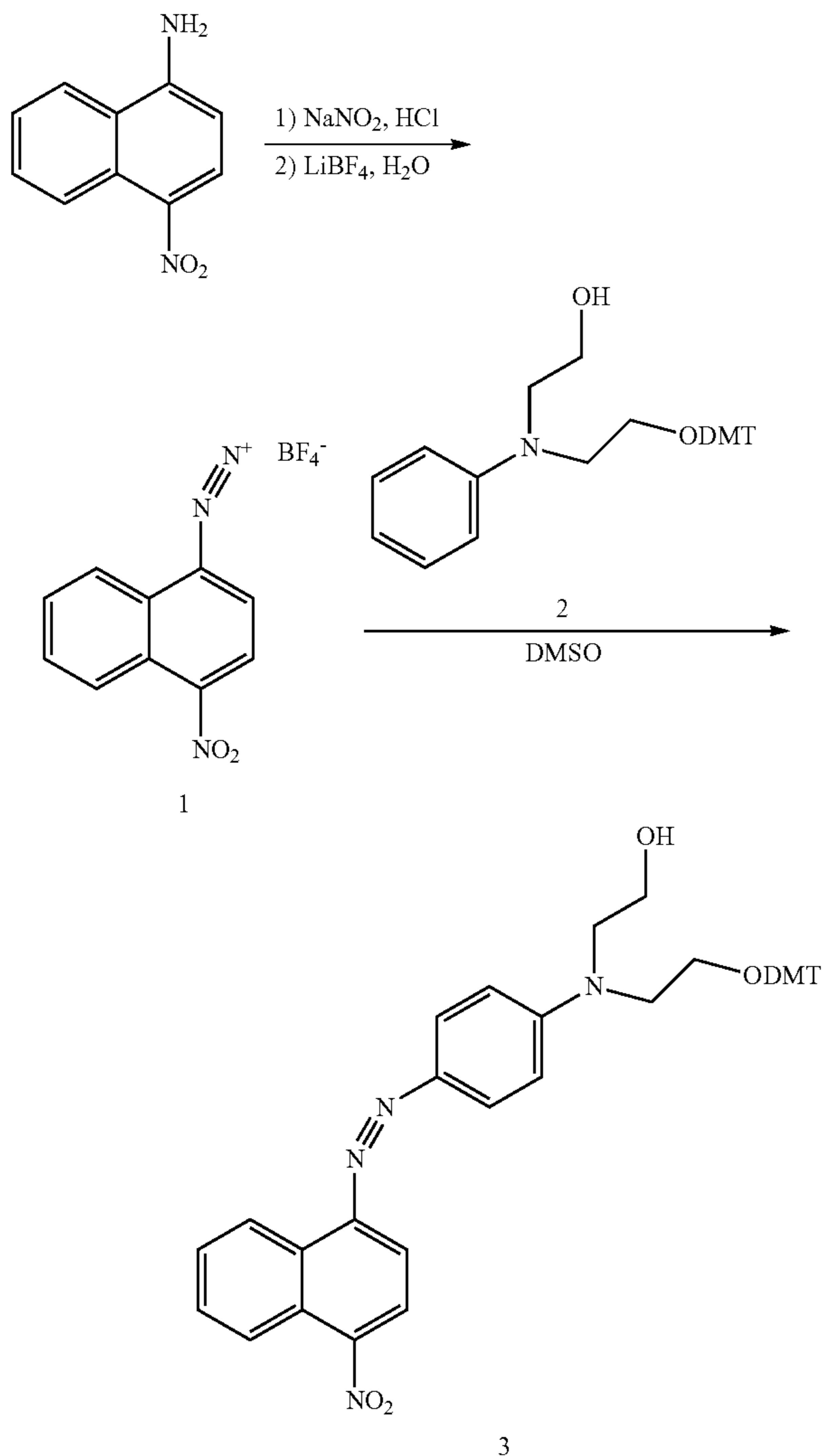
Scheme 1
