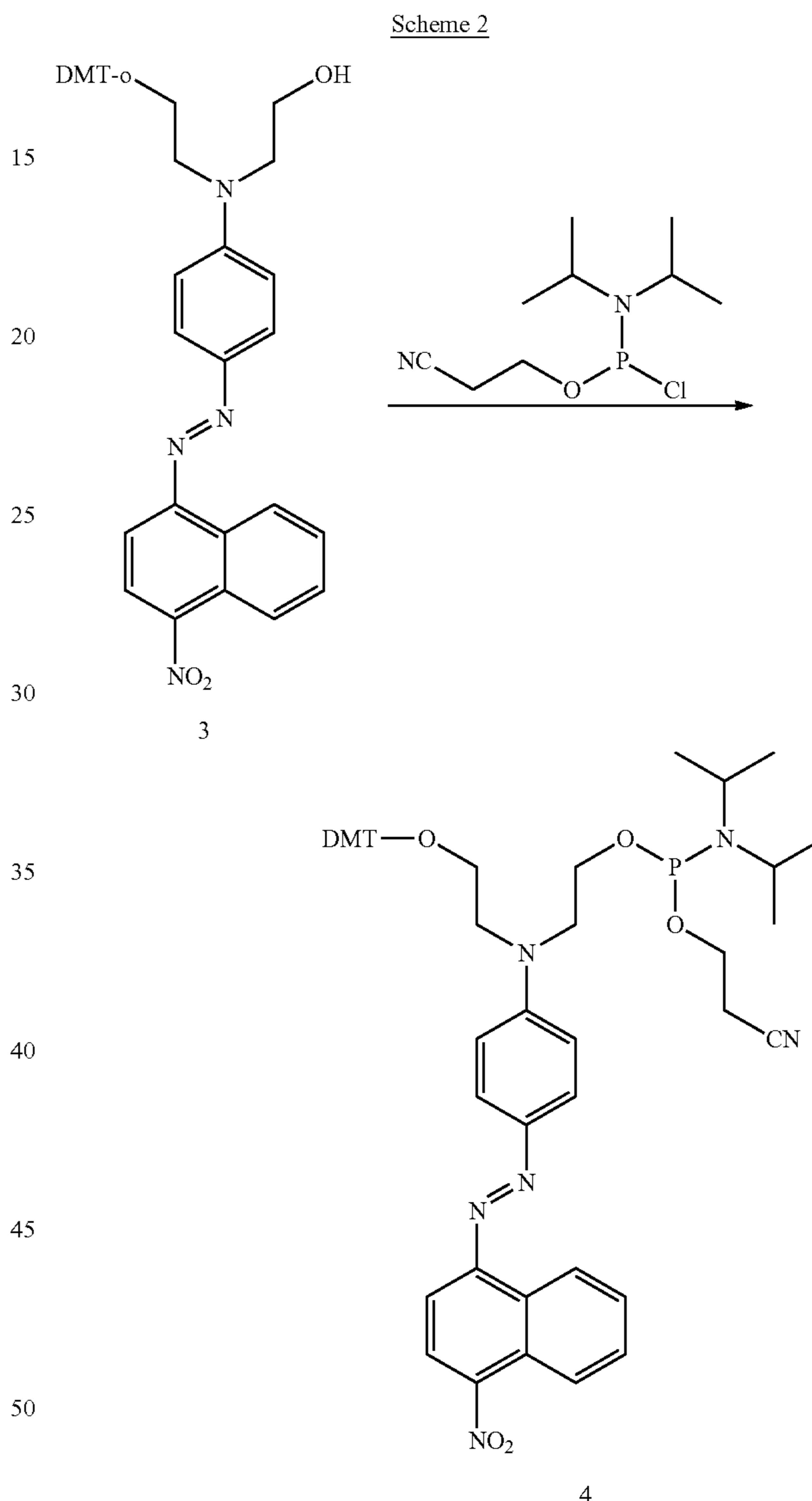
Mono-DMT-4-(1-nitro-4-naphthylazo)-N,N-diethanolamine (3)
