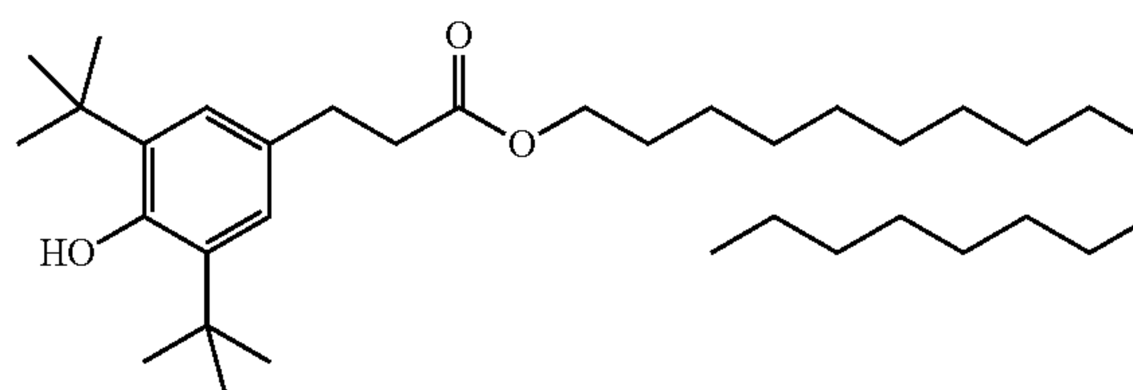
octadecyl-3(3,5-ditertbutyl-4-hydroxyphenyl)propionate (also known as IRGANOX® 1076).
