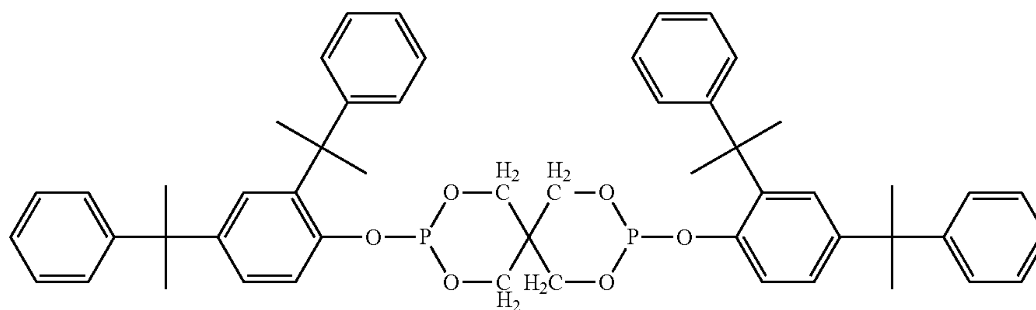
tiris (2,4-di-t-butylphenyl)phosphite (also known as IRGAPHOS® 168),
