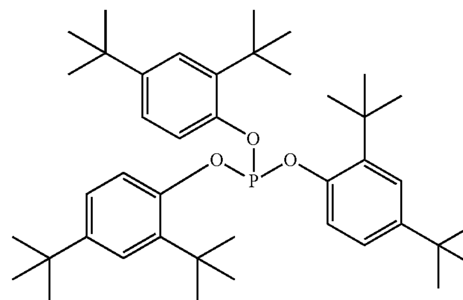
tiris (2,4-di-t-butylphenyl)phosphite (also known as IRGAPHOS® 168),
