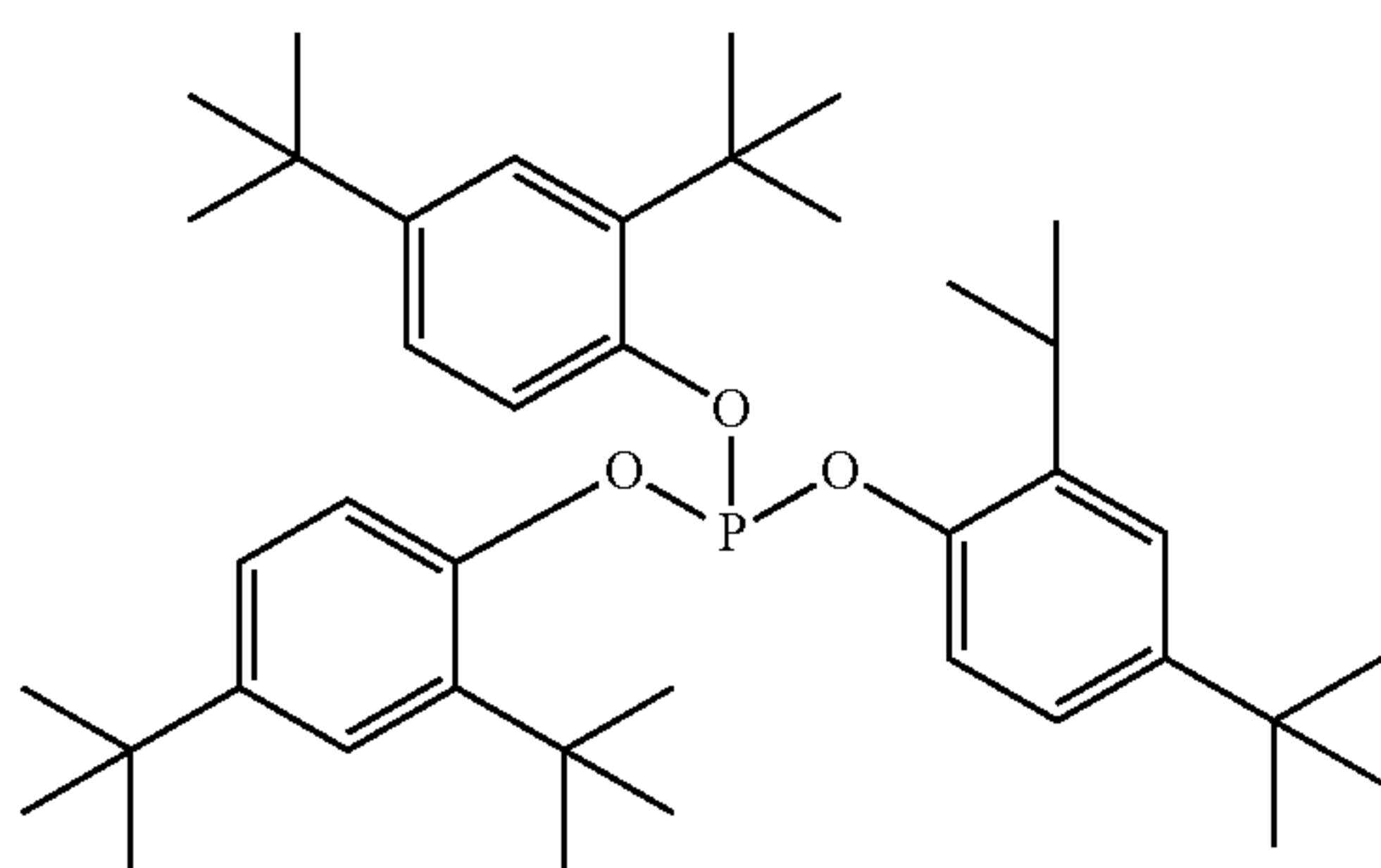
tris(2,4-di- t -butylphenyl)phosphite;
