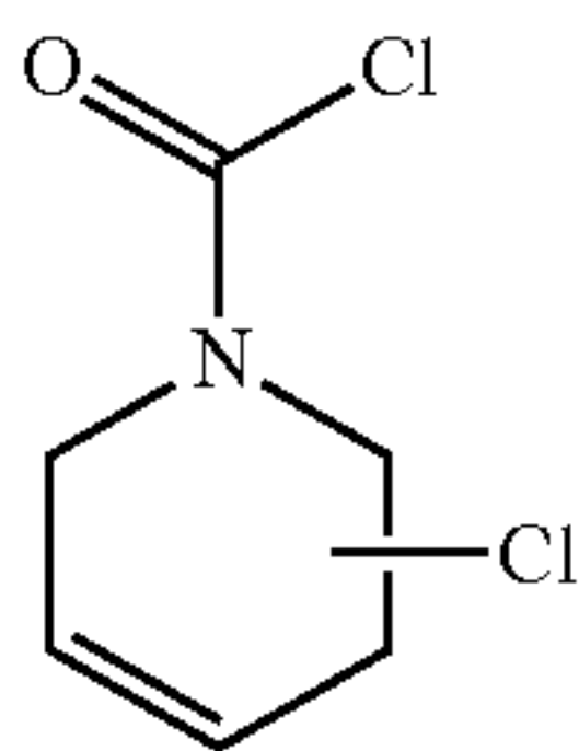
[Chemical Formula 5]
