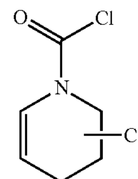
[Chemical Formula 2]
