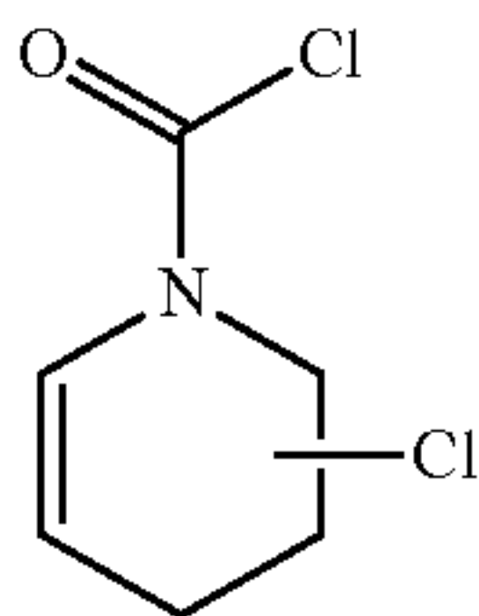
[Chemical Formula 5]
