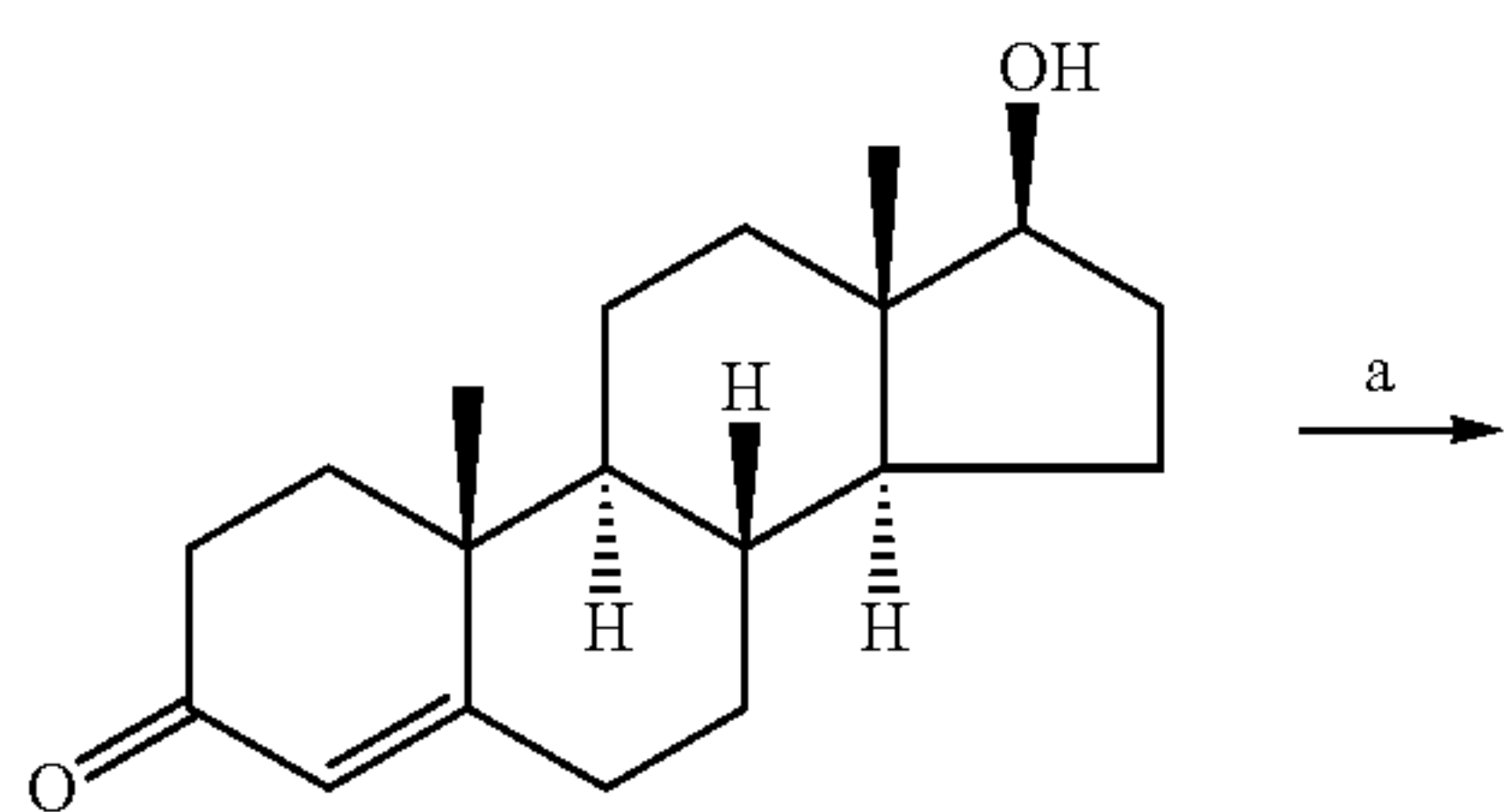
Scheme 7
