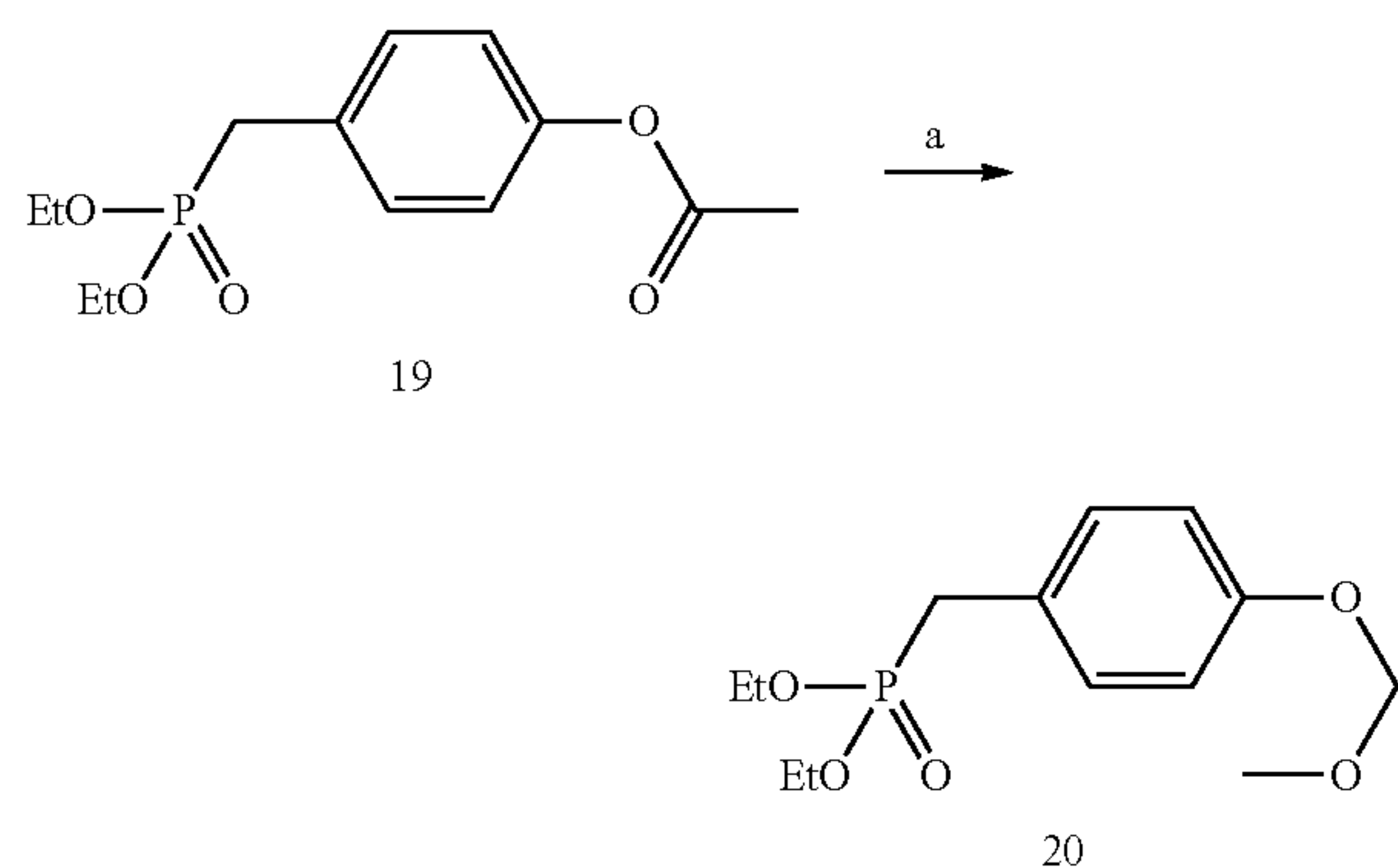
Scheme 4
