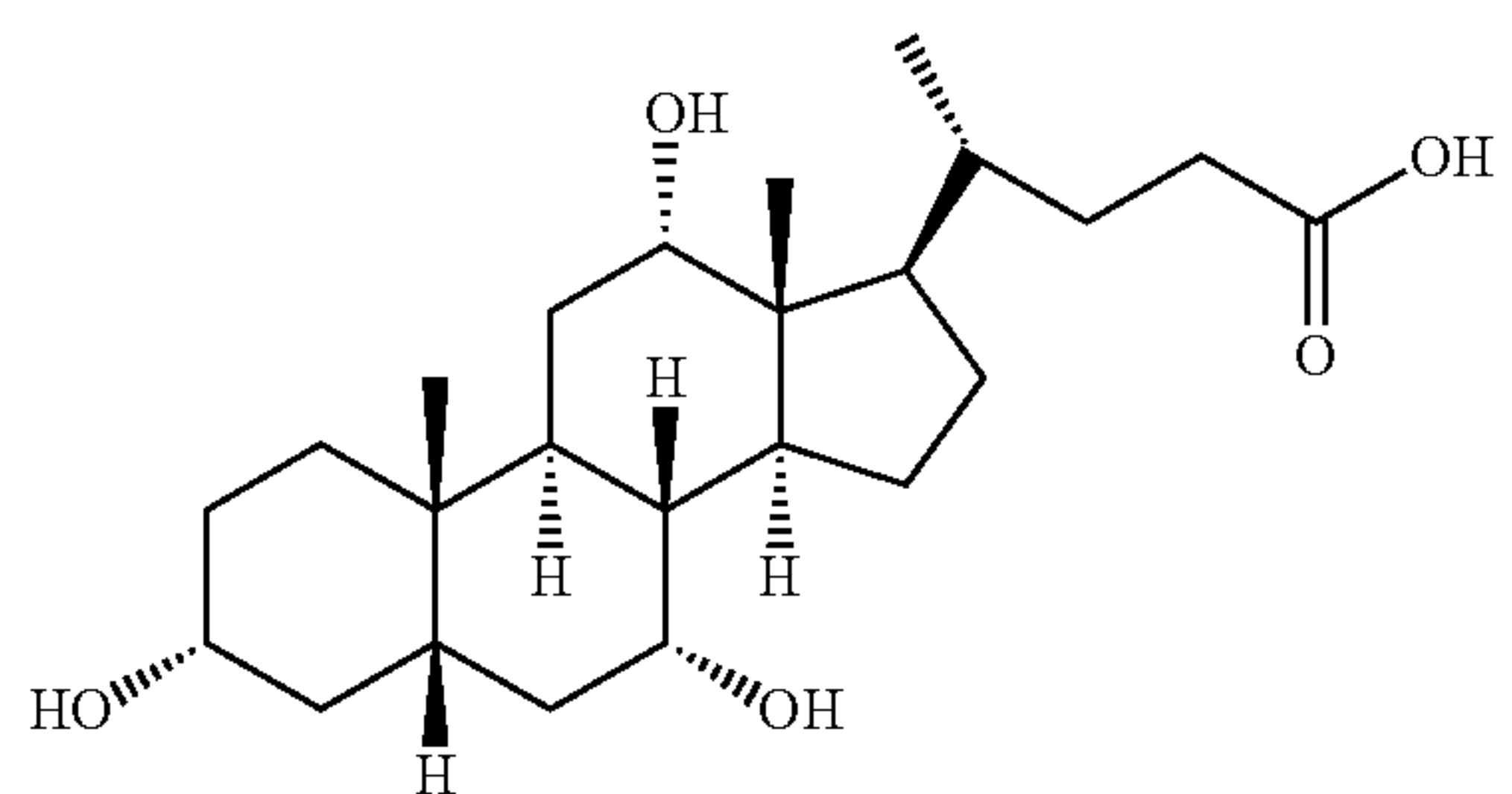
Cholic acid
