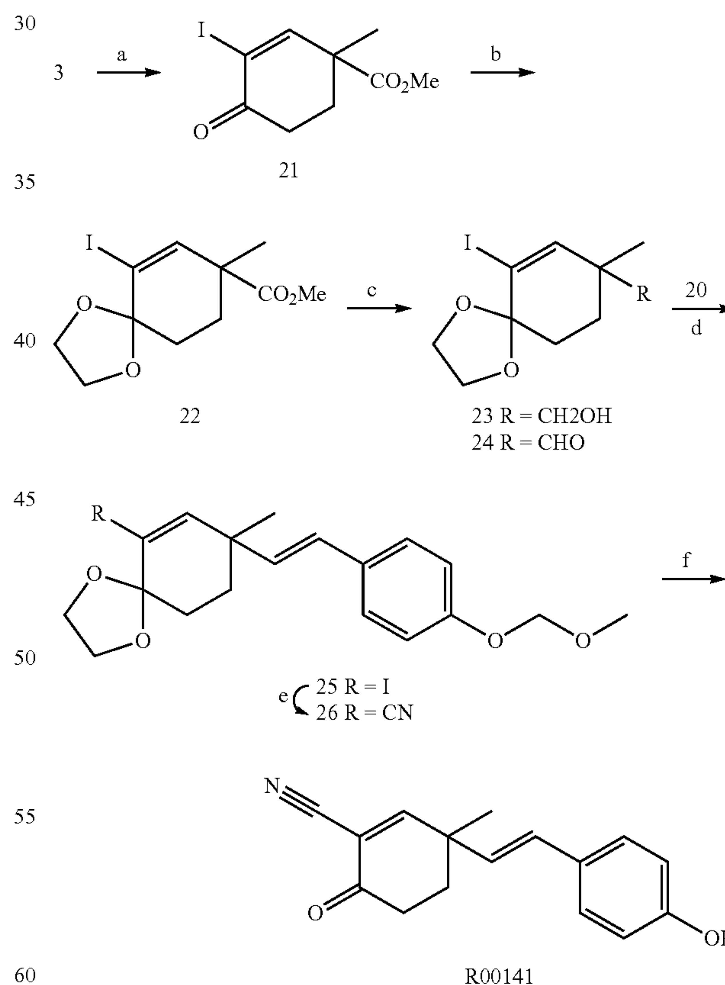
Scheme 5
