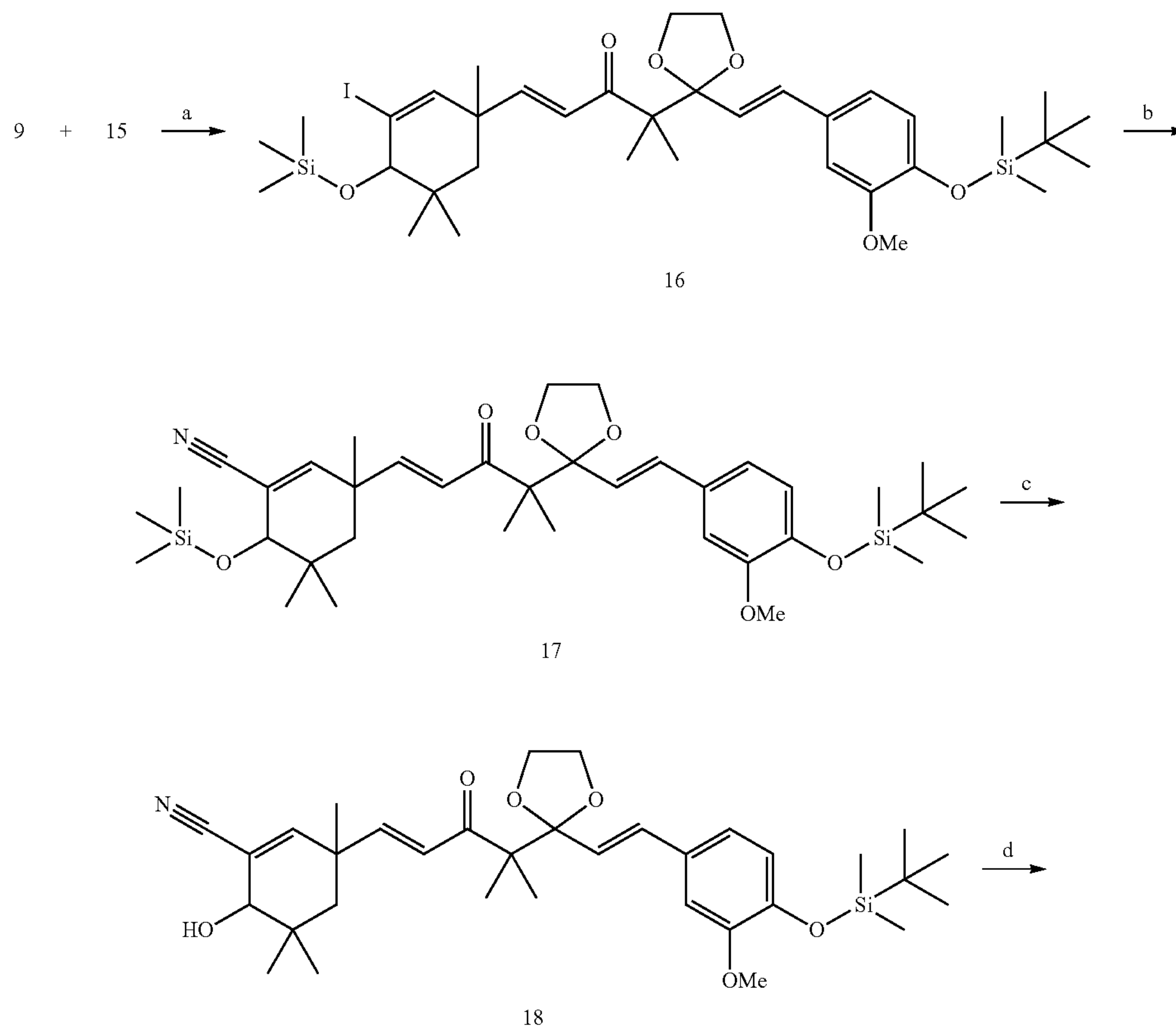
Scheme 3
