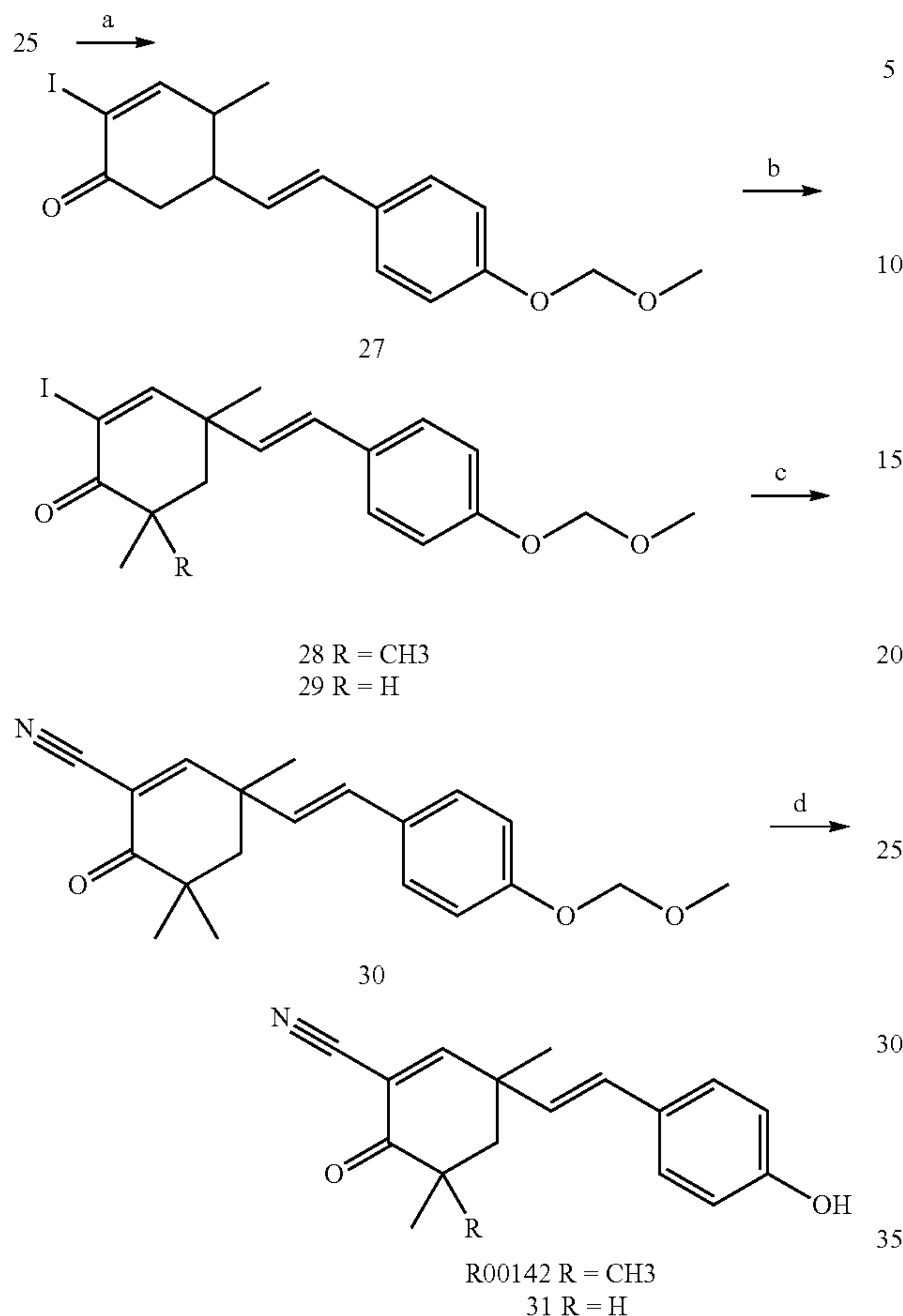
Scheme 6
