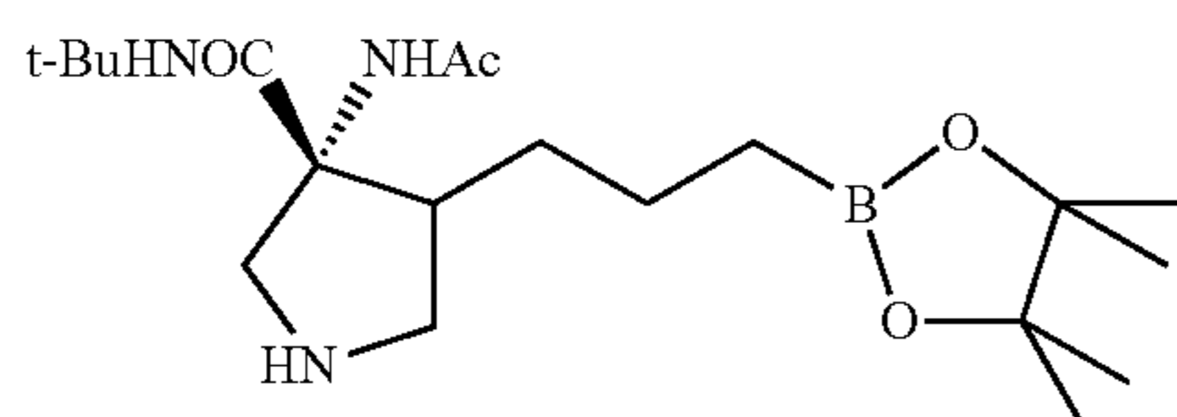
Step 8: (3R,4S)-3-Acetamido-N-tert-butyl-4-[3-(4,4, 5,5-tetramethyl-1,3,2-dioxaborolan-2-yl)propyl]pyrro- lidine-3-carboxamide hydrochloride (racemate)
