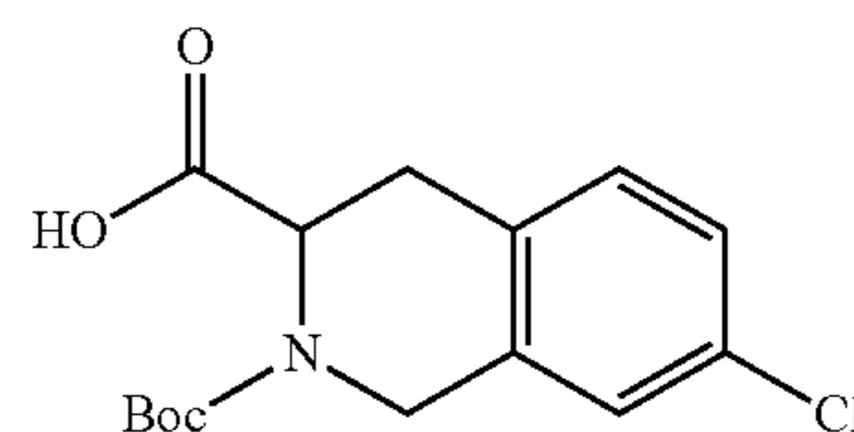
Step 5: 2-(tert-Butoxycarbonyl)-7-chloro-1,2,3,4- tetrahydroisoquinoline-3-carboxylic acid
