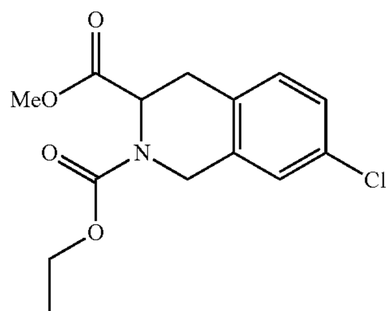
Step 3: 2-Ethyl 3-methyl 7-chloro-3,4-dihydroisoquinoline-2,3(1 H)-dicarboxylate
