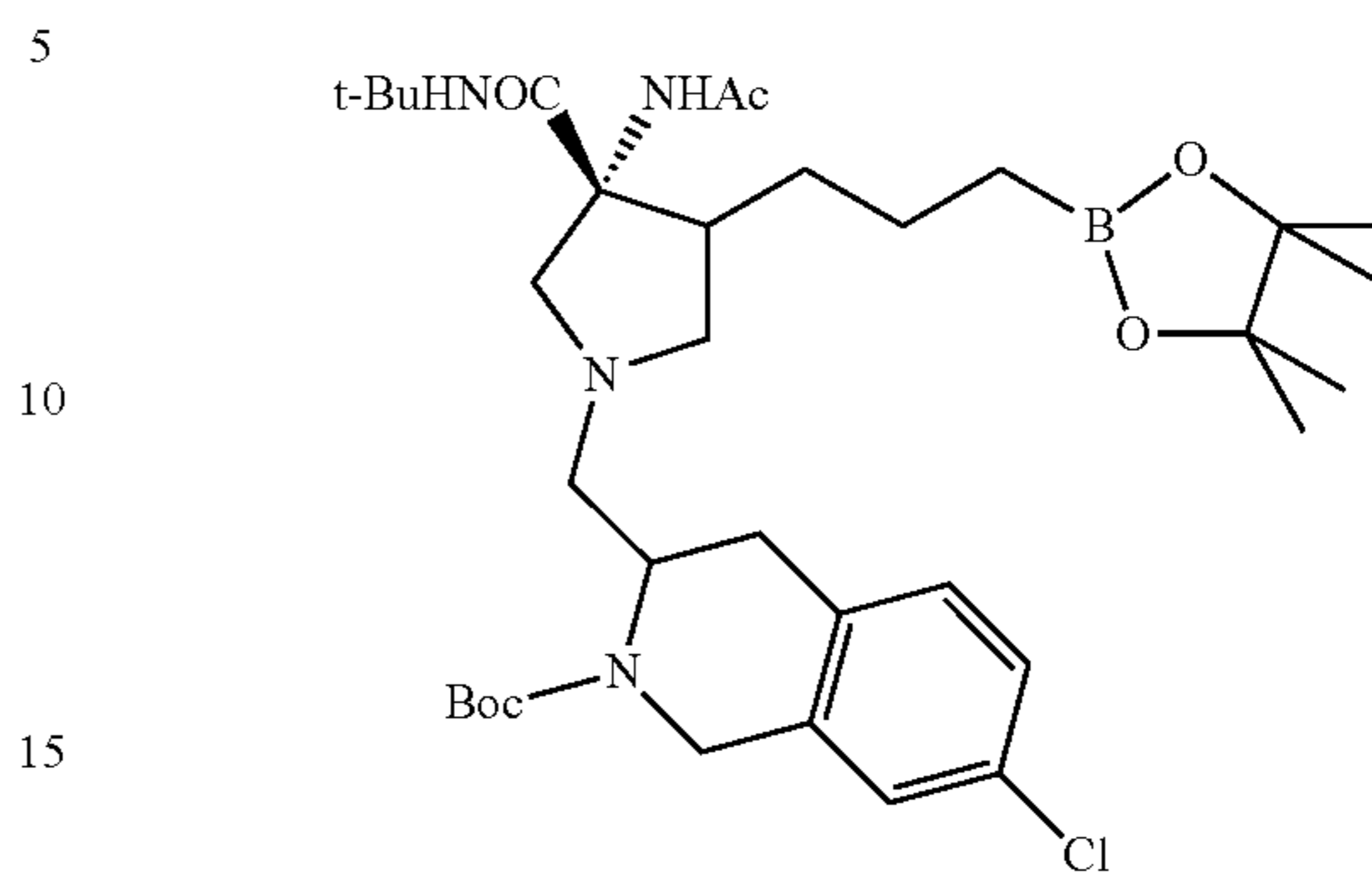
Step 9: tert-Butyl 3-({(3R,4S)-3-acetamido-3-(tert- butylcarbamoyl)-4-[3-(4,4,5,5-tetramethyl-1,3,2- dioxaborolan-2-yl)propyl]pyrrolidin-1-yl}methyl)-7- chloro-3,4-dihydroisoquinoline-2(1 H)-carboxylate
