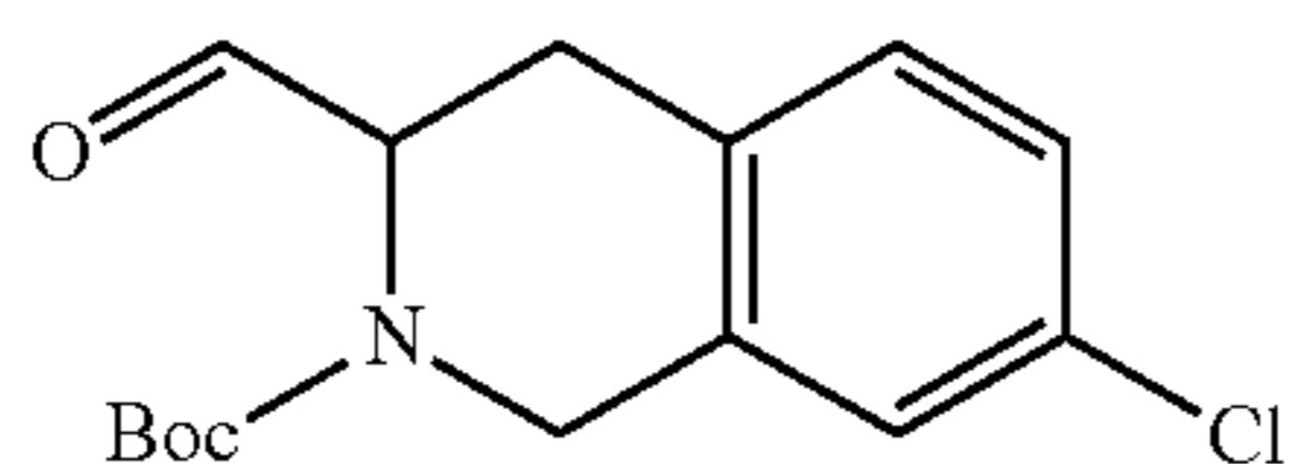
Step 7: tert-Butyl 7-chloro-3-formyl-3,4-dihydroisoquinoline-2(1 H)-carboxylate
