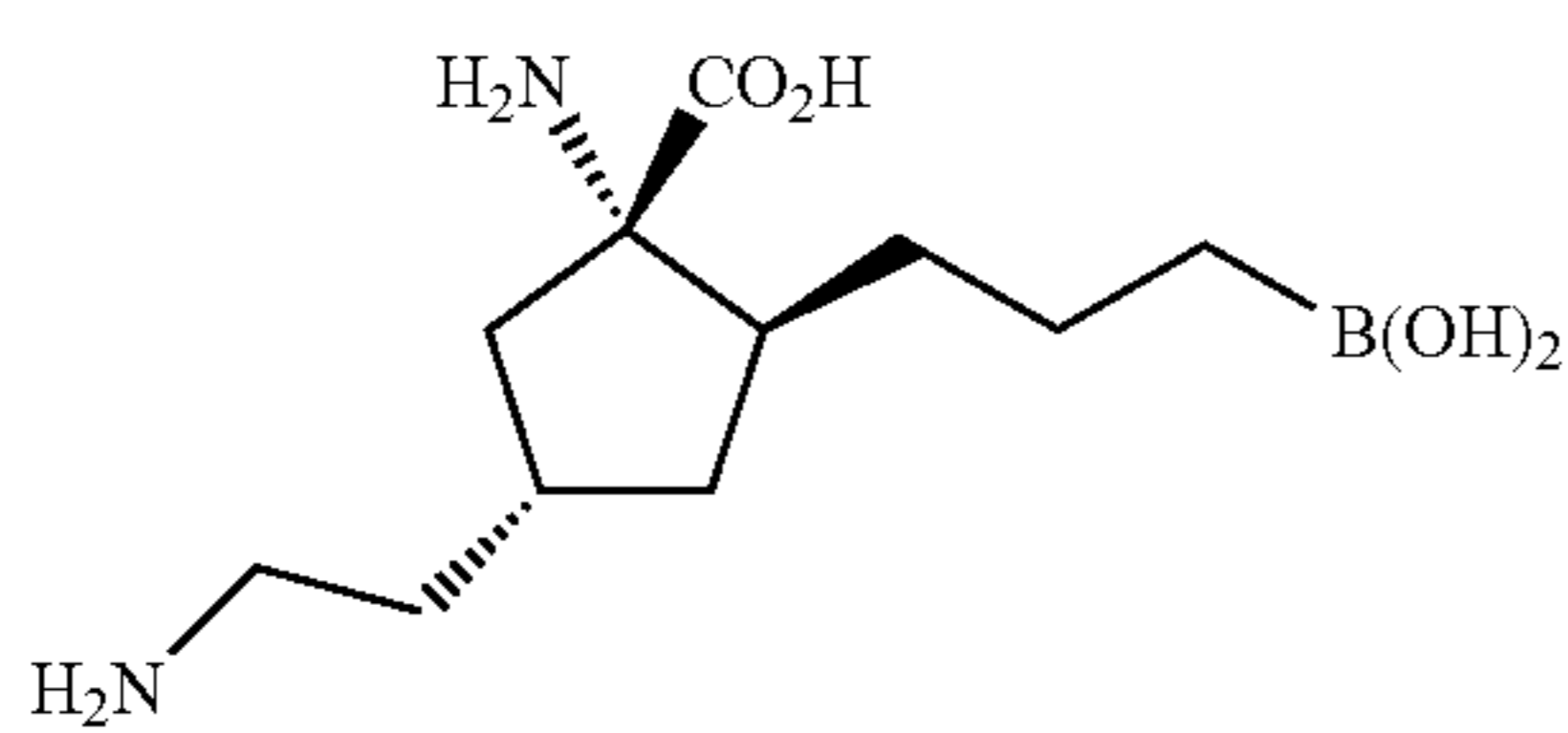
Step 6: (1S,2S,4R)-1-amino-4-(2-aminoethyl)-2-(3-boronopropyl)cyclopentanecarboxylic acid
