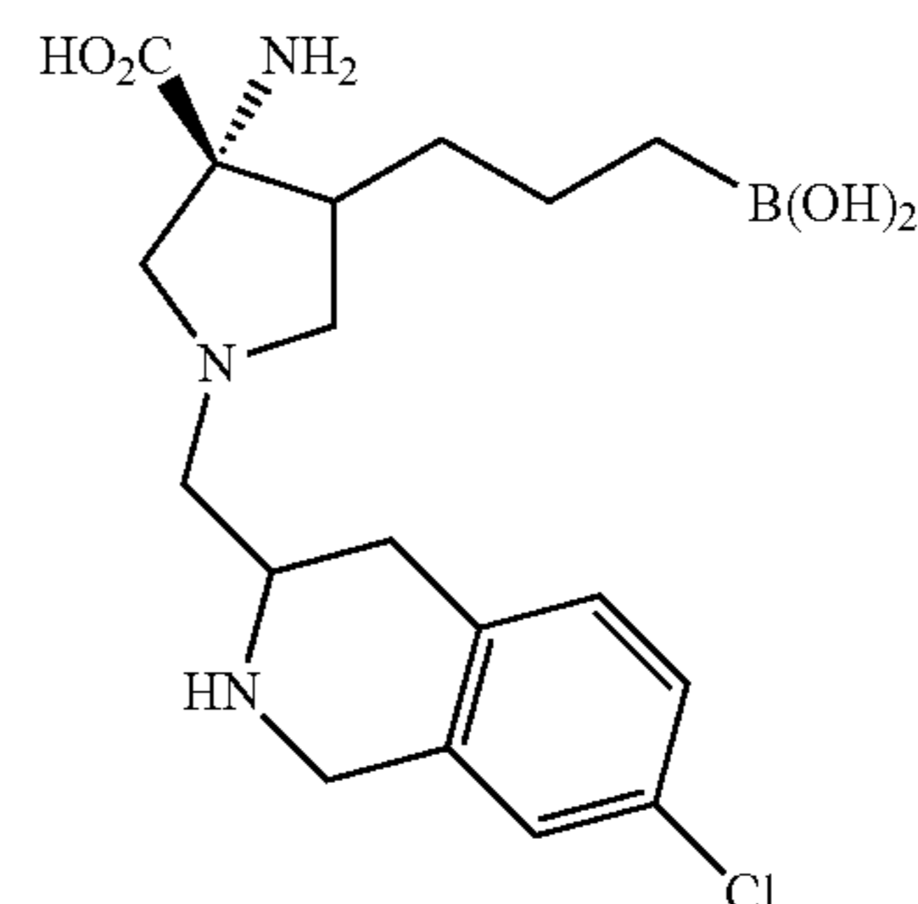
Step 10: (3R,4S)-3-Amino-1-[(7-chloro-1,2,3,4-tet- rahydroisoquinolin-3-yl)methyl]-4-[3-(dihydroxybo- rlyl)propyl]pyrrolidine-3-carboxylic acid trihydro- chloride (mixture of 2 diastereomers, each a racemate)
