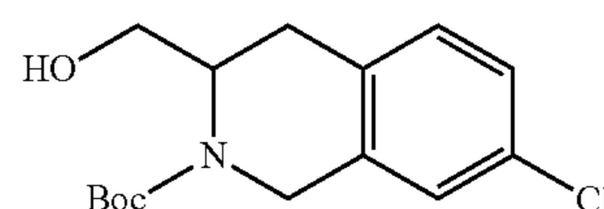
Step 6: tert-Butyl 7-chloro-3-(hydroxymethyl)-3,4- dihydroisoquinoline-2(1 H)-carboxylate
