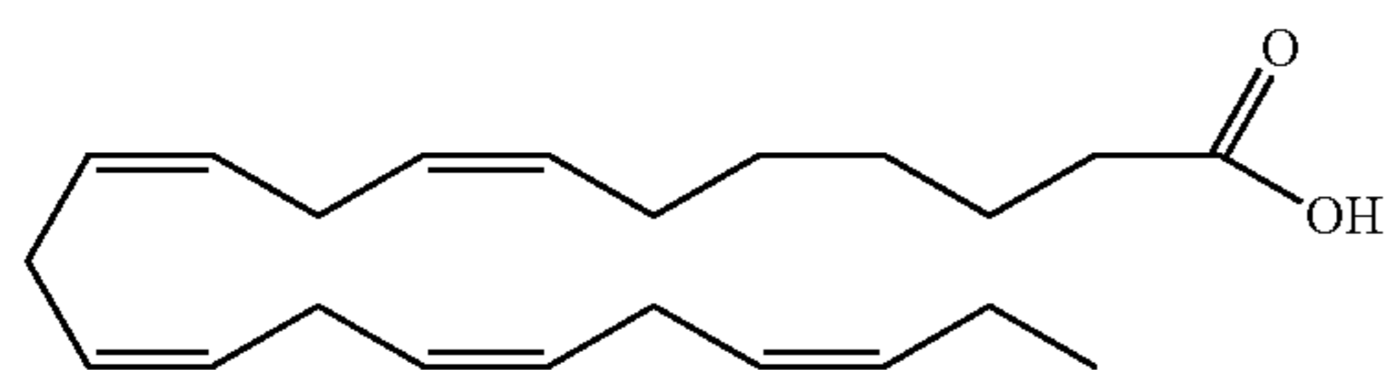
omega-3 docosapentaenoic acid
