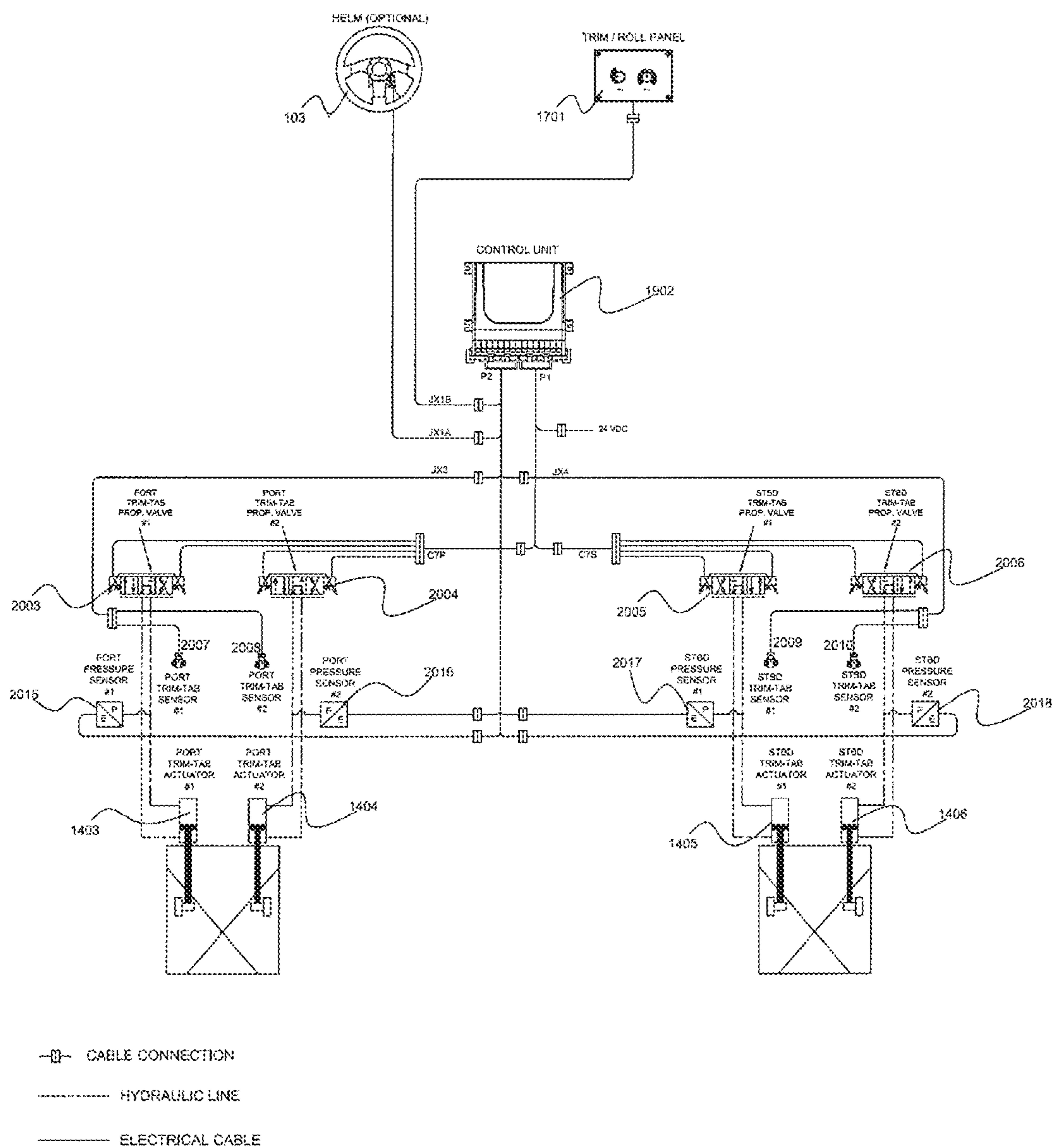
FIGURE 20 SYSTEM DIAGRAM 1DOF TRIM-TAB INTEGRATED WITH WATERJETTS
