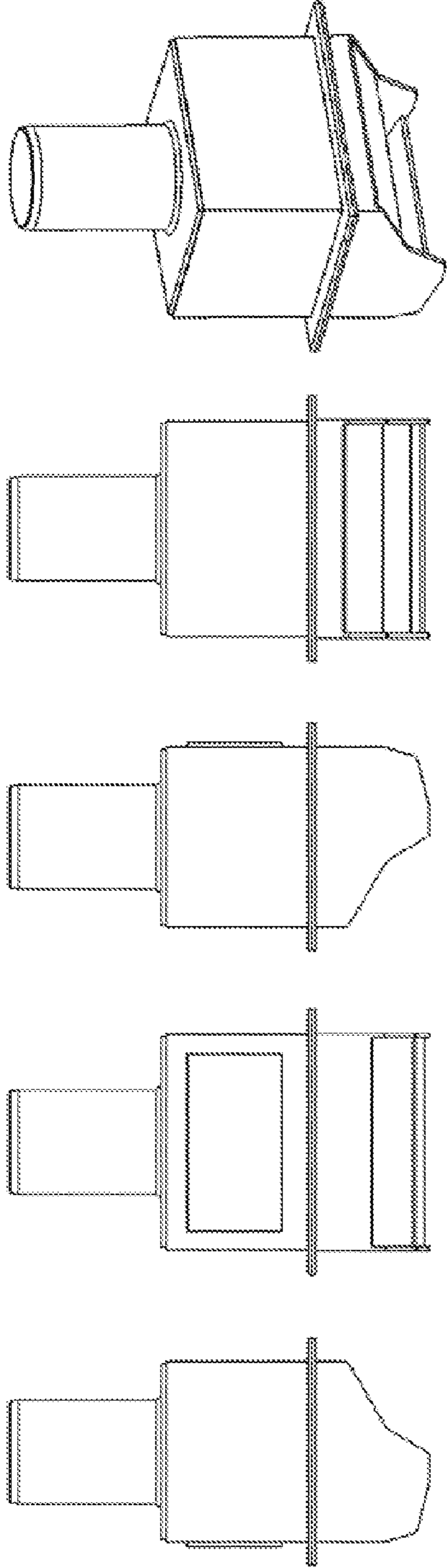
Perspective view
