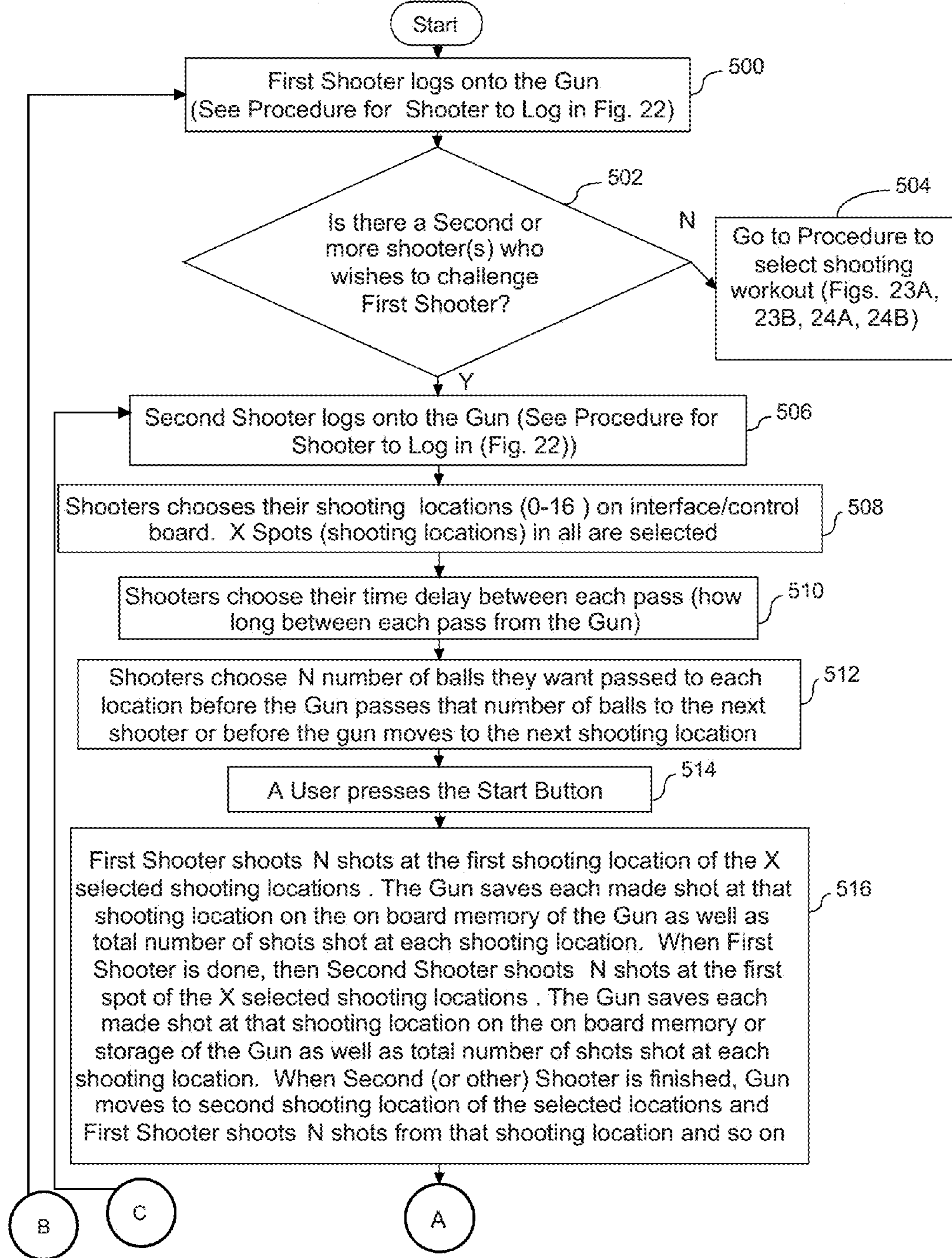
FIG. 28A NOT DEPENDENT ON DOPPLER PROCEDURE TO USE REAL TIME CHALLENGE MODE ON THE GUN FOR TWO PLAYERS TO LOG INTO THE SAME GUN AND SHOOT AGAINST EACH OTHER
