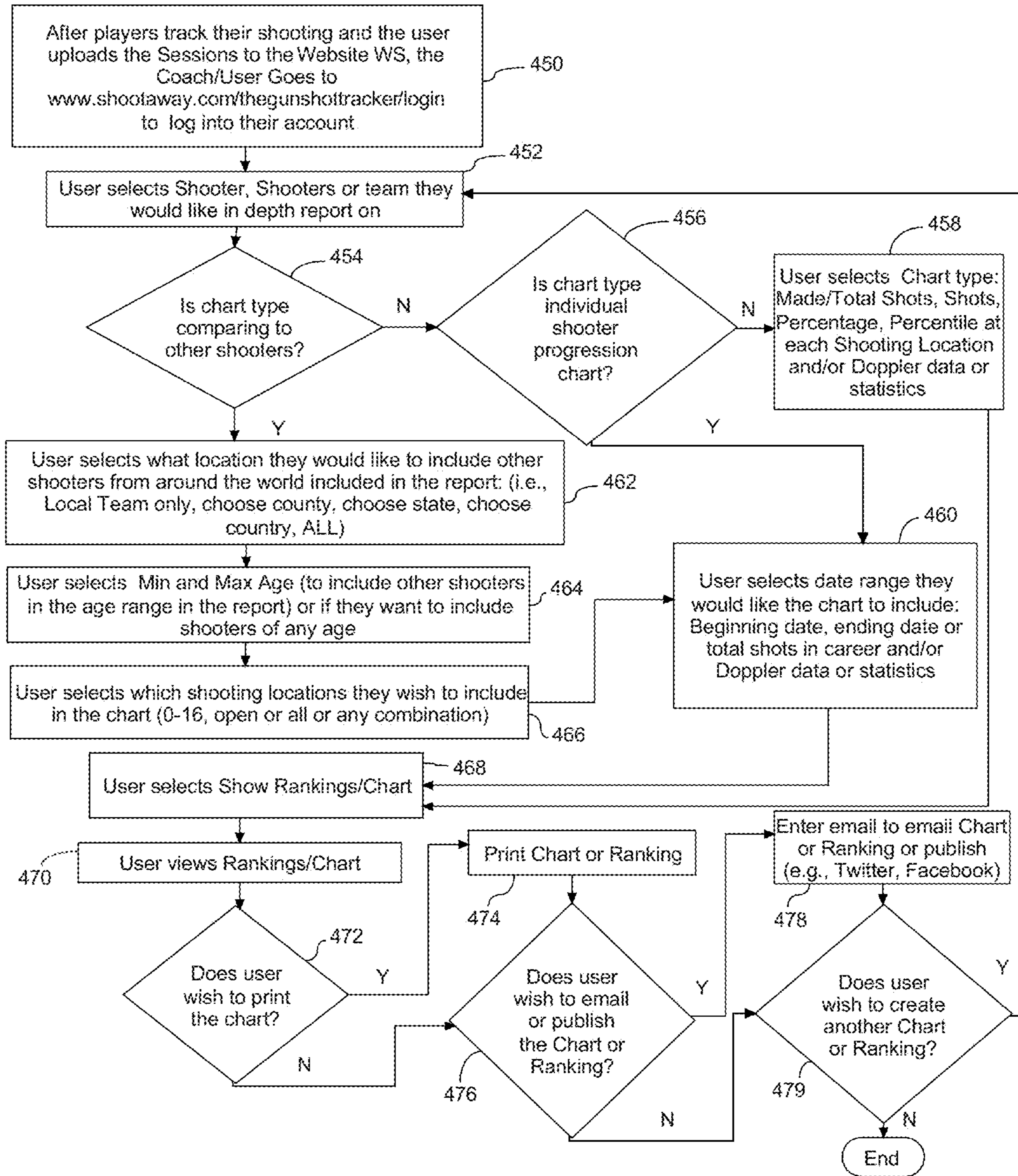
FIG. 27 NOT DEPENDENT ON DOPPLER OR DOPPLER DEPENDENT Procedure to Create Customized Reports on Website
