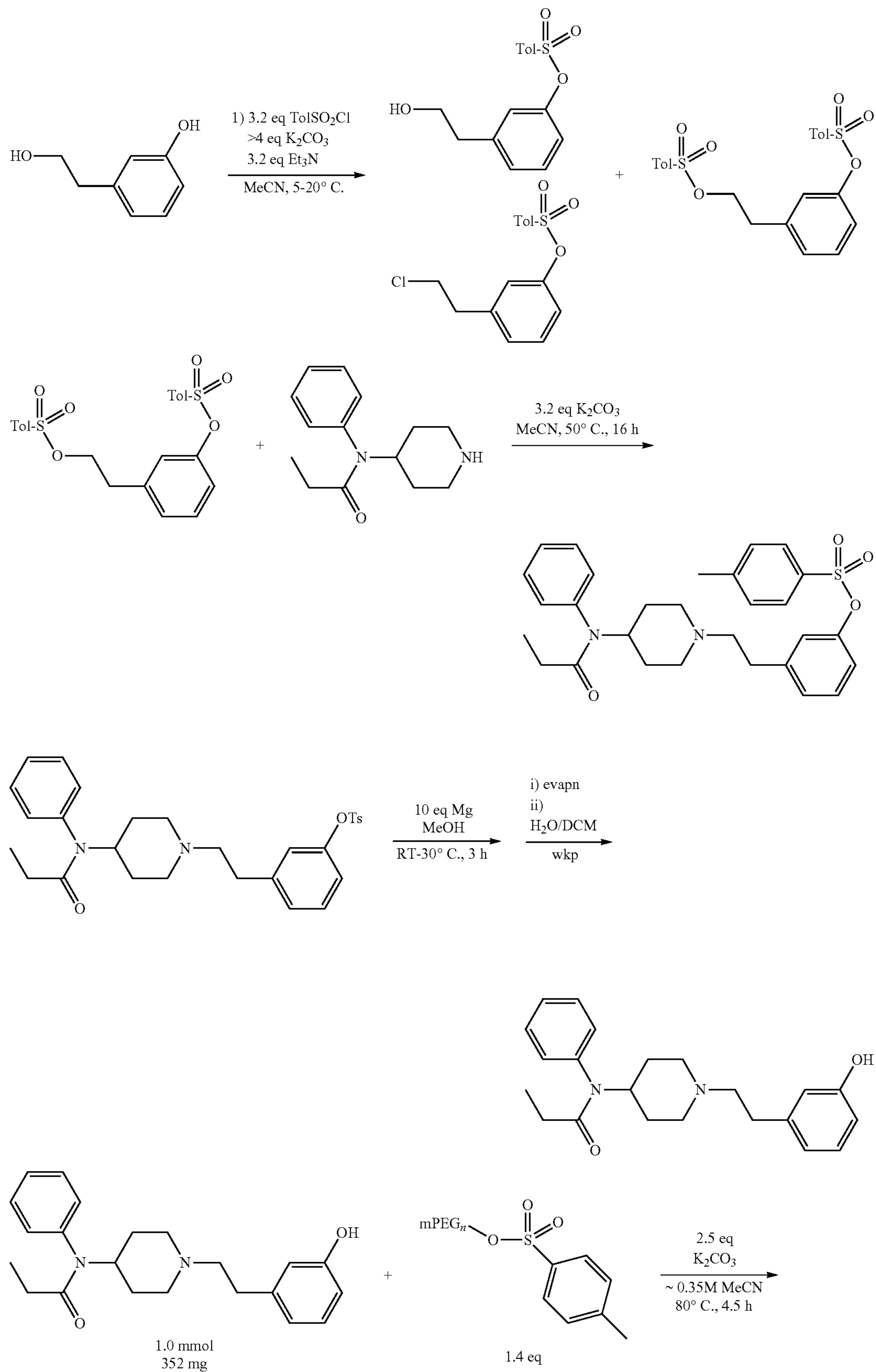
Scheme 11-B
