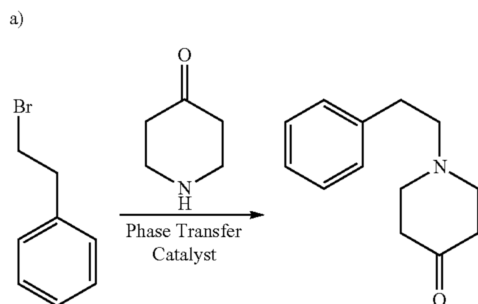
Scheme 11-C
