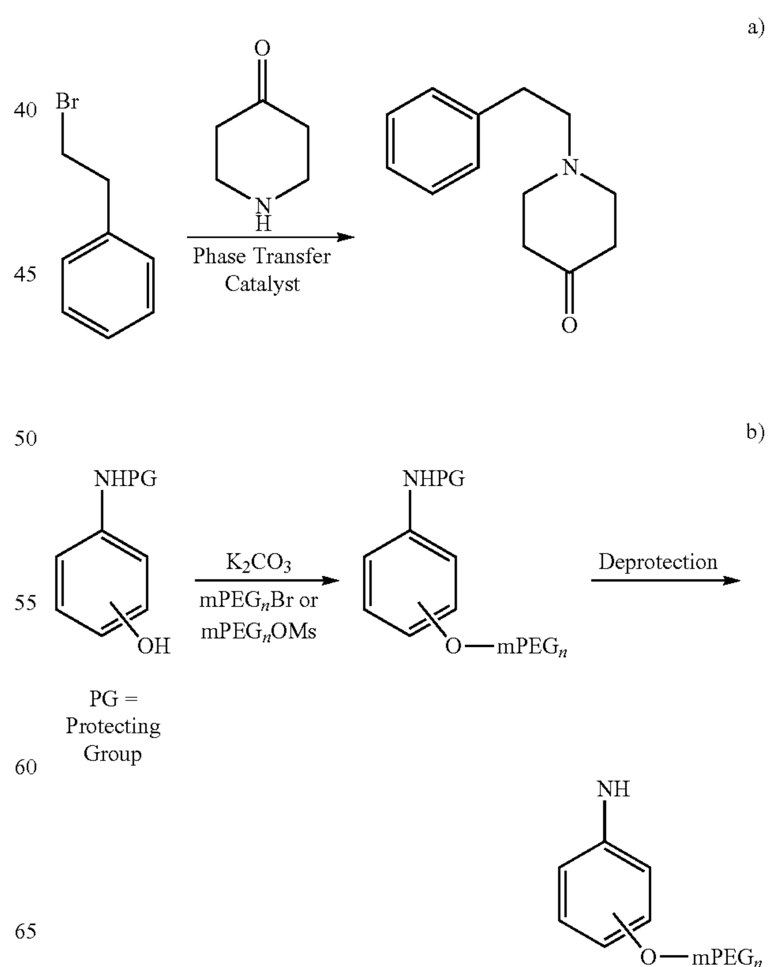
Scheme 11-C
