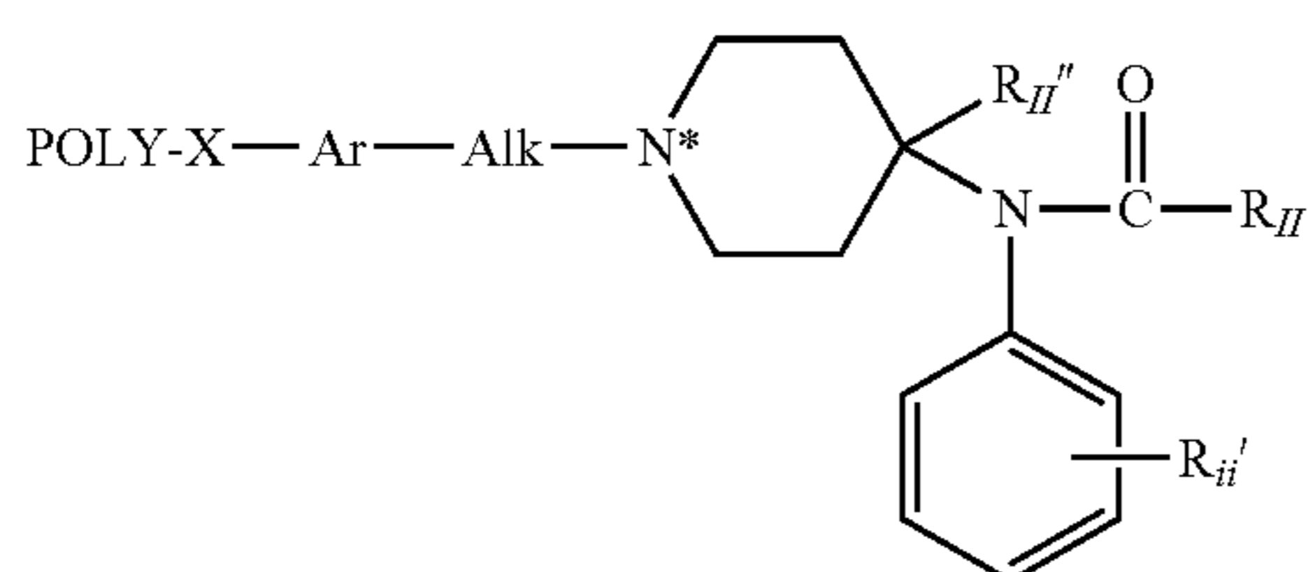
Formula II-Cb
