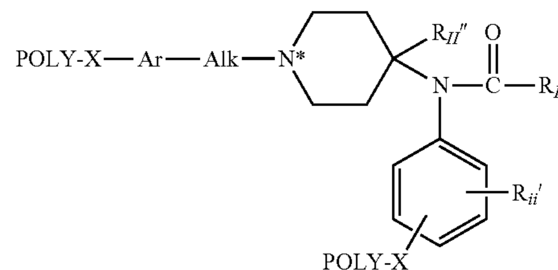
Formula II-Cc
