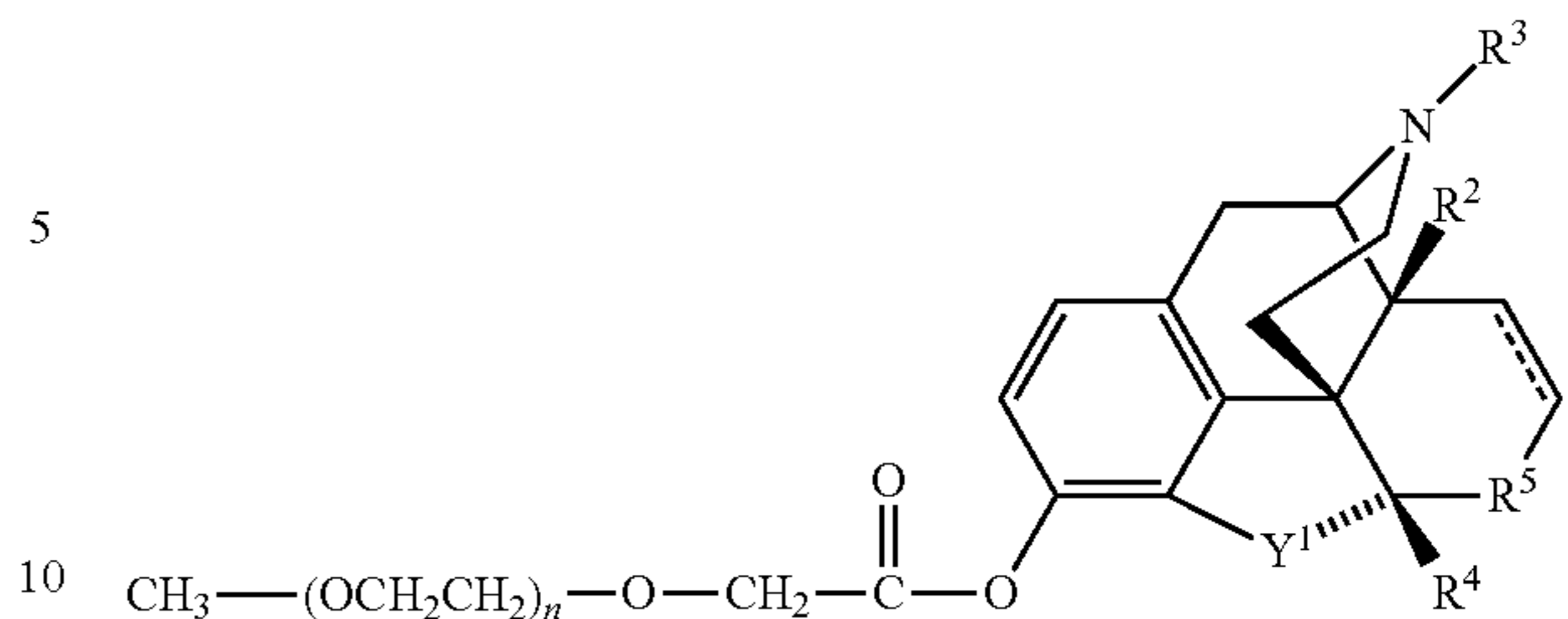
Formula I-Cc
