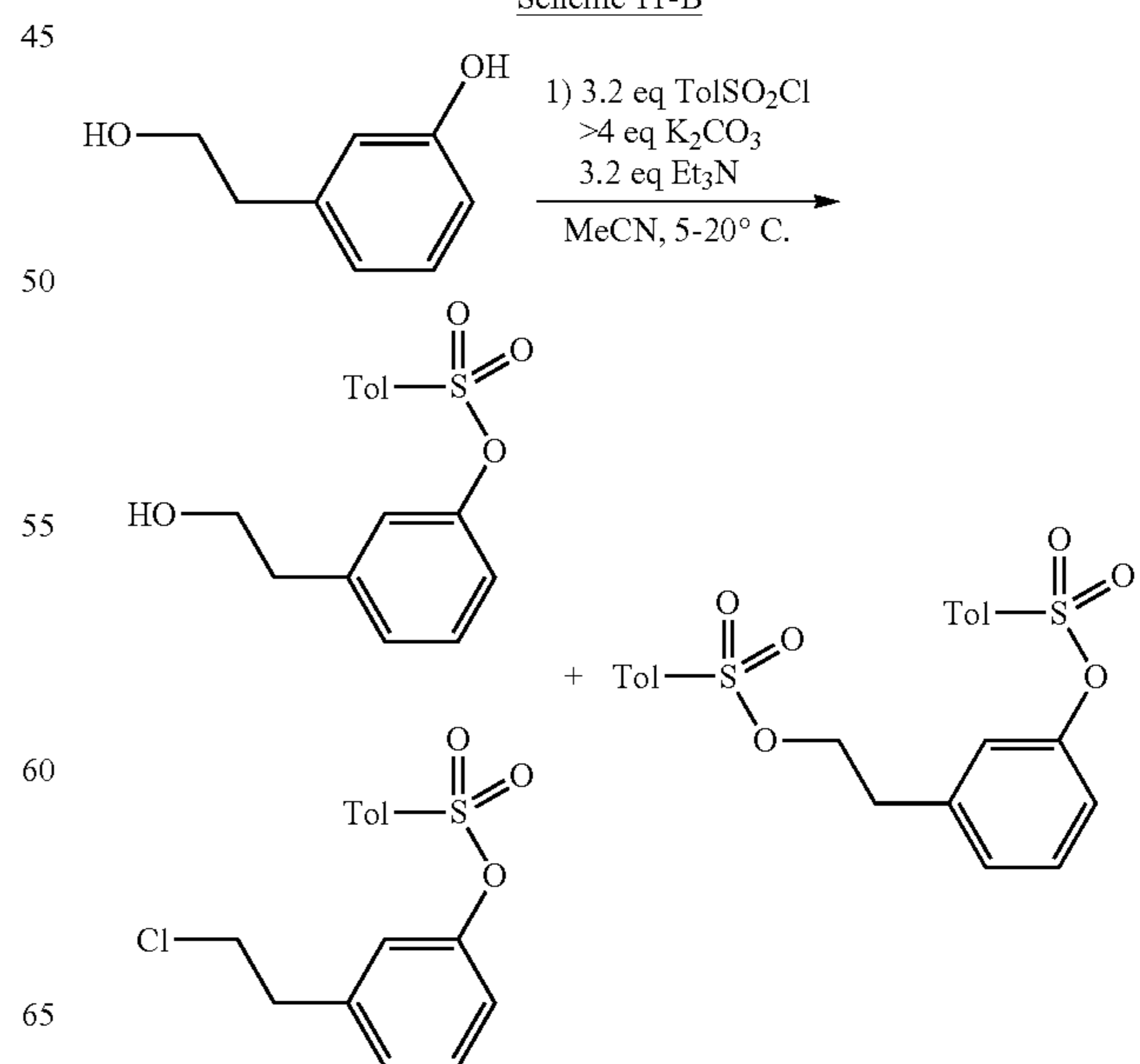
Scheme 11-B
