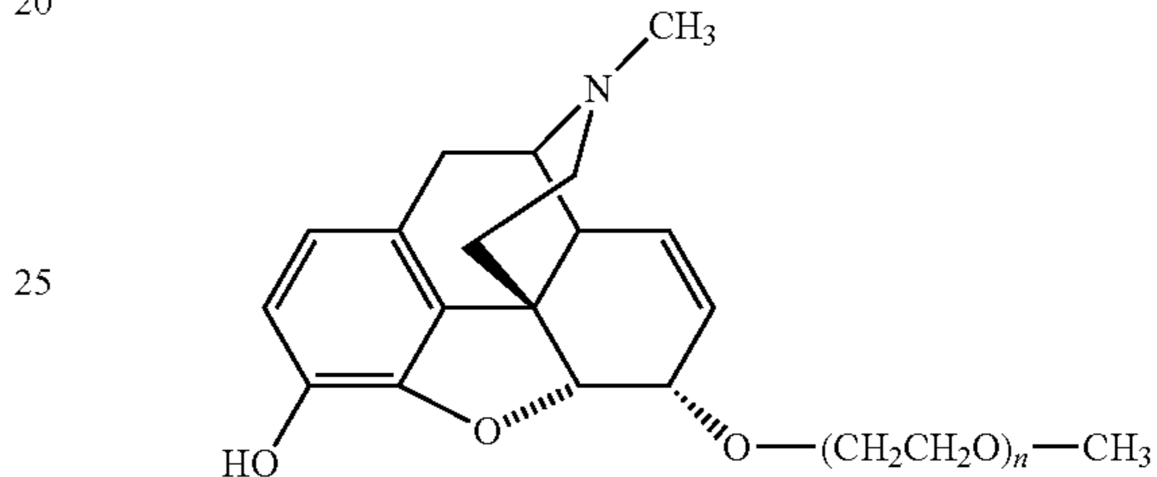
Formula I-Cd
