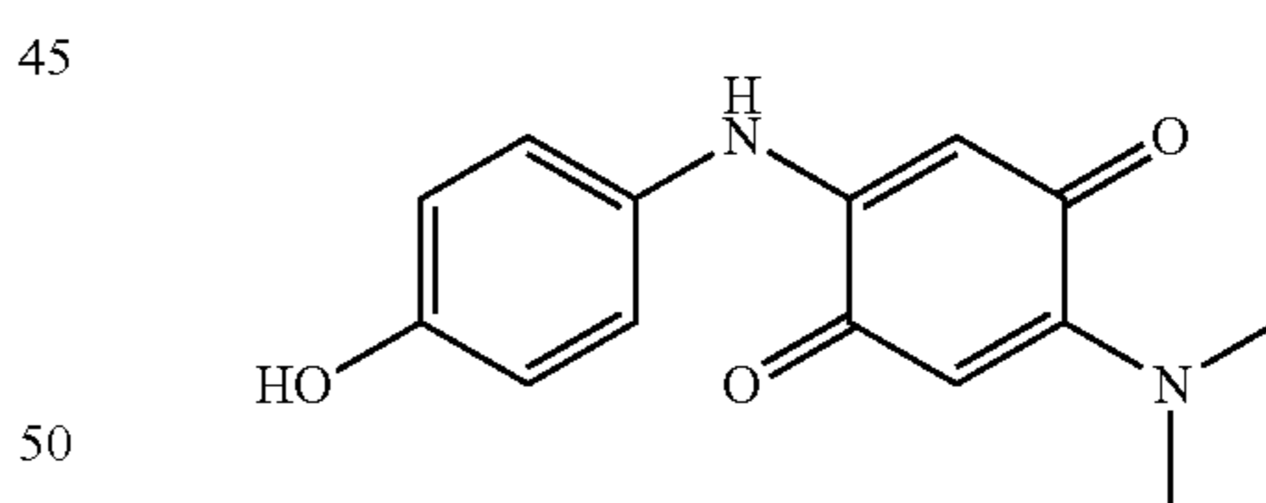
2-Dimethylamino-5-(4-hydroxyphenylamino)[1,4]benzoquinone
