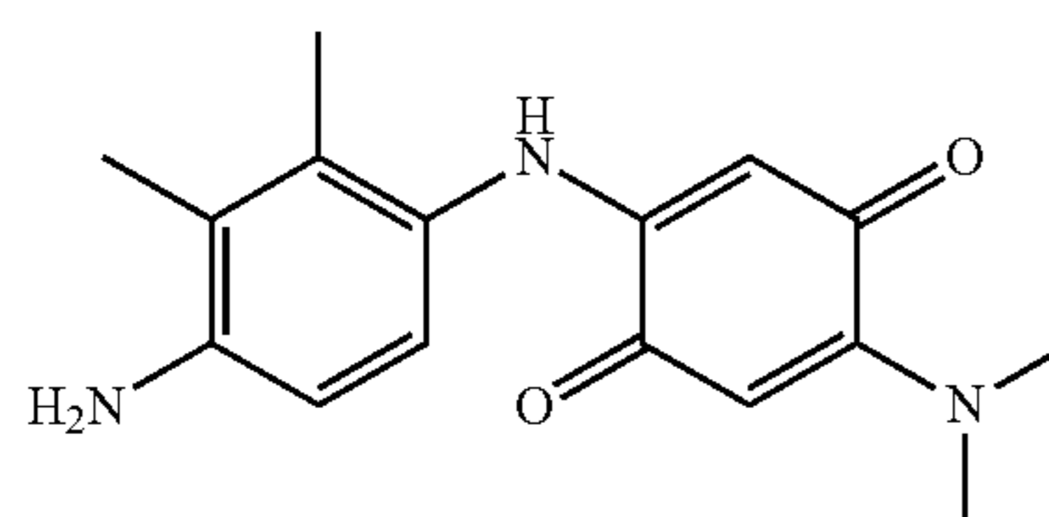
2-(4-Amino-2,3-dimethylphenylamino)-5-dimethylamino[1,4]benzoquinone
