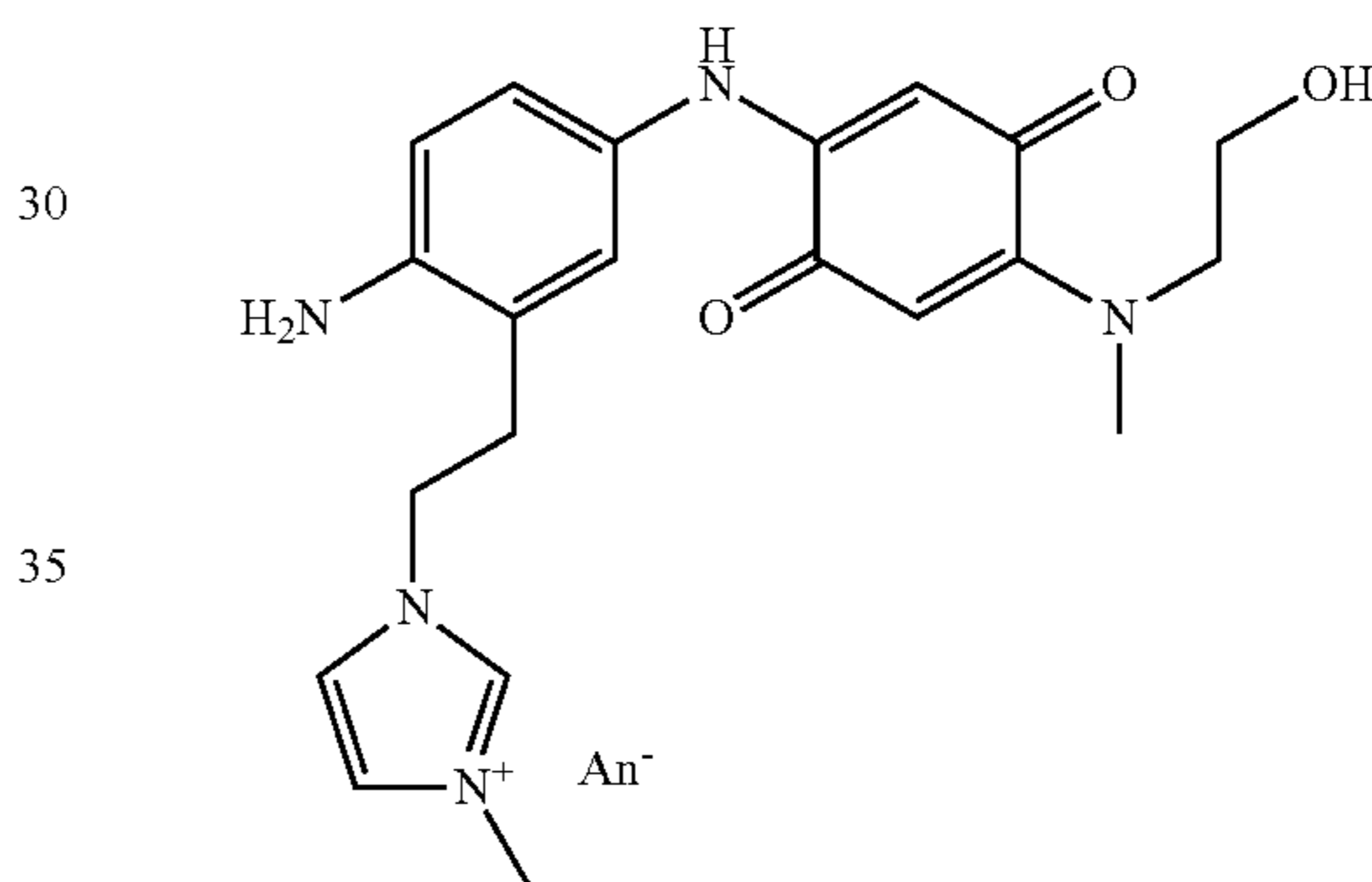
3-[2-(2-Amino-5-{4-[(2-hydroxyethyl)methylamino]-3,6-dioxocyclohexa-1,4-dienylamino}phenyl)ethyl]-1-methyl-3H-imidazol-1-ium
