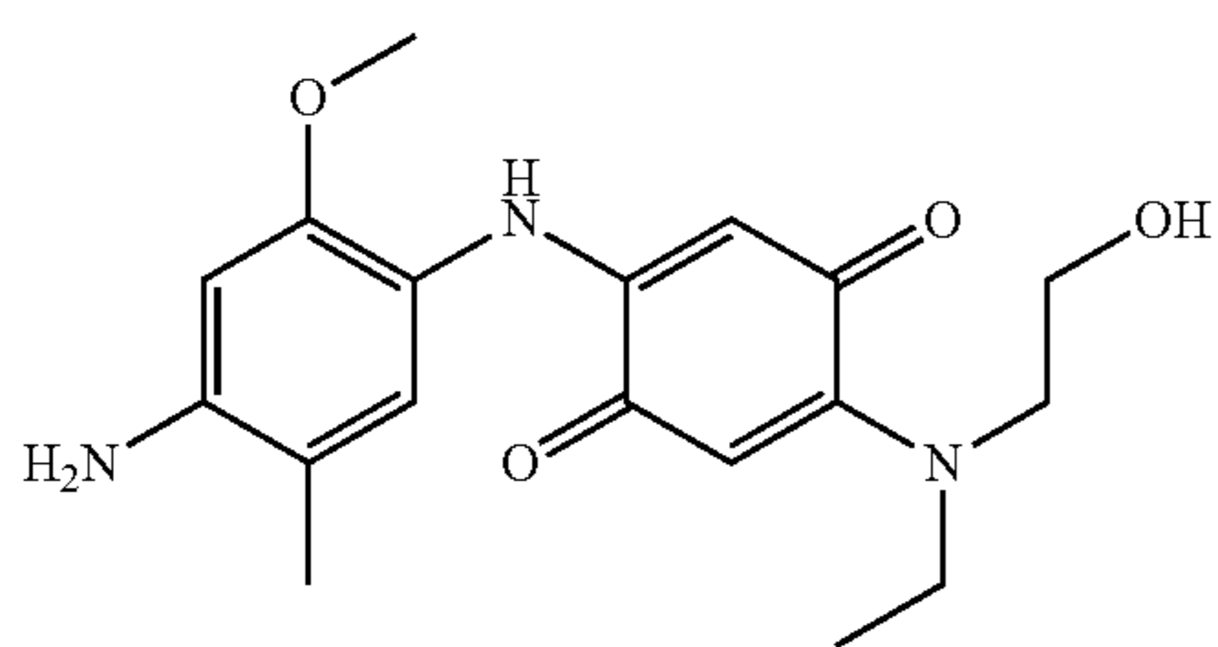
2-(4-Amino-2-methoxy-5-methylphenylamino)-5-[ethyl-(2-hydroxyethyl)amino][1,4]benzoquinone
