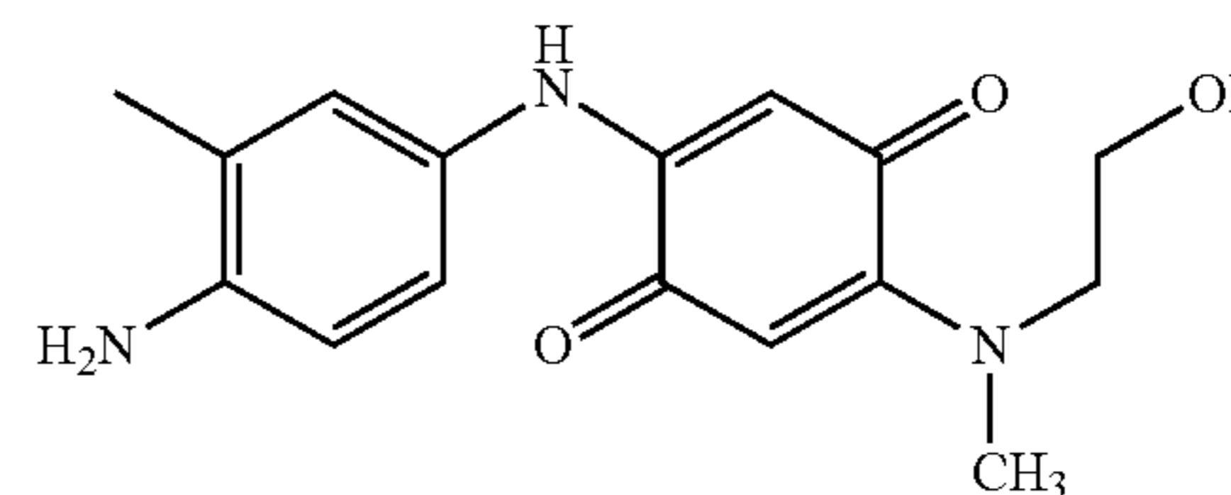
2-(4-Amino-3-methylphenylamino)-5-[(2-hydroxyethyl)methylamino][1,4]benzoquinone
