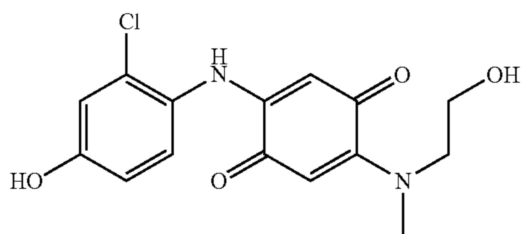
2-(2-Chloro-4-hydroxyphenylamino)-5-[(2-hydroxyethyl)methylamino][1,4]benzoquinone
