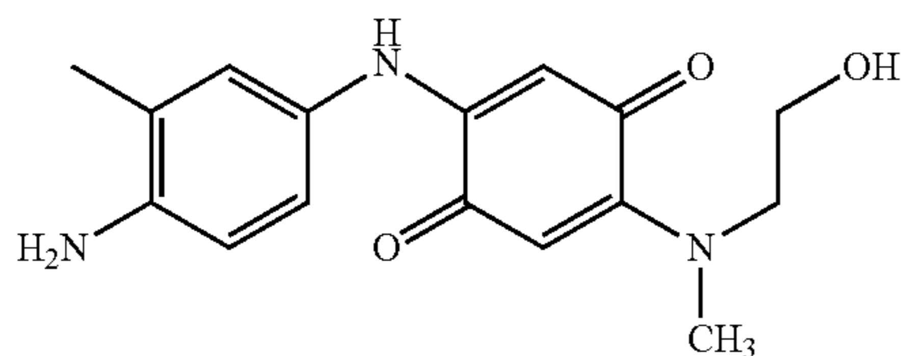
2-(4-Amino-3-methylphenylamino)-5-[(2-hydroxyethyl)methylamino][1,4]benzoquinone
