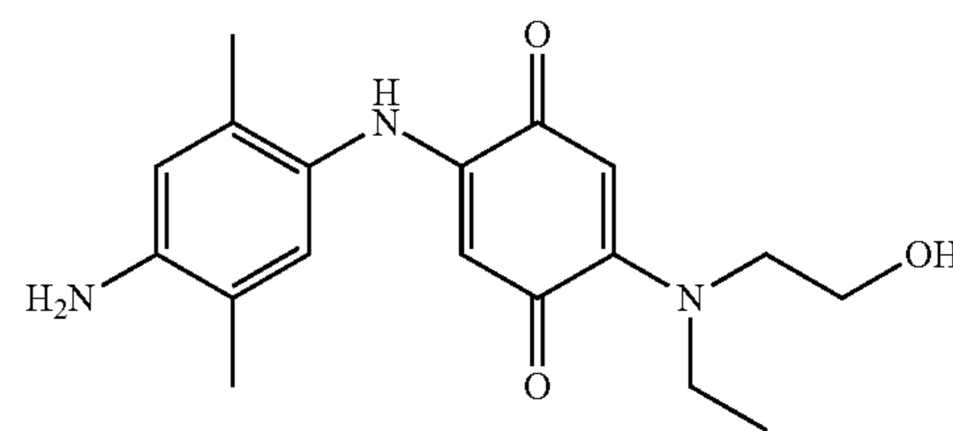
2-(4-amino-2,5-dimethylphenylamino)-5-[(2-hydroxyethyl)methylamino][1,4]benzene-1,4-diol
