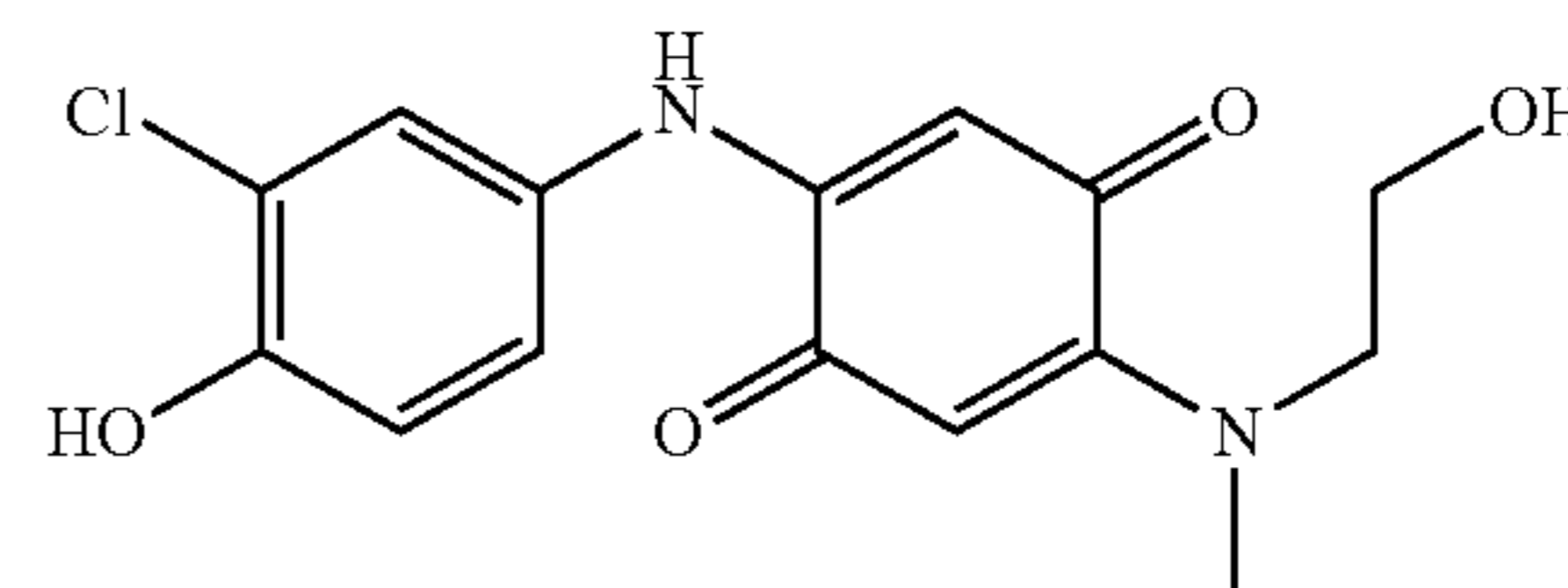
2-(3-Chloro-4-hydroxyphenylamino)-5-[(2-hydroxyethyl)methylamino][1,4]benzoquinone
