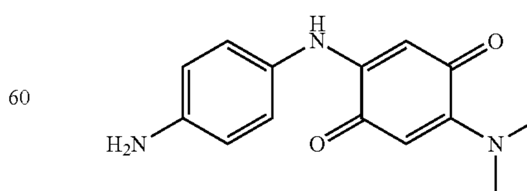
2-(4-Aminophenylamino)-5-dimethylamino[1,4]benzoquinone
