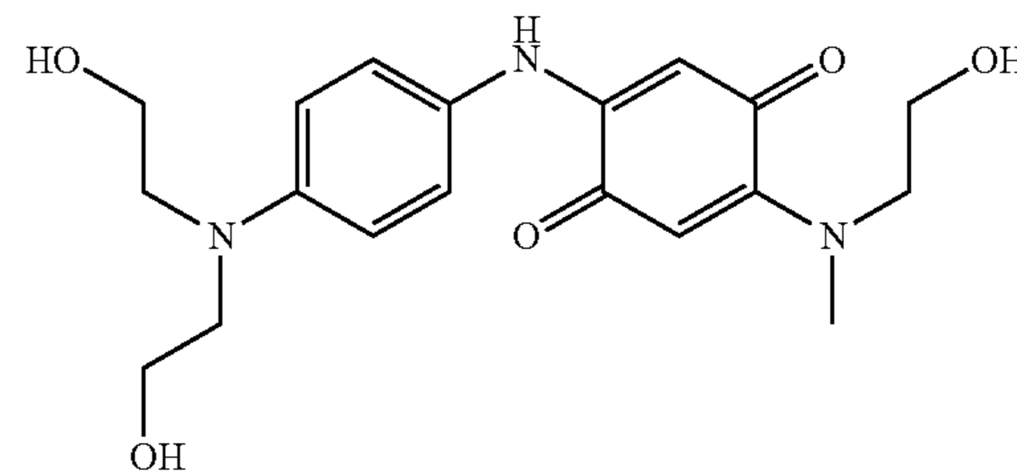
2-{4-[Bis(2-hydroxyethyl)amino]phenylamino}-5-[(2-hydroxyethyl)methylamino][1,4]benzoquinone
