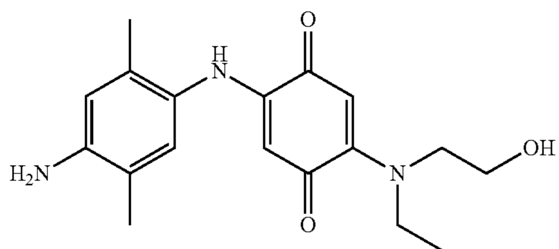
2-(4-amino-2,5-dimethylphenylamino)-5-[(2-hydroxyethyl)methylamino][1,4]benzene-1,4-diol
