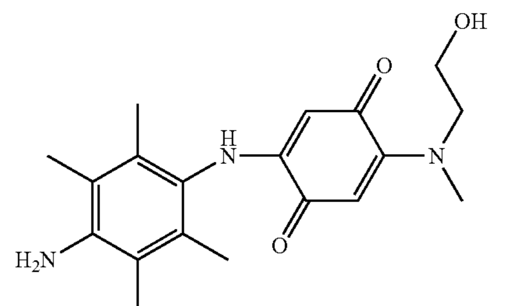
2-(4-Amino-2,3,5,6-tetramethylphenylamino)-5-[(2-hydroxyethyl)methylamino][1,4]benzoquinone
