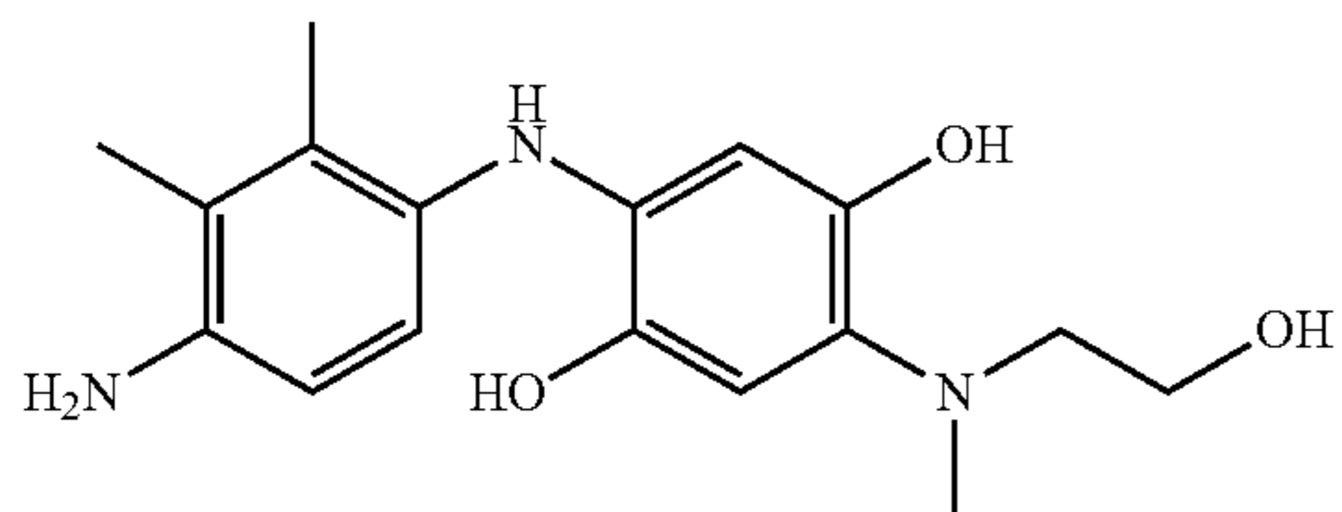
2-[(4-amino-2,3-dimethylphenyl)amino]-5-[(2-hydroxyethyl)(methyl)amino]benzene-1,4-diol
