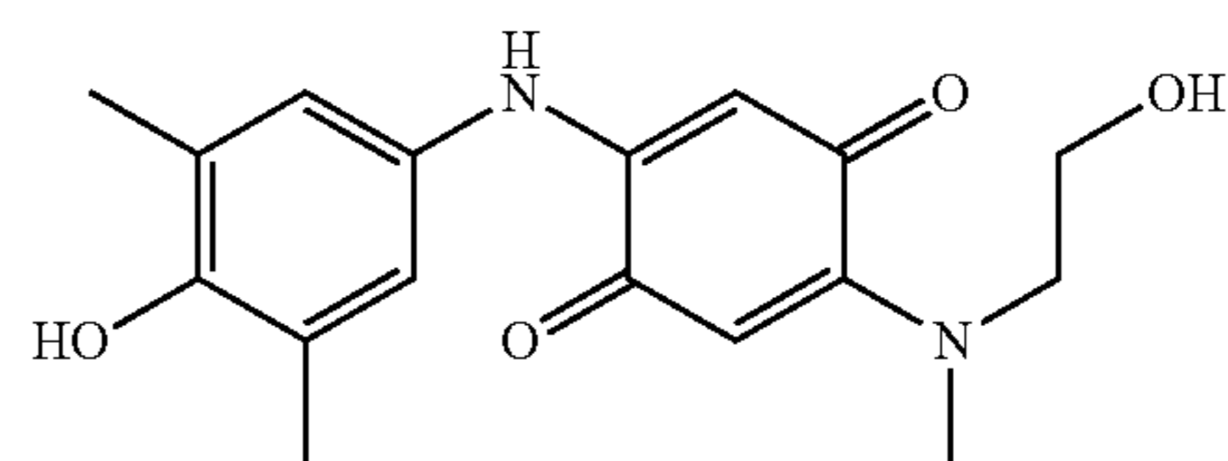
2-(4-Hydroxy-3,5-dimethylphenylamino)-5-[(2-hydroxyethyl)methylamino][1,4]benzoquinone
