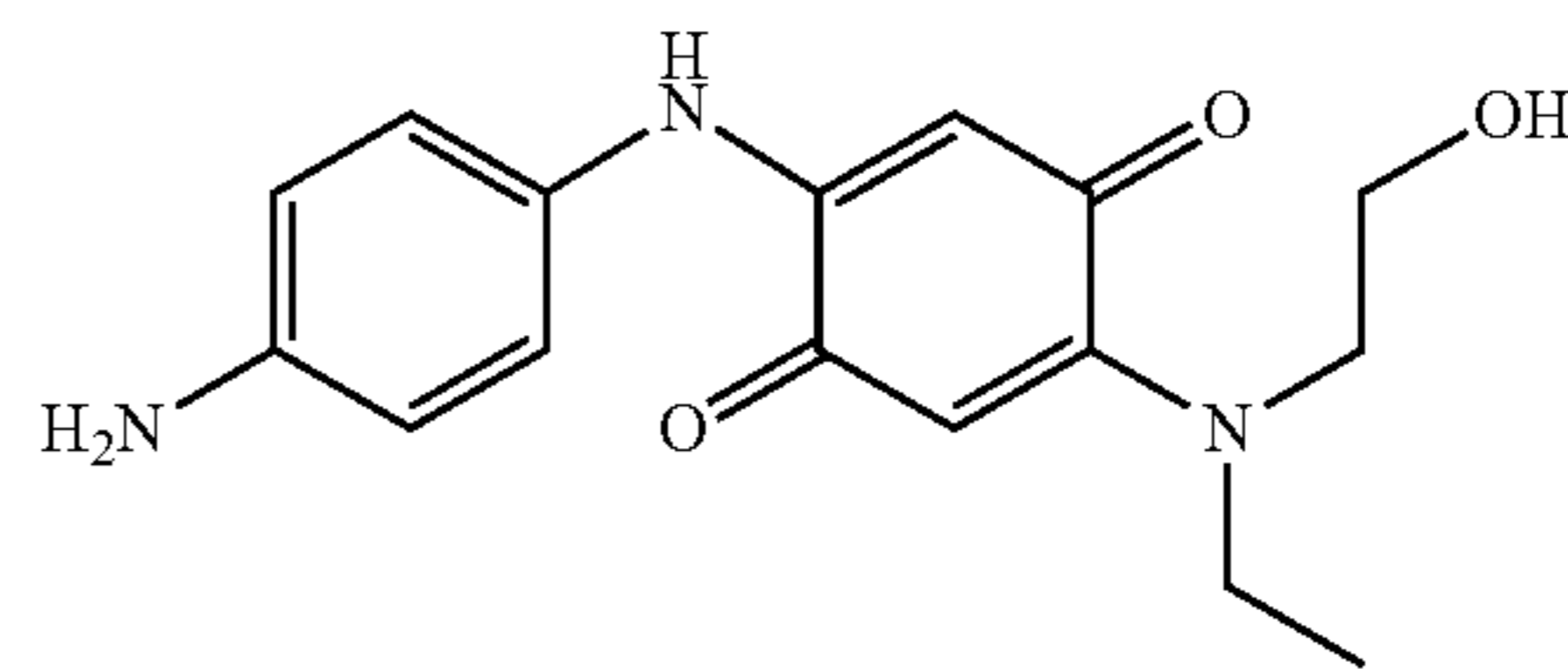
2-(4-(Aminophenylamino)-5-[(2-hydroxyethyl)ethylamino][1,4]benzoquinone
