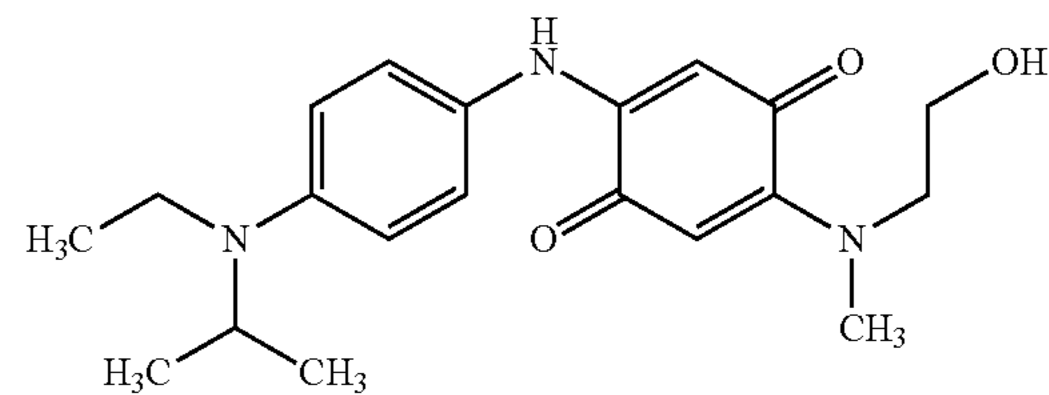
2-[4-(Ethylisopropylamino)phenylamino]-5-[(2-hydroxyethyl)methylamino][1,4]benzoquinone
