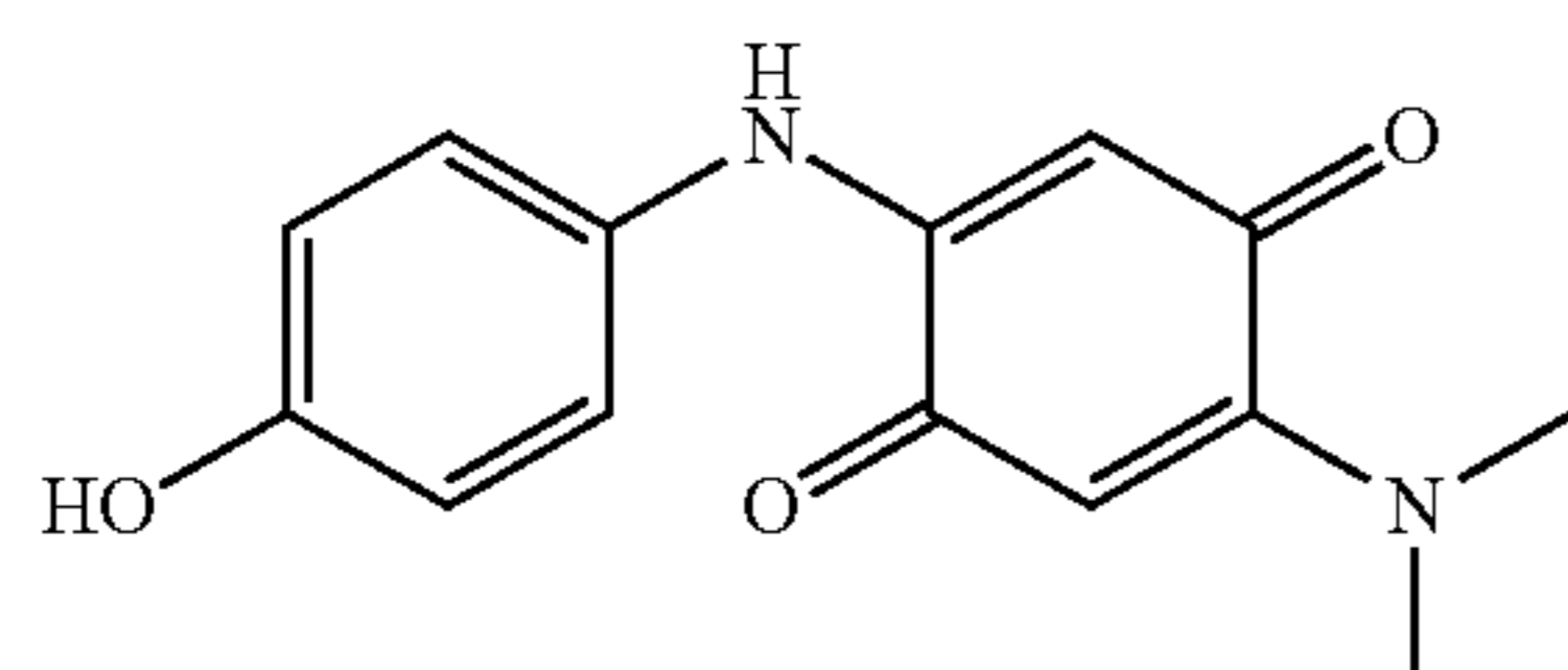
2-Dimethylamino-5-(4-hydroxyphenylamino)[1,4]benzoquinone
