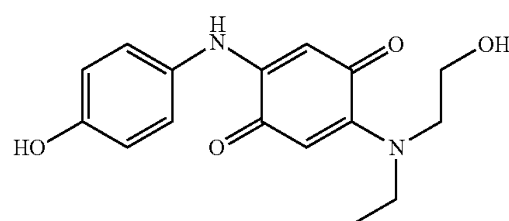
2-[(2-Hydroxyethyl)ethylamino]-5-(4-hydroxyphenylamino)[1,4]benzoquinone
