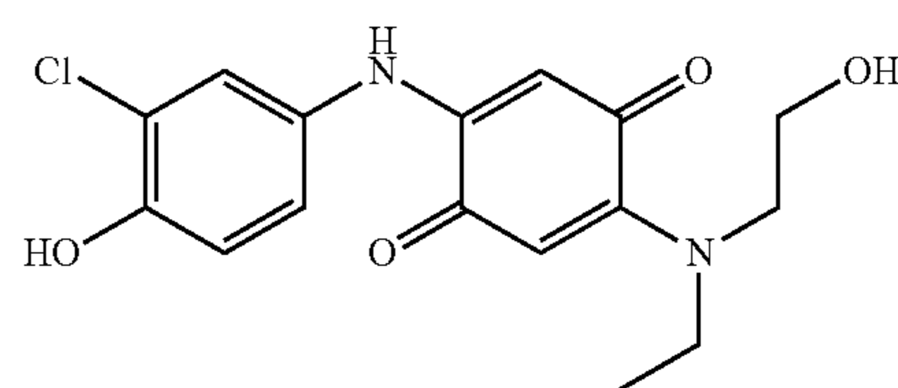
2-(3-Chloro-4-hydroxyphenylamino)-5-[(2-hydroxyethyl)ethylamino][1,4]benzoquinone
