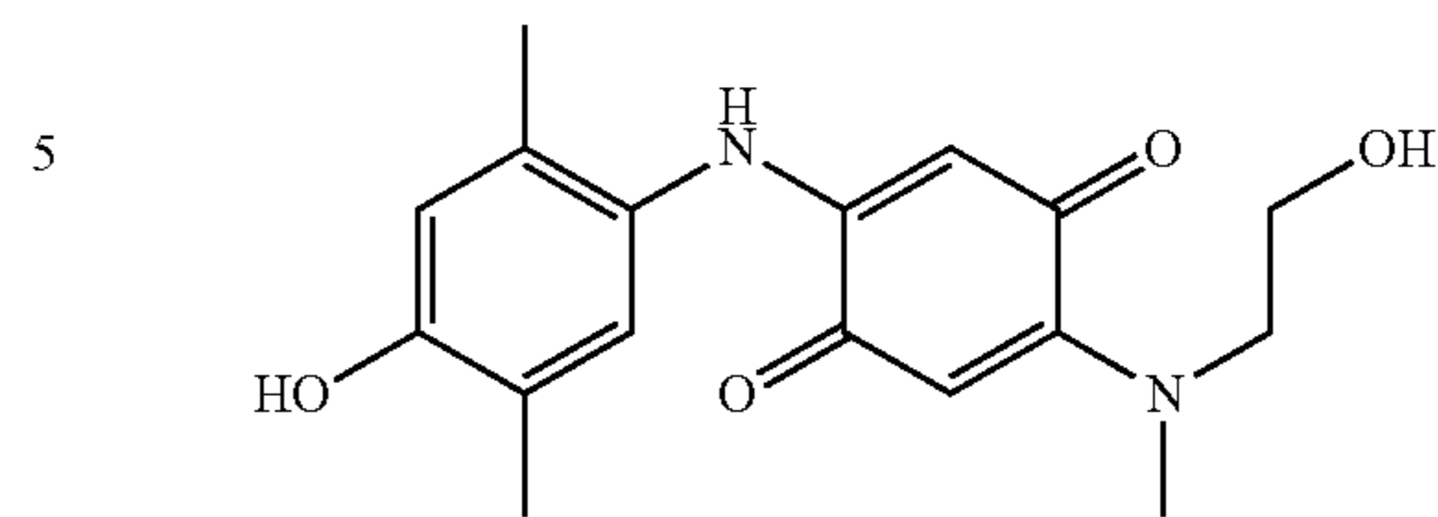
2-(4-Hydroxy-2,5-dimethylphenylamino)-5-[(2-hydroxyethyl)methylamino][1,4]benzoquinone
