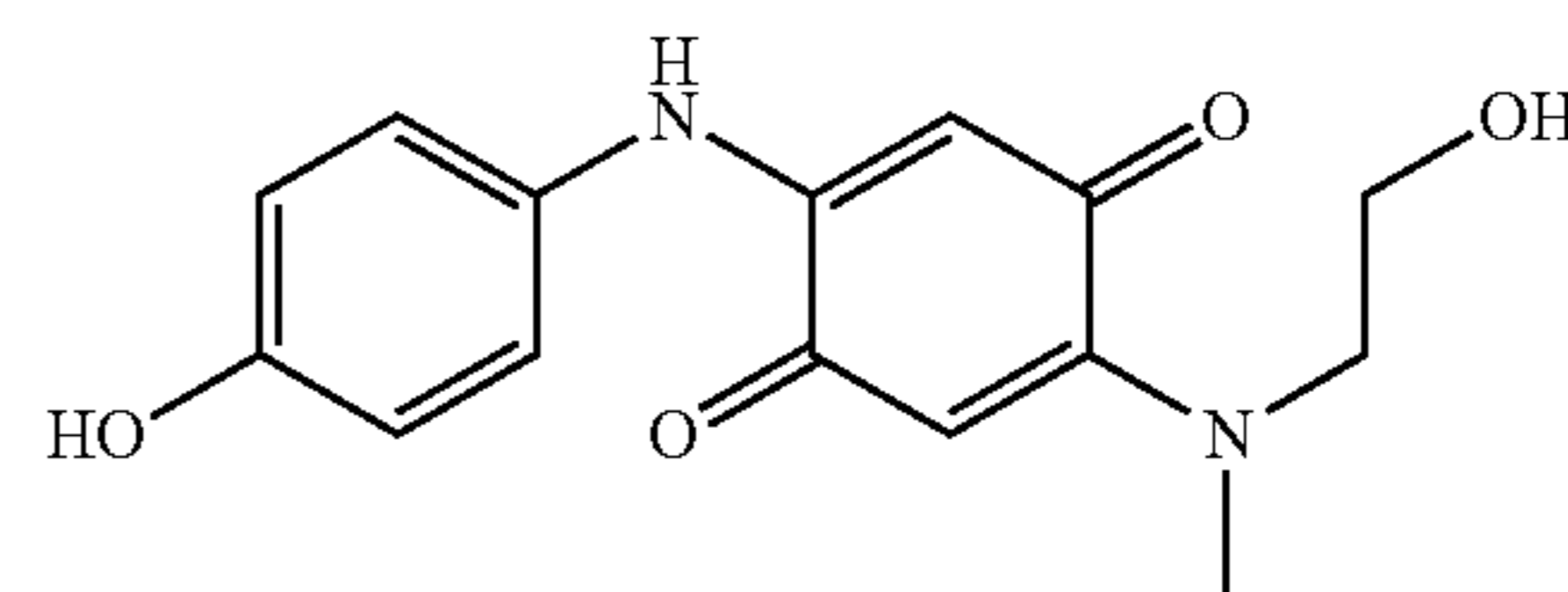
2-[(2-Hydroxyethyl)methylamino]-5-(4-hydroxyphenylamino)[1,4]benzoquinone
