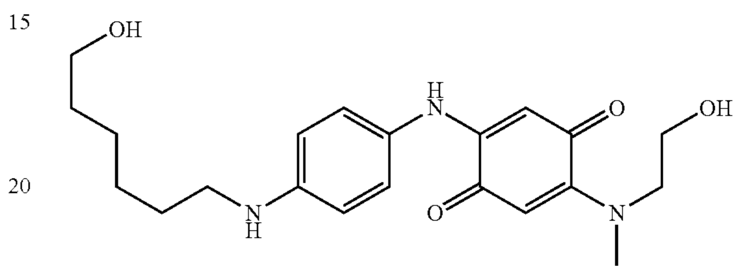
2-[(2-Hydroxyethyl)methylamino]-5-[4-(6-hydroxy-hexylamino)phenylamino][1,4]benzoquinone
