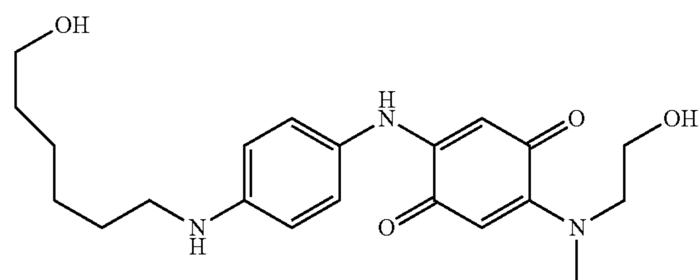
2-[(2-Hydroxyethyl)methylamino]-5-[4-(6-hydroxyhexylamino)phenylamino][1,4]benzoquinone
