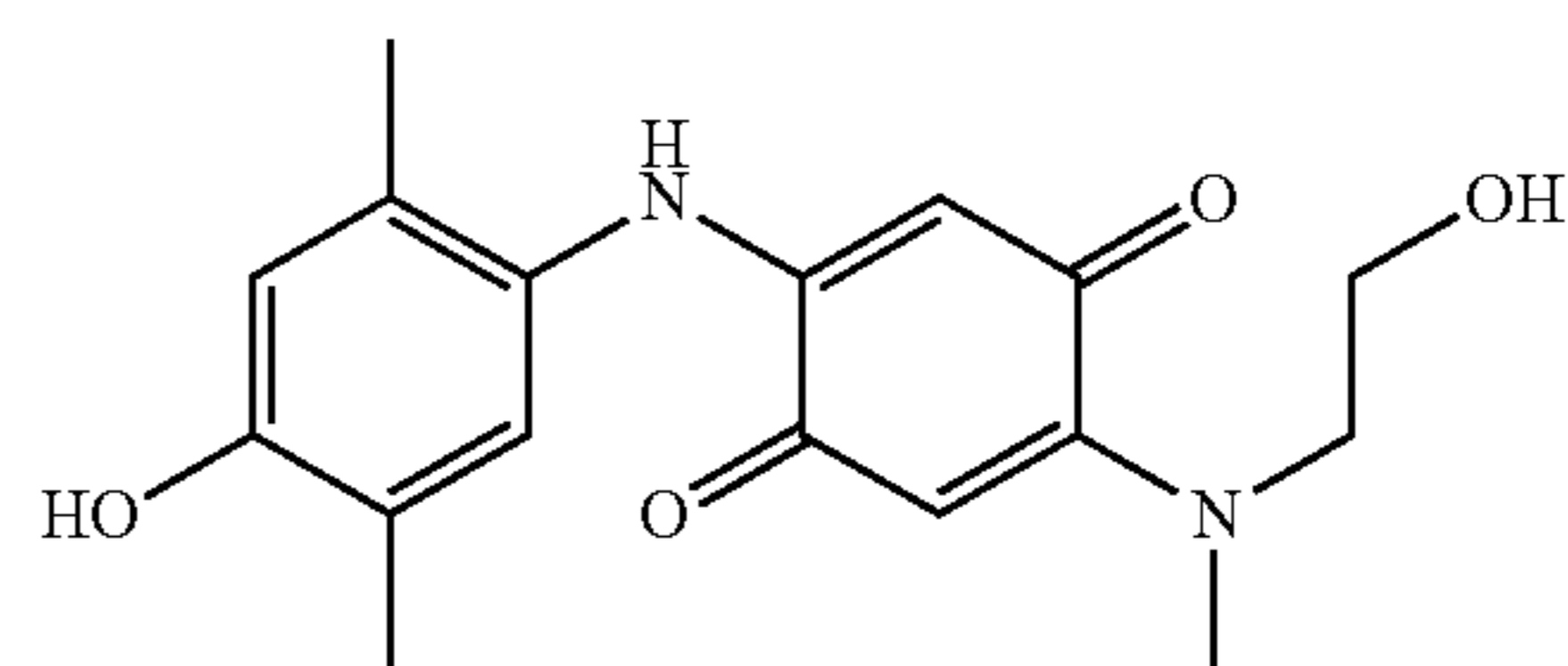
2-(4-Hydroxy-2,5-dimethylphenylamino)-5-[(2-hydroxyethyl)methylamino][1,4]benzoquinone
