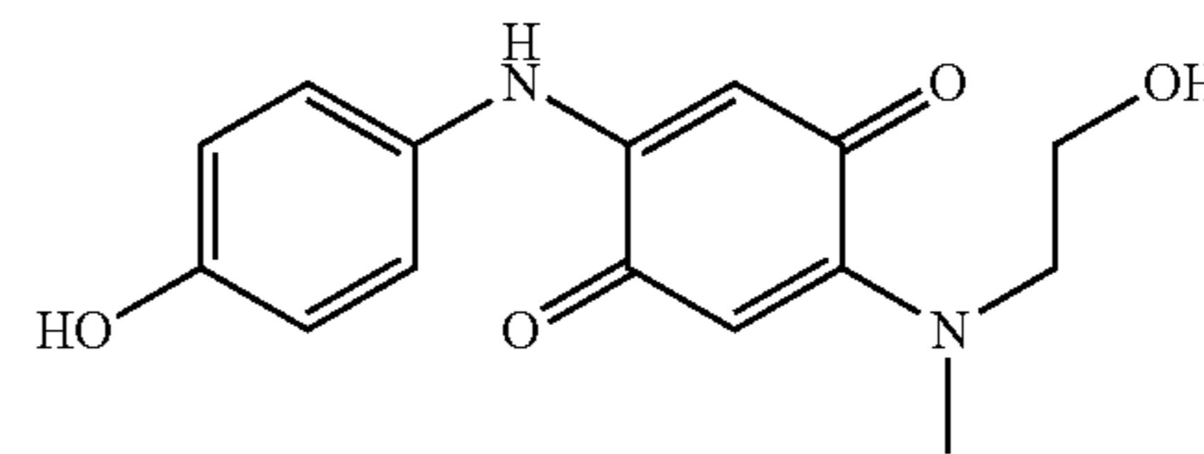
2-[(2-Hydroxyethyl)methylamino]-5-(4-hydroxyphenylamino)[1,4]benzoquinone
