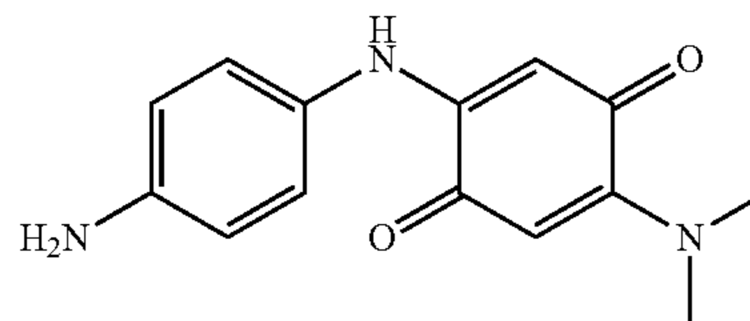
2-(4-Aminophenylamino)-5-dimethylamino[1,4]benzoquinone
