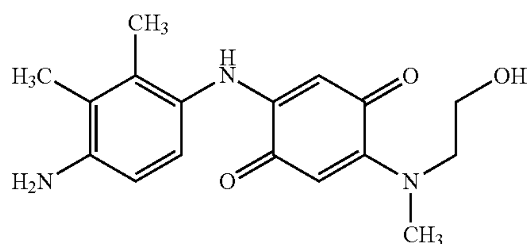
2-(4-Amino-2,3-dimethylphenylamino)-5-[2-(2-hydroxyethyl)methylamino][1,4]benzoquinone
