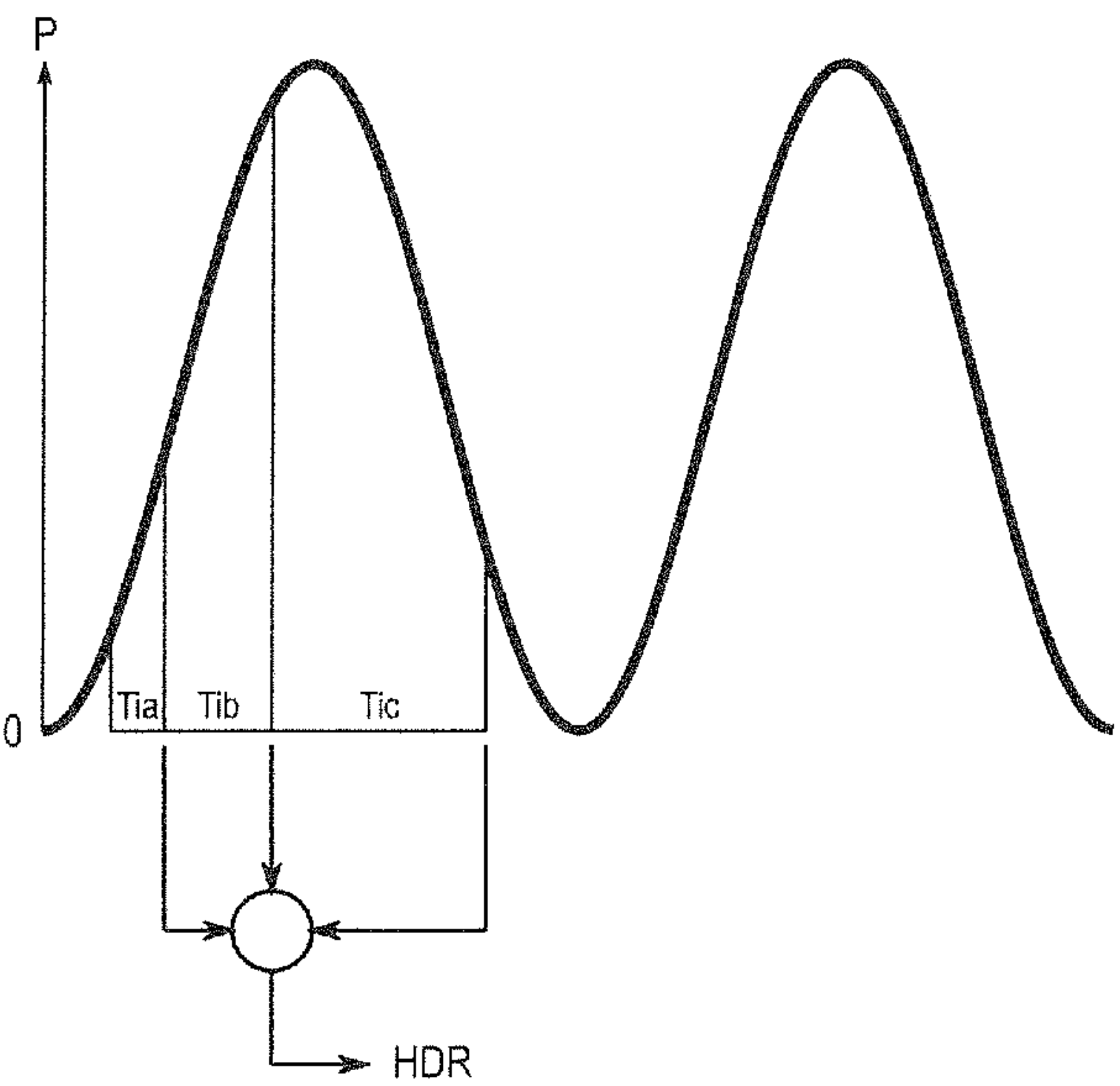
Fig 2 (Prior Art)
