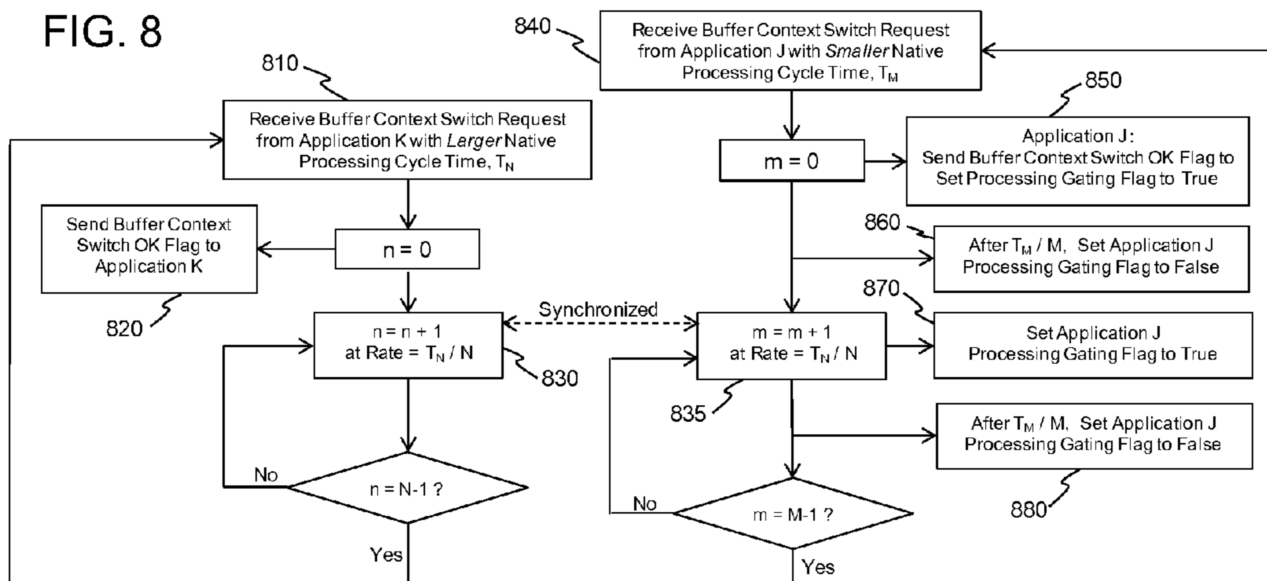
665 Shared Buffer Memory Manager for Application K and J with Native Processing Cycle Times T_N and T_M where T_N > T_M
