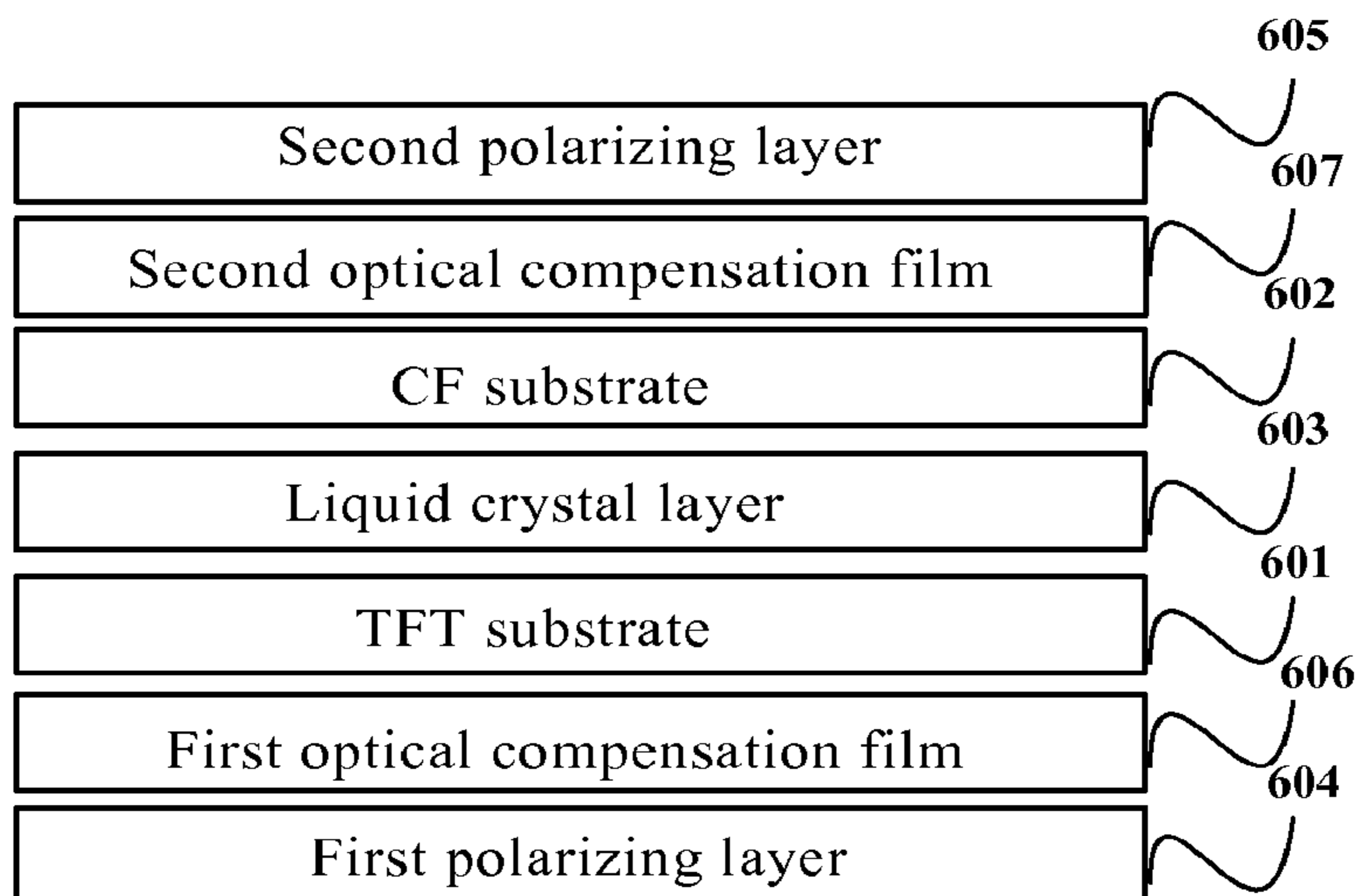
FIG.5 Prior Art
