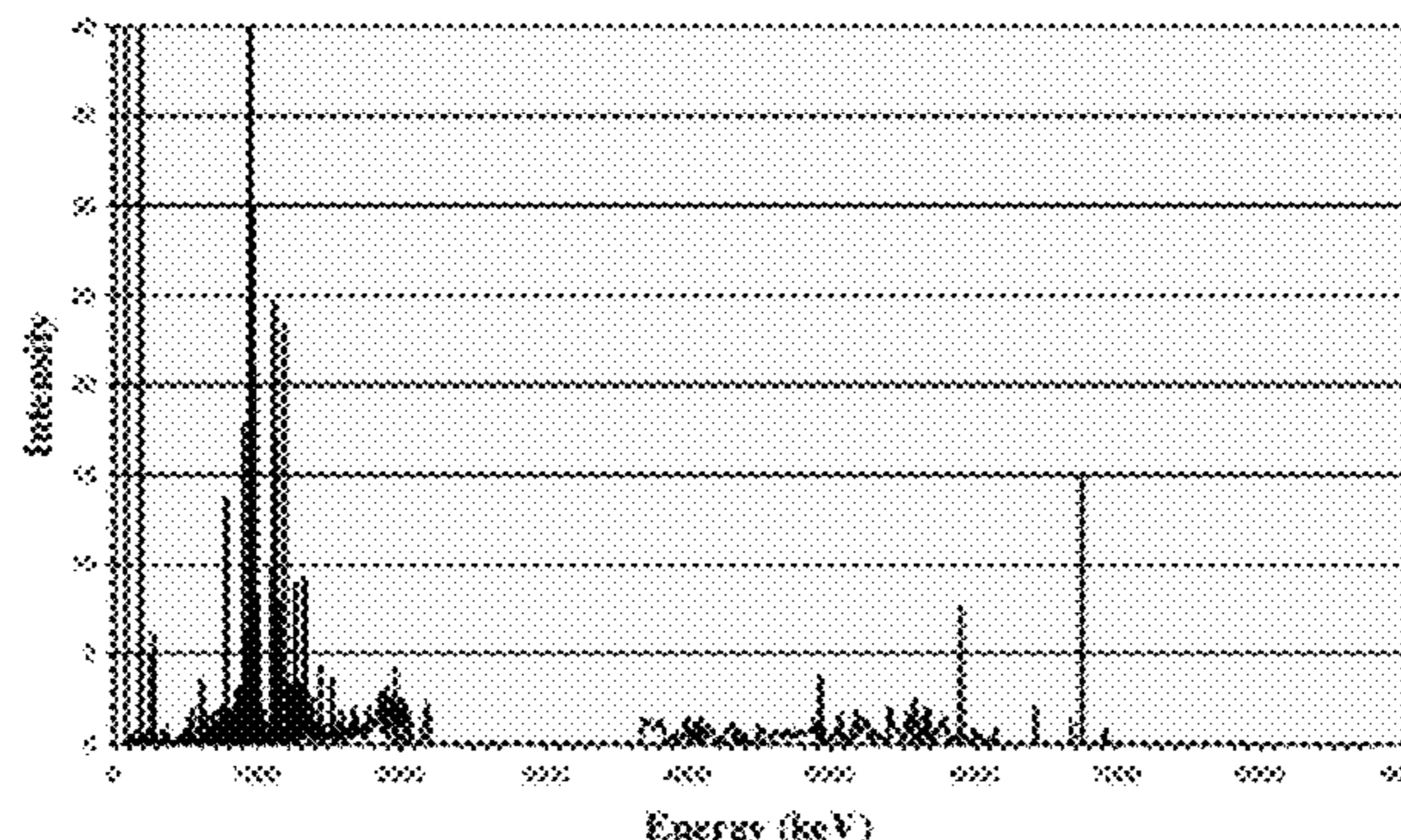
Gd-158 Gamma-Rays
