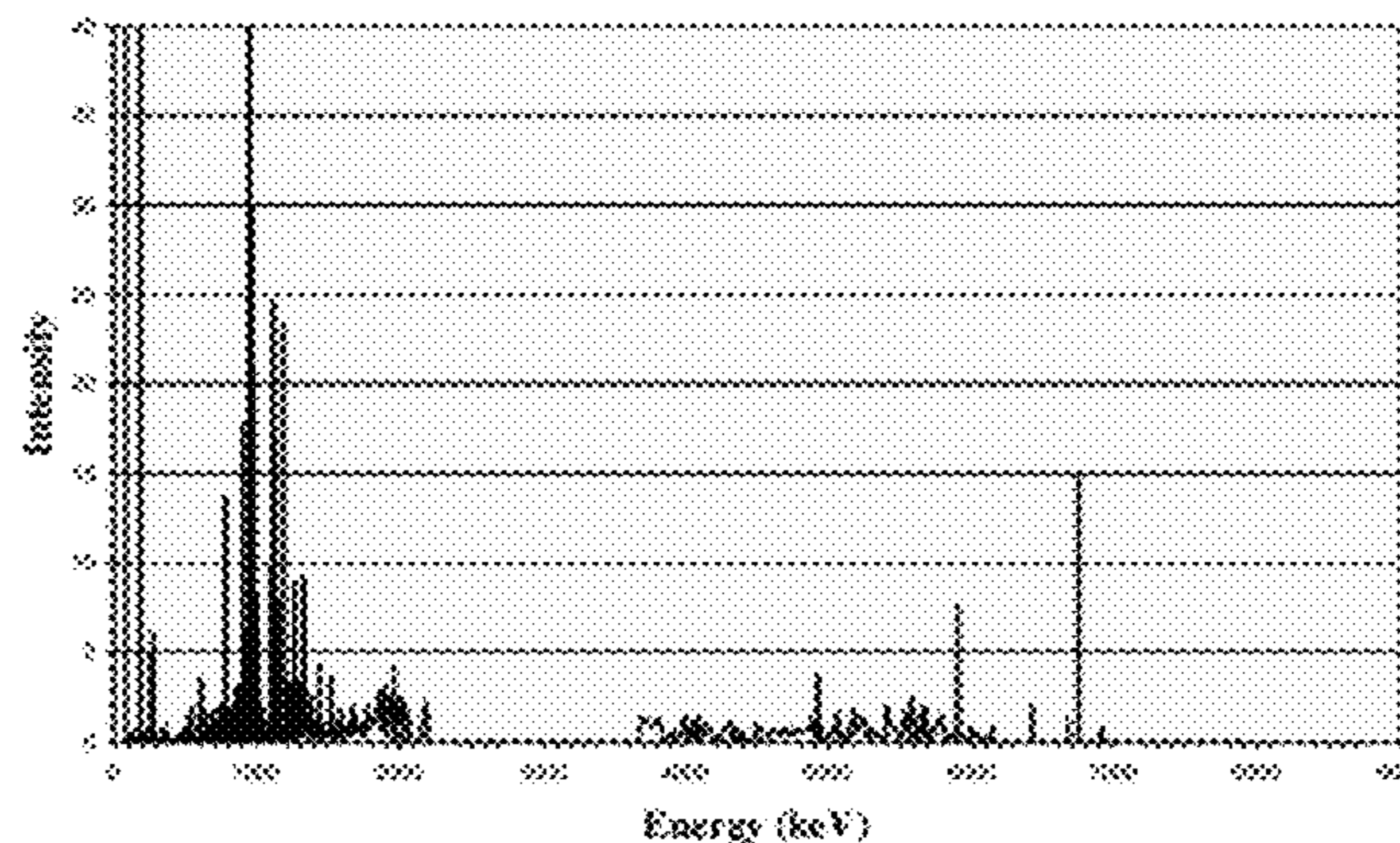
Gd-158 Gamma-Rays
