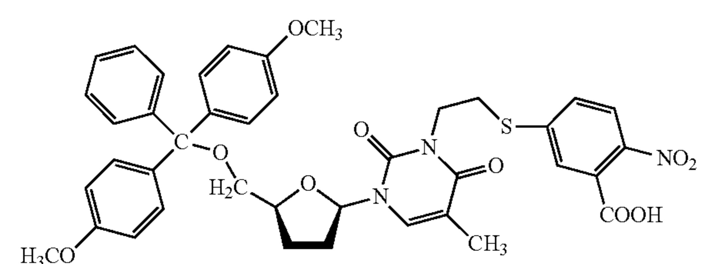
Reaction Scheme N
