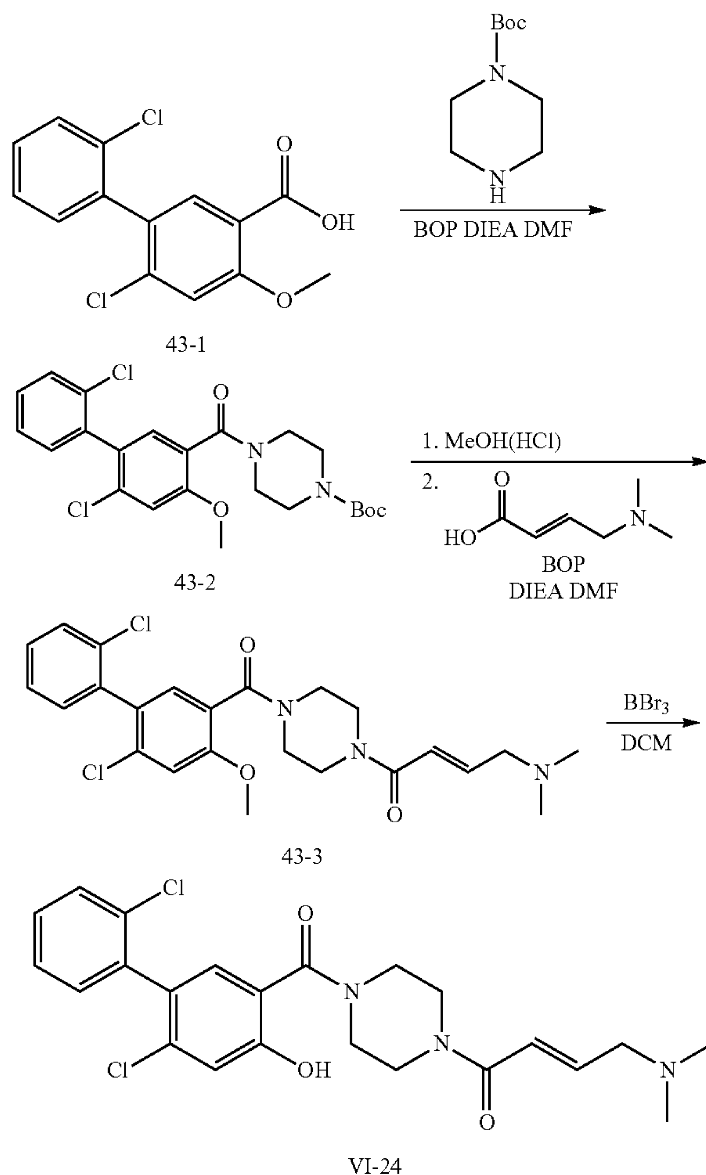
tert-Butyl 4-(2',6-dichloro-4-methoxy-[1,1'-biphenyl]-3-carbonyl)piperazine-1-carboxylate
