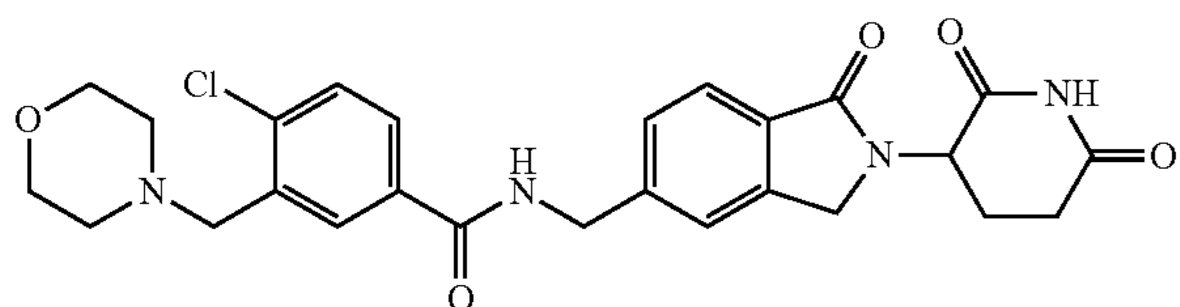
4-chloro-N-((2-(2,6-dioxopiperidin-3-yl)-1-oxoisindolin-5-yl)methyl)-3-(morpholinomethyl)benzamide;
