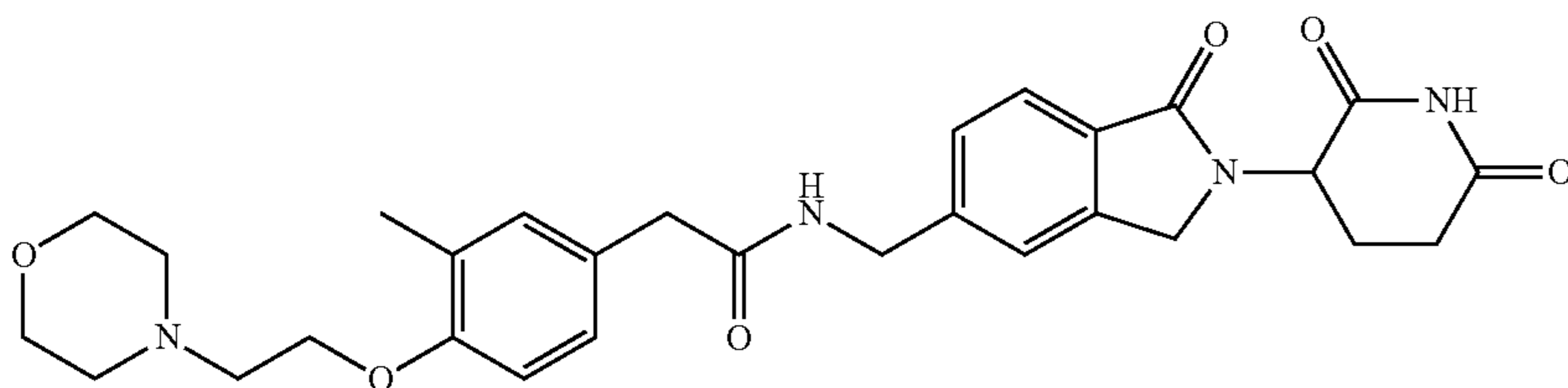
N-((2-(2,6-dioxopiperidin-3-yl)-1-oxoisindolin-5-yl)methyl)-2-(3-methyl-4-(2-morpholinoethoxy)phenyl)acetamide;
