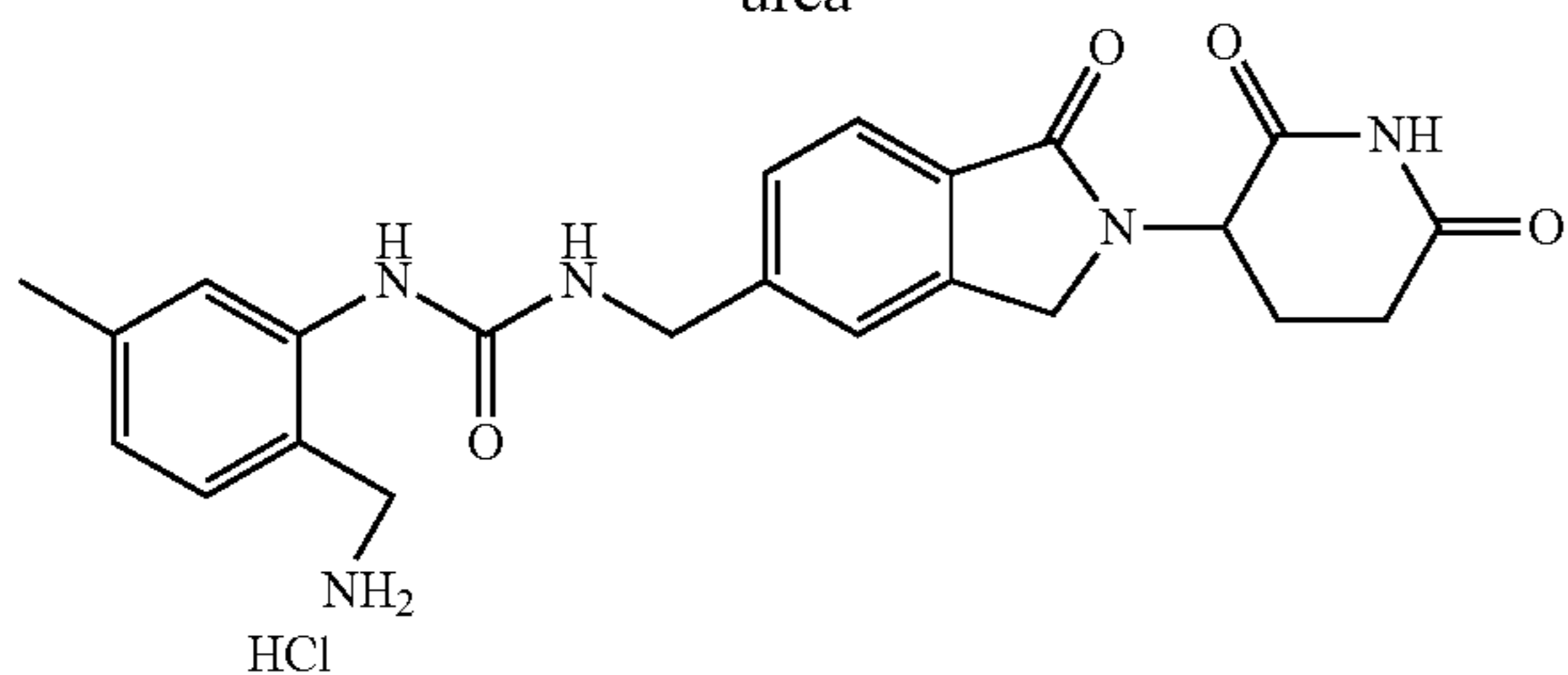
5.24 1-(2-(Aminomethyl)-5-methylphenyl)-3-((2-(2,6-dioxopiperidin-3-yl)-1-oxoisindolin-5-yl)methyl)urea
