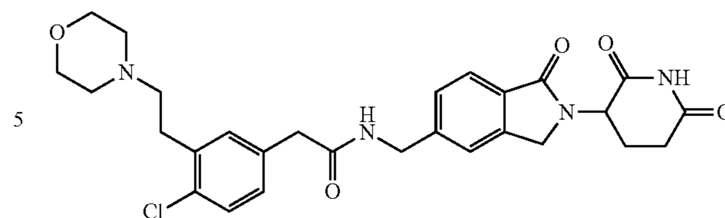
2-(4-chloro-3-(2-morpholinoethyl)phenyl)-N-((2-(2,6-dioxopiperidin-3-yl)-1-oxoindolin-5-yl)methyl)acetamide;
