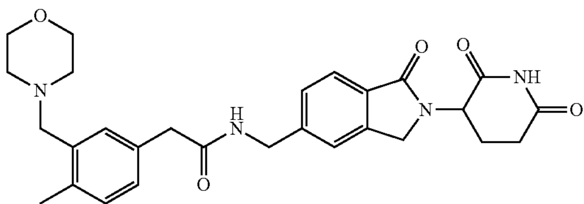
N-((2-(2,6-dioxopiperidin-3-yl)-1-oxoindolin-5-yl)methyl)-2-(4-methyl-3-(morpholinomethyl)phenyl)acetamide;
