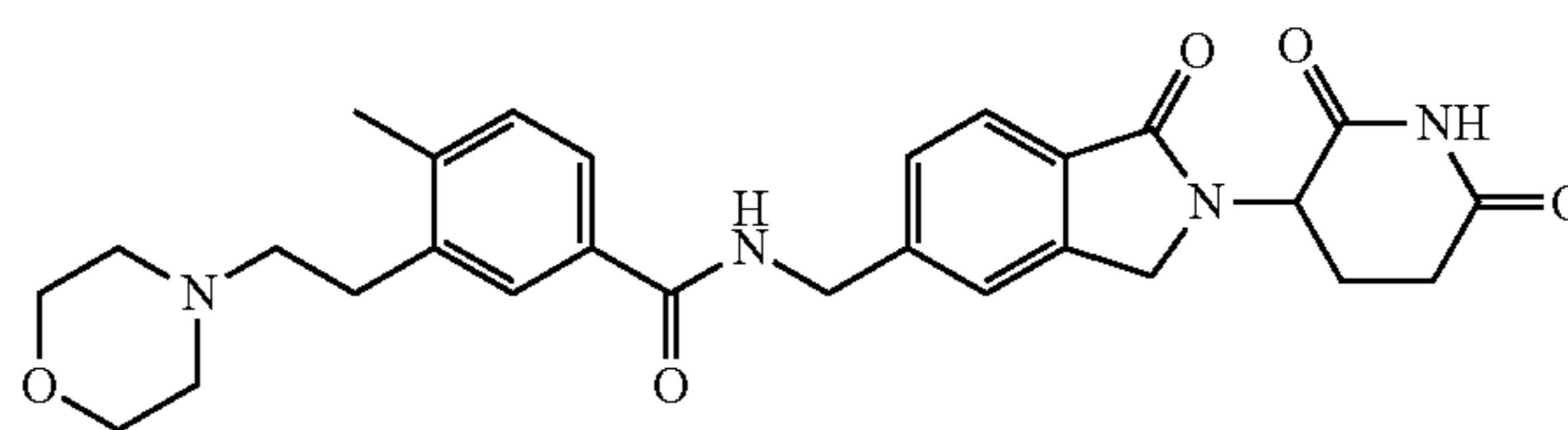
N-((2-(2,6-dioxopiperidin-3-yl)-1-oxoisindolin-5-yl)methyl)-4-methyl-3-(2-morpholinoethyl)benzamide;
