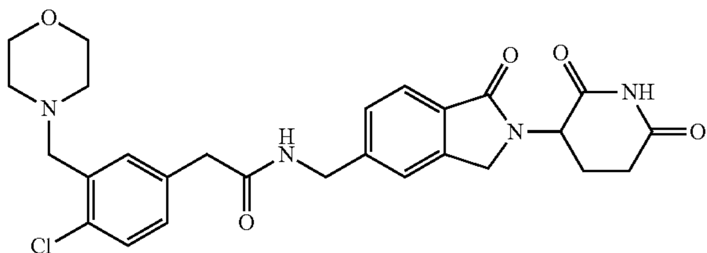
N-((2-(2,6-dioxopiperidin-3-yl)-1-oxoindolin-5-yl)methyl)-2-(4-(morpholinomethyl)phenyl)acetamide;
