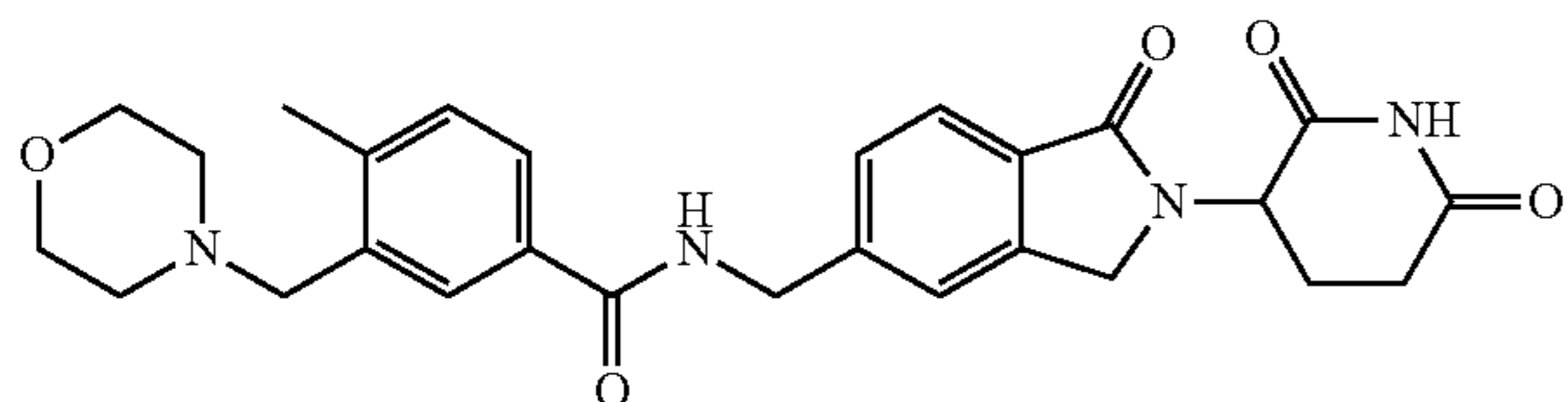
N-((2-(2,6-dioxopiperidin-3-yl)-1-oxoisindolin-5-yl)methyl)-4-methyl-3-(morpholinomethyl)benzamide;
