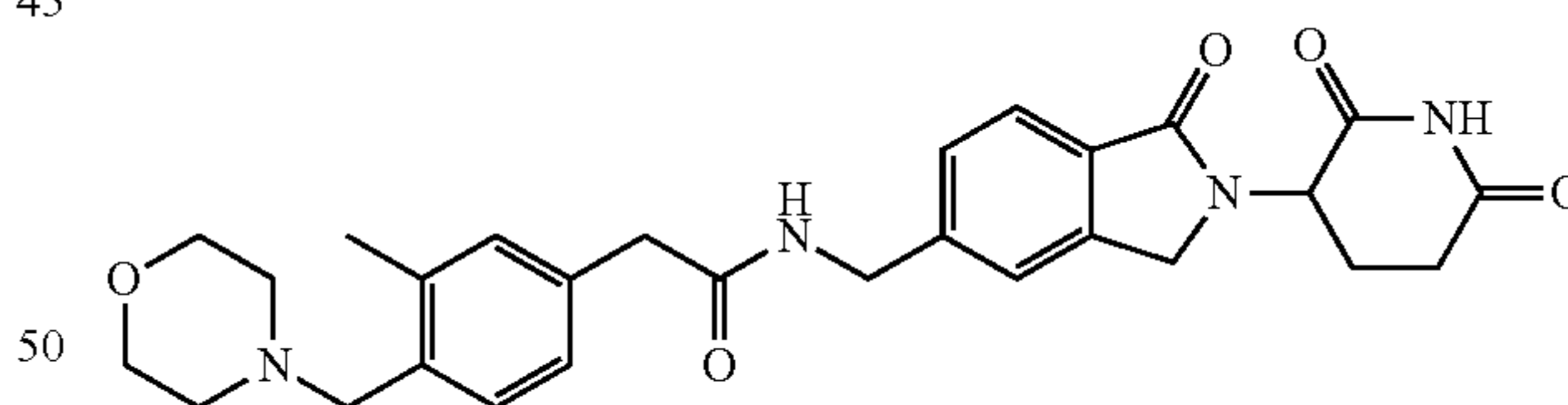
N-((2-(2,6-dioxopiperidin-3-yl)-1-oxoindolin-5-yl)methyl)-2-(3-methyl-4-(morpholinomethyl)phenyl)acetamide;
