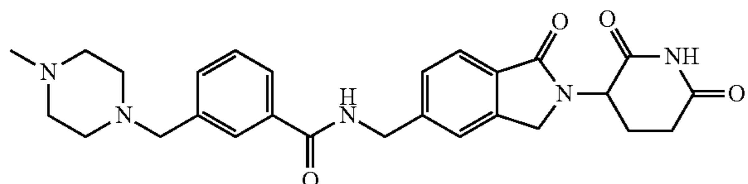
N-((2-(2,6-dioxopiperidin-3-yl)-1-oxoisindolin-5-yl)methyl)-3-((4-methylpiperazin-1-yl)methyl)benzamide;
