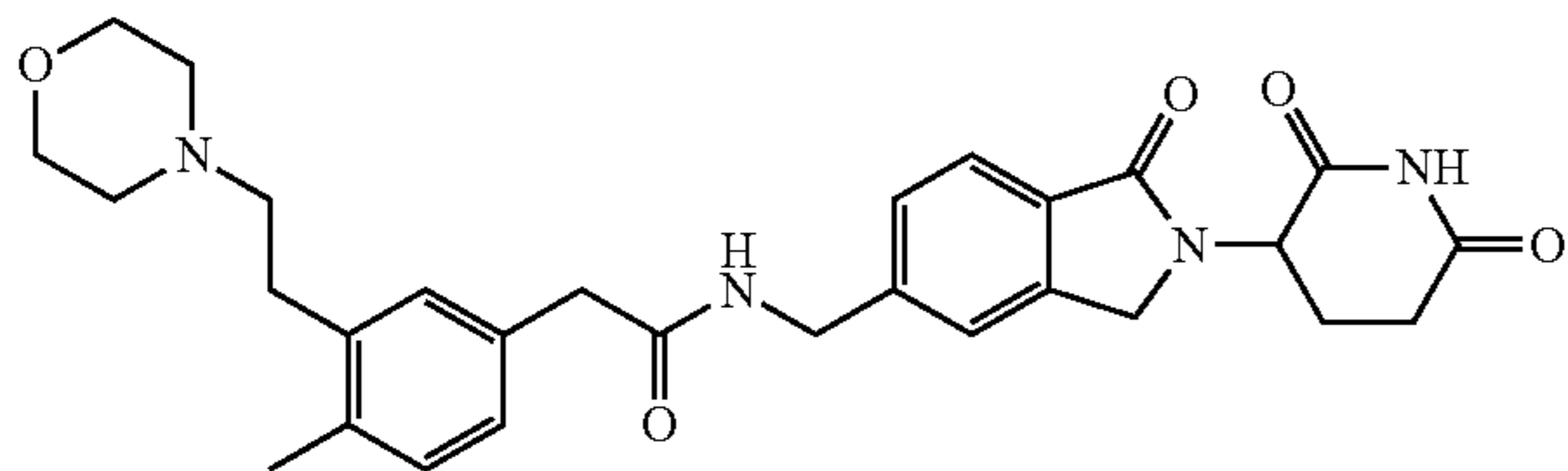
N-((2-(2,6-dioxopiperidin-3-yl)-1-oxoindolin-5-yl)methyl)-2-(4-methyl-3-(2-morpholinoethyl)phenyl)acetamide;
