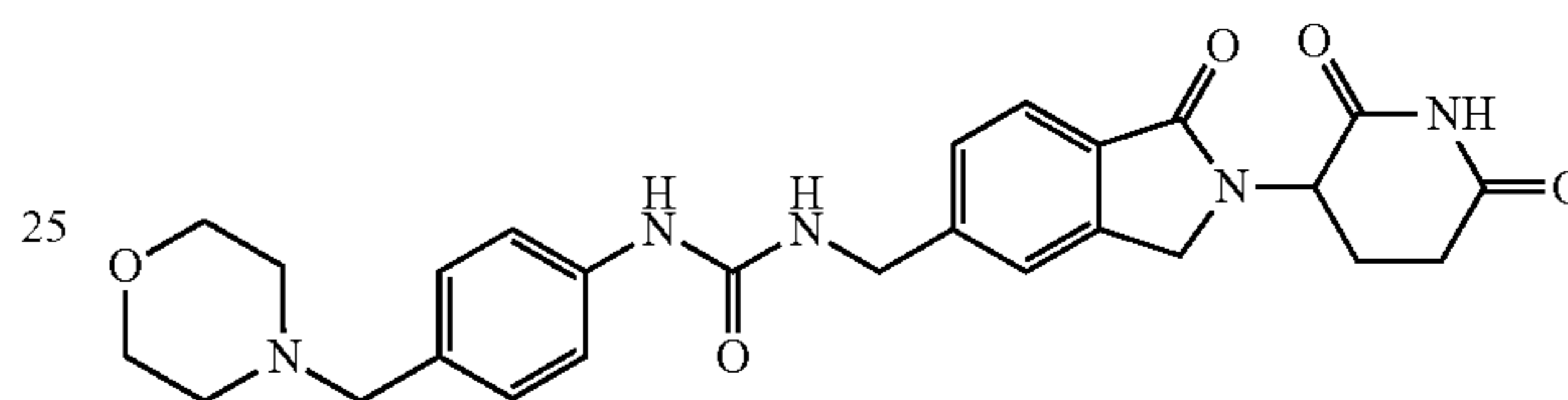
5.25 1-((2-(2,6-Dioxopiperidin-3-yl)-1-oxoisindolin-5-yl)methyl)-3-(4-(morpholinomethyl)phenyl)urea
