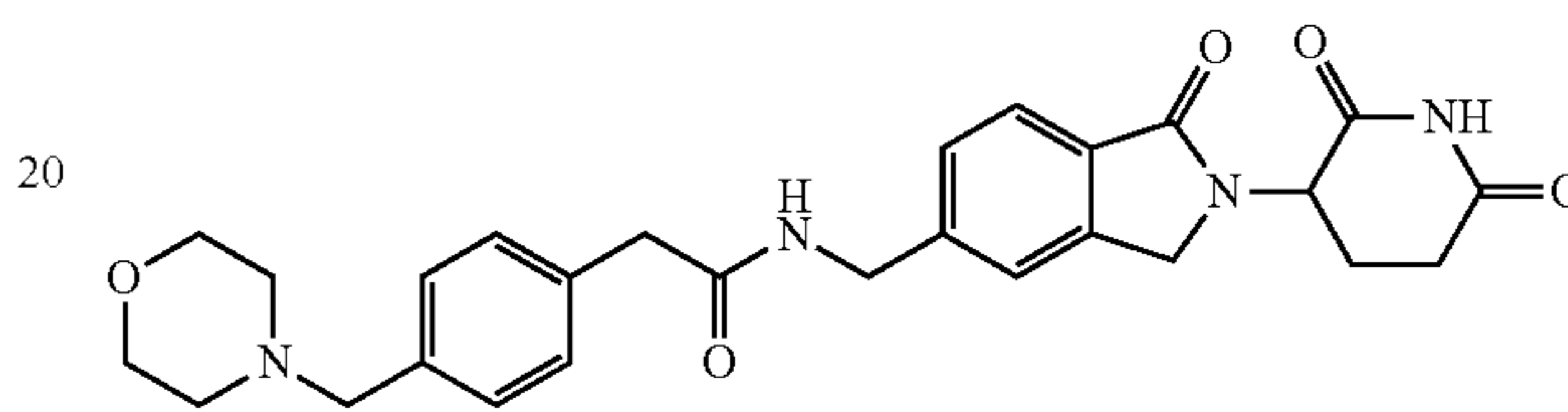
N-((2-(2,6-dioxopiperidin-3-yl)-1-oxoindolin-5-yl)methyl)-2-(4-(morpholinomethyl)phenyl)acetamide;
