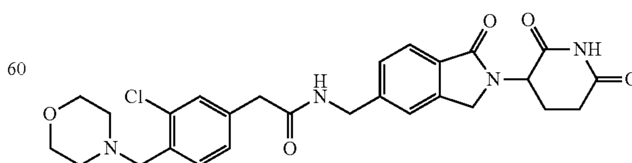
2-(3-chloro-4-(morpholinomethyl)phenyl)-N-((2-(2,6-dioxopiperidin-3-yl)-1-oxoindolin-5-yl)methyl)acetamide;
