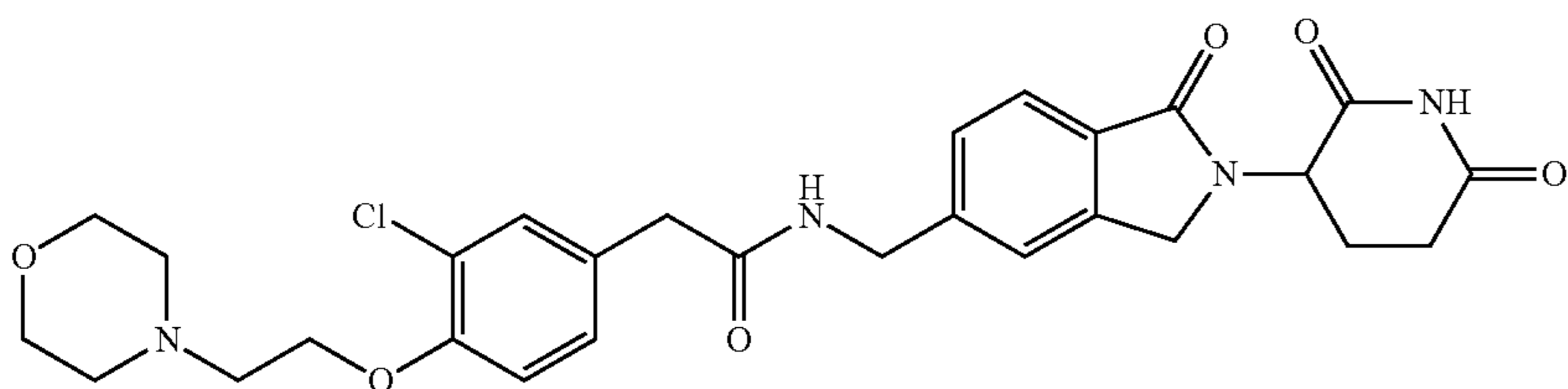
2-(3-chloro-4-(2-morpholinoethoxy)phenyl)-N-((2-(2,6-dioxopiperidin-3-yl)-1-oxoisindolin-5-yl)methyl)acetamide;
