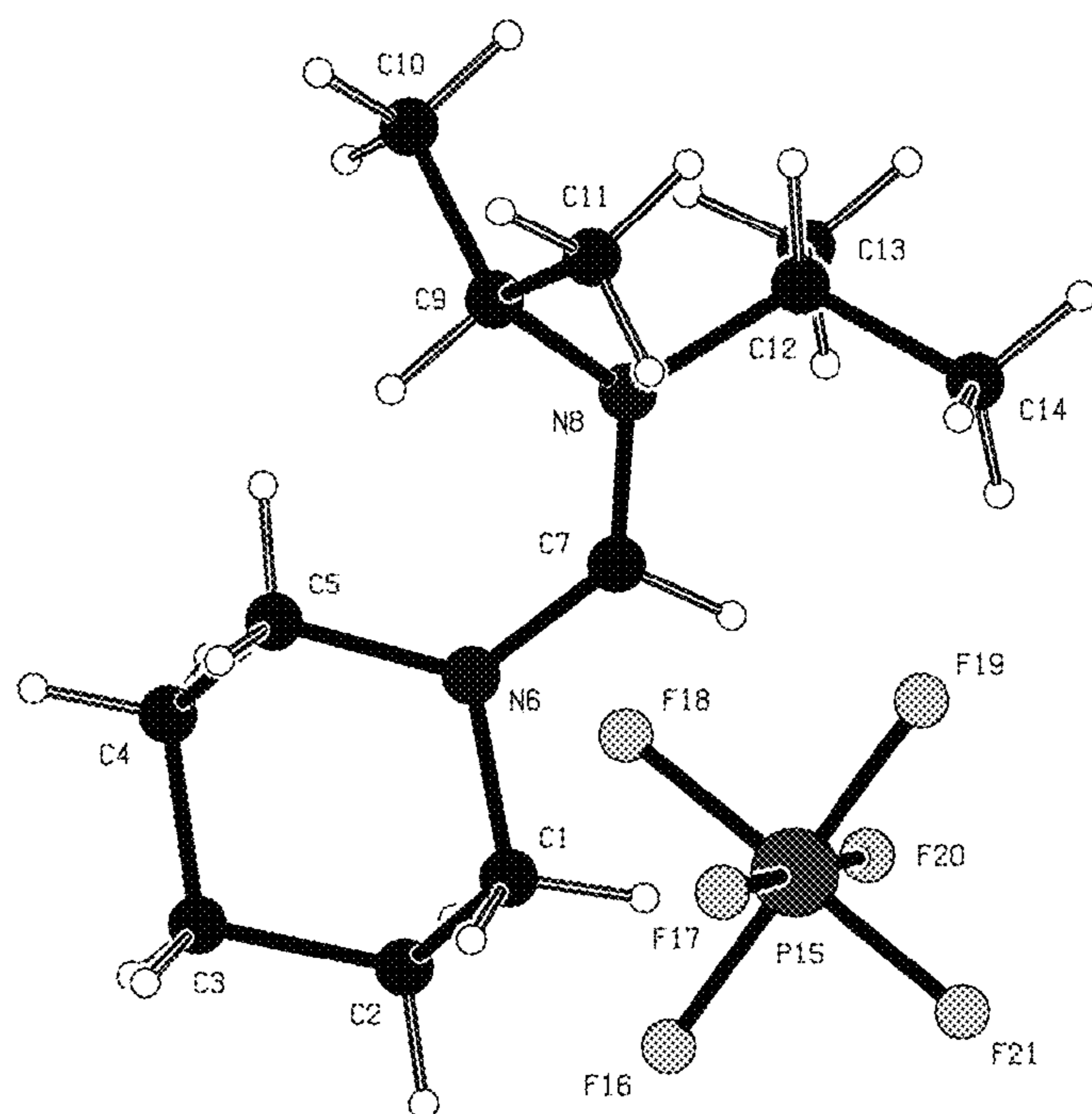
Diisopropyl(piperidin-1-ylmethylidene)ammonium hexafluorophosphate
