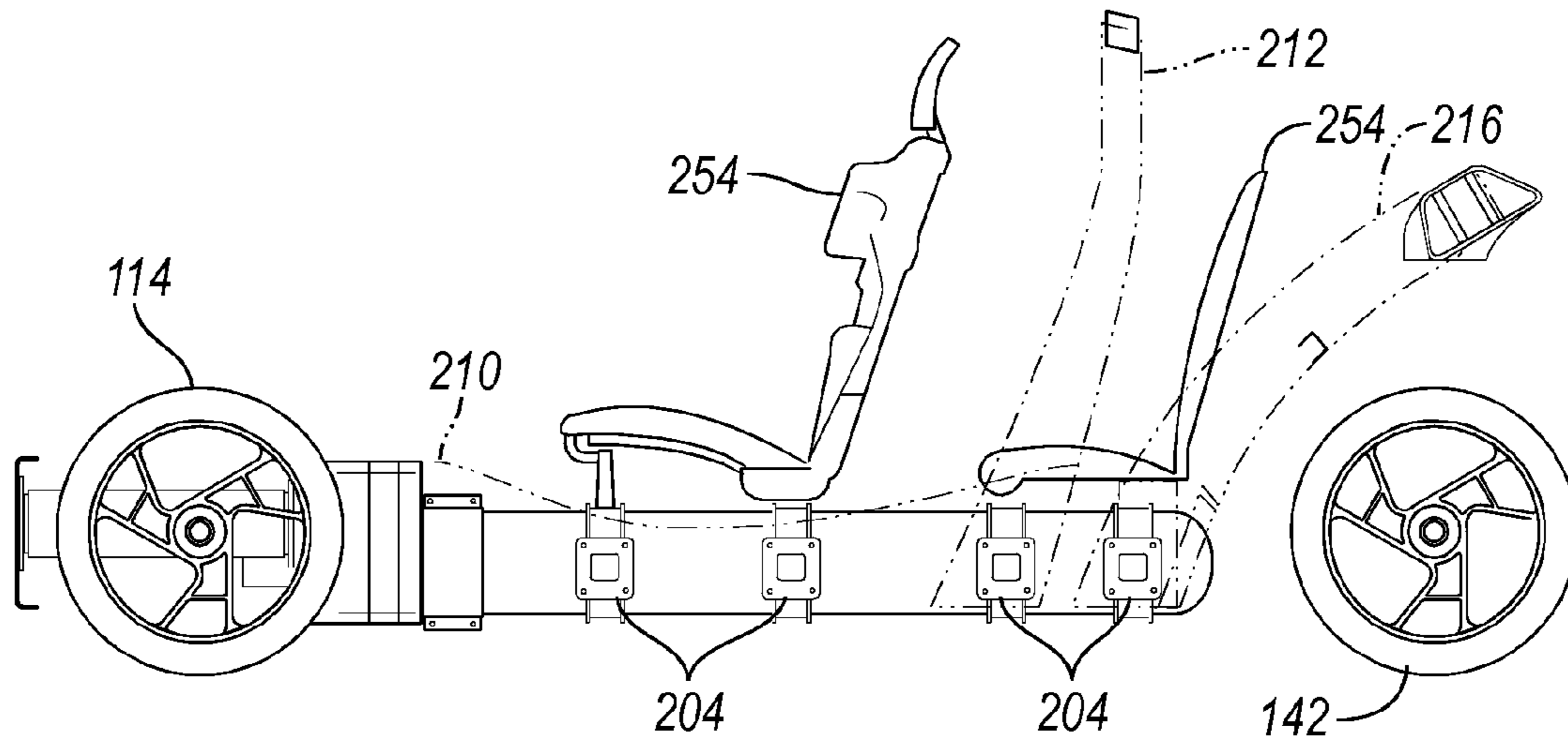
SIDE STRUCTURE
