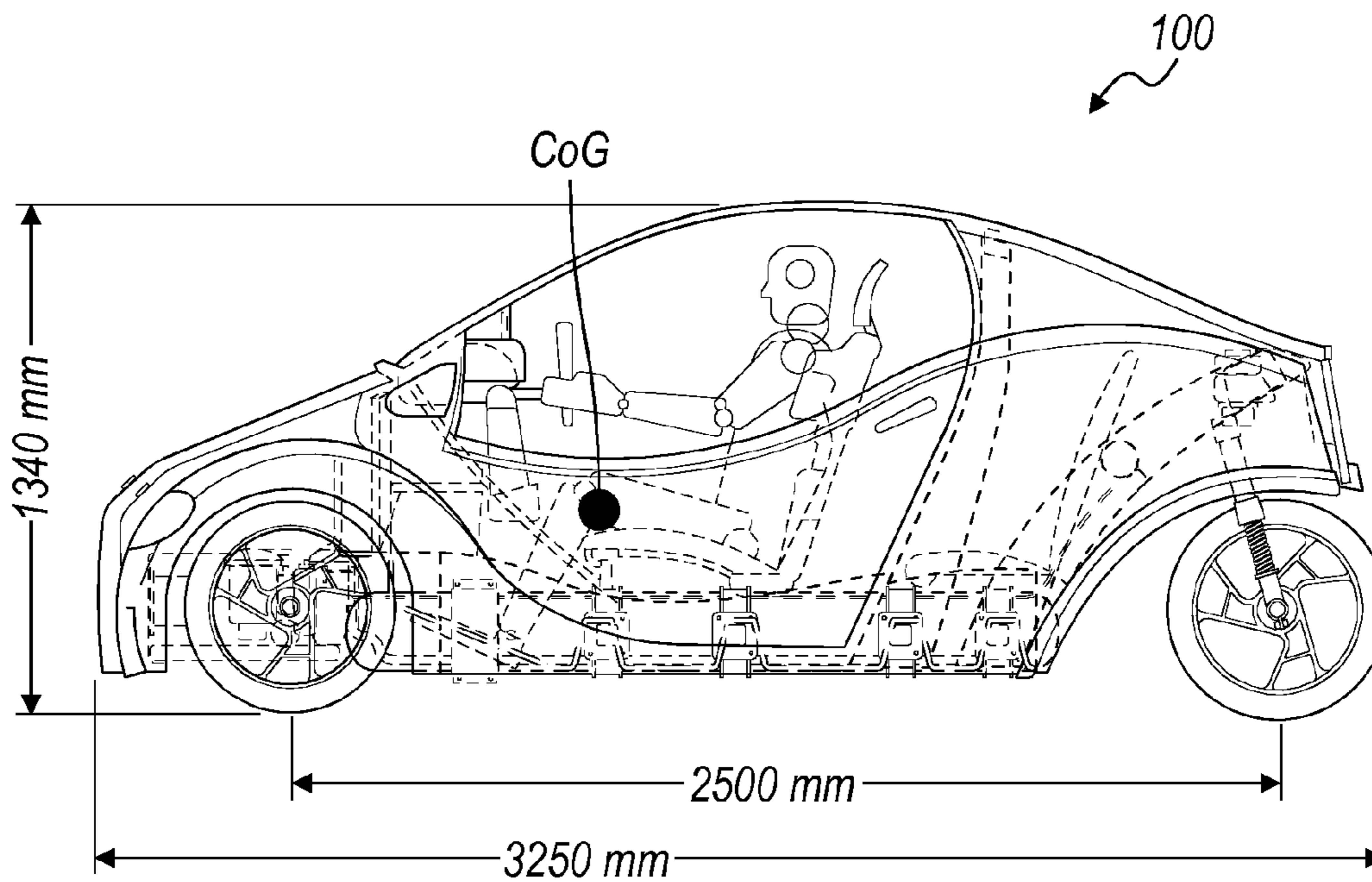
VEHICLE DIMENSIONS
