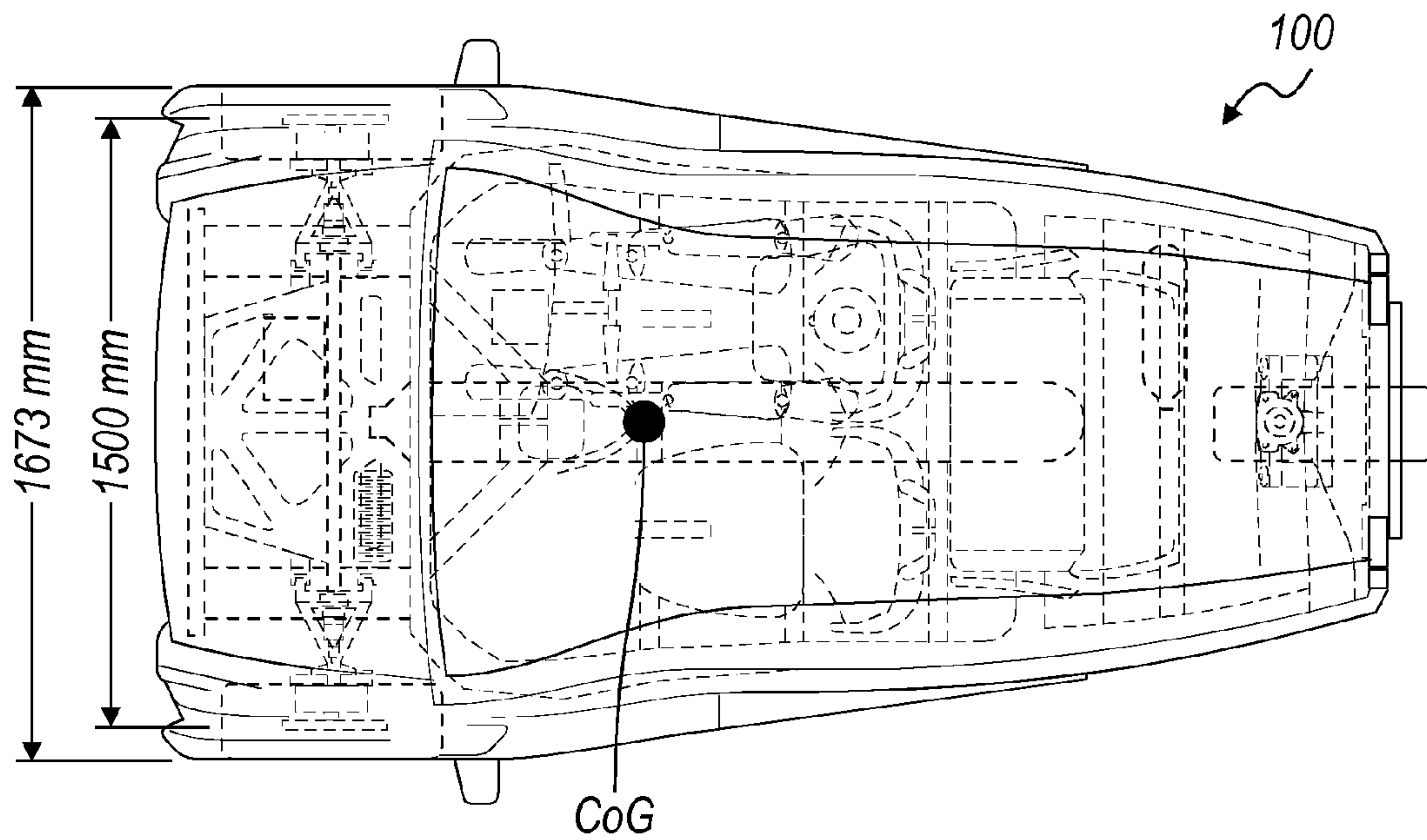
VEHICLE DIMENSIONS
