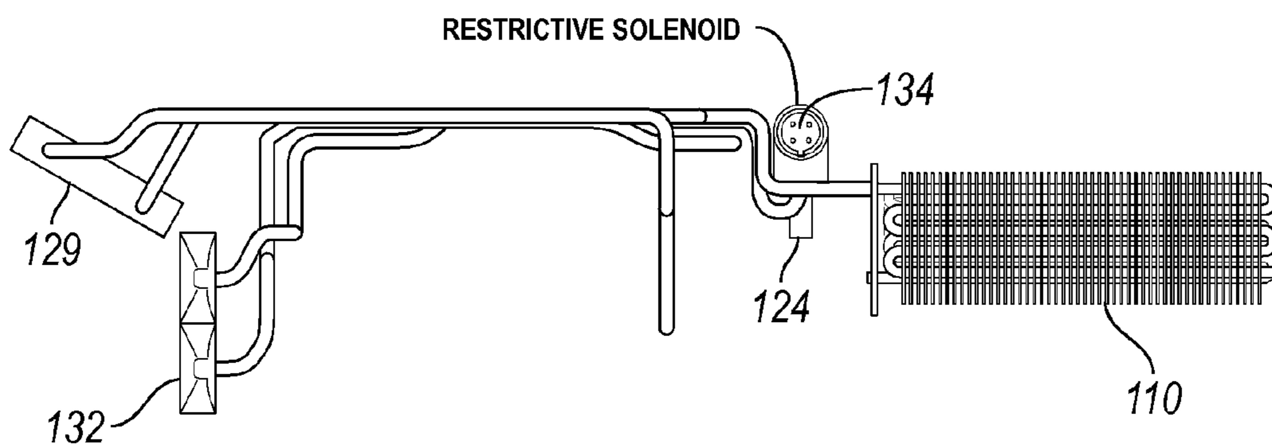
ANOTHER VIEW OF THE HVAC CONNECTIONS
