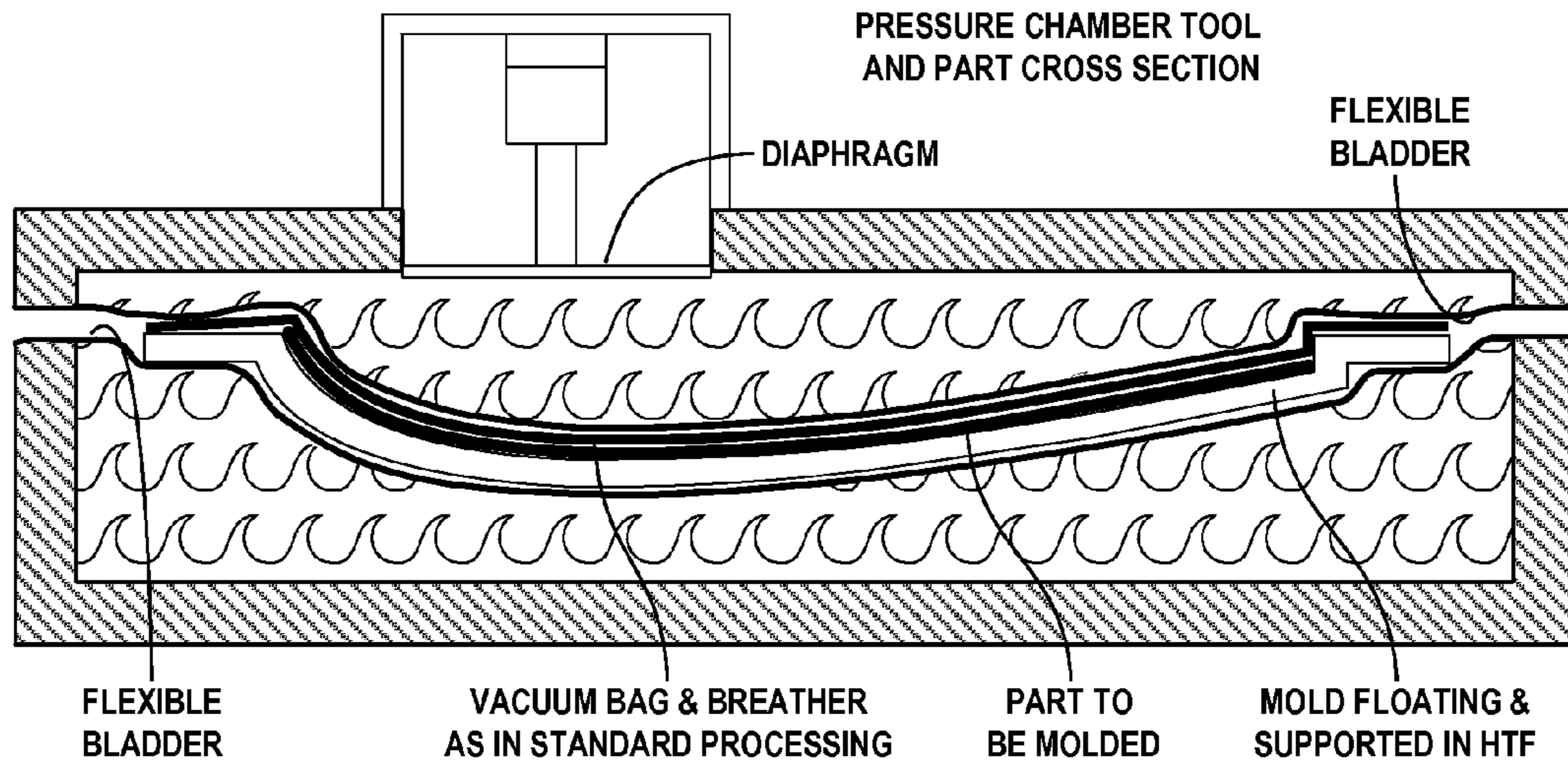
SCHEMATIC OF THE COMPOSITE LAYER PROCESS
