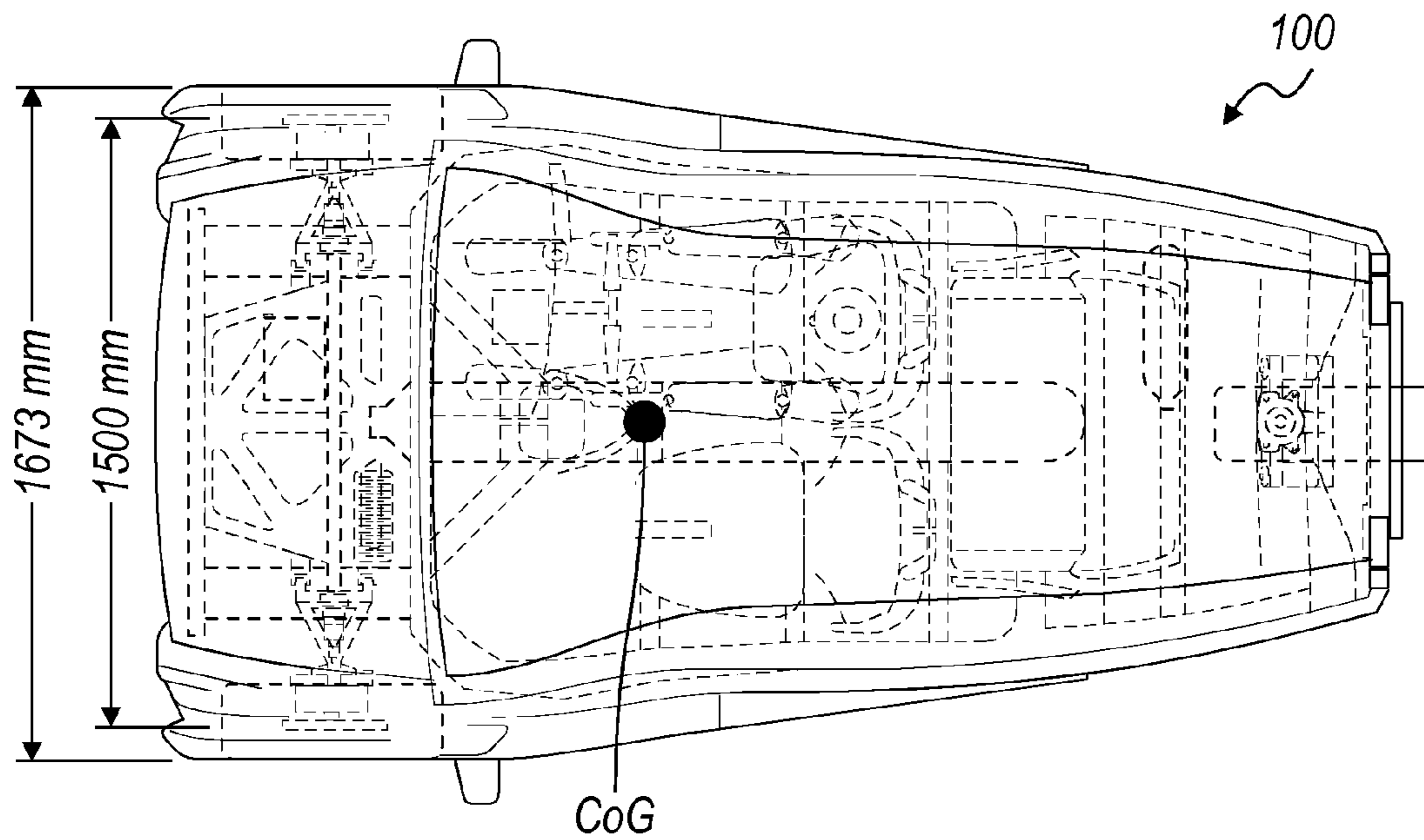
VEHICLE DIMENSIONS
