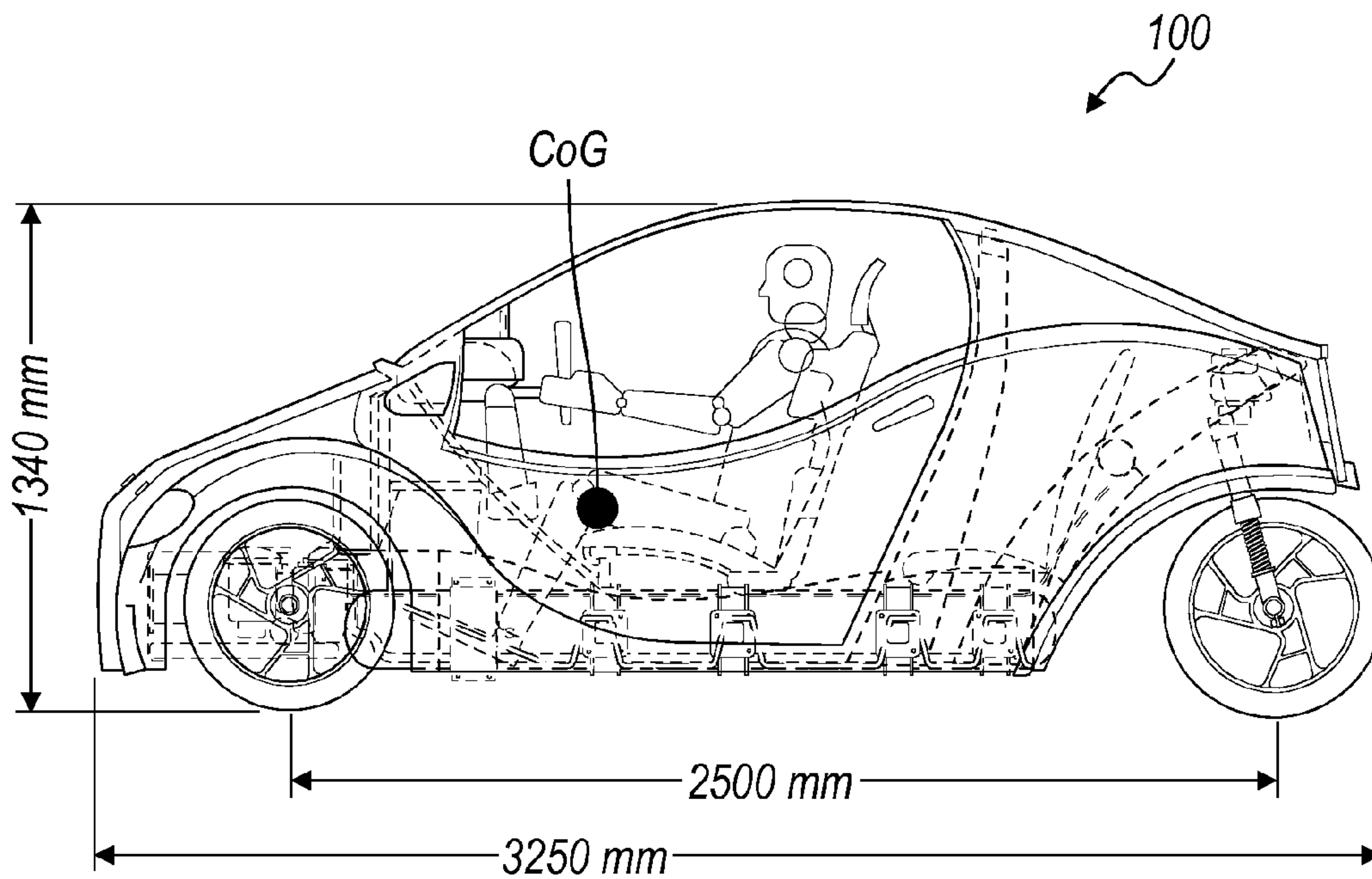
VEHICLE DIMENSIONS
