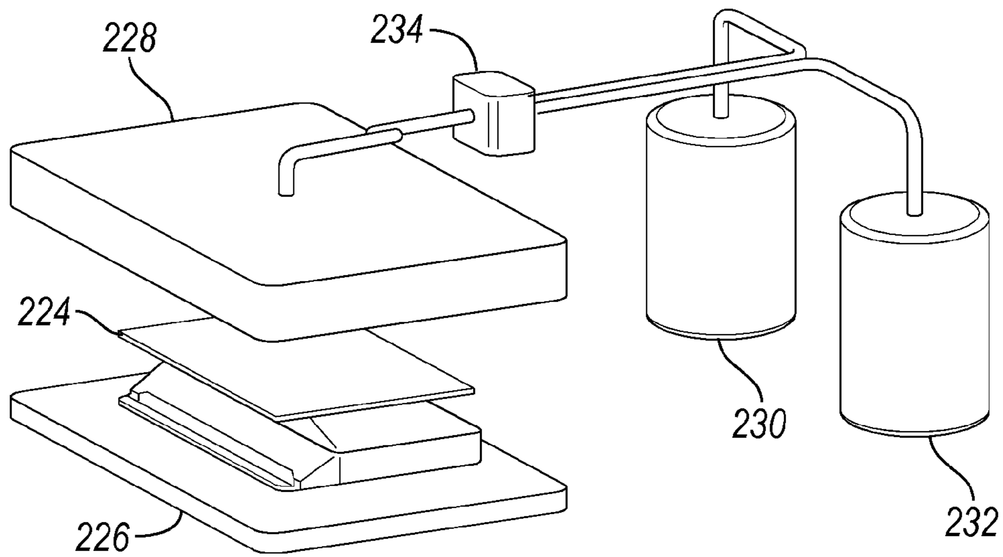
THE RTM PROCESS FOR THERMOSETS
