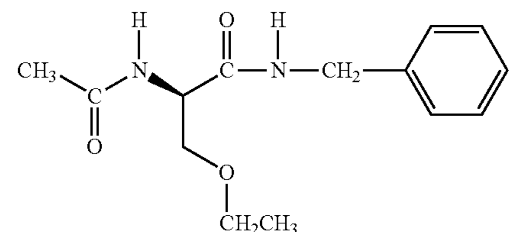
(R)-N-benzyl-2-acetamido-3-ethoxy propionamide
