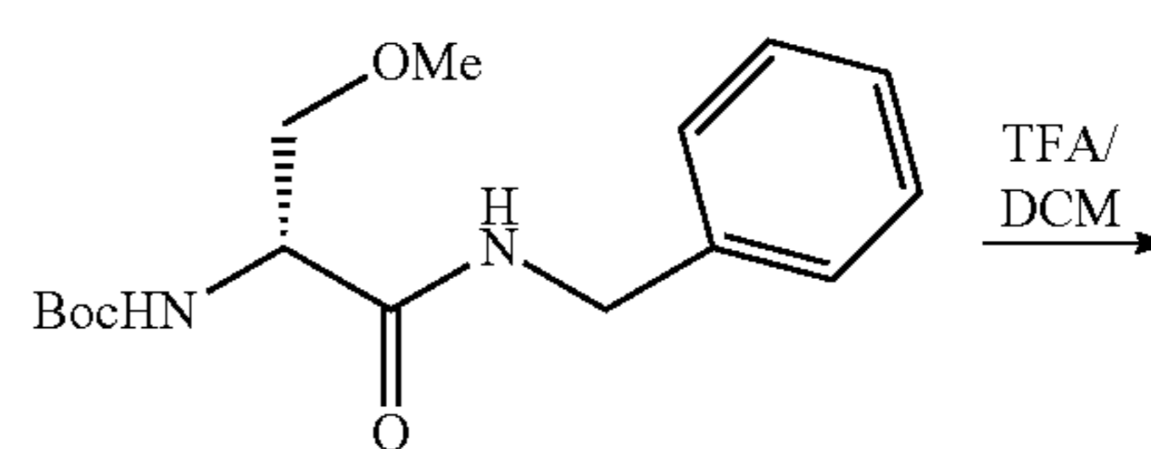
(R)-N-benzyl-2-N-Boc-amino-3-methoxypropionamide
