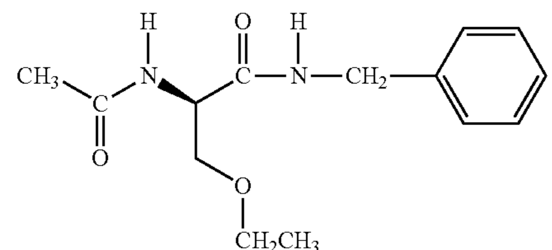
(R)-N-benzyl-2-acetamido-3-ethoxy propionamide
