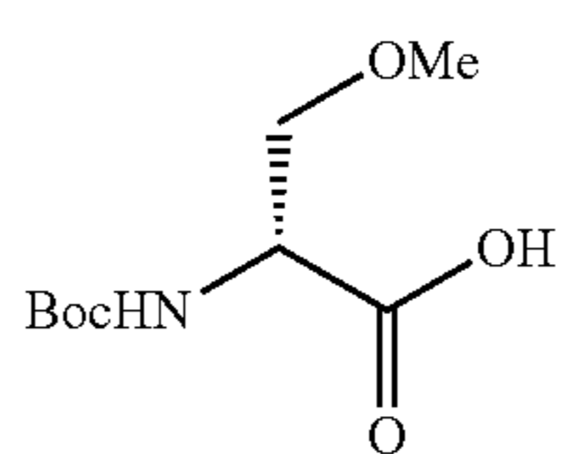
(R)-2-N-Boc-amino-3-methoxypropanoic acid
