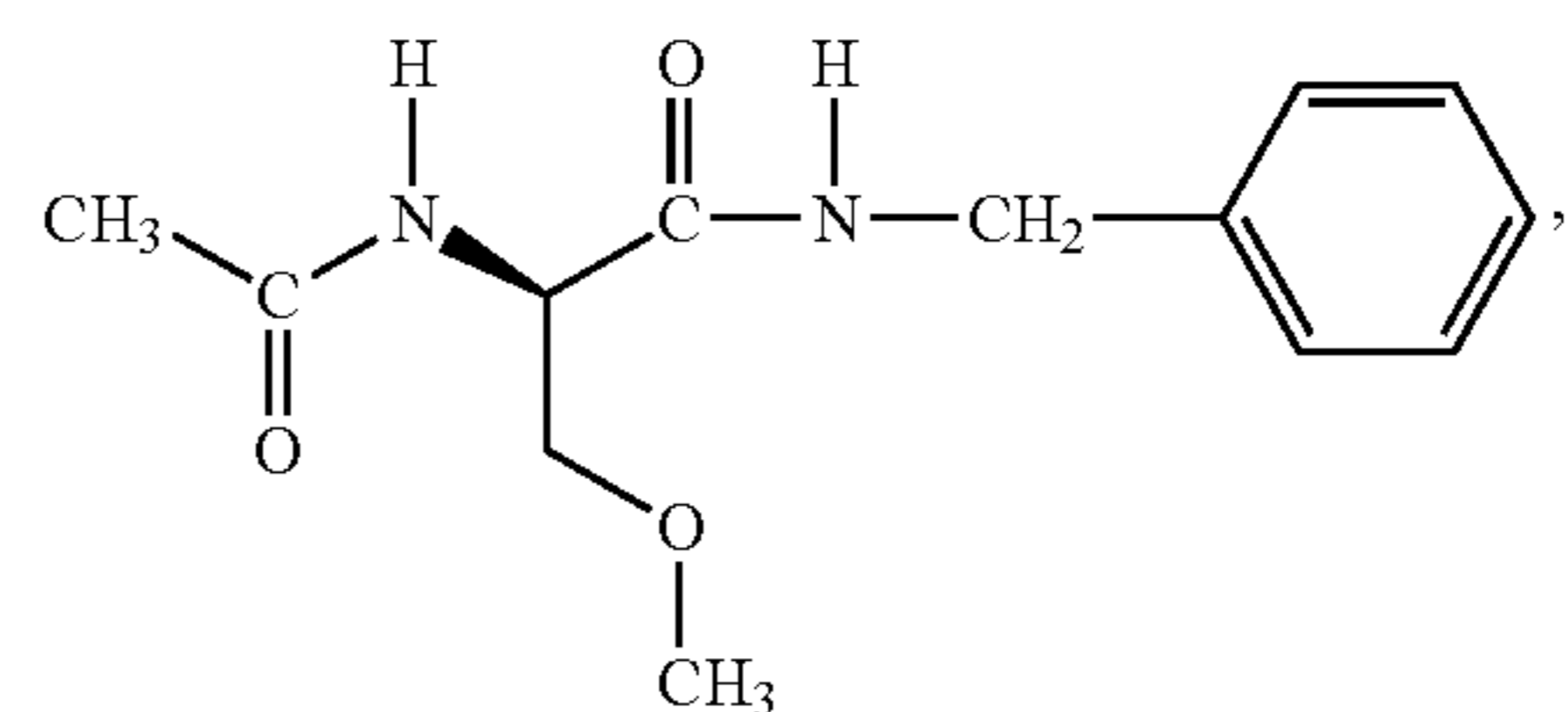
(R)-N-benzyl-2-acetamido-3-methoxy propionamide (lacosamide)
