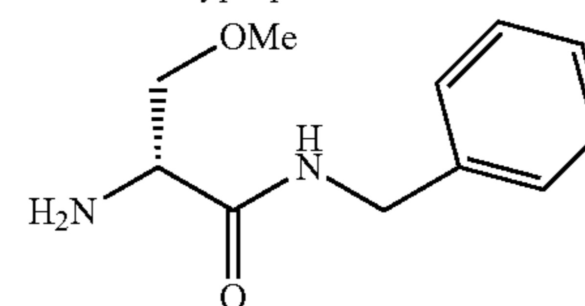
(R)-2-amino-N-benzyl-3-methoxypropionamide
