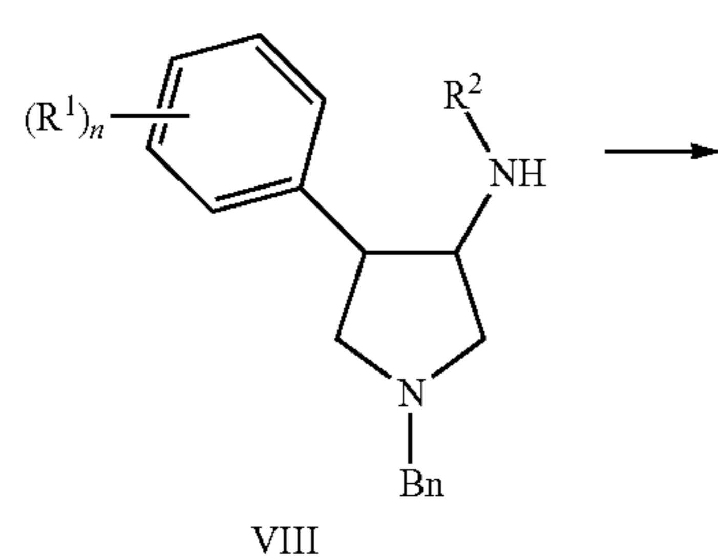
Scheme 2
