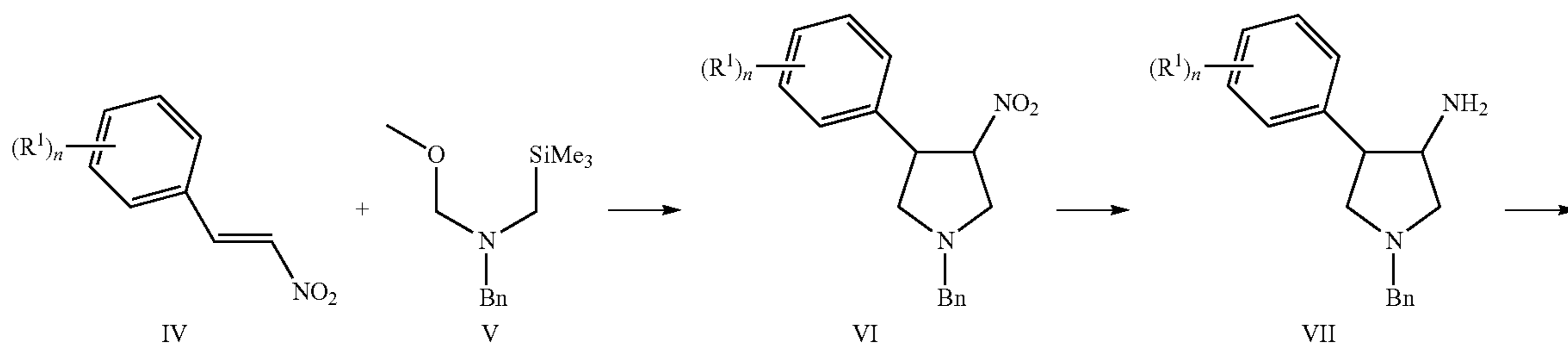
Scheme 1
