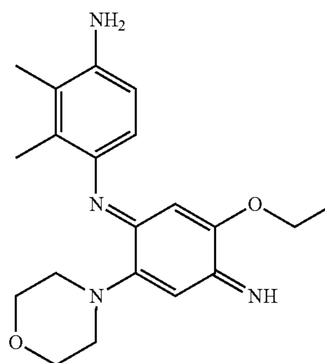
N-(5-Ethoxy-4-imino-2-morpholin-4-ylcyclohexa-2,5-dienylidene)-2,3-dimethylbenzene-1,4-diamine
