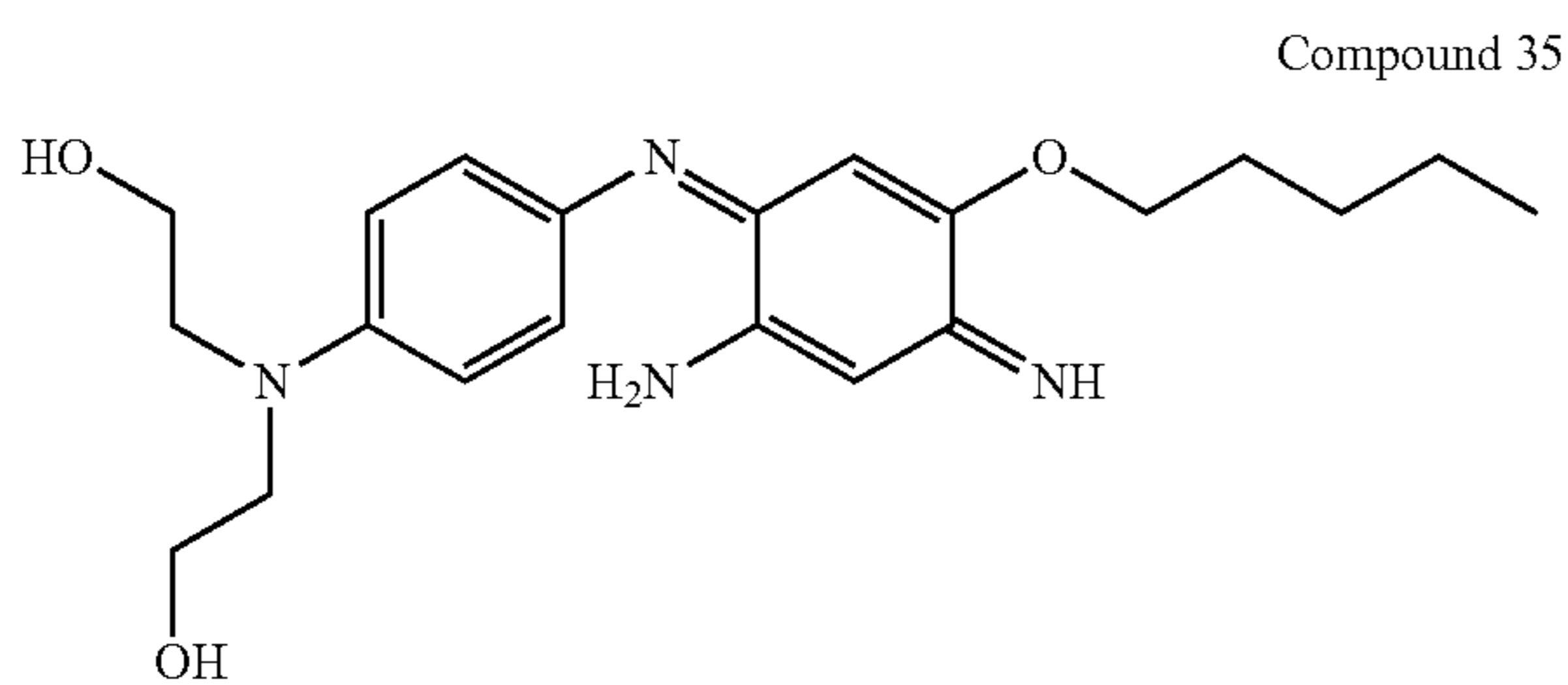
2-[[4-(2-Amino-5-pentyloxy-4-iminocyclohexa-2,5-dienylideneamino)phenyl(2-hydroxyethyl)amino]ethanol
