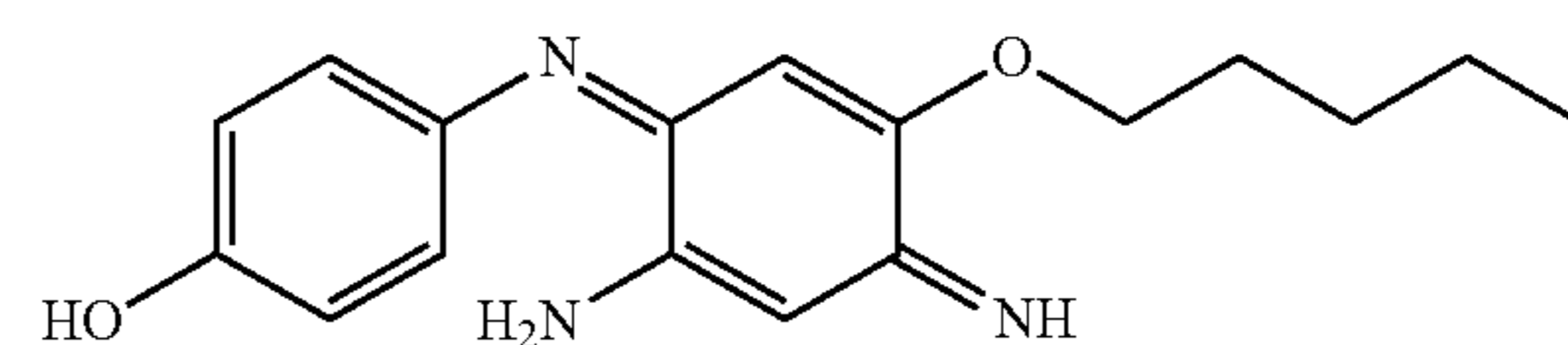
4-(2-Amino-5-hexyloxy-4-iminocyclohexa-2,5-dienylideneamino)phenol
