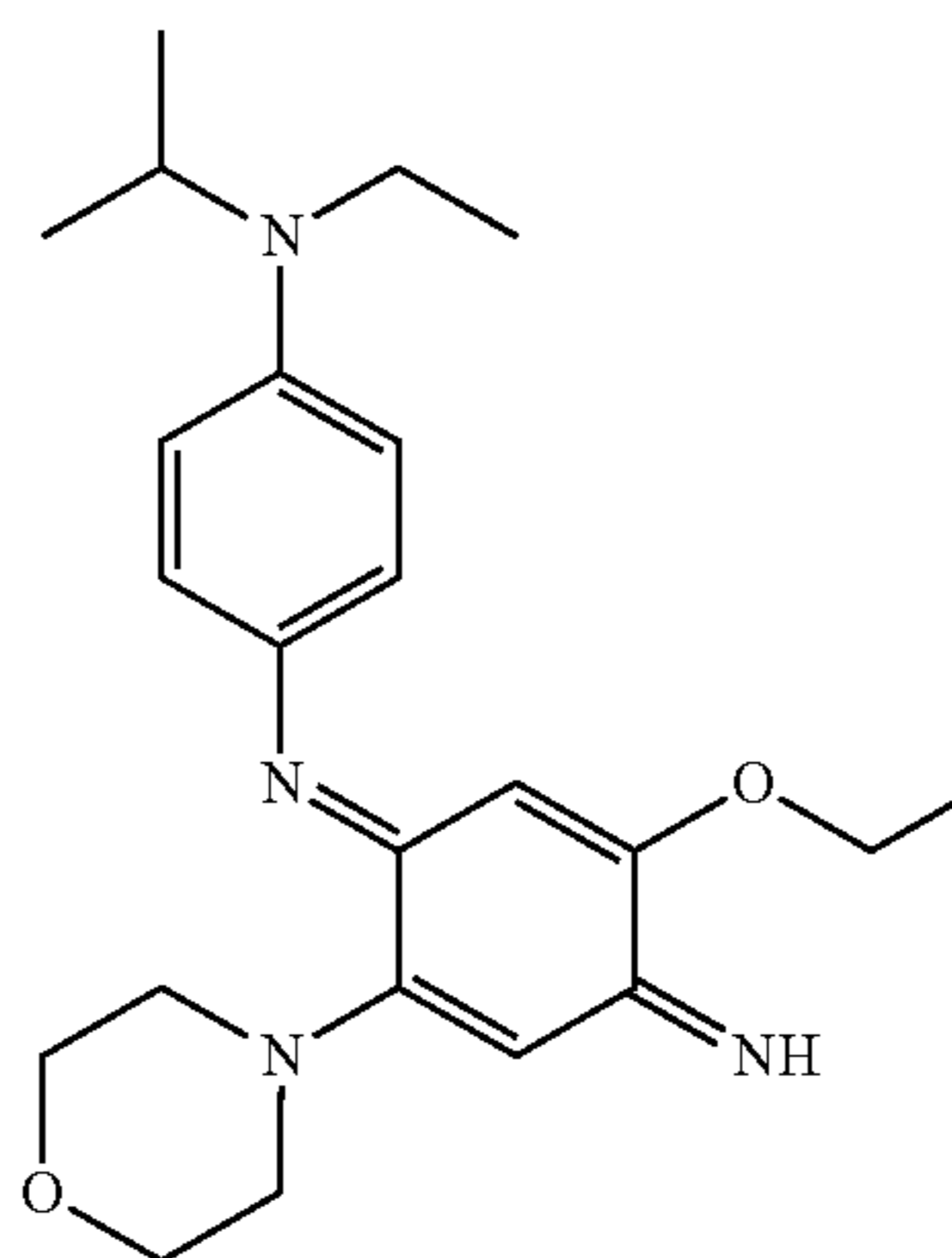
N-(5-Ethoxy-4-imino-2-morpholin-4-ylcyclohexa-2,5-dienylidene)-N'-ethyl-N'-isopropylbenzene-1,4-diamine
