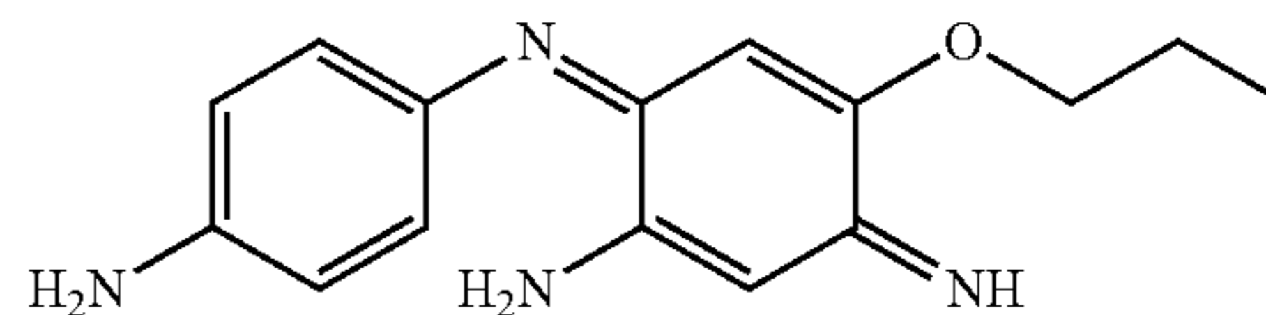
6-(4-Aminophenylimino)-4-propoxy-3-iminocyclohexa-1,4-dienylamine
