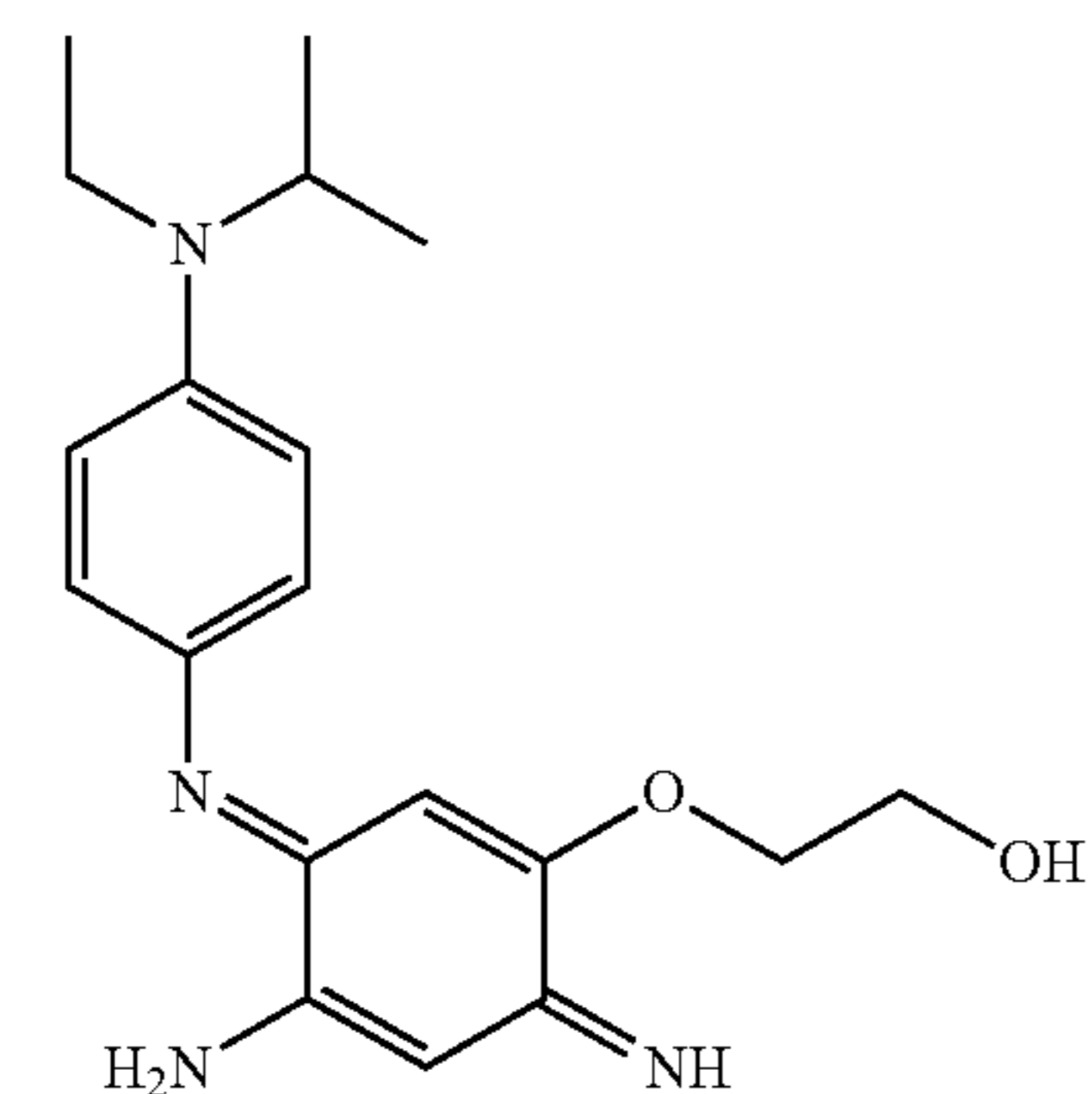
2-{4-Amino-3-[4-(ethylisopropylamino)phenylimino]-6-iminocyclohexa-1,4-dienyloxy}ethanol
