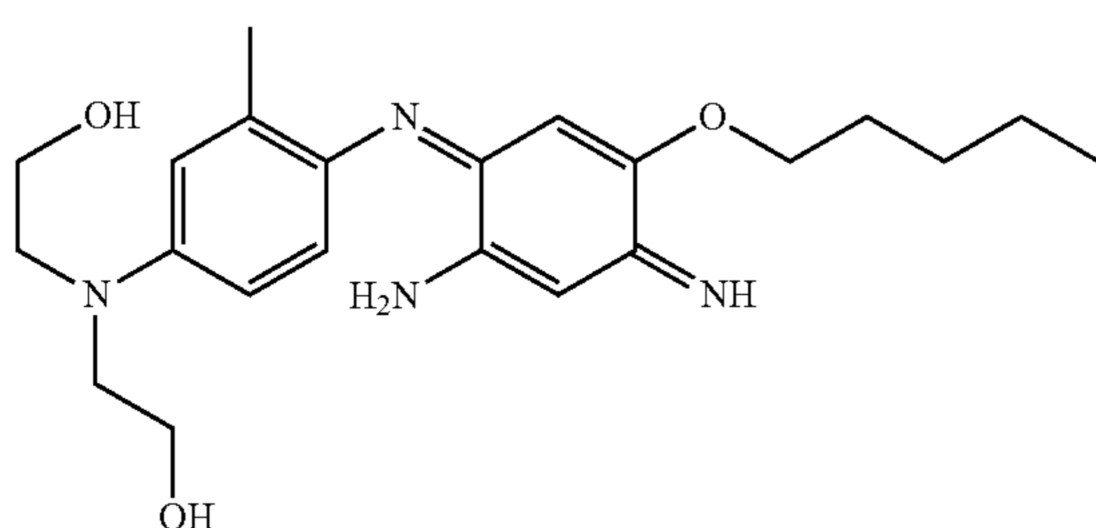
2-[[4-(2-Amino-5-pentyloxy-4-iminocyclohexa-2,5-dienylideneamino)-3-methylphenyl(2-hydroxyethyl)amino]ethanol
