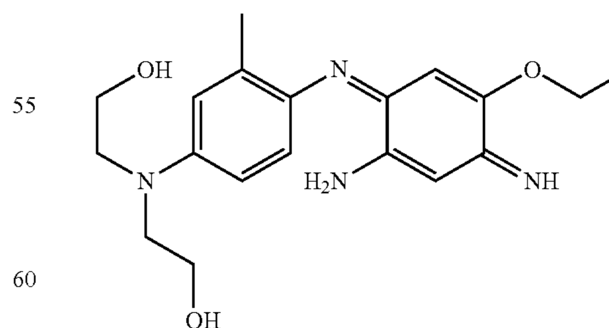
2-[[4-(2-Amino-5-ethoxy-4-iminocyclohexa-2,5-dienylideneamino)-3-methylphenyl](2-hydroxyethyl)amino] ethanol
