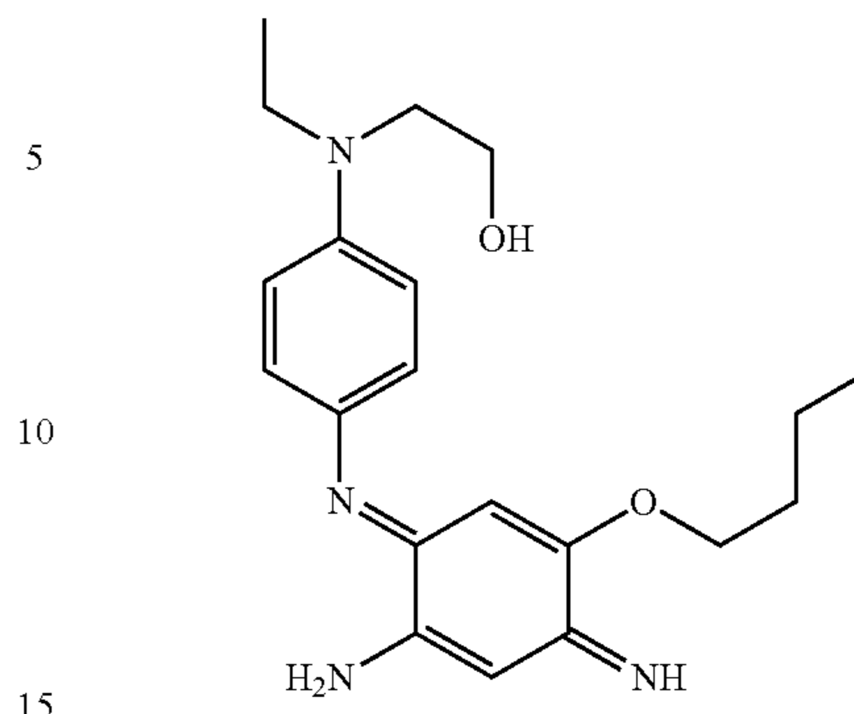
2-((4-[2-Amino-5-butoxy-4-iminocyclohexa-2,5-dienylideneamino]phenyl)ethylamino)ethanol
