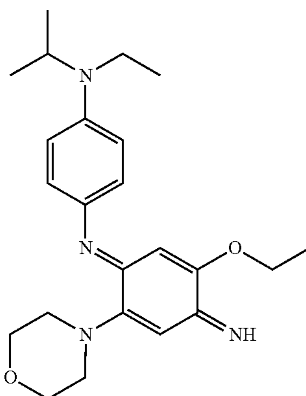
N-(5-Ethoxy-4-imino-2-morpholin-4-ylcyclohexa-2,5-dienylidene)-N'-ethyl-N'-isopropylbenzene-1,4-diamine
