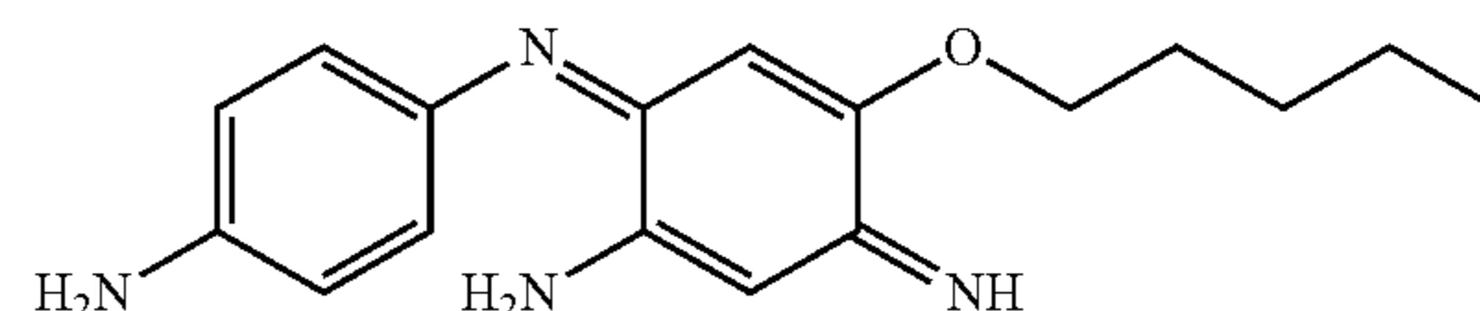
6-(4-Aminophenylimino)-4-hexyloxy-3-iminocyclohexa-1,4-dienylamine
