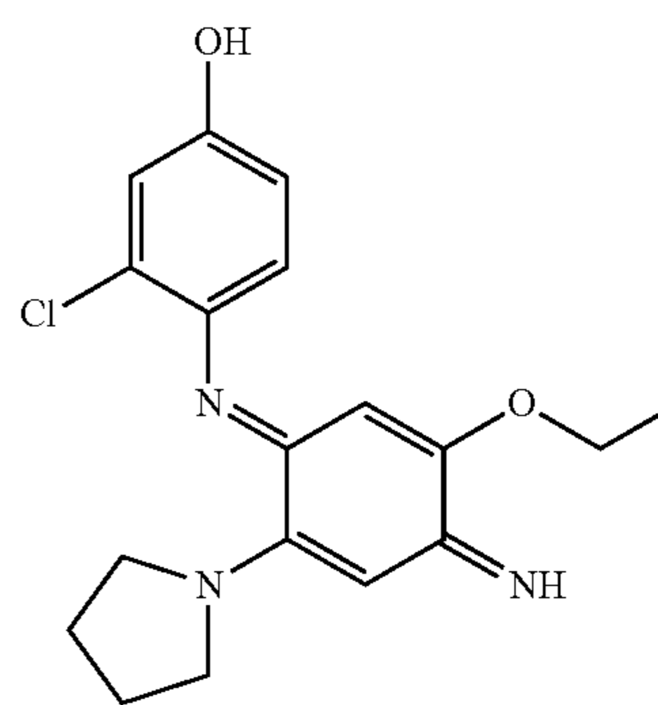
3-Chloro-4-(5-ethoxy-4-imino-2-pyrrolidin-1-ylcyclohexa-2,5-dienylideneamino)phenol
