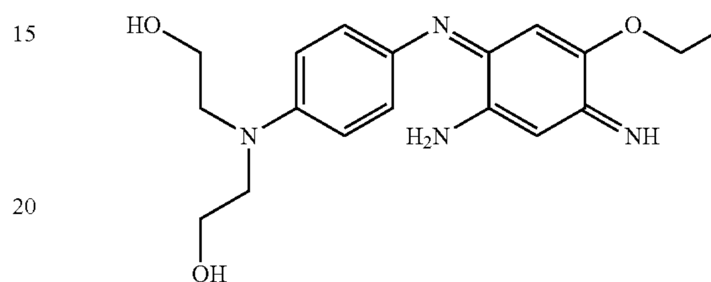
2-[[4-(2-Amino-5-ethoxy-4-iminocyclohexa-2,5-dienylideneamino)phenyl](2-hydroxyethyl)amino] ethanol
