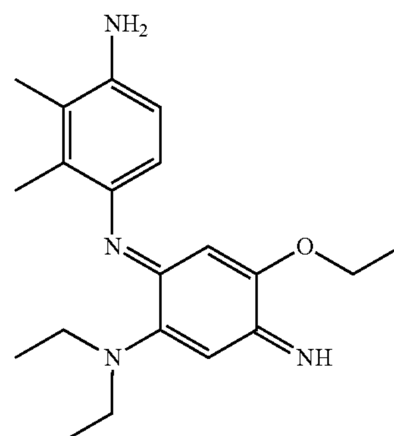
N-(2-Diethylamino-5-ethoxy-4-iminocyclohexa-2,5-dienylidene)-2,3-dimethylbenzene-1,4-diamine
