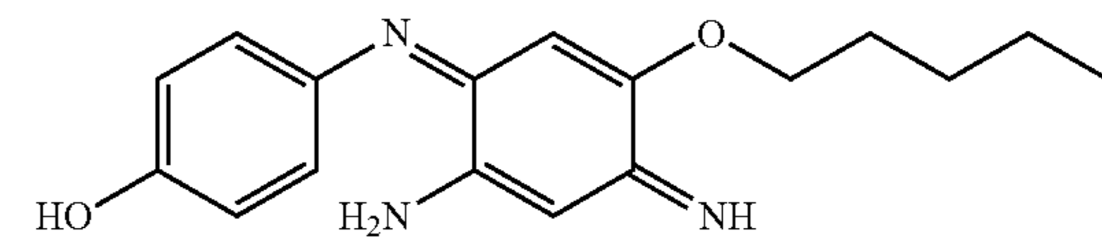
4-(2-Amino-5-pentyloxy-4-aminocyclohexa-2,5-dienylideneamino)phenol
