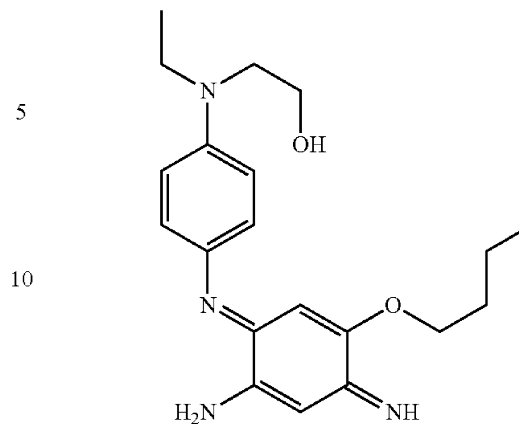
2-({4-[2-Amino-5-butoxy-4-iminocyclohexa-2,5-dienylideneamino]phenyl}ethylamino)ethanol
