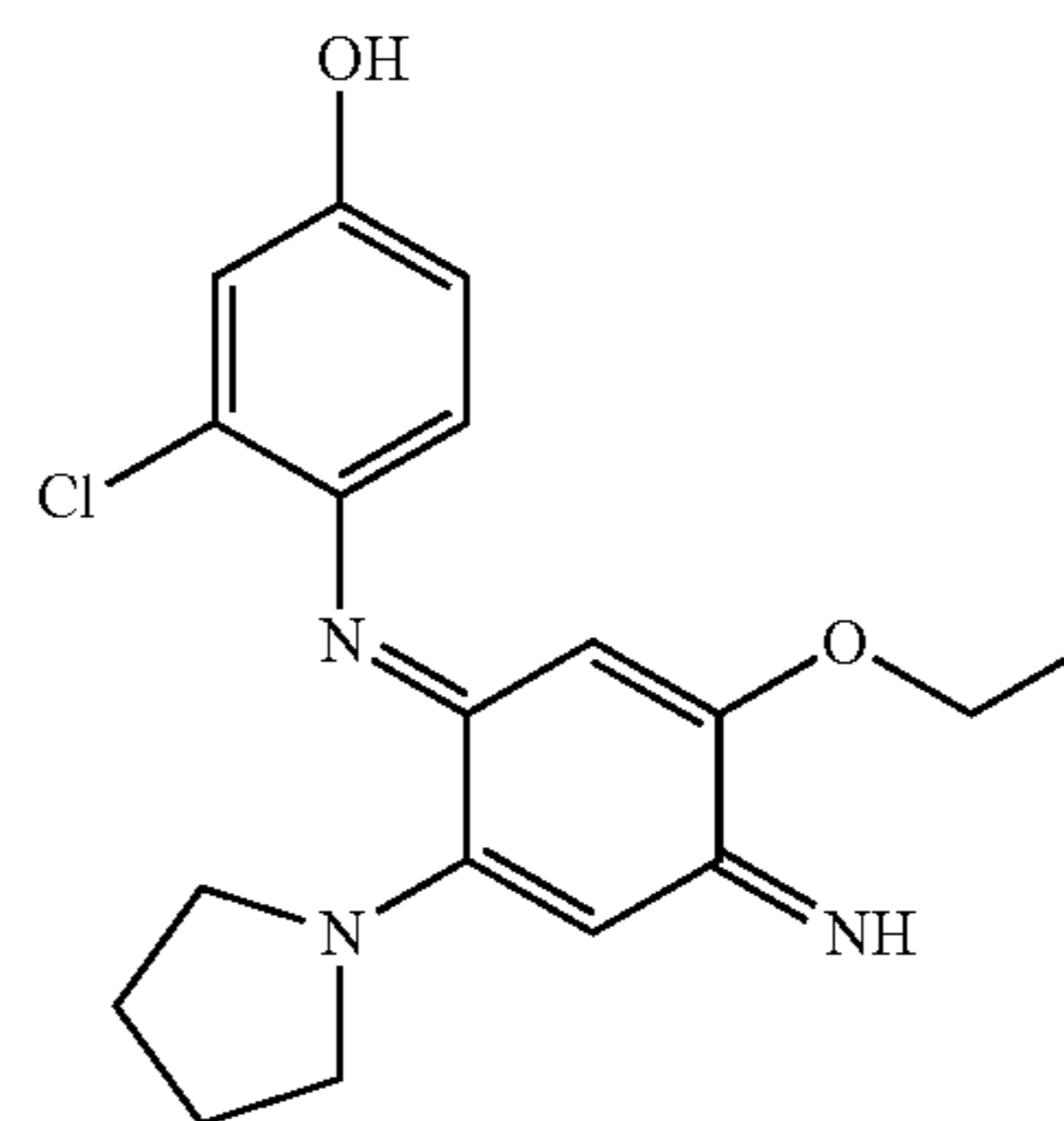
3-Chloro-4-(5-ethoxy-4-imino-2-pyrrolidin-1-ylcyclohexa-2,5-dienylideneamino)phenol
