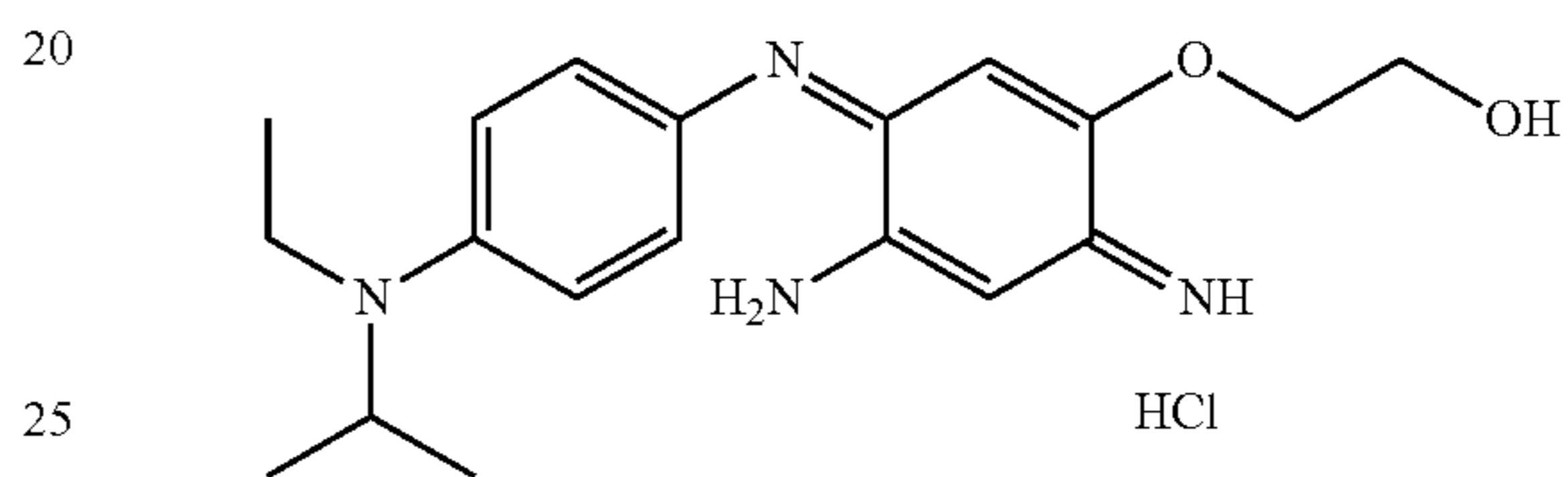
2-(4-amino-3-[4-(ethylisopropylamino)phenylimino]-6-iminocyclohexa-1,4-dienyloxy)ethanol
