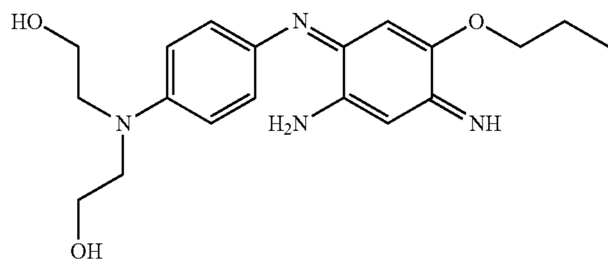
2-[[4-(2-Amino-5-propoxy-4-iminocyclohexa-2,5-dienylideneamino)phenyl](2-hydroxyethyl)amino]ethanol
