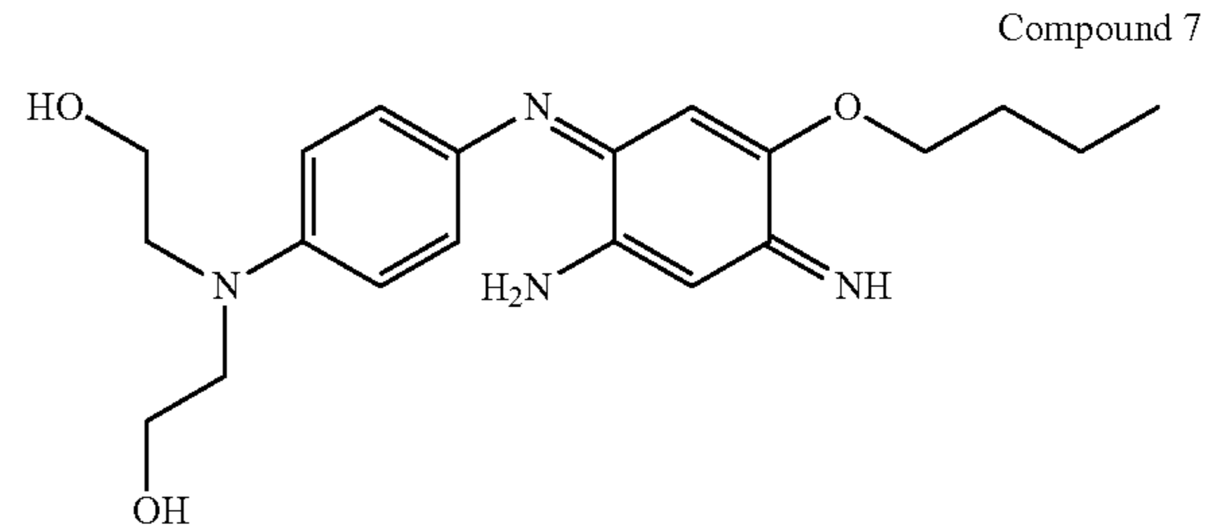
2-([4-(2-Amino-5-butoxy-4-iminocyclohexa-2,5-dienylideneamino)phenyl](2-hydroxyethyl)amino)ethanol
