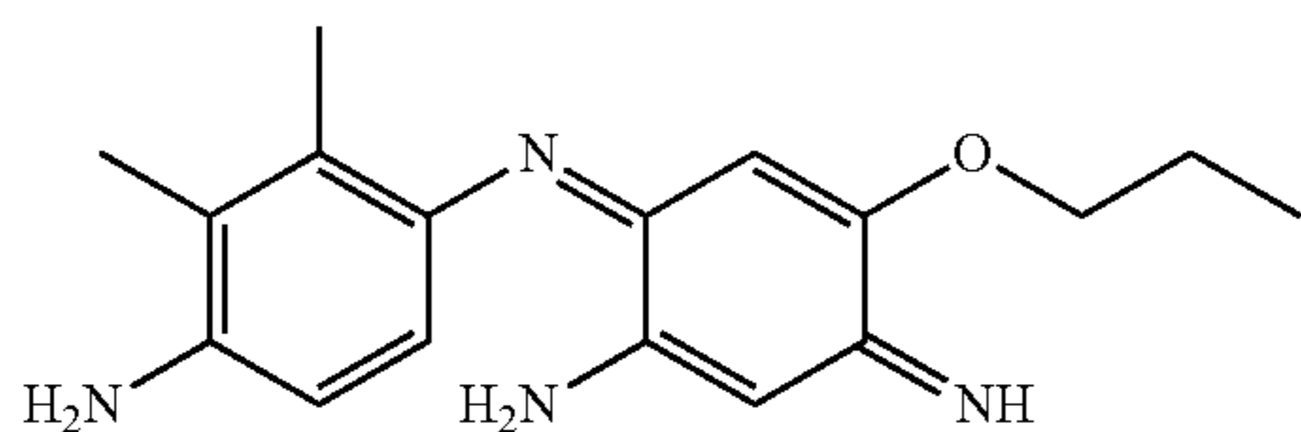
6-(2-Amino-2,3-dimethylphenylimino)-4-propoxy-3-iminocyclohexa-1,4-dienylamine
