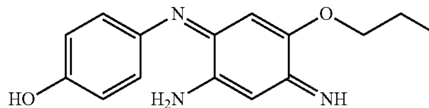
4-(2-Amino-5-butoxy-4-iminocyclohexa-2,5-dienylideneamino)phenol
