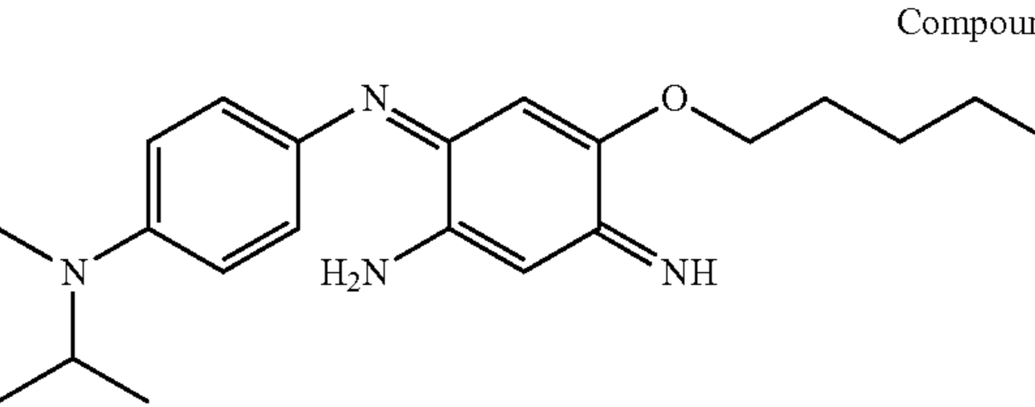
4-pentyloxy-6-[4-(ethylisopropylamino)phenylimino]-3-iminocyclohexa-1,4-dienylamine
