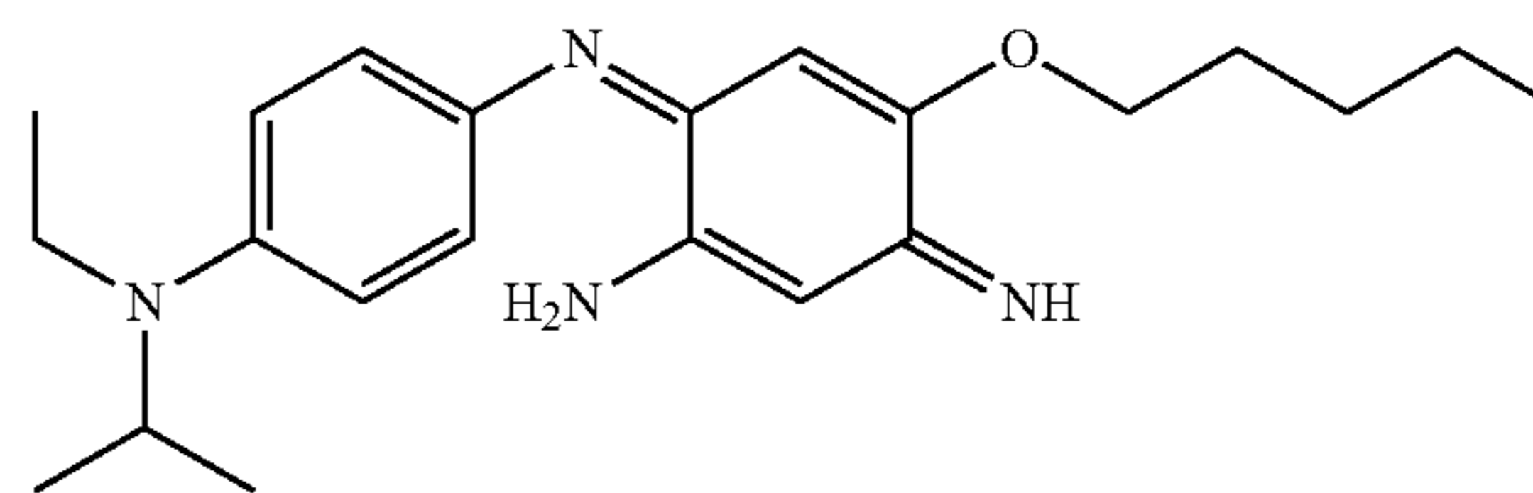
4-hexyloxy-6-[4-(ethylisopropylamino)phenylimino]-3-iminocyclohexa-1,4-dienylamine
