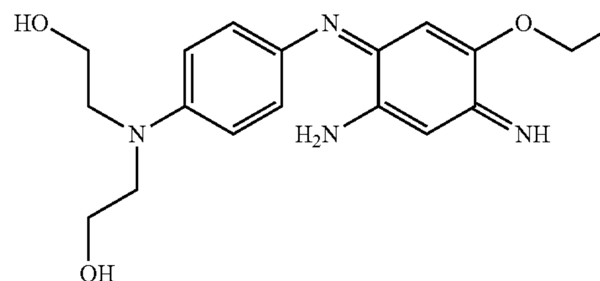
2-[[4-(2-Amino-5-ethoxy-4-iminocyclohexa-2,5-dienylideneamino)phenyl](2-hydroxyethyl)amino]ethanol
