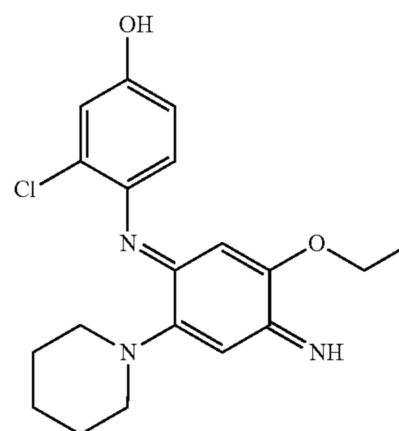
3-Chloro-4-(5-ethoxy-4-imino-2-piperidin-1-ylcyclohexa-2,5-dienylideneamino)phenol
