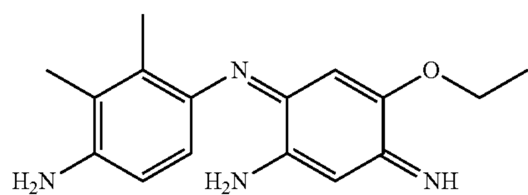
6-(4-Amino-2,3-dimethylphenylimino)-4-ethoxy-3-aminocyclohexa-1,4-dienylamine
