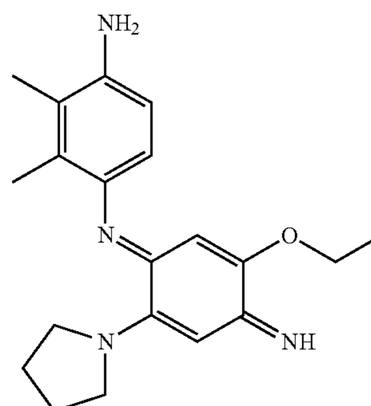
N-(5-Ethoxy-4-imino-2-pyrrolidin-1-ylcyclohexa-2,5-dienylidene)-2,3-dimethylbenzene-1,4-diamine
