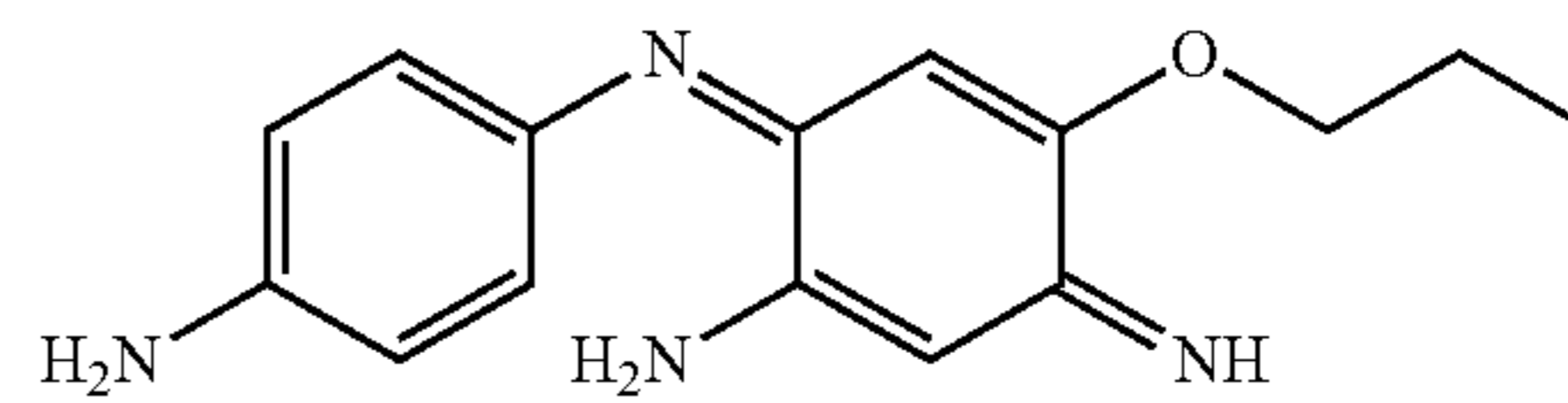
6-(4-Aminophenylimino)-4-propoxy-3-iminocyclohexa-1,4-dienylamine
