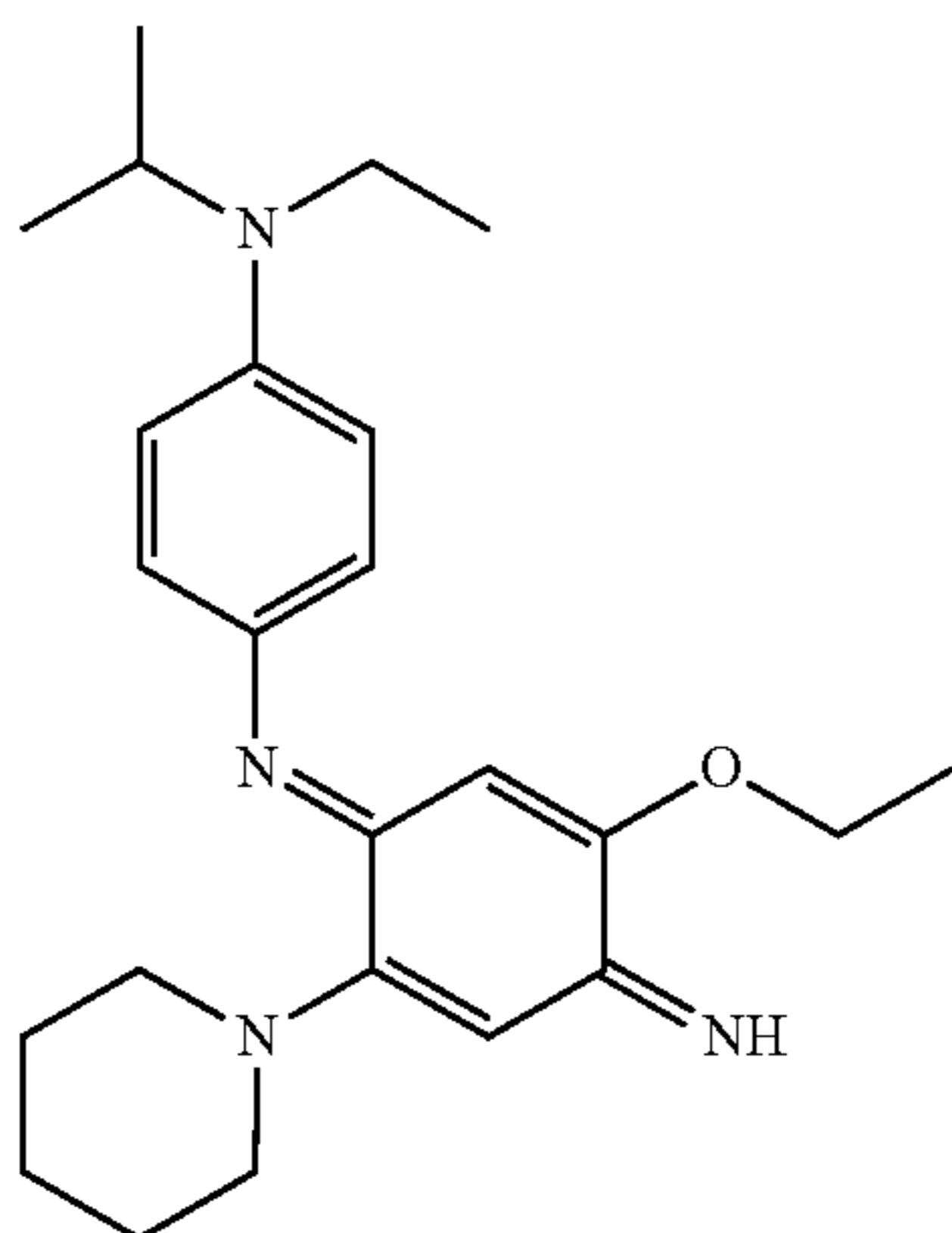
N-(5-Ethoxy-4-imino-2-piperidin-1-ylcyclohexa-2,5-dienylidene)-N'-ethyl-N'-isopropylbenzene-1,4-diamine
