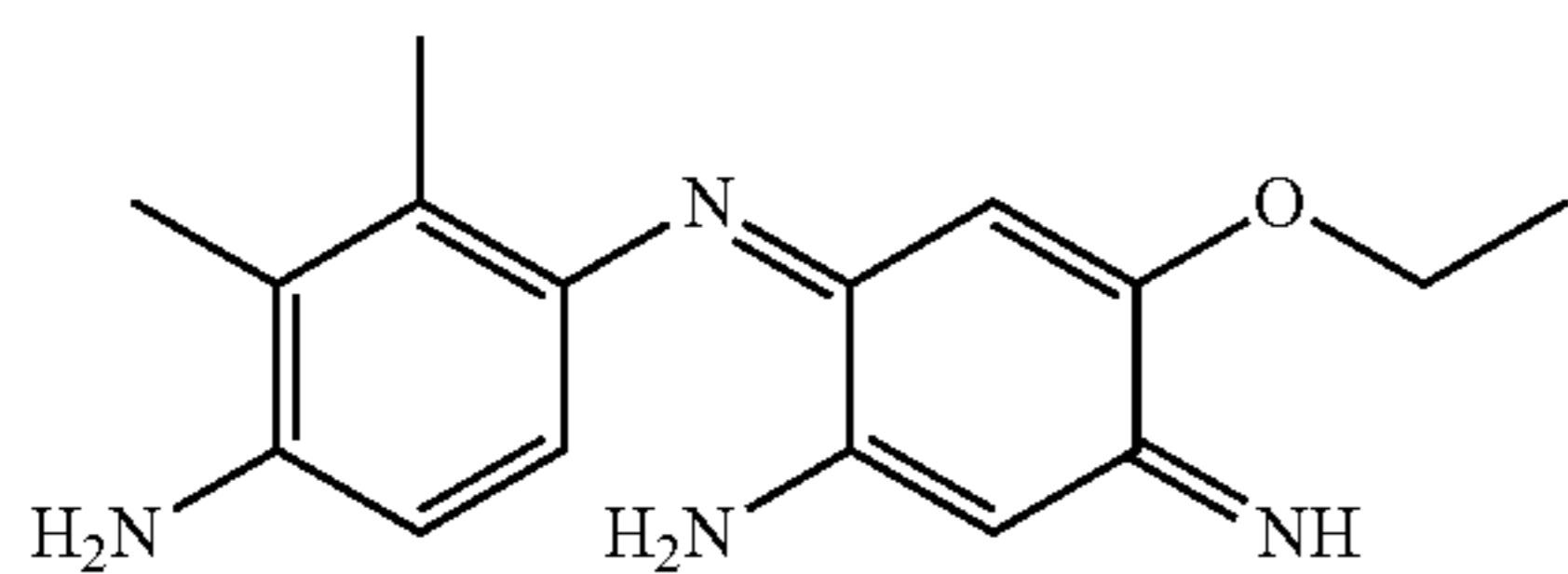
6-(4-Amino-2,3-dimethylphenylimino)-4-ethoxy-3-iminocyclohexa-1,4-dienylamine
