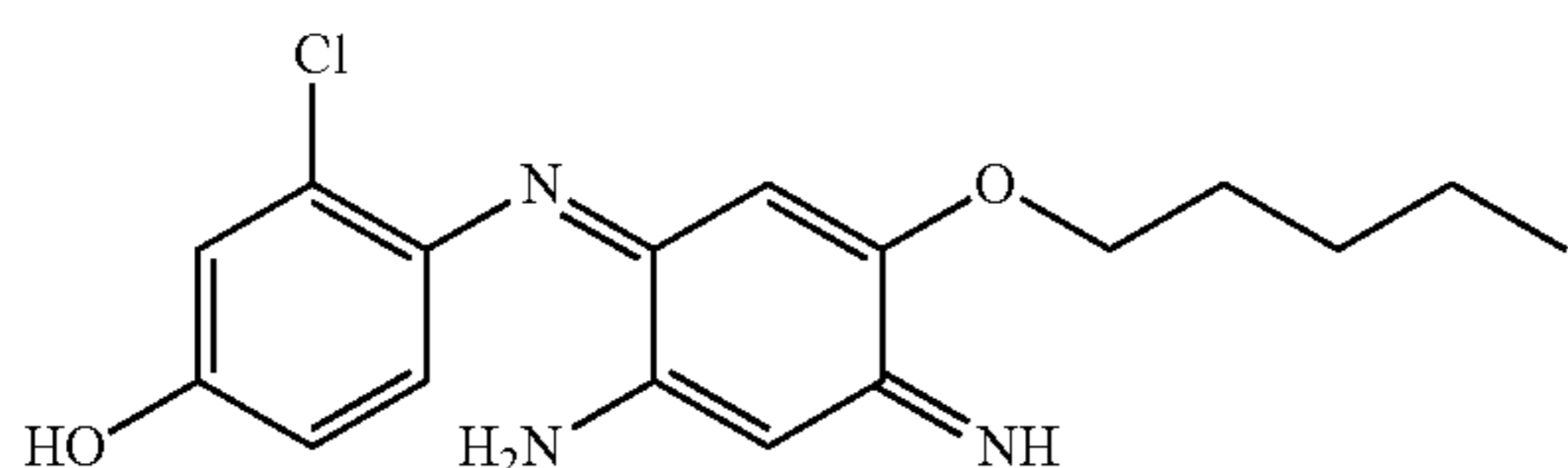
4-(2-Amino-5-pentyloxy-4-iminocyclohexa-2,5-dienylideneamino)-3-chlorophenol
