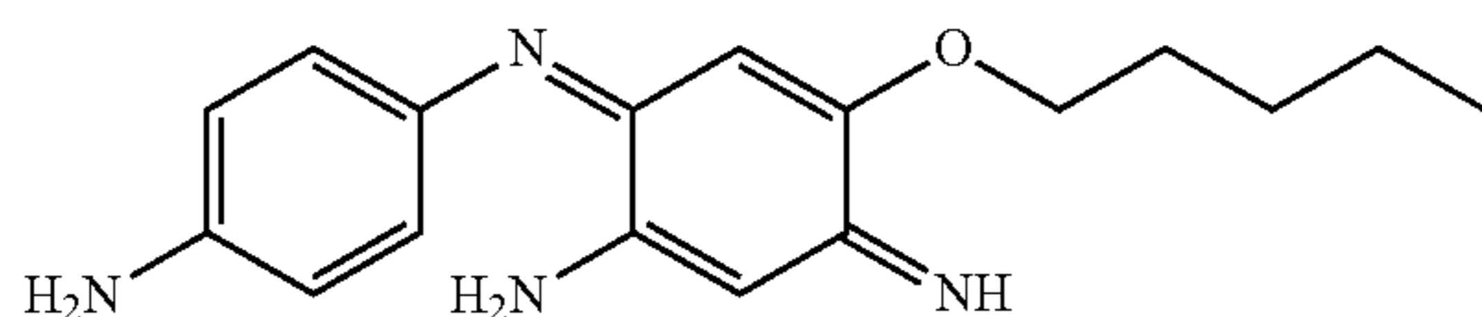
6-(4-Aminophenylimino)-4-pentyloxy-3-iminocyclohexa-1,4-dienylamine
