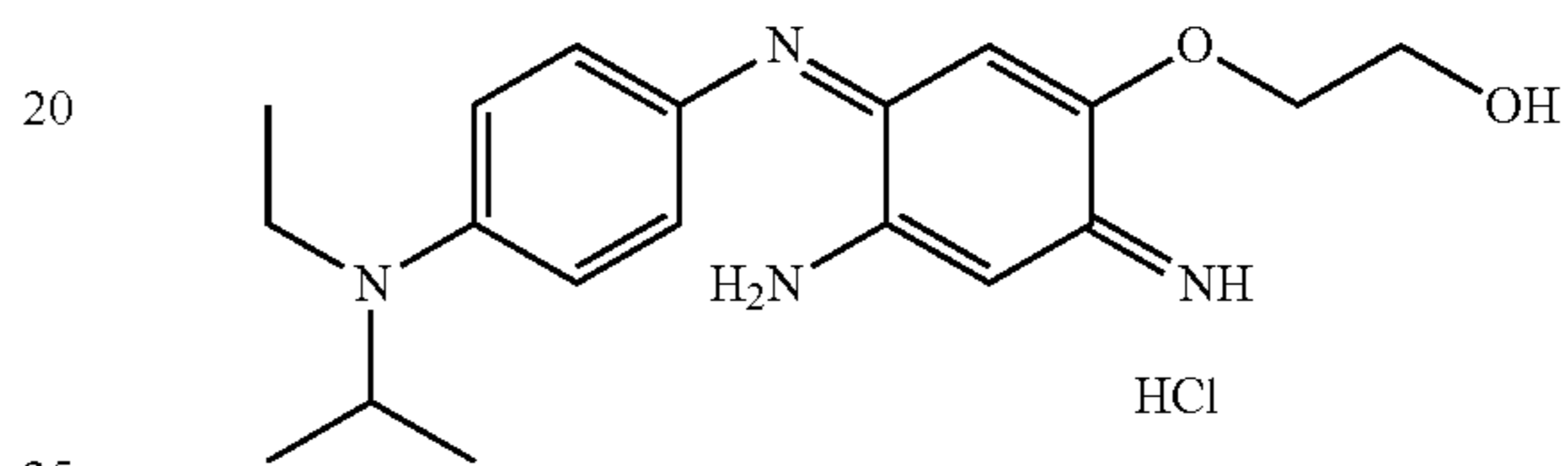
2-({4-amino-3-[4-(ethylisopropylamino)phenylimino]-6-iminocyclohexa-1,4-dienyloxy}ethanol
