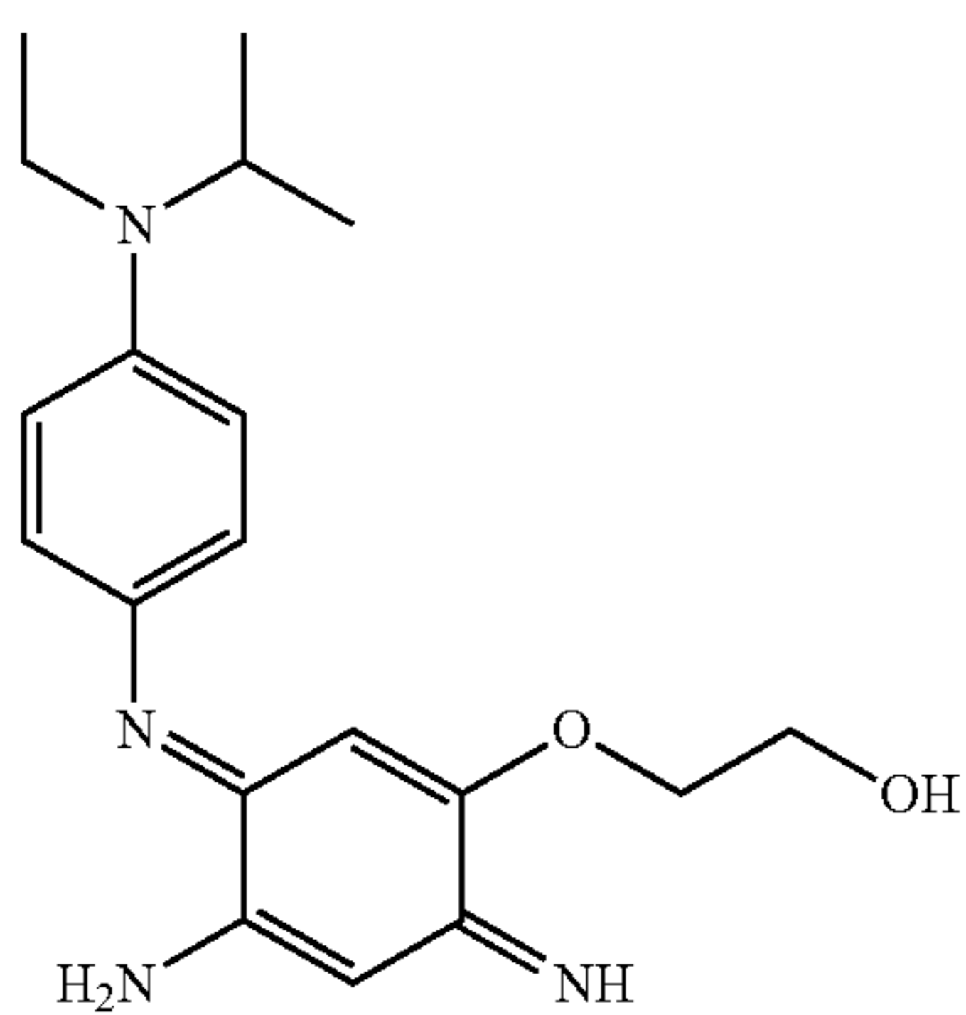
2-(4-Amino-3-[4-(ethylisopropylamino)phenylimino]-6-iminocyclohexa-1,4-dienyloxy)ethanol
