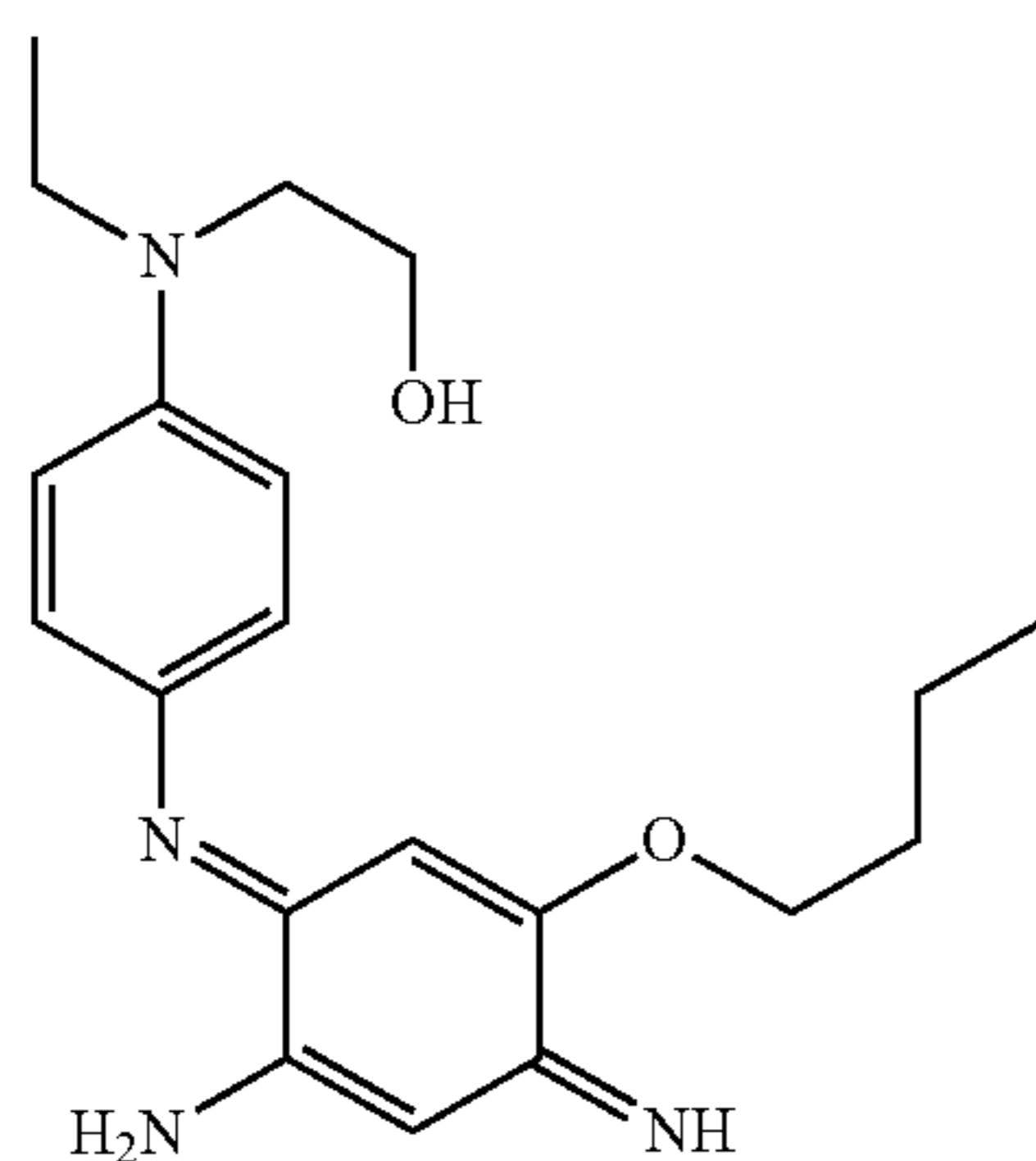
2-((4-[2-Amino-5-butoxy-4-iminocyclohexa-2,5-dienylideneamino]phenyl)ethylamino)ethanol
