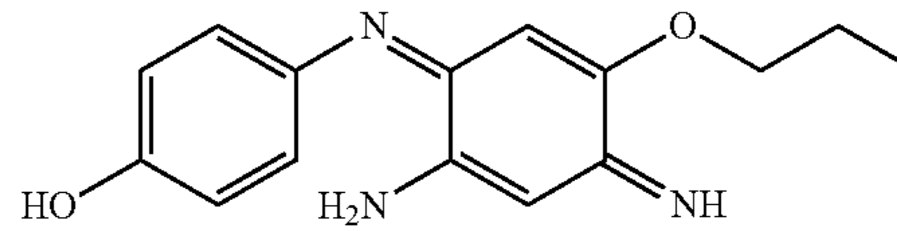
4-(2-Amino-5-butoxy-4-iminocyclohexa-2,5-dienylideneamino)phenol
