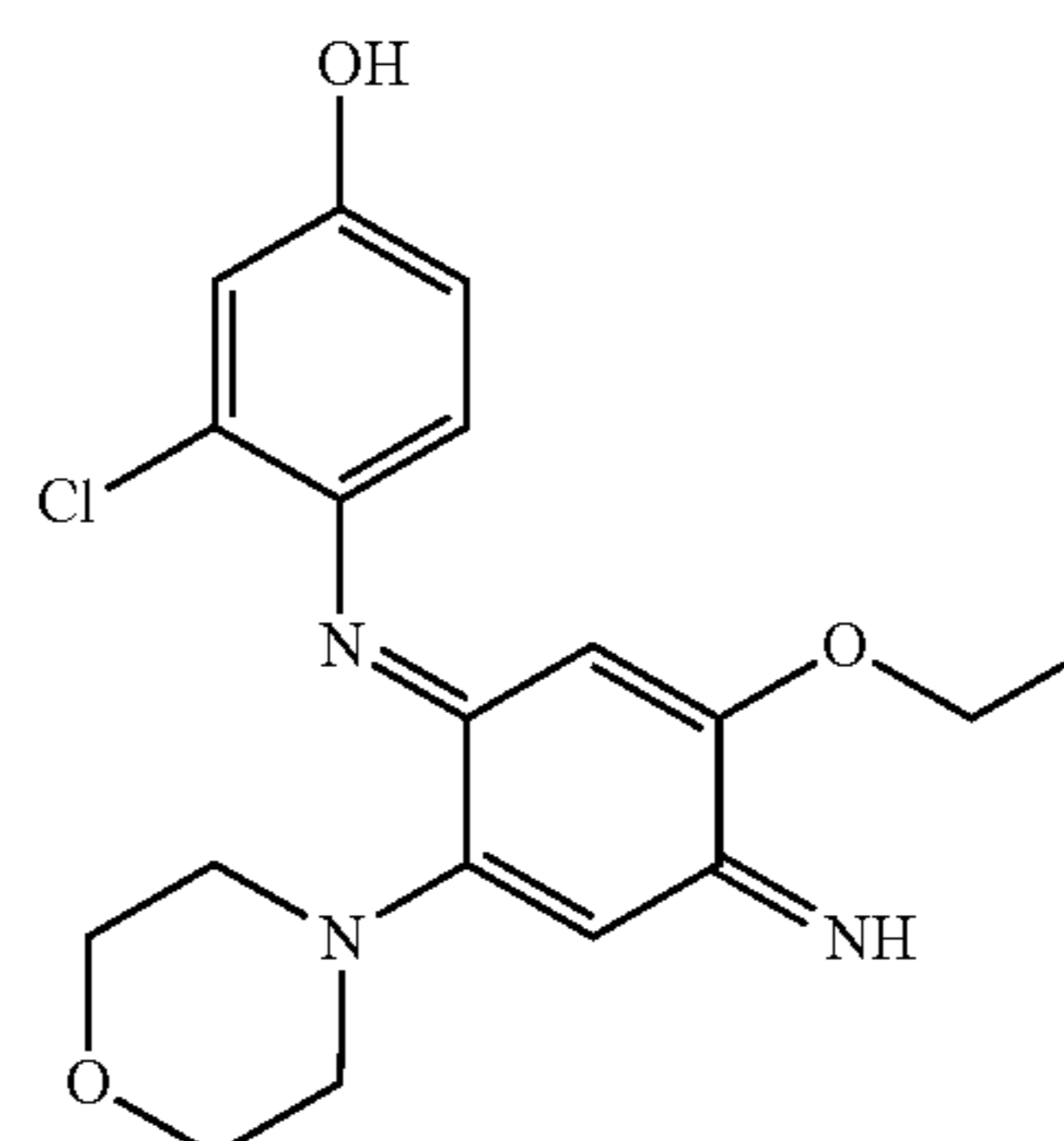
3-Chloro-4-(5-ethoxy-4-imino-2-morpholin-4-ylcyclohexa-2,5-dienylideneamino)phenol
