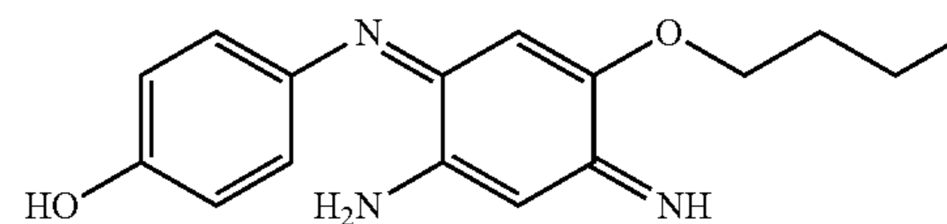
4-(2-Amino-5-butoxy-4-iminocyclohexa-2,5-dienylideneamino)phenol
