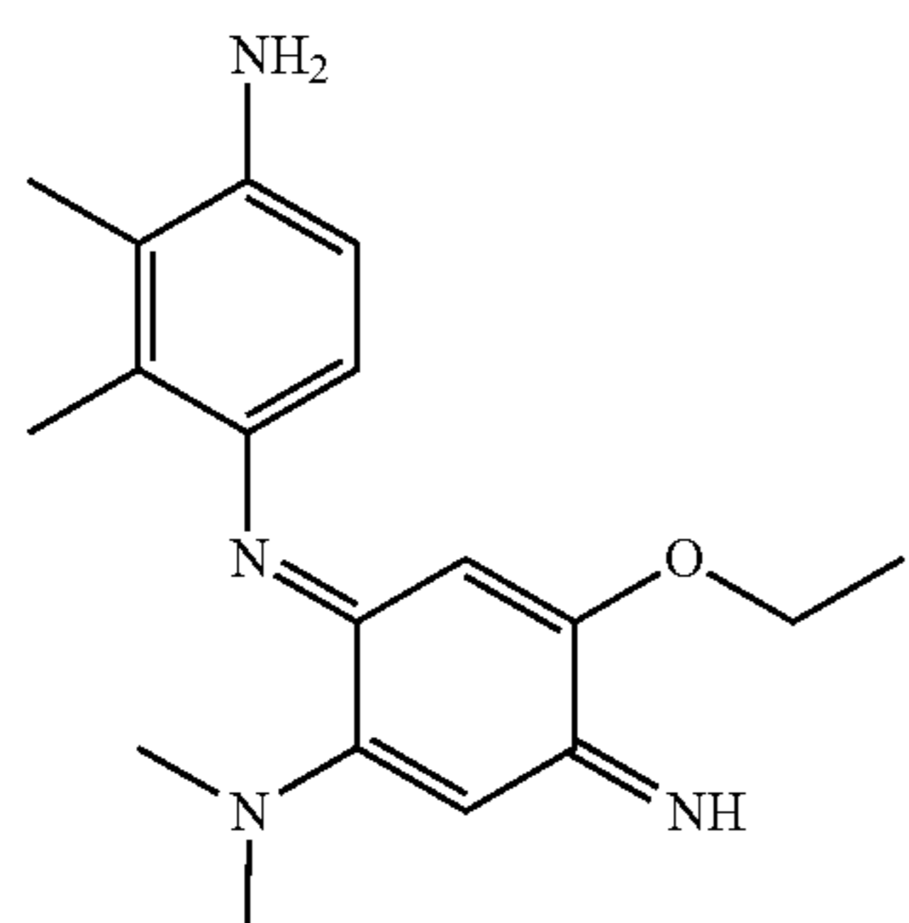
N-(2-Dimethylamino-5-ethoxy-4-imino cyclohexa-2,5-dienylidene)-2,3-dimethylbenzene-1,4-diamine
