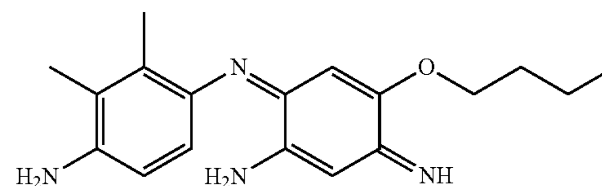
6-(4-Amino-2,3-dimethylphenylimino)-4-butoxy-3-iminocyclohexa-1,4-dienylamine
