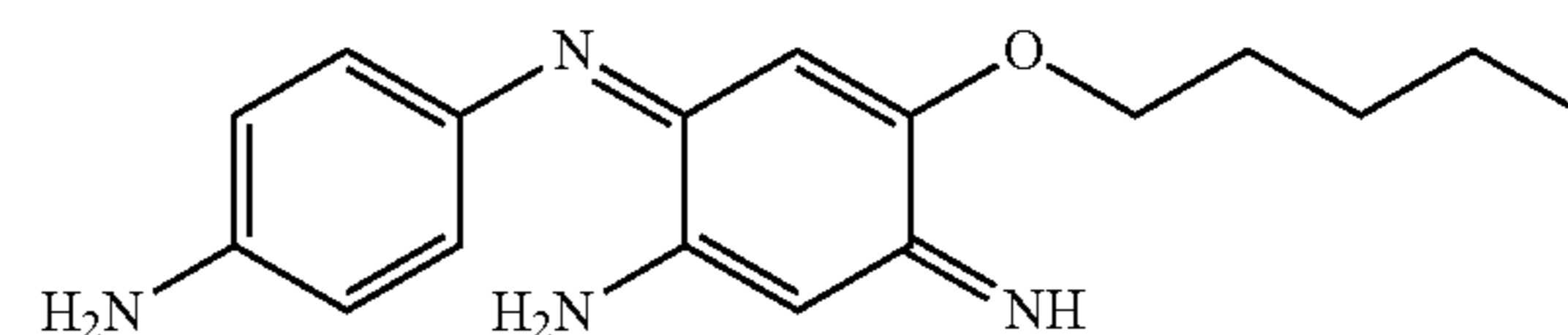
6-(4-Aminophenylimino)-4-pentyloxy-3-aminocyclohexa-1,4-dienylamine
