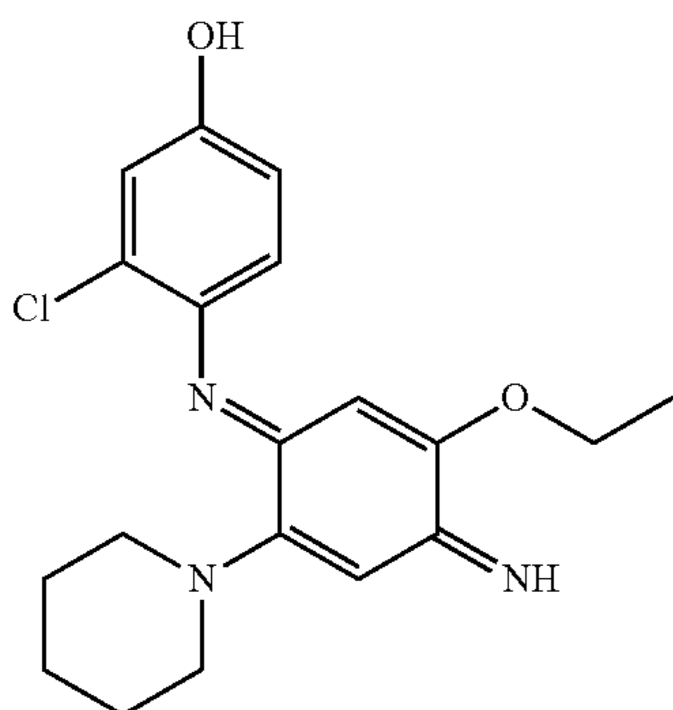
3-Chloro-4-(5-ethoxy-4-imino-2-piperidin-1-ylcyclohexa-2,5-dienylideneamino)phenol
