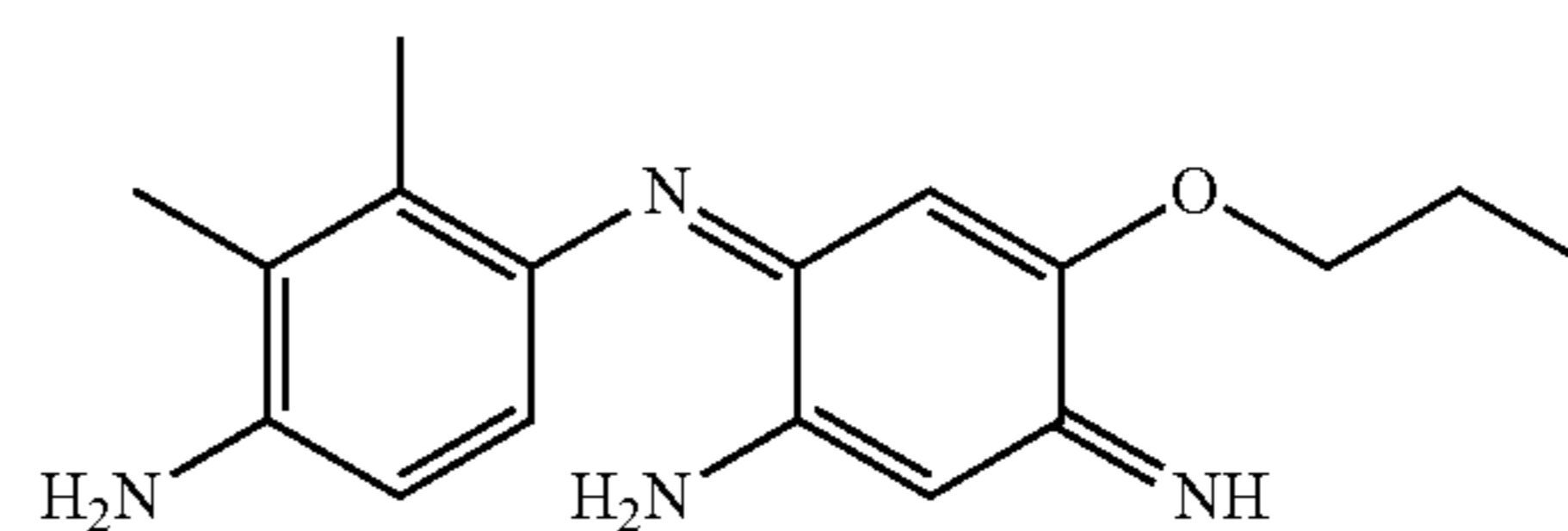
6-(2-Amino-2,3-dimethylphenylimino)-4-propoxy-3-iminocyclohexa-1,4-dienylamine
