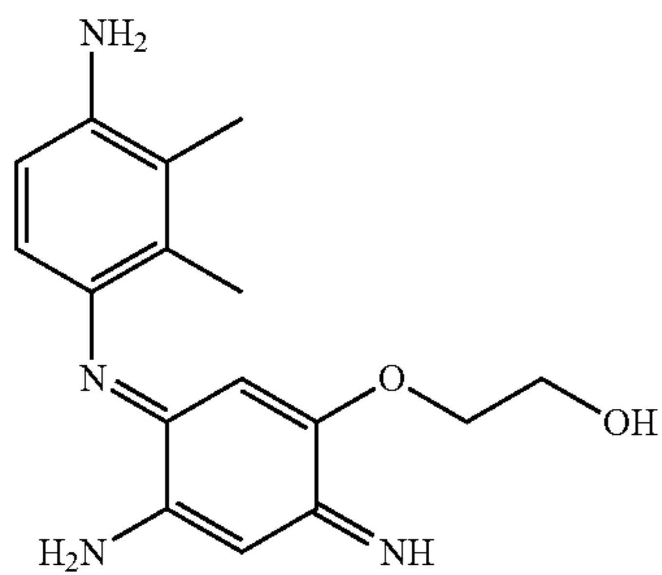
2-(4-Amino-3-[4-amino-2,3-dimethylphenylimino]-6-iminocyclohexa-1,4-dienyloxy)ethanol
