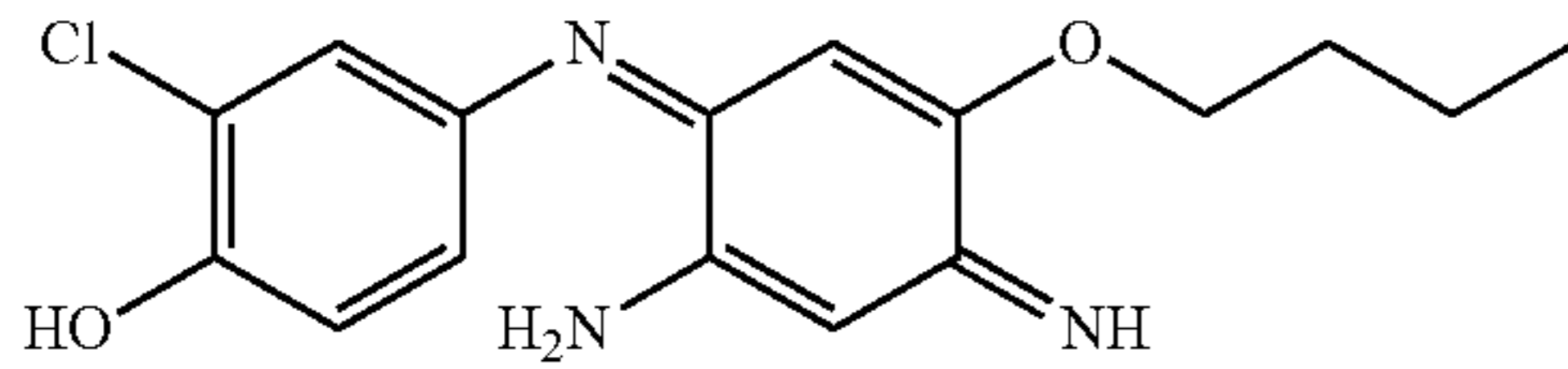
4-(2-Amino-5-butoxy-4-iminocyclohexa-2,5-dienylideneamino)-2-chlorophenol
