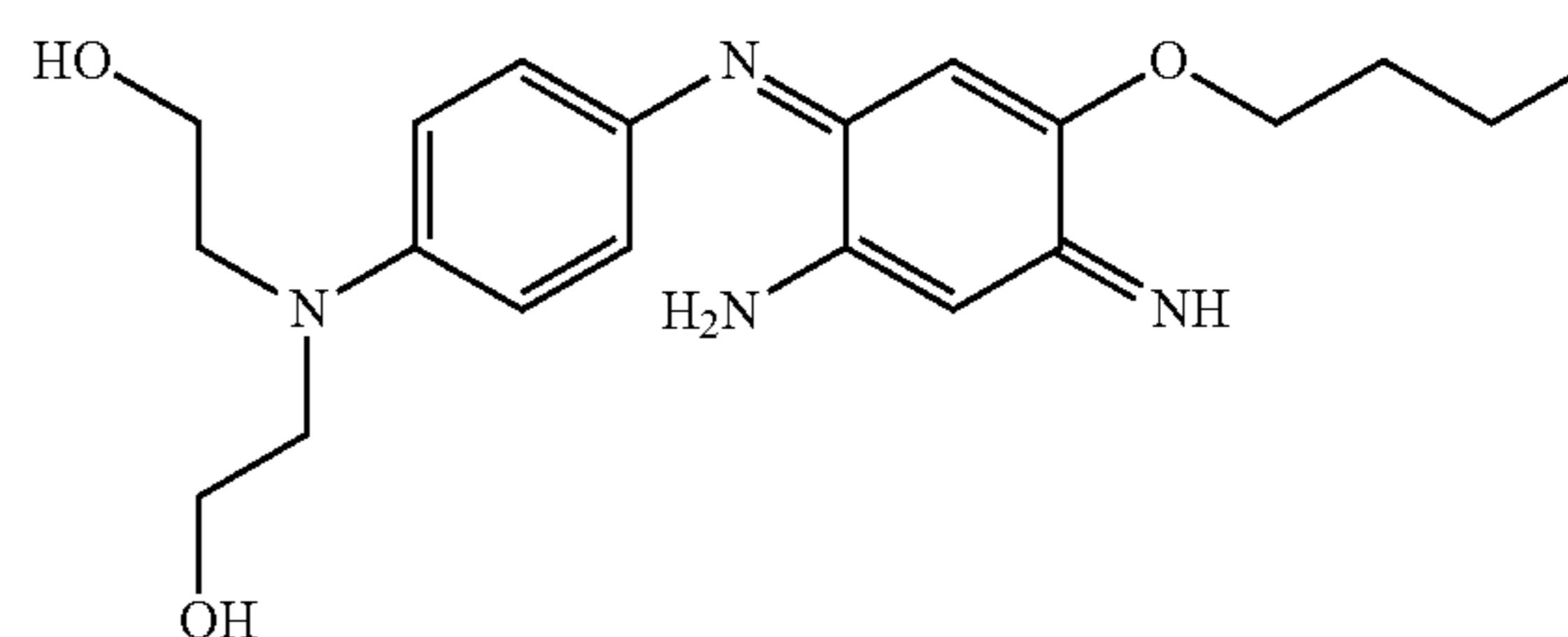
2-[[4-(2-Amino-5-butoxy-4-iminocyclohexa-2,5-dienylideneamino)phenyl](2-hydroxyethyl)amino]ethanol
