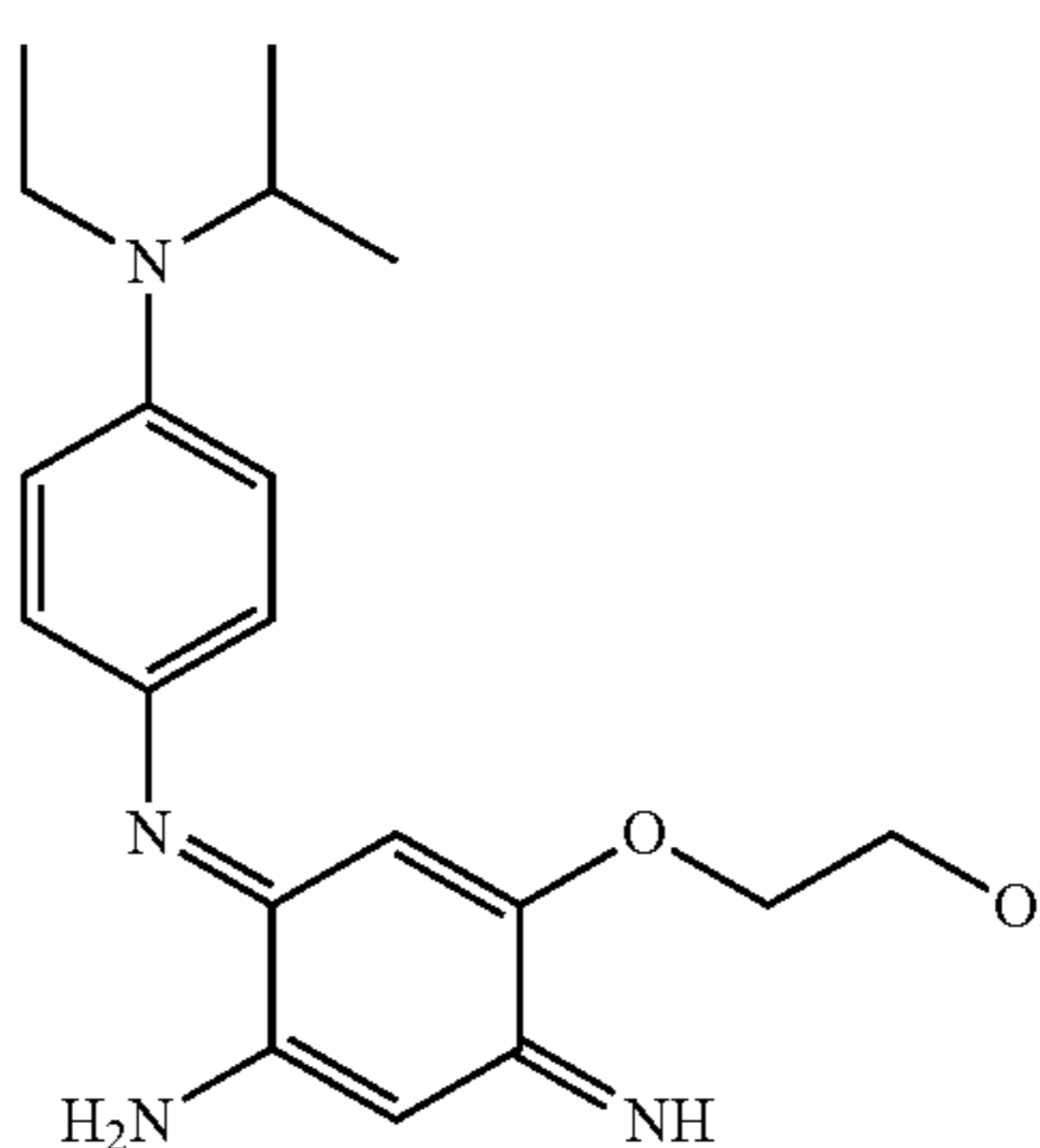
2-{4-Amino-3-[4-(ethylisopropylamino)phenylimino]-6-iminocyclohexa-1,4-dienyloxy}ethanol
