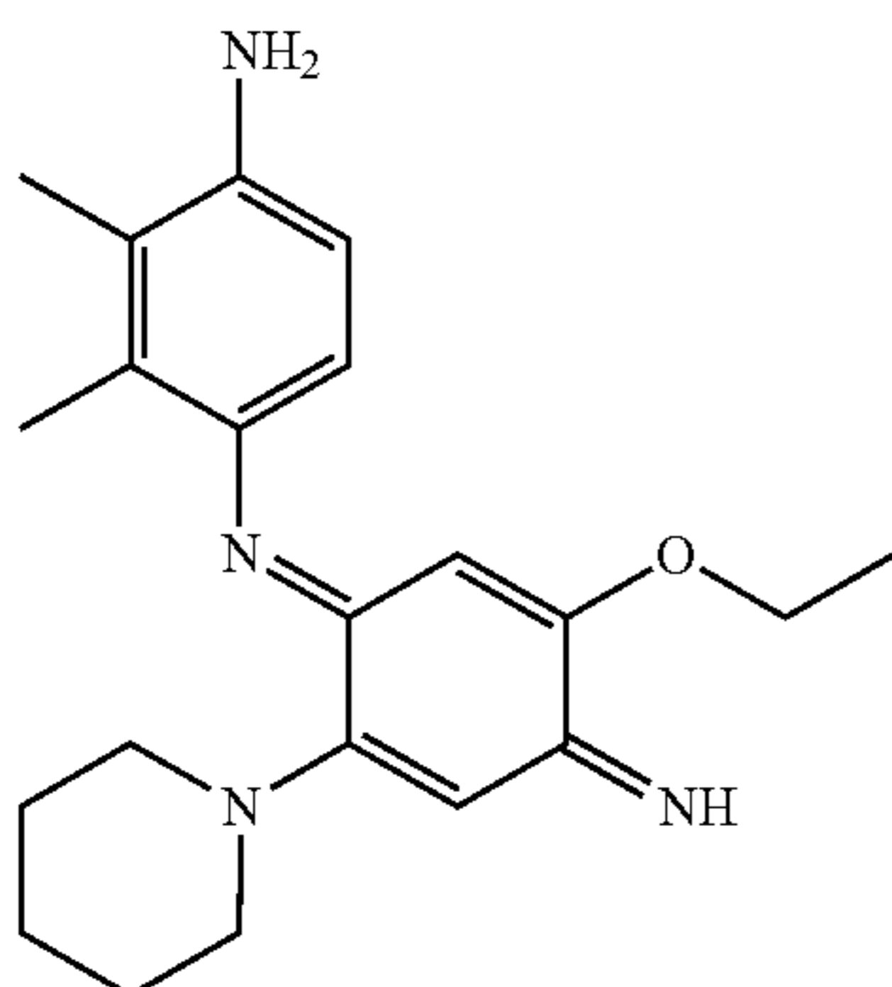
N-(5-Ethoxy-4-imino-2-piperidin-1-ylcyclohexa-2,5-dienylidene)-2,3-dimethylbenzene-1,4-diamine
