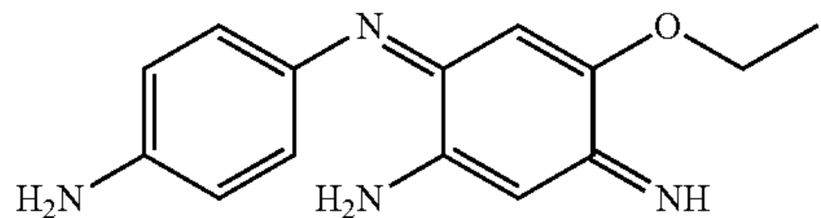
6-(4-Aminophenylimino)-4-ethoxy-3-iminocyclohexa-1,4-dienylamine
