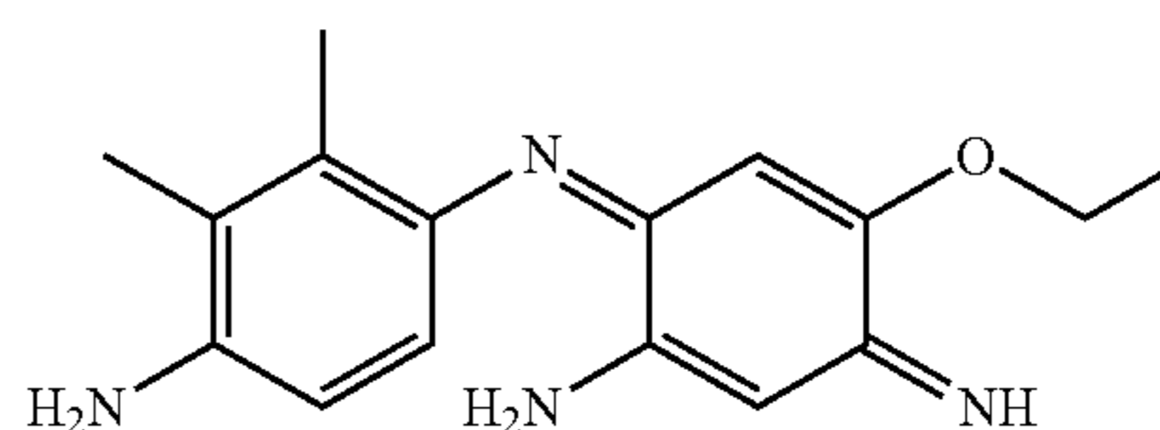
6-(4-Amino-2,3-dimethylphenylimino)-4-ethoxy-3-iminocyclohexa-1,4-dienylamine
