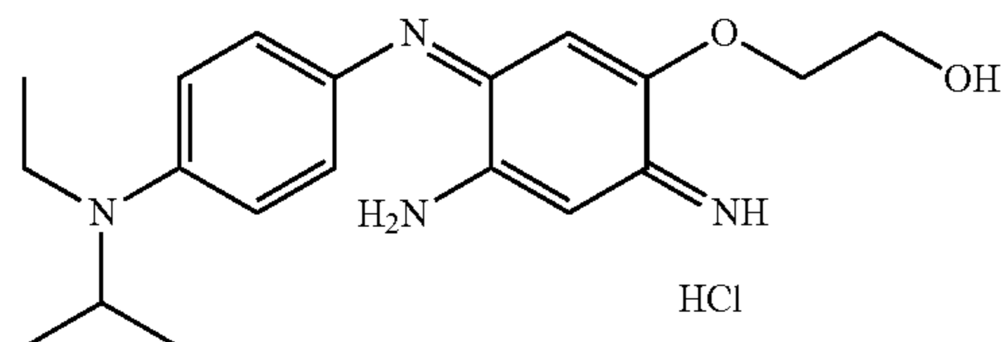
2-(4-amino-3-[4-(ethylisopropylamino)phenylimino]-6-iminocyclohexa-1,4-dienyloxy)ethanol
