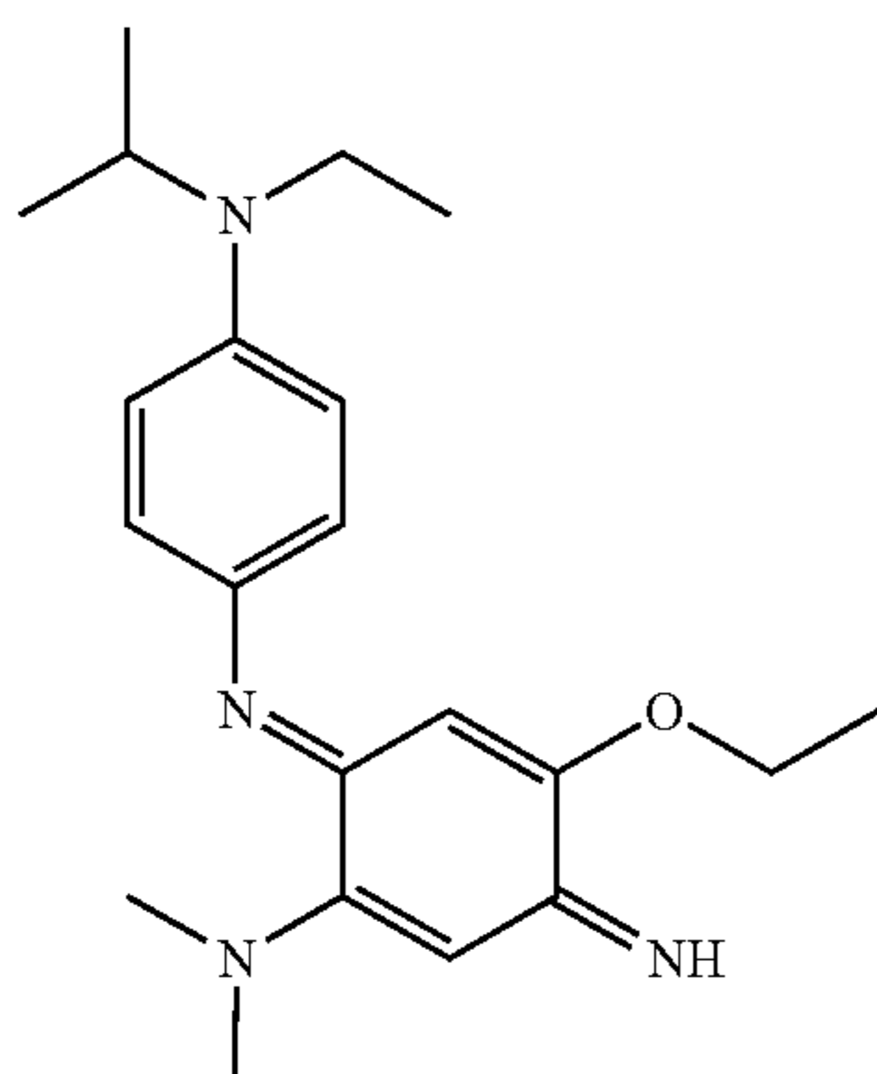
N-(2-methylamino-5-ethoxy-4-iminocyclohexa-2,5-dienylidene)-N'-ethyl-N'-isopropylbenzene-1,4-diamine
