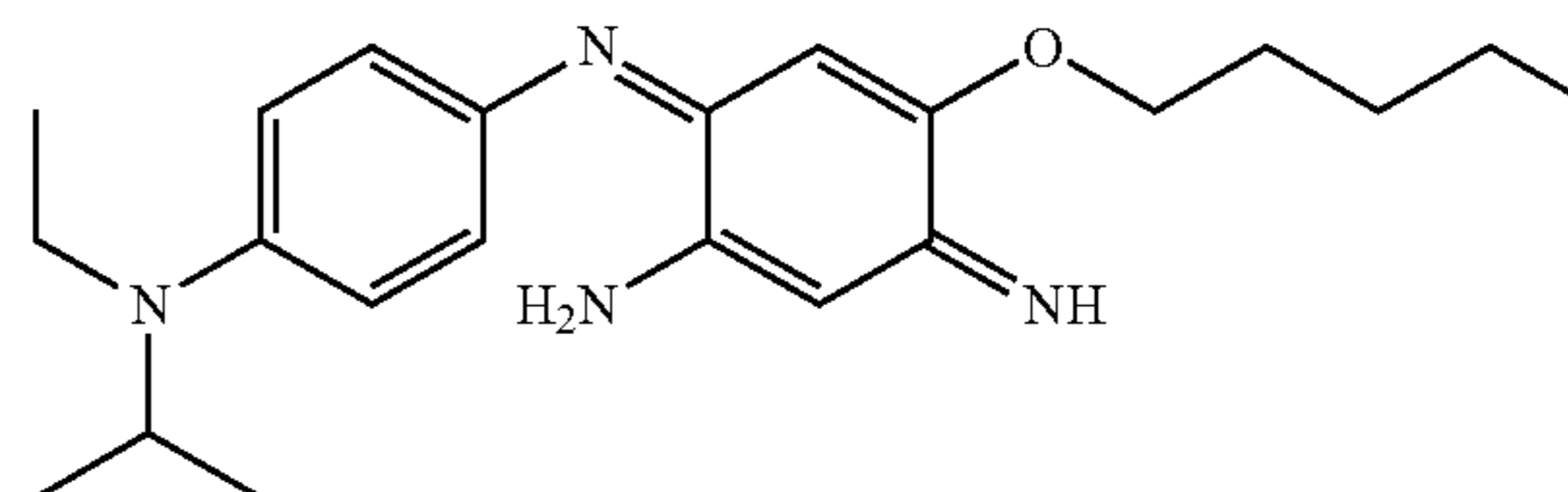
4-pentyloxy-6-[4-(ethylisopropylamino)phenylimino]-3-aminocyclohexa-1,4-dienylamine
