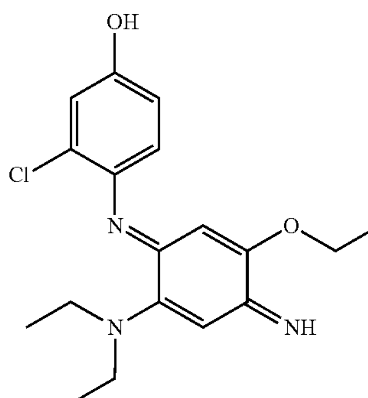
3-Chloro-4-(2-diethylamino-5-ethoxy-4-iminocyclohexa-2,5-dienylideneamino)phenol
