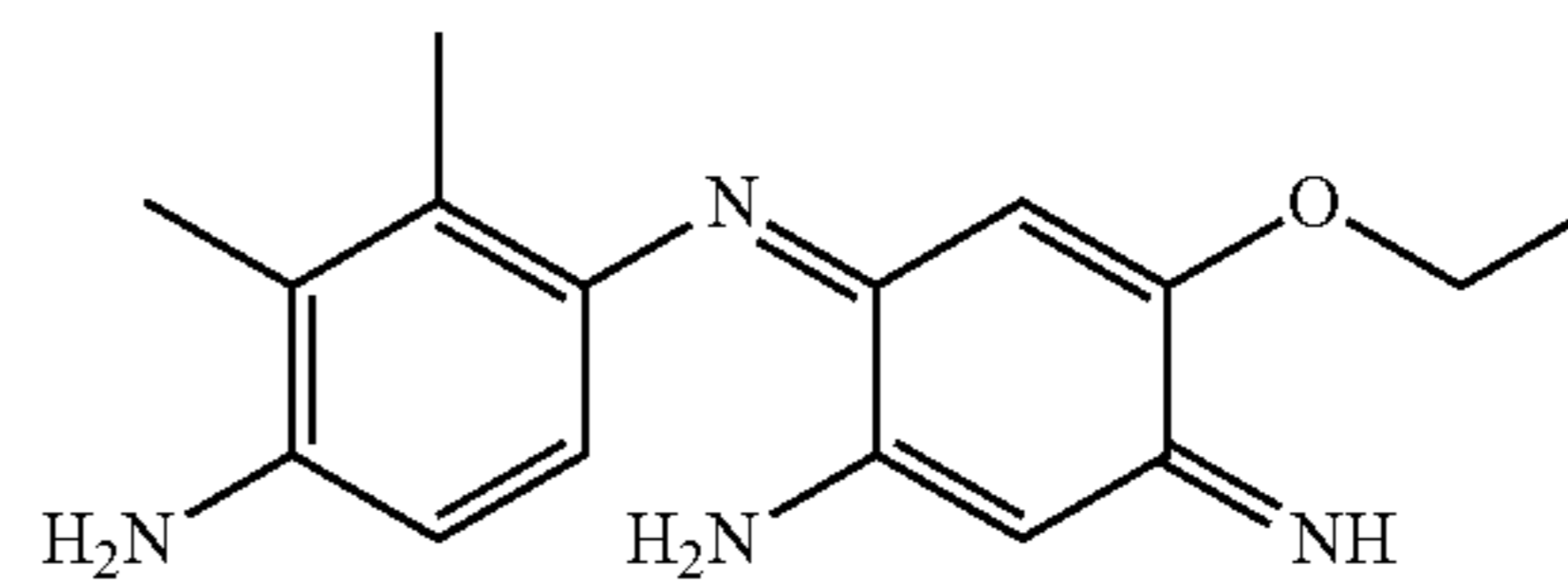
6-(4-Amino-2,3-dimethylphenylimino)-4-ethoxy-3-iminocyclohexa-1,4-dienylamine
