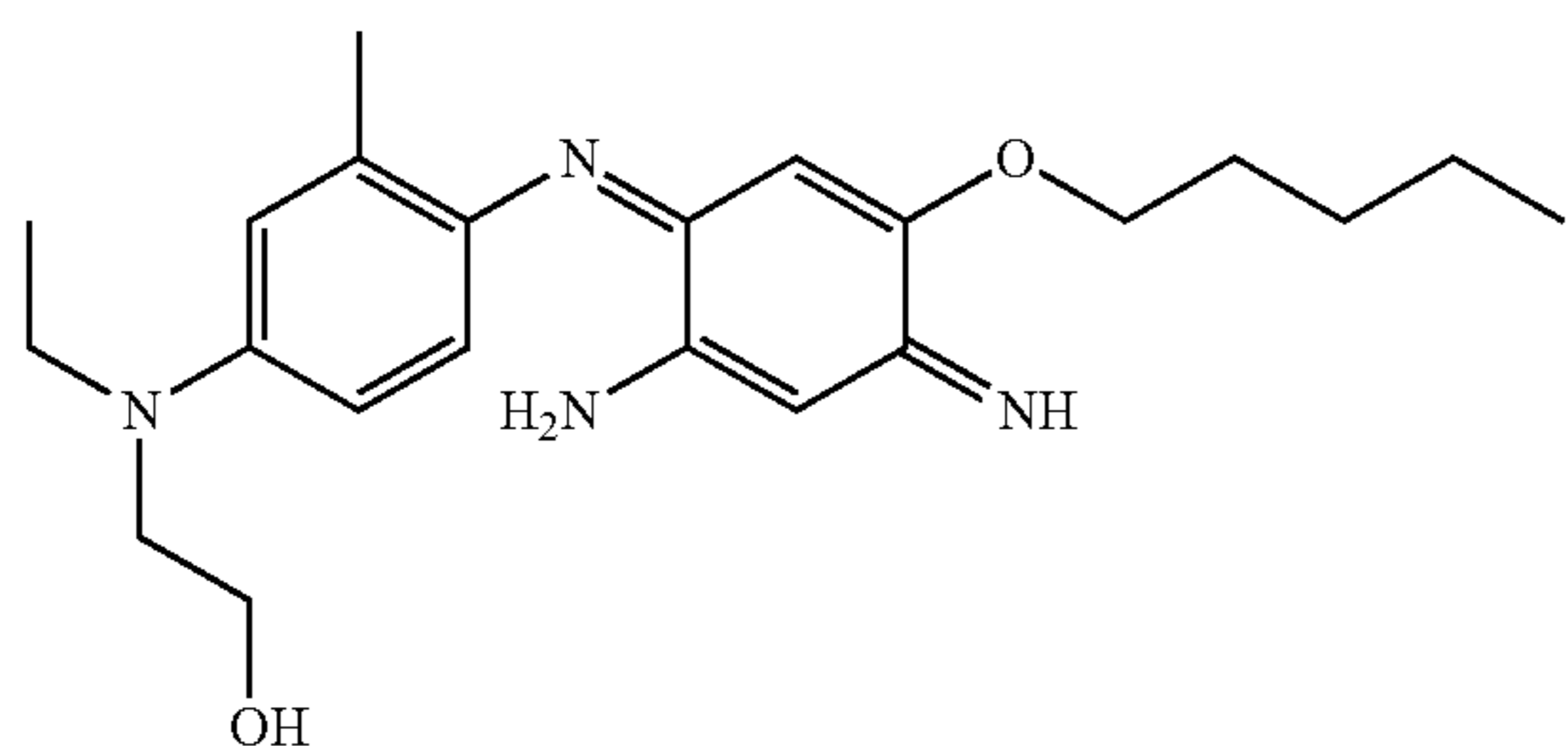
2-{[4-(2-Amino-5-pentyloxy-4-iminocyclohexa-2,5-dienylideneamino)-3-methylphenyl]ethylamino}ethanol
