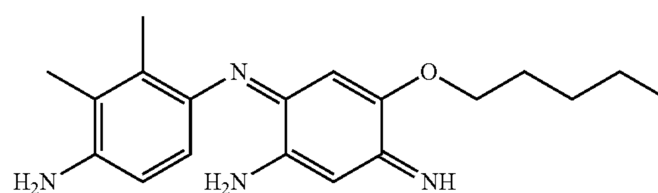
6-(4-Amino-2,3-dimethylphenylimino)-4-hexyloxy-3-iminocyclohexa-1,4-dienylamine
