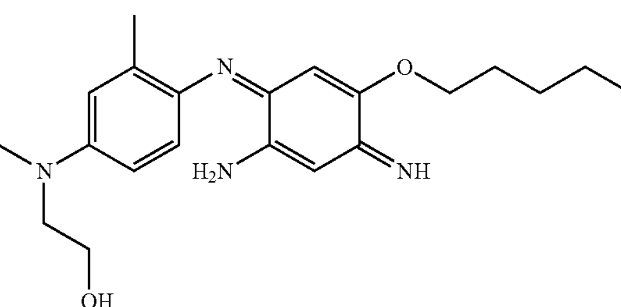
2-[[4-(2-Amino-5-pentyloxy-4-iminocyclohexa-2,5-dienylideneamino)-3-methylphenyl]ethylamino]ethanol
