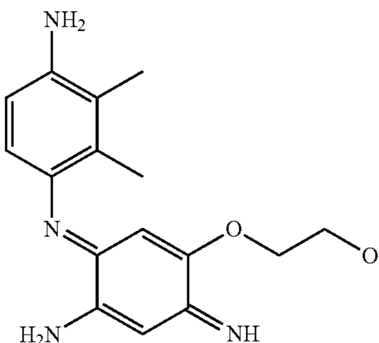
2-(4-Amino-3-[4-amino-2,3-dimethylphenylimino]-6-iminocyclohexa-1,4-dienyloxy)ethanol
