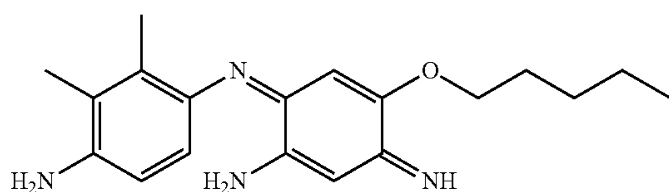
6-(4-Amino-2,3-dimethylphenylimino)-4-pentyloxy-3-iminocyclohexa-1,4-dienylamine
