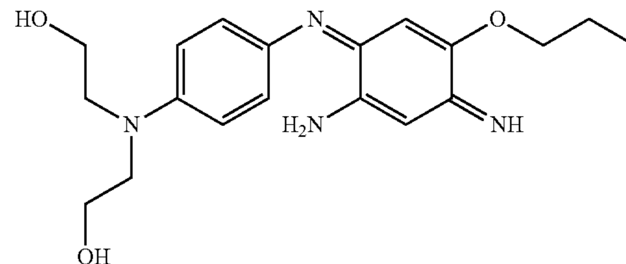
2-[[4-(2-Amino-5-propoxy-4-iminocyclohexa-2,5-dienylideneamino)phenyl](2-hydroxyethyl)amino]ethanol
