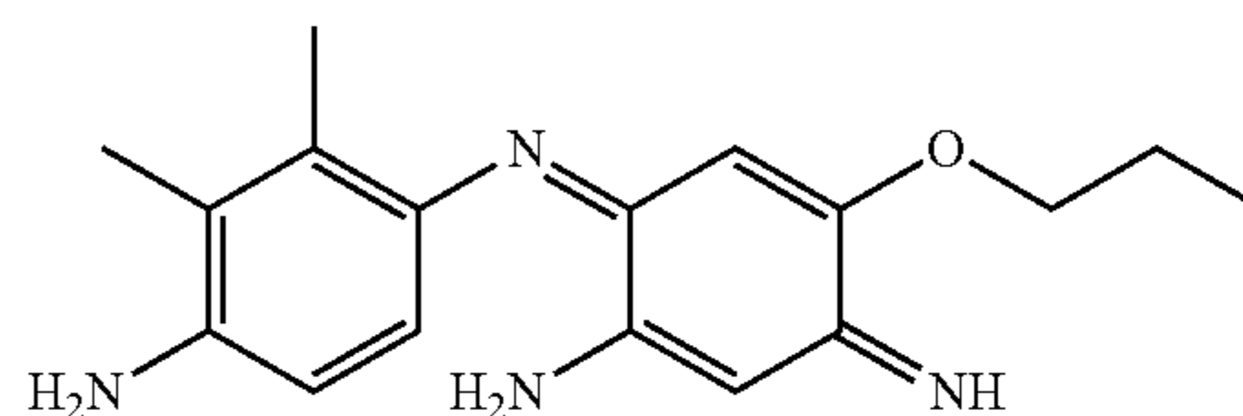
6-(2-Amino-2,3-dimethylphenylimino)-4-propoxy-3-iminocyclohexa-1,4-dienylamine
