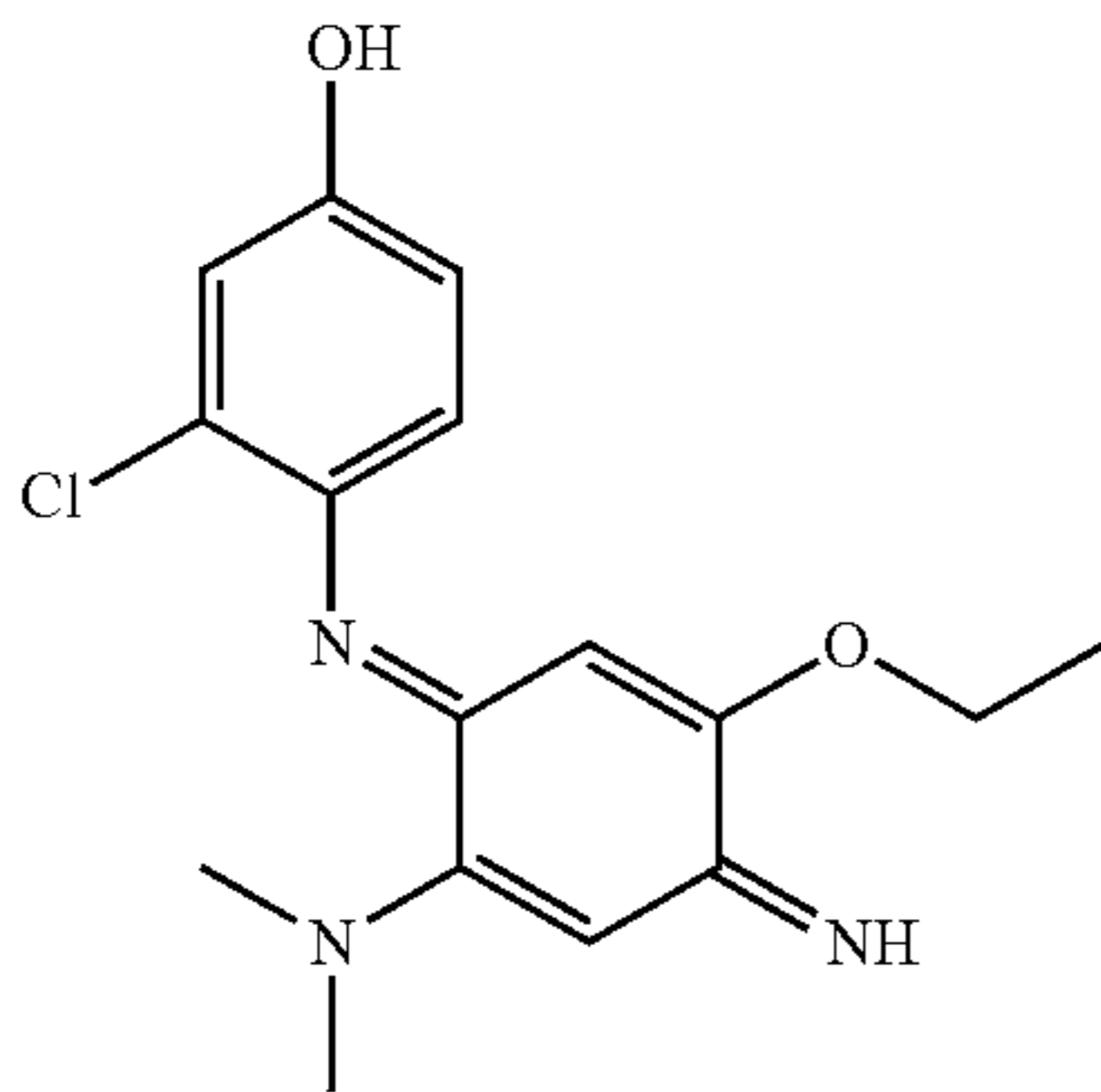
3-Chloro-4-(2-diethylamino-5-ethoxy-4-iminocyclohexa-2,5-dienylideneamino)phenol
