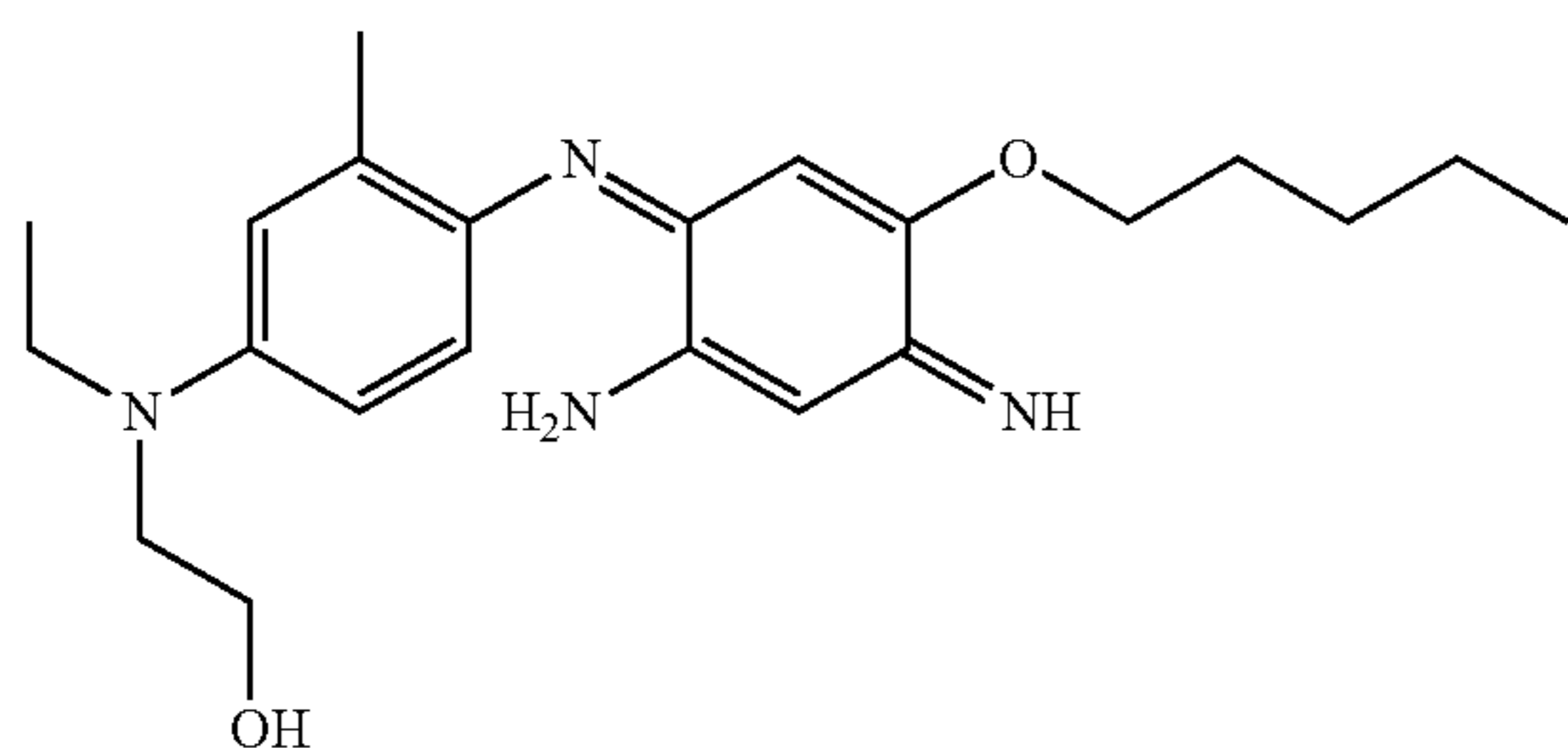
2-{[4-(2-Amino-5-pentyloxy-4-iminocyclohexa-2,5-dienylideneamino)-3-methylphenyl]ethylamino}ethanol
