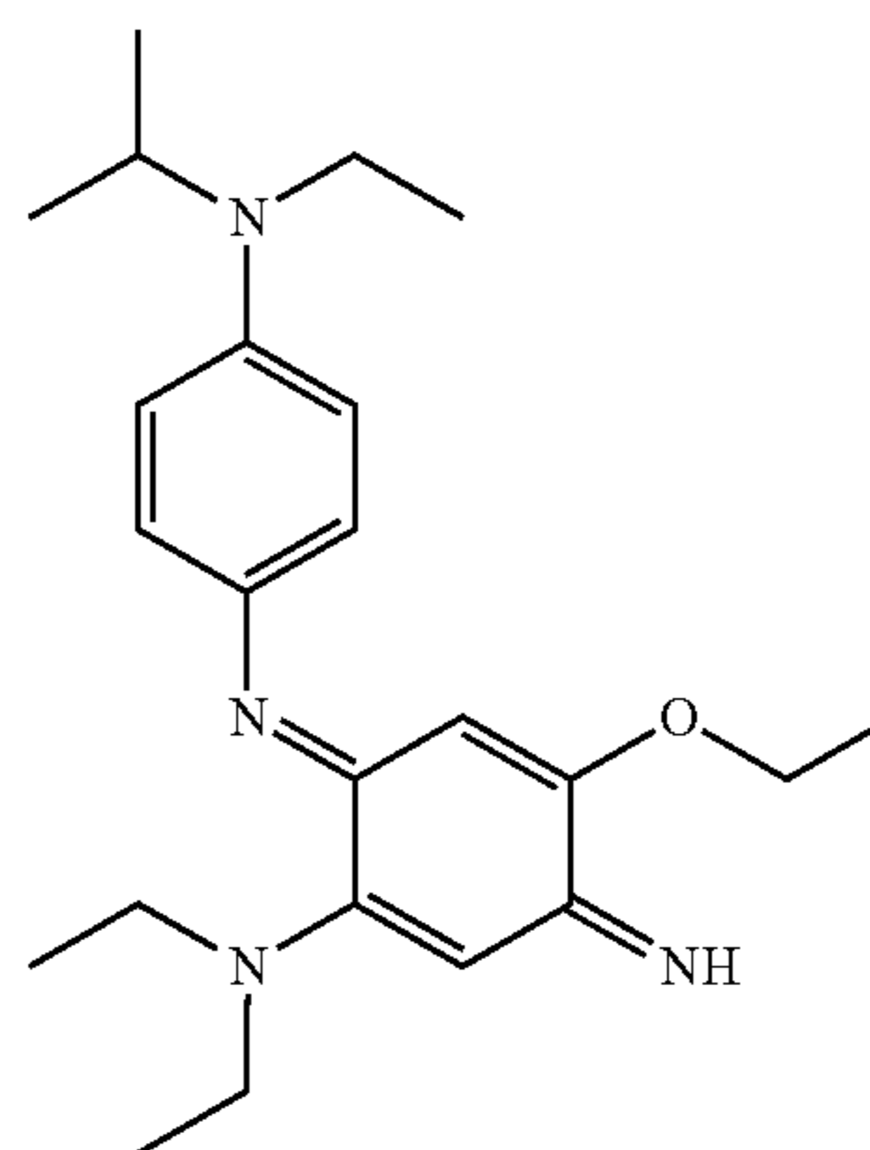
N-(2-Diethylamino-5-ethoxy-4-iminocyclohexa-2,5-dienylidene)-N'-ethyl-N'-isopropylbenzene-1,4-diamine
