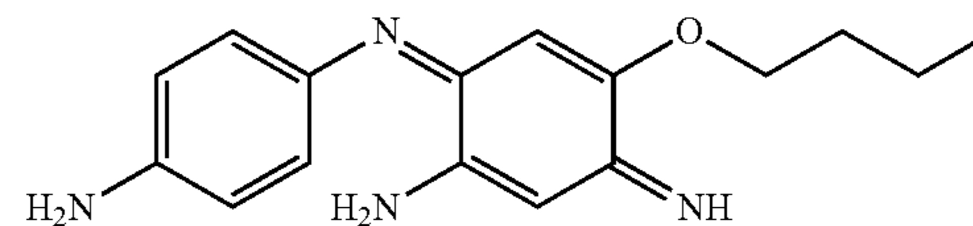
6-(4-Aminophenylimino)-4-butoxy-3-iminocyclohexa-1,4-dienylamine
