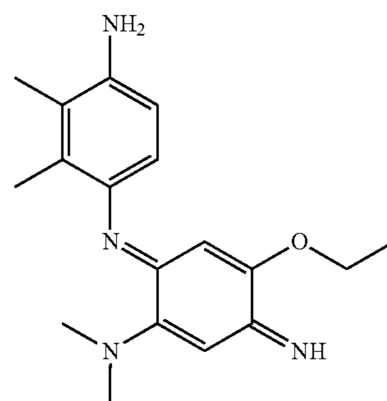
N-(2-Dimethylamino-5-ethoxy-4-iminocyclohexa-2,5-dienylidene)-2,3-dimethylbenzene-1,4-diamine
