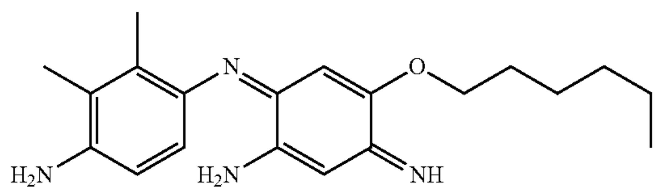
6-(4-Amino-2,3-dimethylphenylimino)-4-hexyloxy-3-iminocyclohexa-1,4-dienylamine
