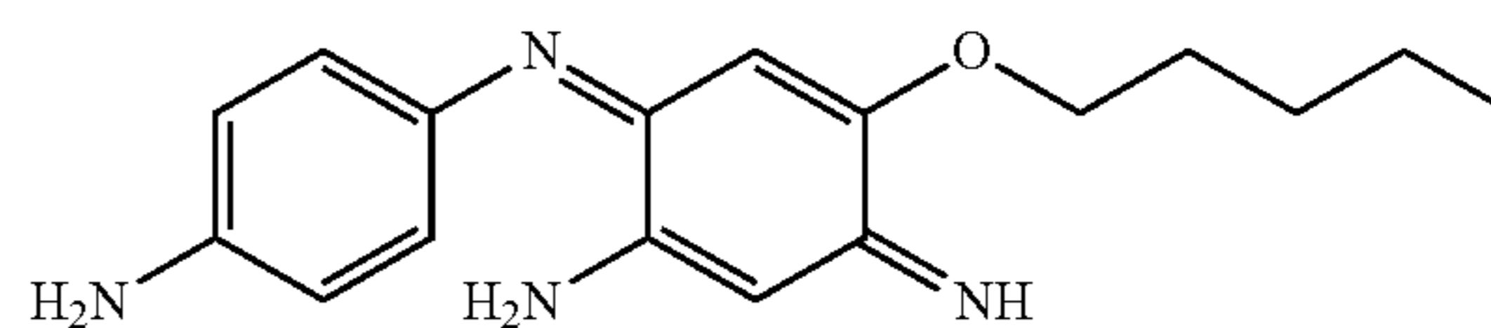
6-(4-Aminophenylimino)-4-hexyloxy-3-iminocyclohexa-1,4-dienylamine
