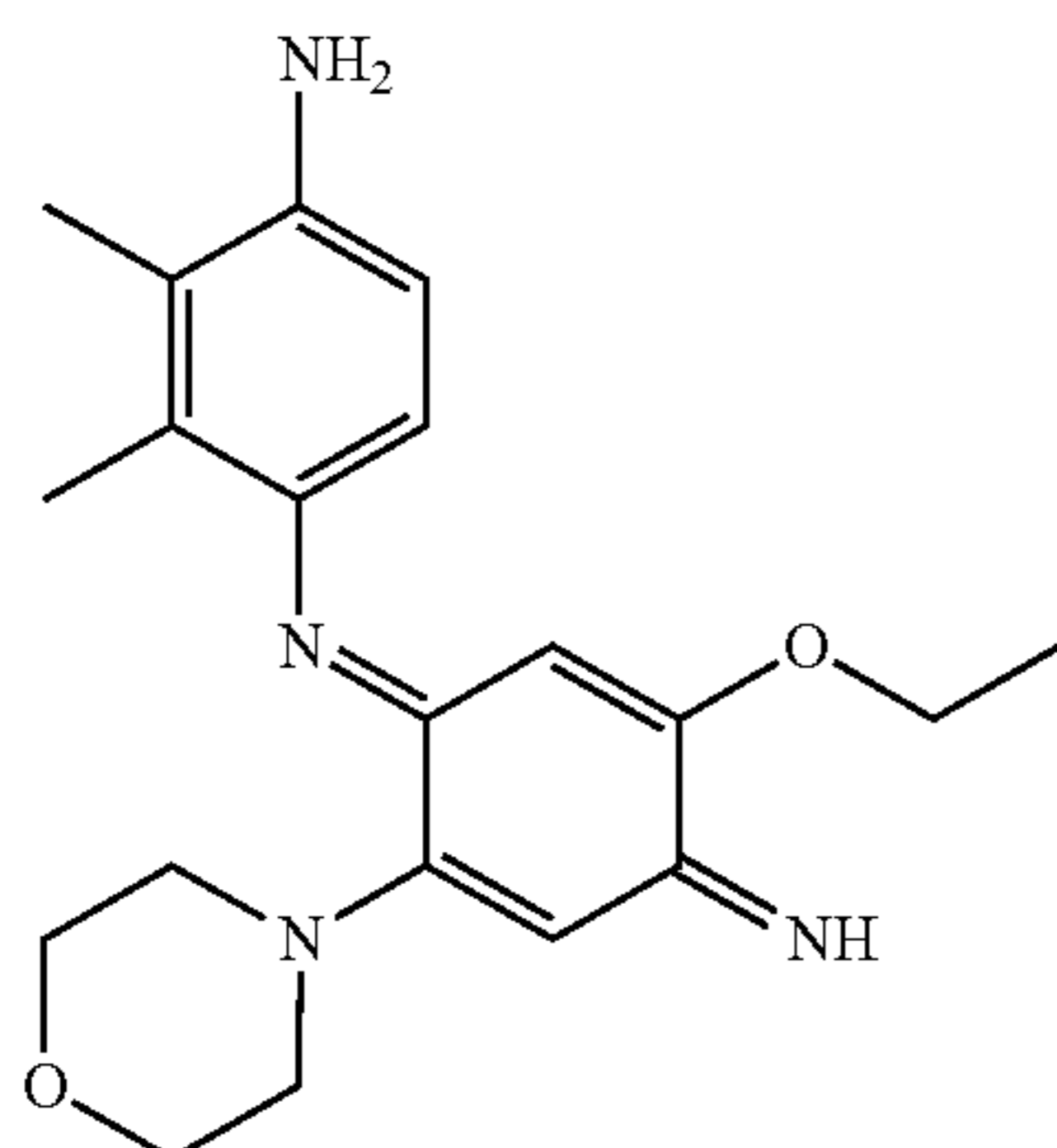
N-(5-Ethoxy-4-imino-2-morpholin-4-ylcyclohexa-2,5-dienylidene)-2,3-dimethylbenzene-1,4-diamine
