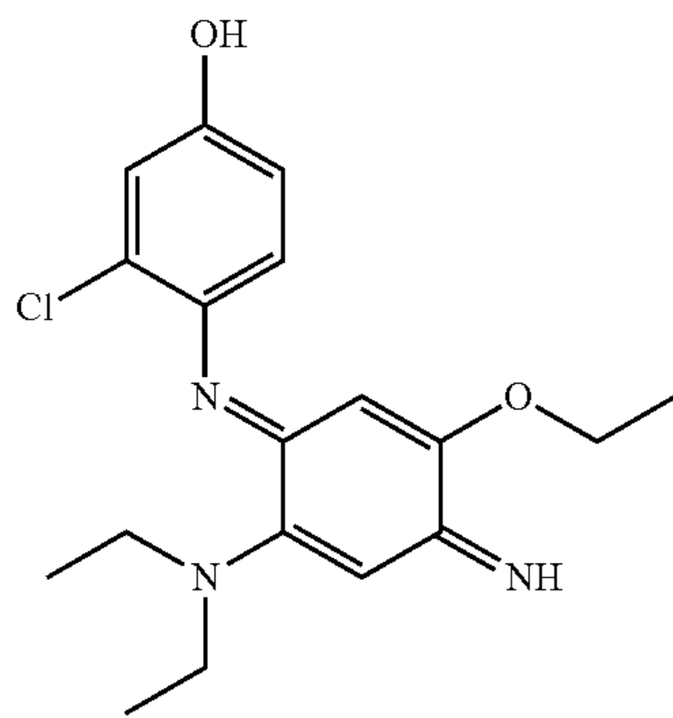
3-Chloro-4-(2-diethylamino-5-ethoxy-4-iminocyclohexa-2,5-dienylideneamino)phenol
