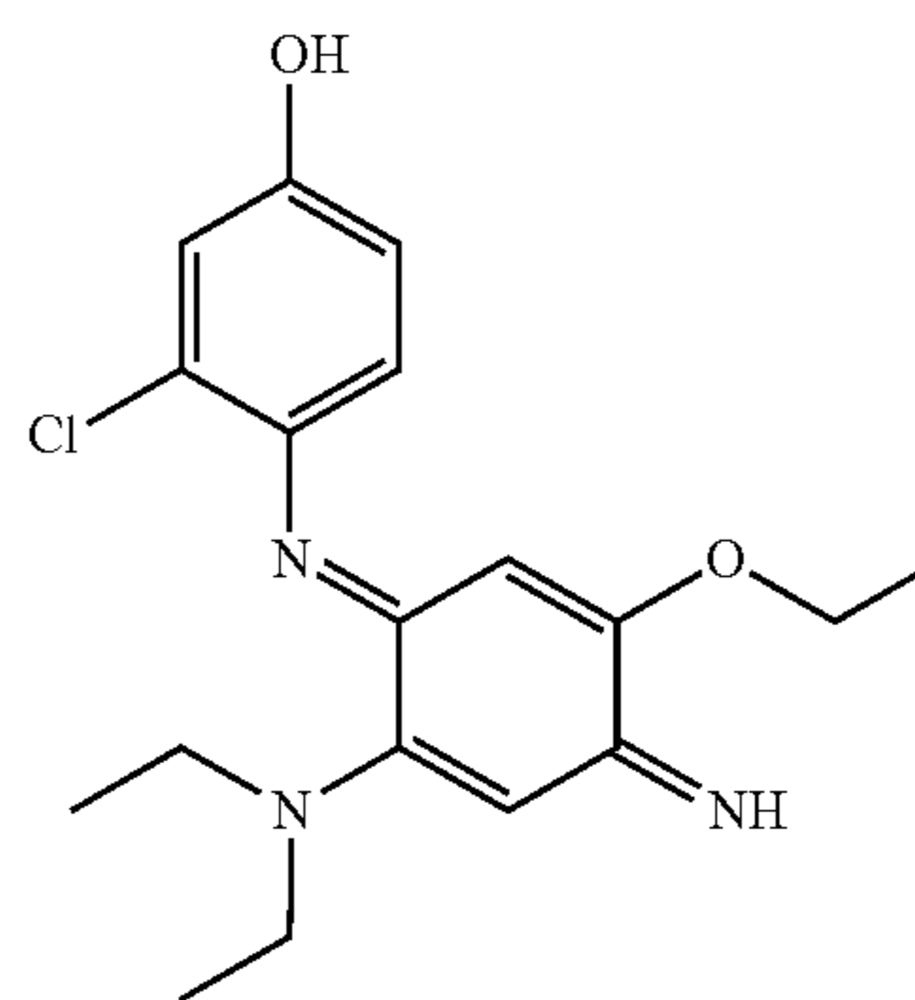
3-Chloro-4-(2-diethylamino-5-ethoxy-4-iminocyclohexa-2,5-dienylideneamino)phenol
