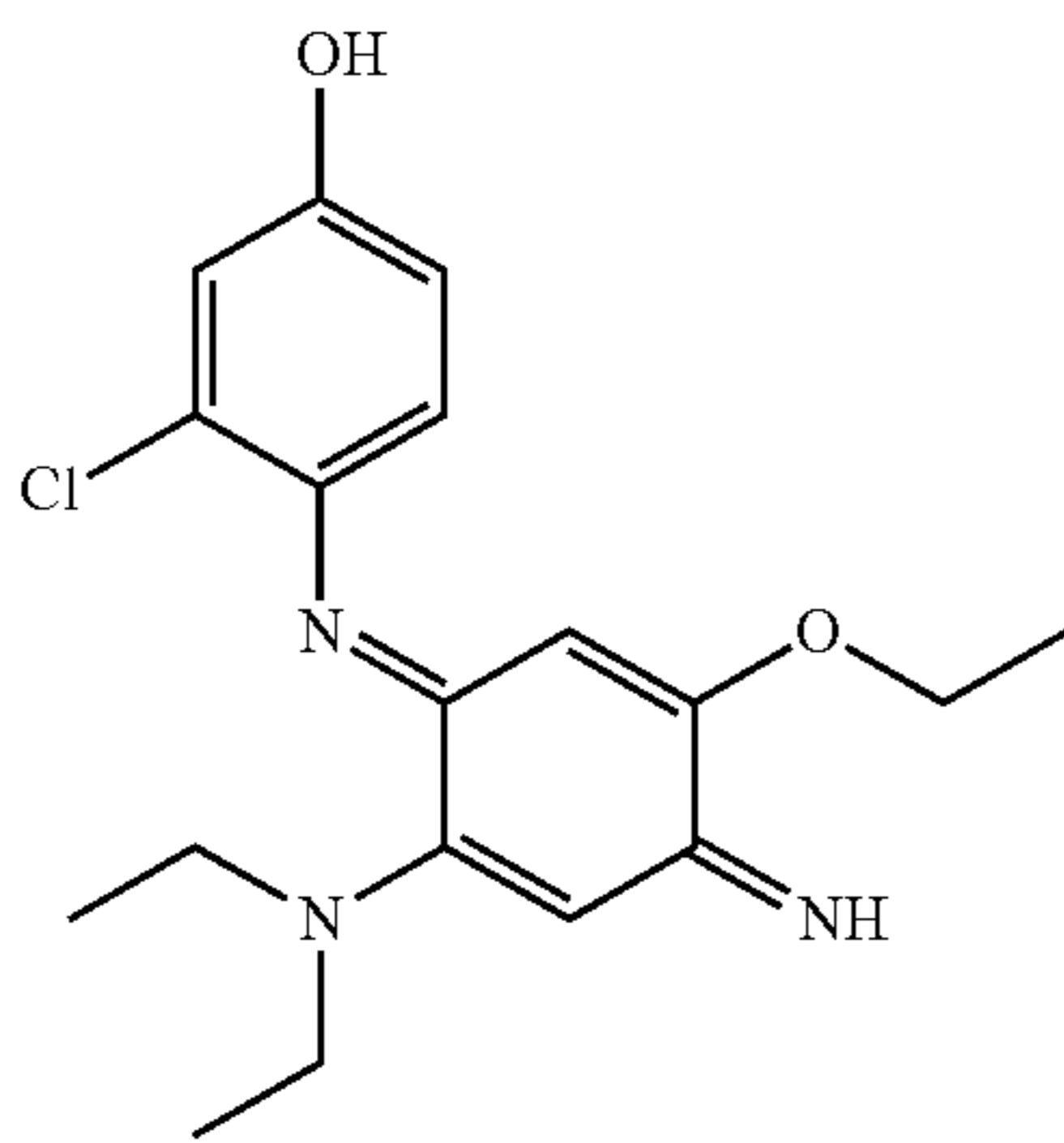
3-Chloro-4-(2-diethylamino-5-ethoxy-4-iminocyclohexa-2,5-dienylideneamino)phenol
