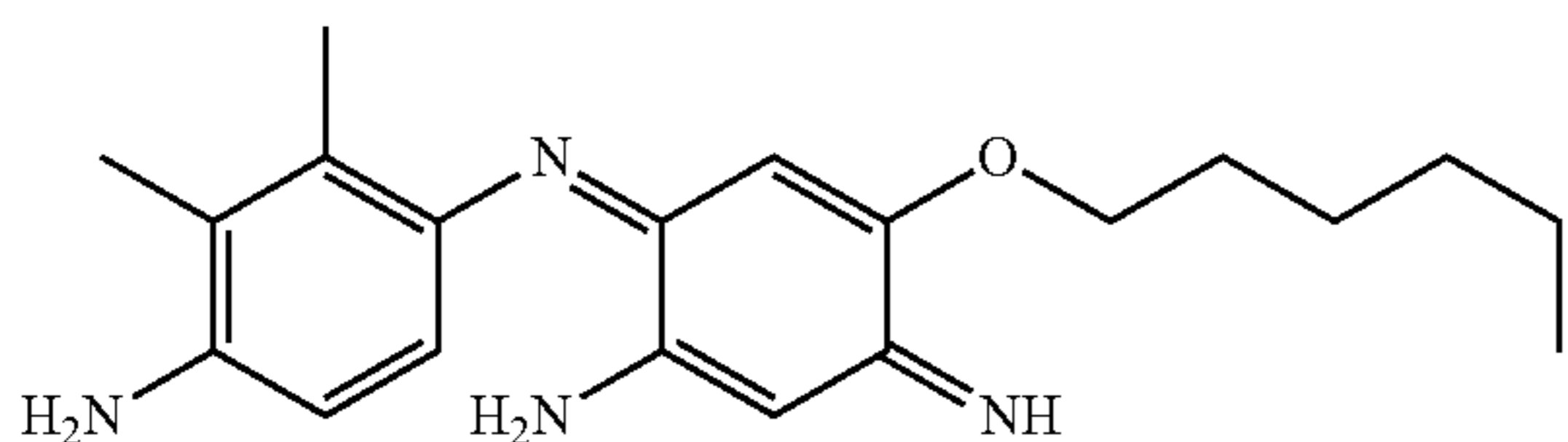
6-(4-Amino-2,3-dimethylphenylimino)-4-hexyloxy-3-iminocyclohexa-1,4-dienylamine
