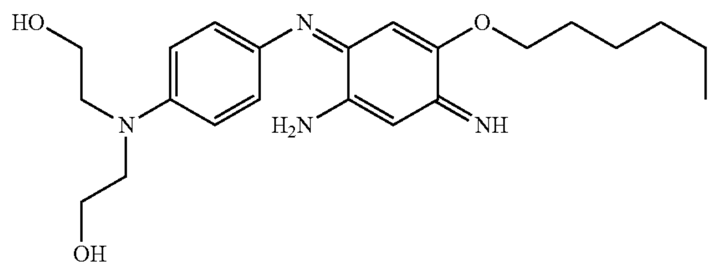
2-[[4-(2-Amino-5-hexyloxy-4-iminocyclohexa-2,5-dienylideneamino)phenyl](2-hydroxyethyl)amino]ethanol
