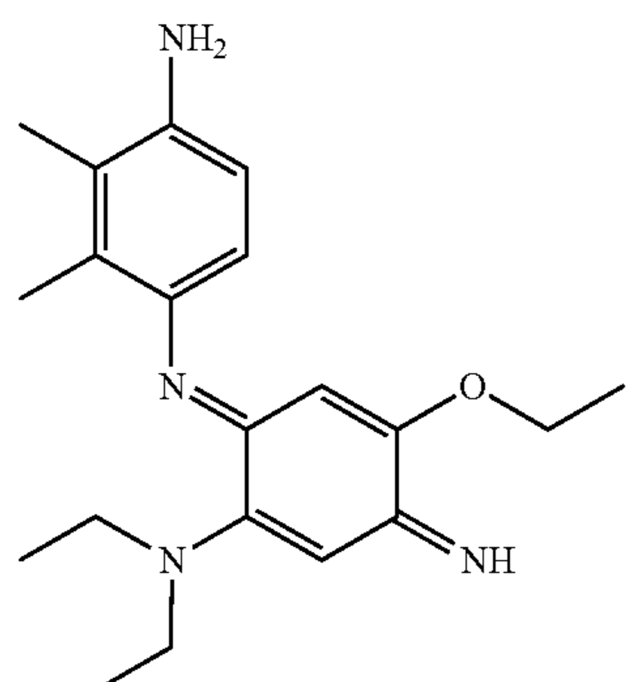
N-(2-Diethylamino-5-ethoxy-4-iminocyclohexa-2,5-dienylidene)-2,3-dimethylbenzene-1,4-diamine
