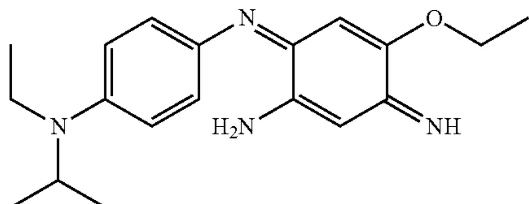
4-ethoxy-6-[4-(ethylisopropylamino)phenylimino]-3-iminocyclohexa-1,4-dienylamine
