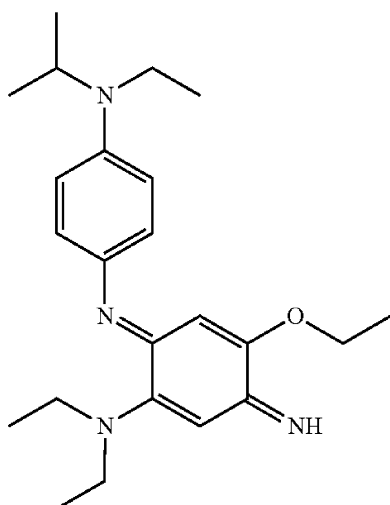
N-(2-Diethylamino-5-ethoxy-4-iminocyclohexa-2,5-dienylidene)-N'-ethyl-N'-isopropylbenzene-1,4-diamine
