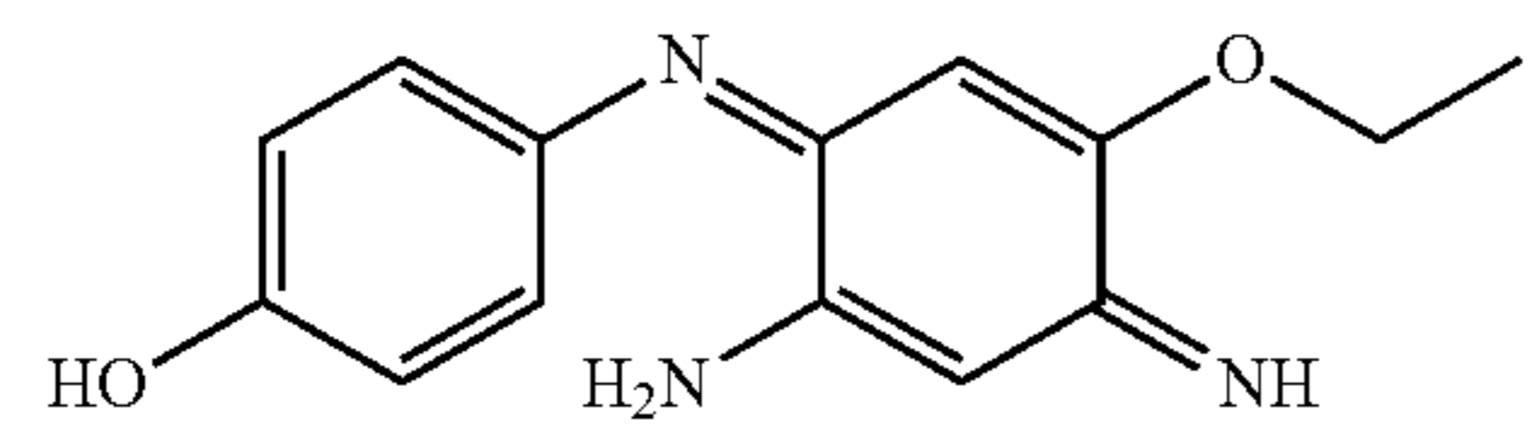
4-(2-Amino-5-ethoxy-4-iminocyclohexa-2,5-dienylideneamino)phenol
