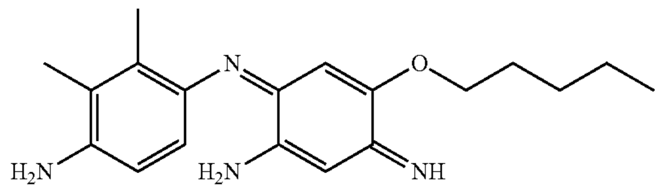
6-(4-Amino-2,3-dimethylphenylimino)-4-pentyloxy-3-iminocyclohexa-1,4-dienylamine
