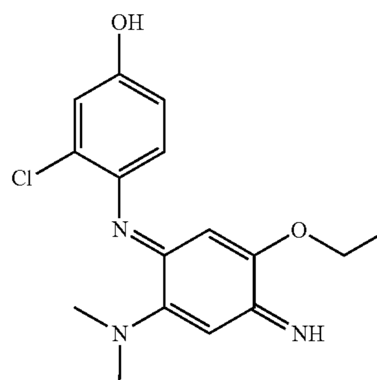
3-Chloro-4-(2-diethylamino-5-ethoxy-4-iminocyclohexa-2,5-dienylideneamino)phenol
