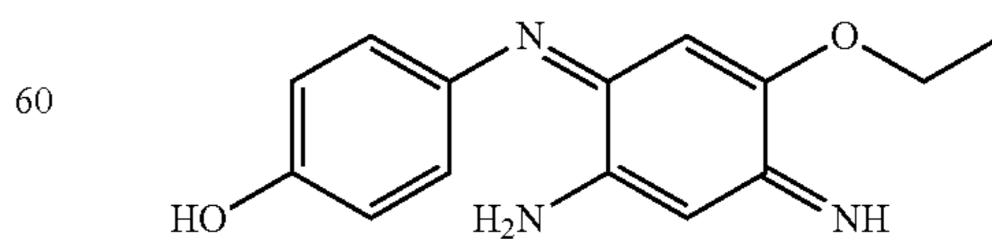
4-(2-Amino-5-ethoxy-4-iminocyclohexa-2,5-dienylideneamino)phenol
