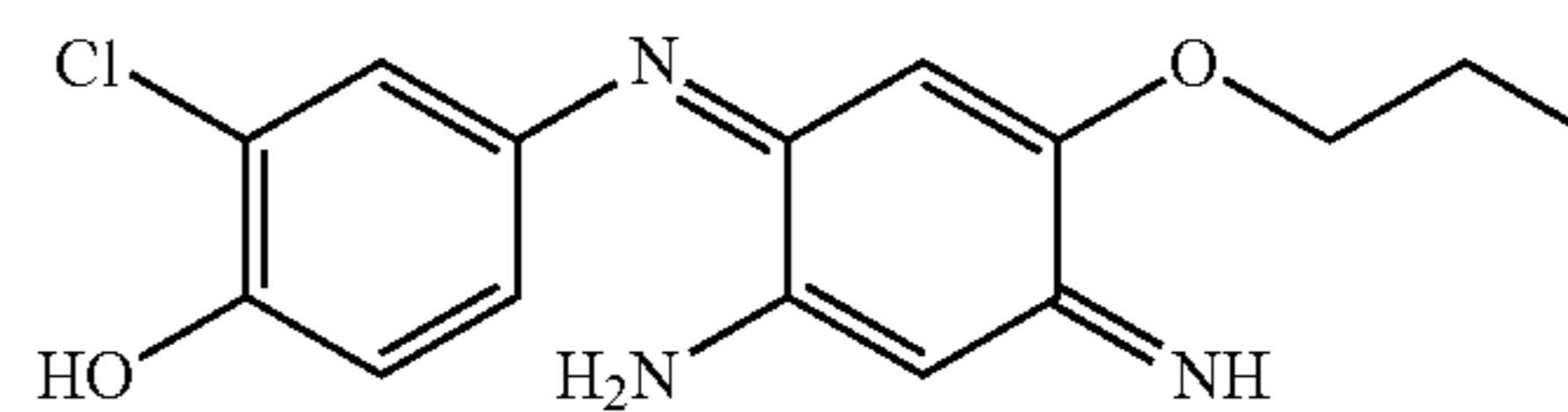
4-(2-Amino-5-propoxy-4-iminocyclohexa-2,5-dienylideneamino)-2-chlorophenol
