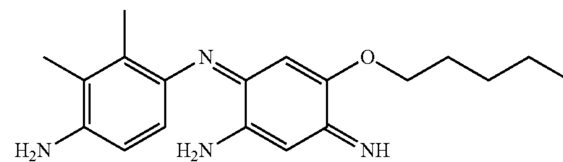
6-(4-Amino-2,3-dimethylphenylimino)-4-pentyloxy-3-aminocyclohexa-1,4-dienylamine
