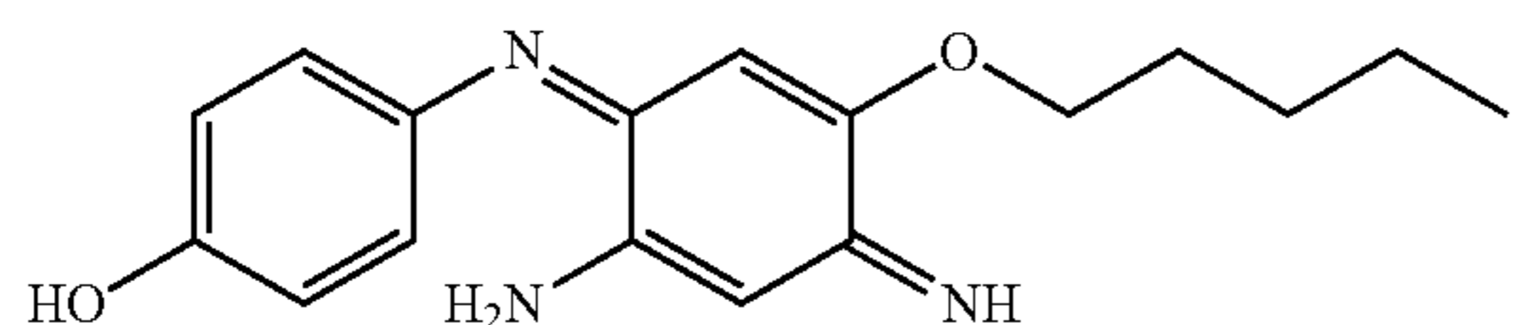
4-(2-Amino-5-pentyloxy-4-iminocyclohexa-2,5-dienylideneamino)phenol
