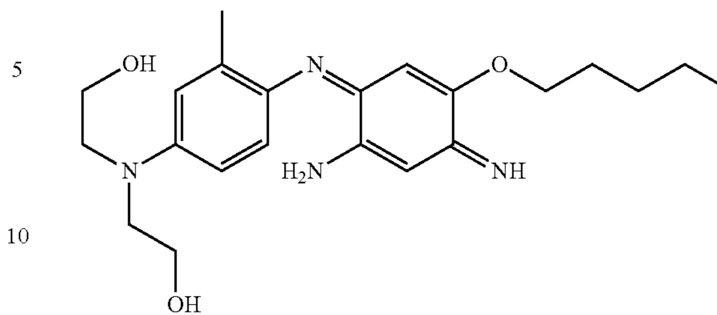
2-[[4-(2-Amino-5-pentyloxy-4-iminocyclohexa-2,5-dienylideneamino)-3-methylphenyl](2-hydroxyethyl)amino]ethanol
