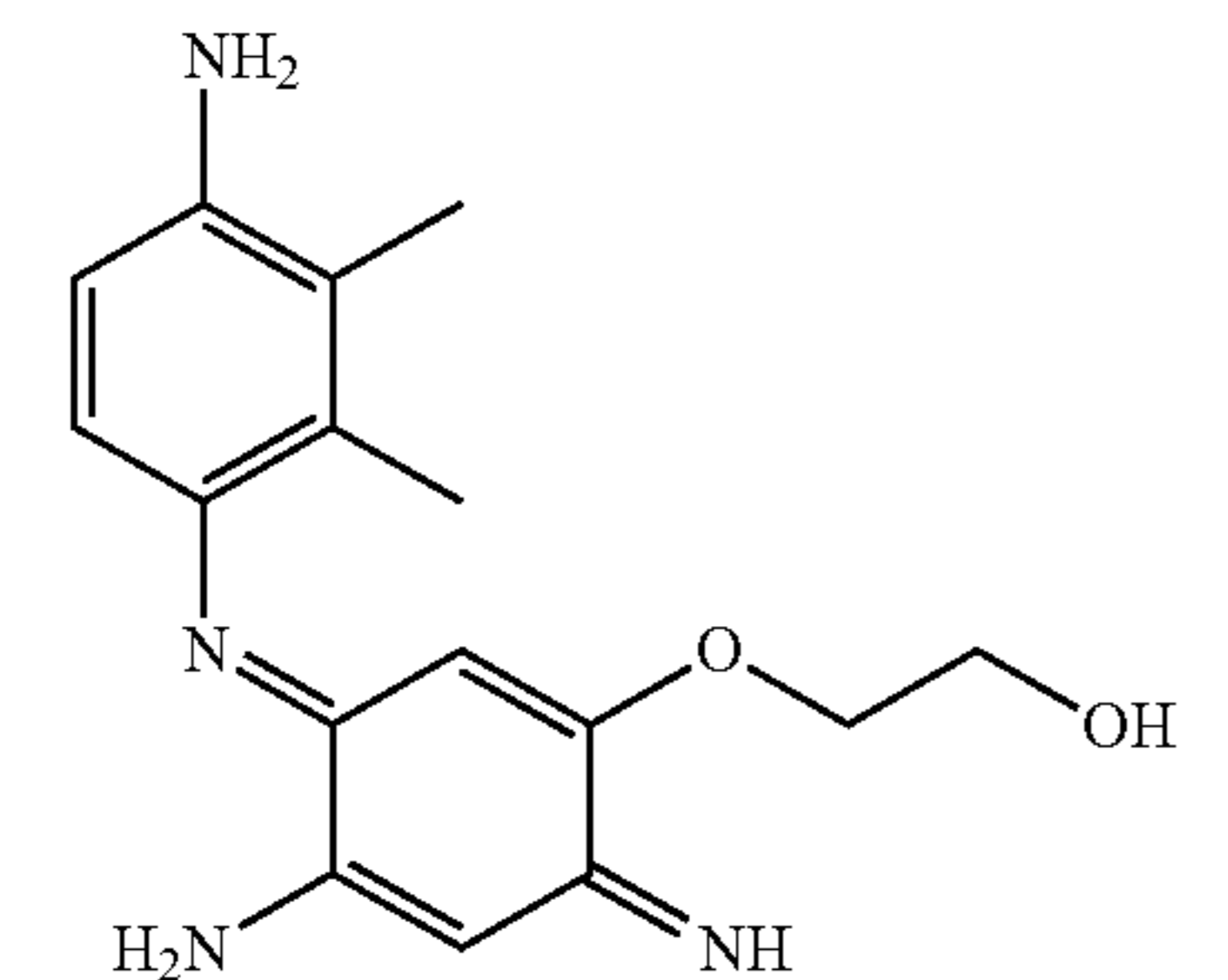
2-{4-Amino-3-[4-amino-2,3-dimethylphenylimino]-6-iminocyclohexa-1,4-dienyloxy}ethanol
