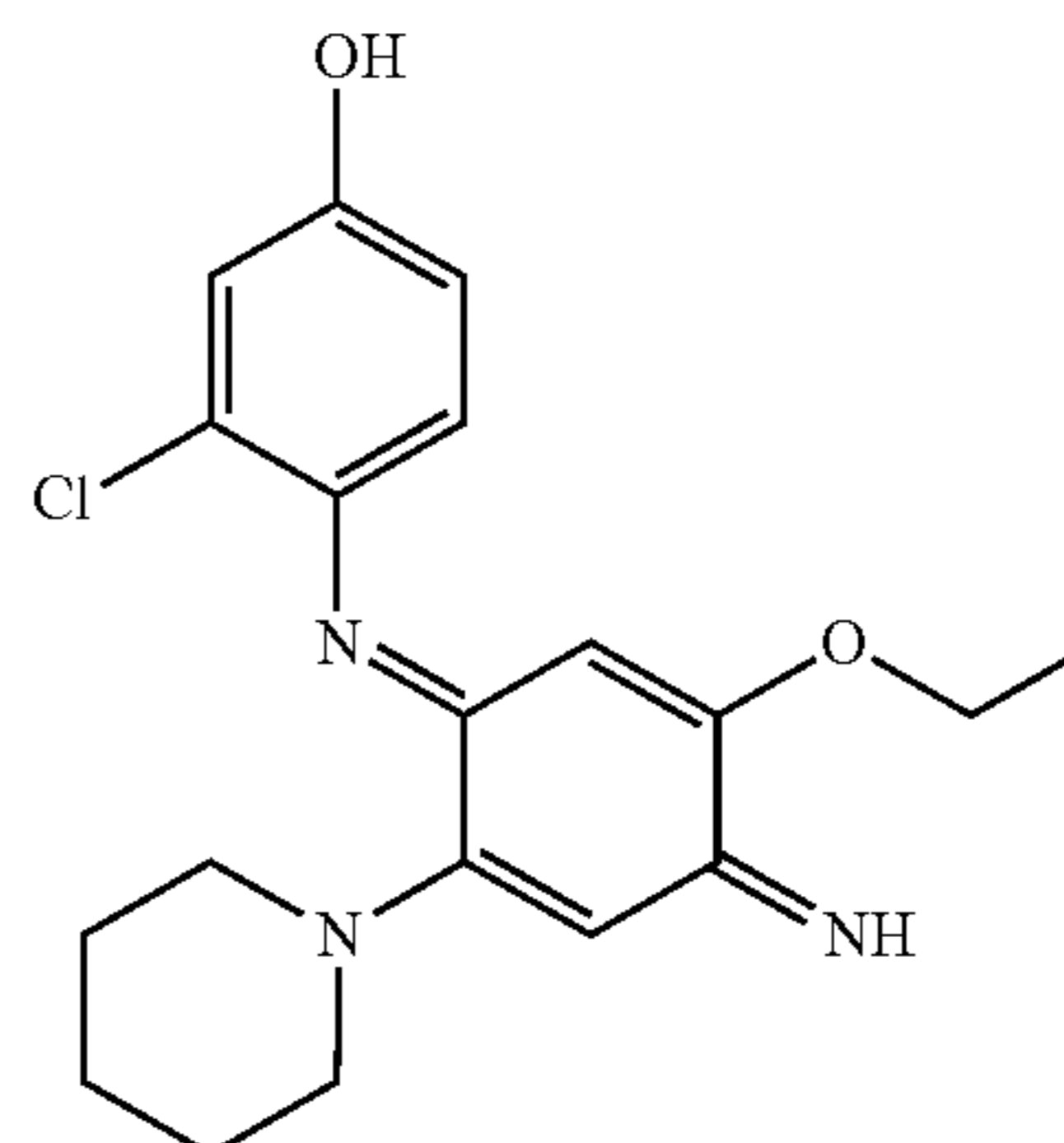
3-Chloro-4-(5-ethoxy-4-imino-2-piperidin-1-ylcyclohexa-2,5-dienylideneamino)phenol
