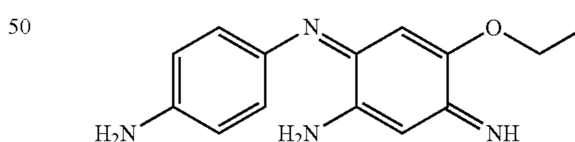
6-(4-Aminophenylimino)-4-ethoxy-3-iminocyclohexa-1,4-dienylamine
