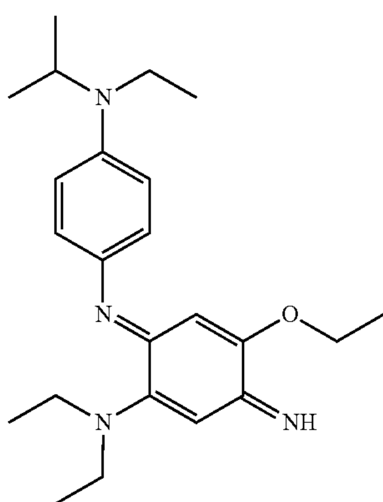
N-(2-Diethylamino-5-ethoxy-4-iminocyclohexa-2,5-dienylidene)-N'-ethyl-N'-isopropylbenzene-1,4-diamine
