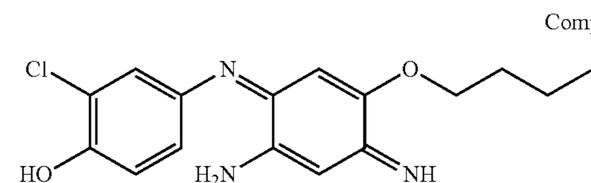
4-(2-Amino-5-butoxy-4-iminocyclohexa-2,5-dienylideneamino)-2-chlorophenol
