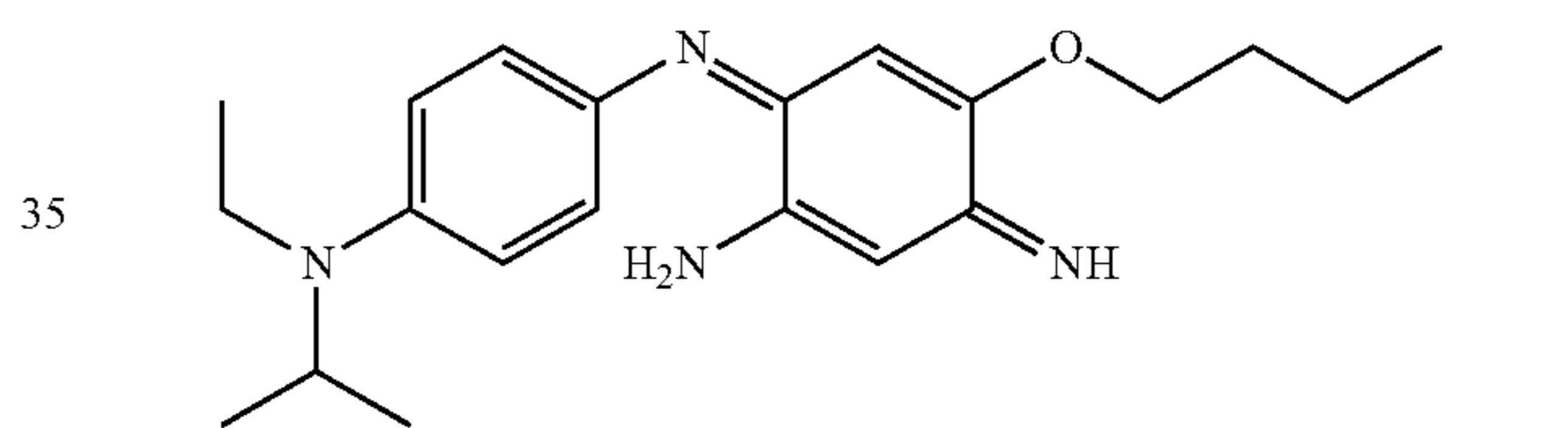
4-Butoxy-6-[4-(ethylisopropylamino)phenylimino]-3-iminocyclohexa-1,4-dienylamine
