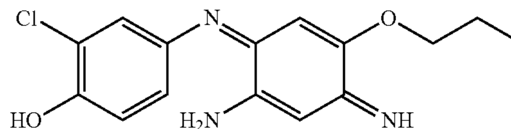
4-(2-Amino-5-propoxy-4-iminocyclohexa-2,5-dienylideneamino)-2-chlorophenol
