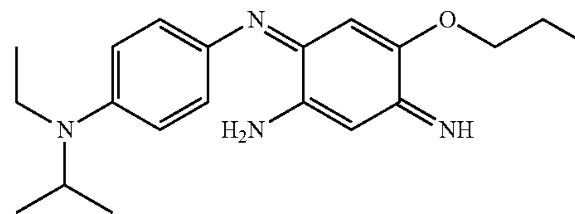
4-propoxy-6-[4-(ethylisopropylamino)phenylimino]-3-iminocyclohexa-1,4-dienylamine
