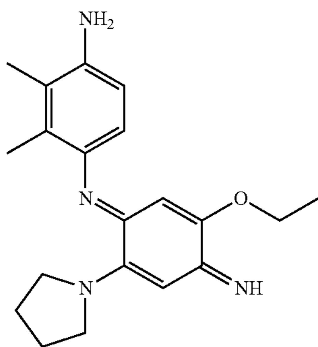
N-(5-Ethoxy-4-imino-2-pyrrolidin-1-ylcyclohexa-2,5-dienylidene)-2,3-dimethylbenzene-1,4-diamine
