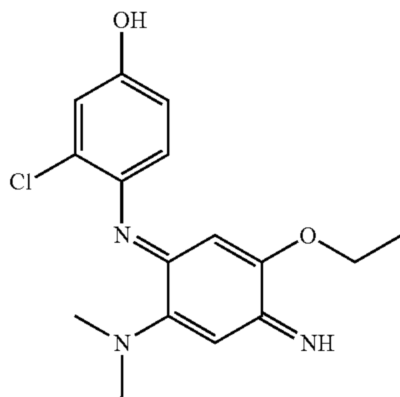
3-Chloro-4-(2-diethylamino-5-ethoxy-4-iminocyclohexa-2,5-dienylideneamino)phenol
