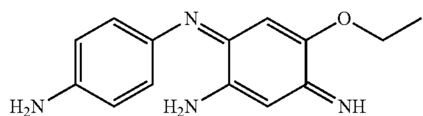
6-(4-Aminophenylimino)-4-ethoxy-3-iminocyclohexa-1,4-dienylamine
