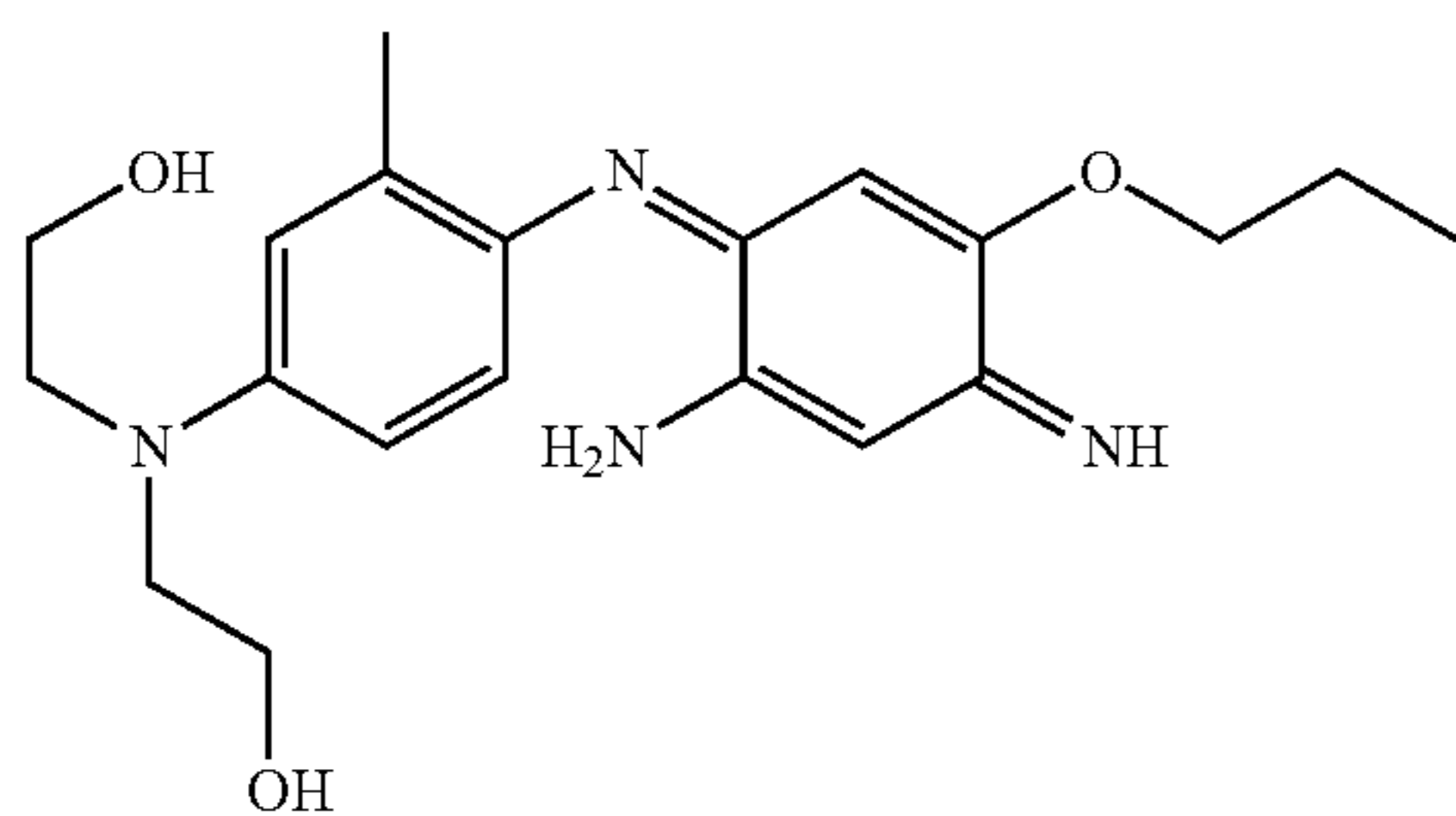
2-[[4-(2-Amino-5-propoxy-4-iminocyclohexa-2,5-dienylideneamino)-3-methylphenyl](2-hydroxyethyl)amino] ethanol
