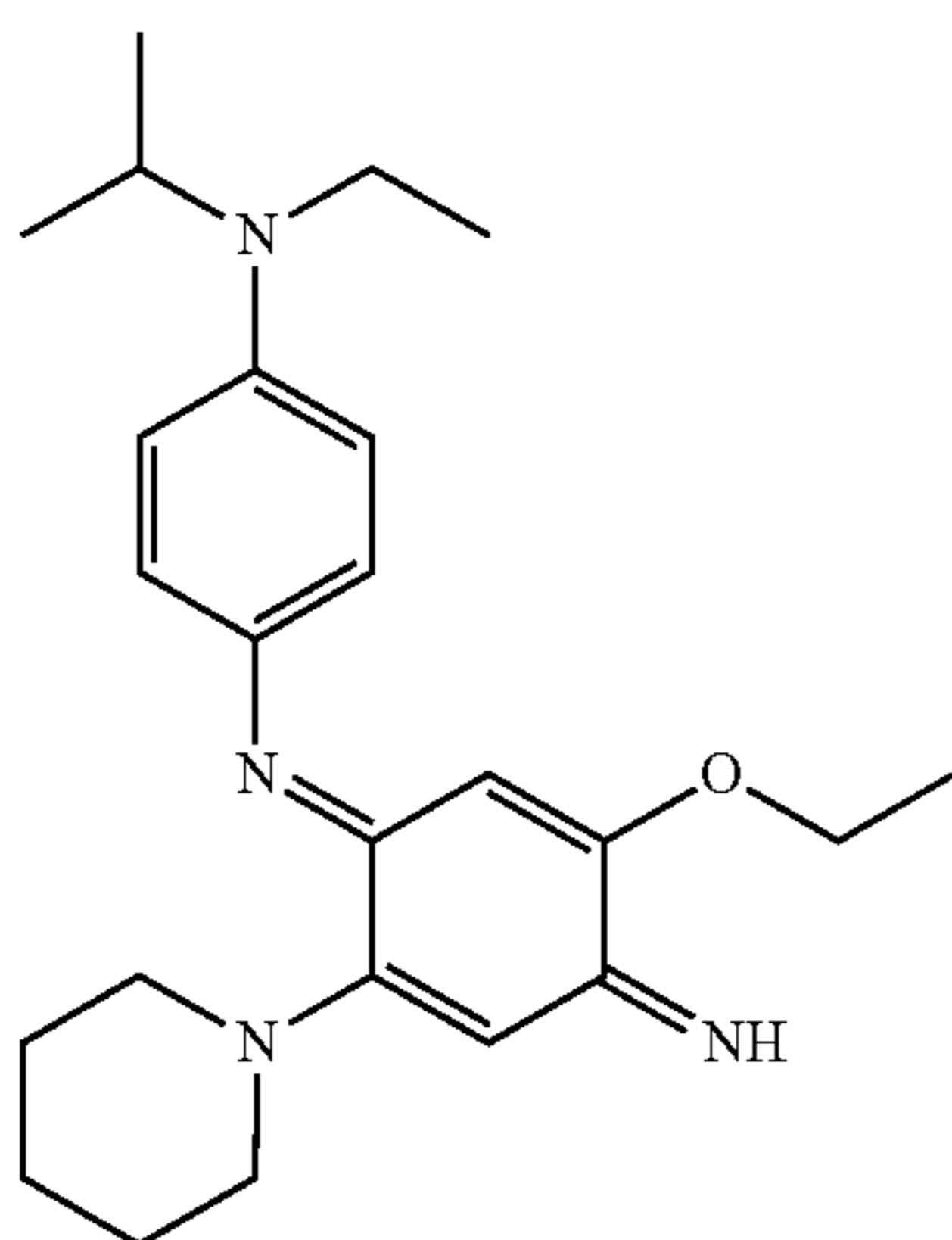
N-(5-Ethoxy-4-imino-2-piperidin-1-ylcyclohexa-2,5-dienylidene)-N'-ethyl-N'-isopropylbenzene-1,4-diamine
