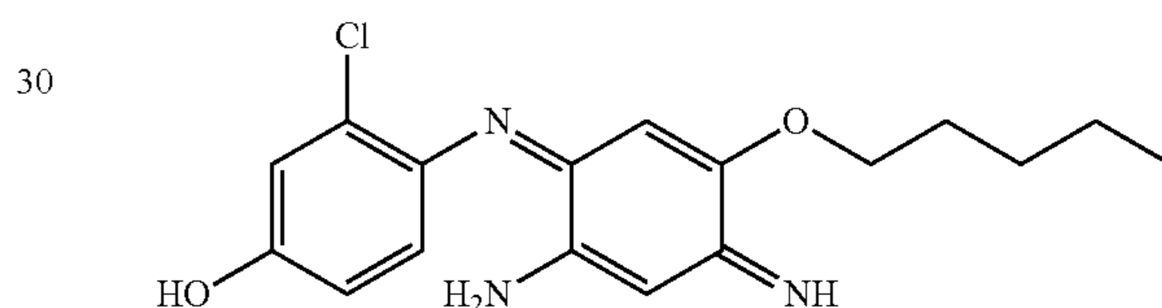
4-(2-Amino-5-pentyloxy-4-iminocyclohexa-2,5-dienylideneamino)-3-chlorophenol
