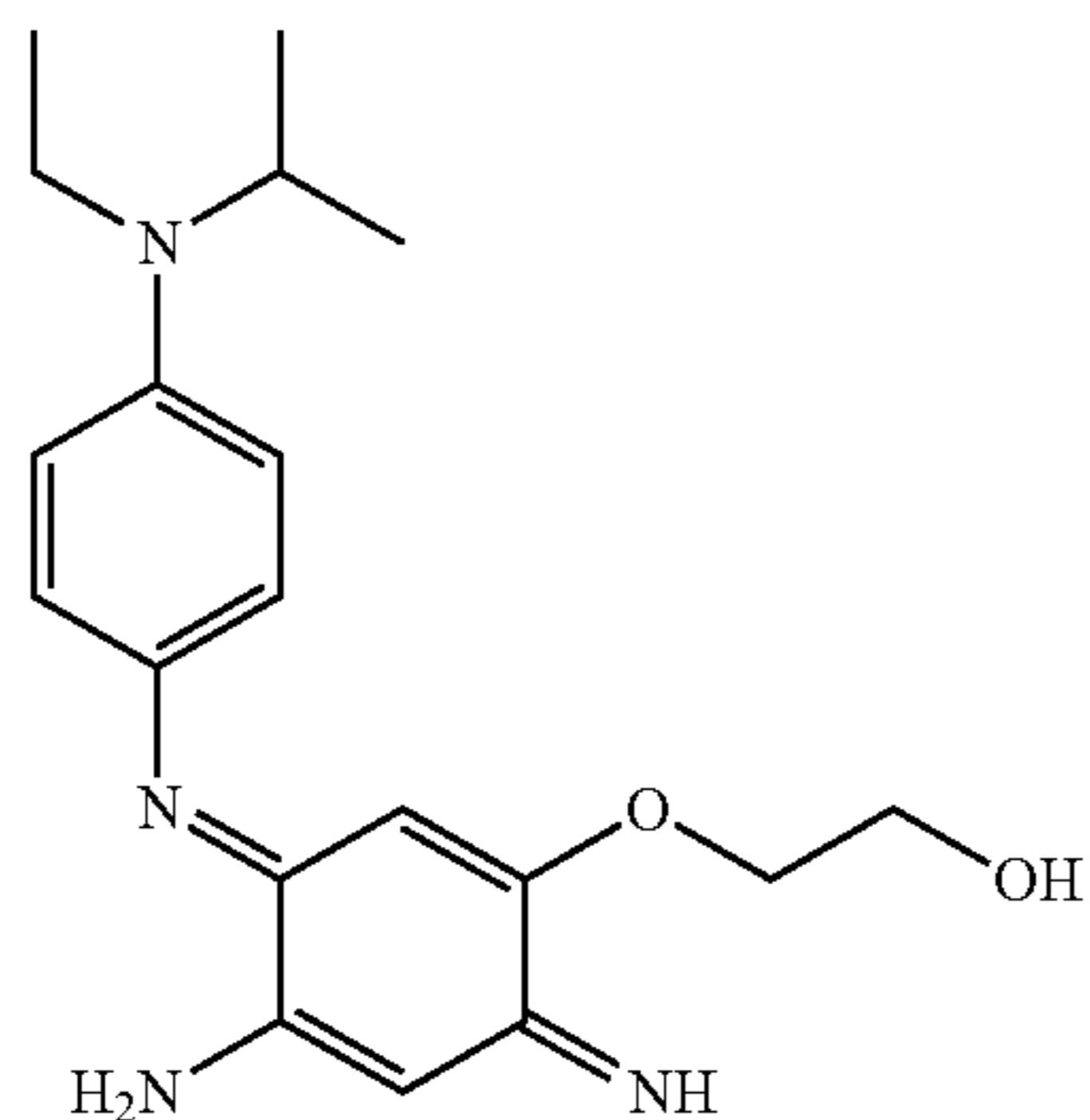
2-(4-Amino-3-[4-(ethylisopropylamino)phenylimino]-6-iminocyclohexa-1,4-dienyloxy)ethanol
