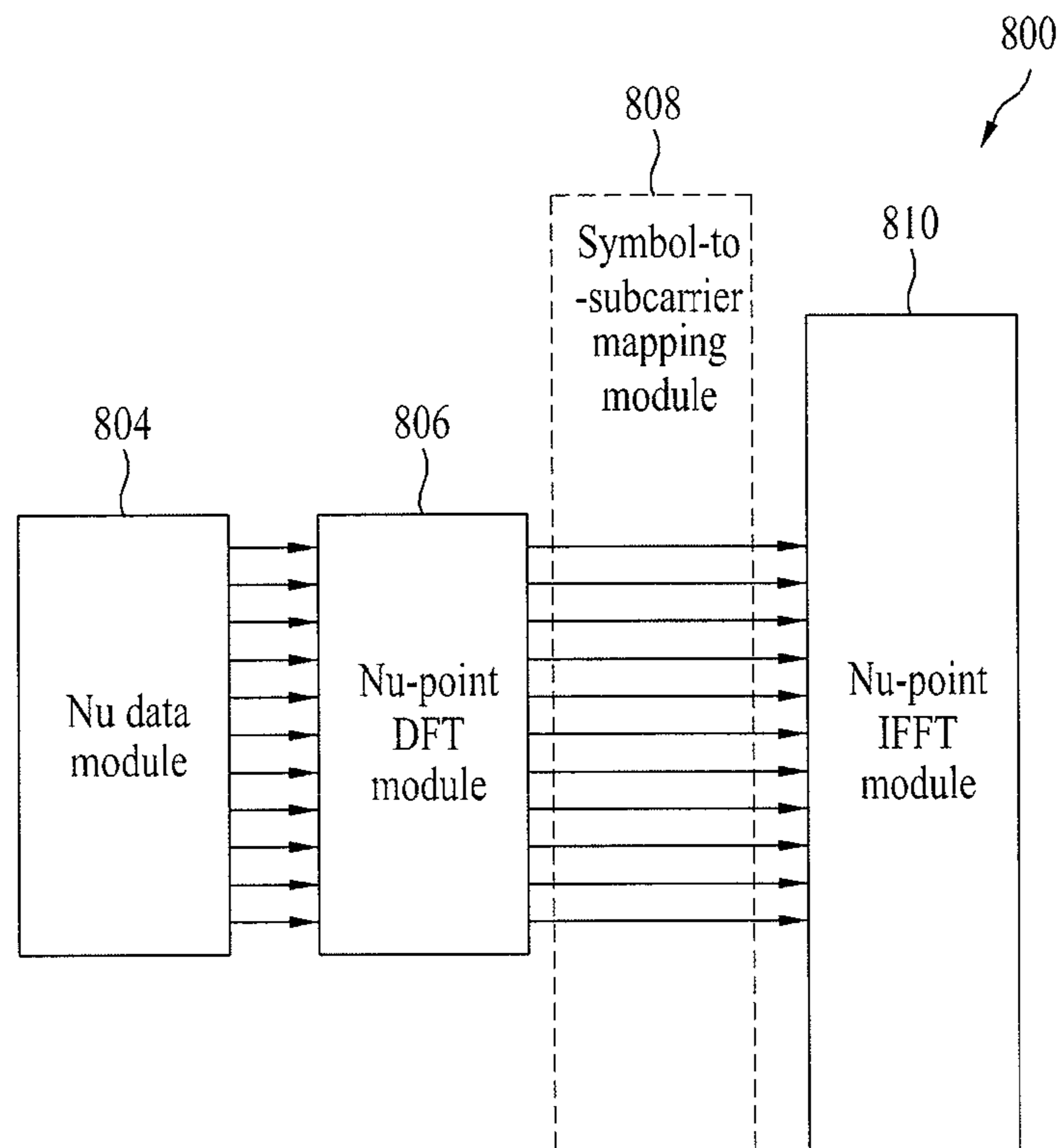
Localized DFT-s-OFDMA
