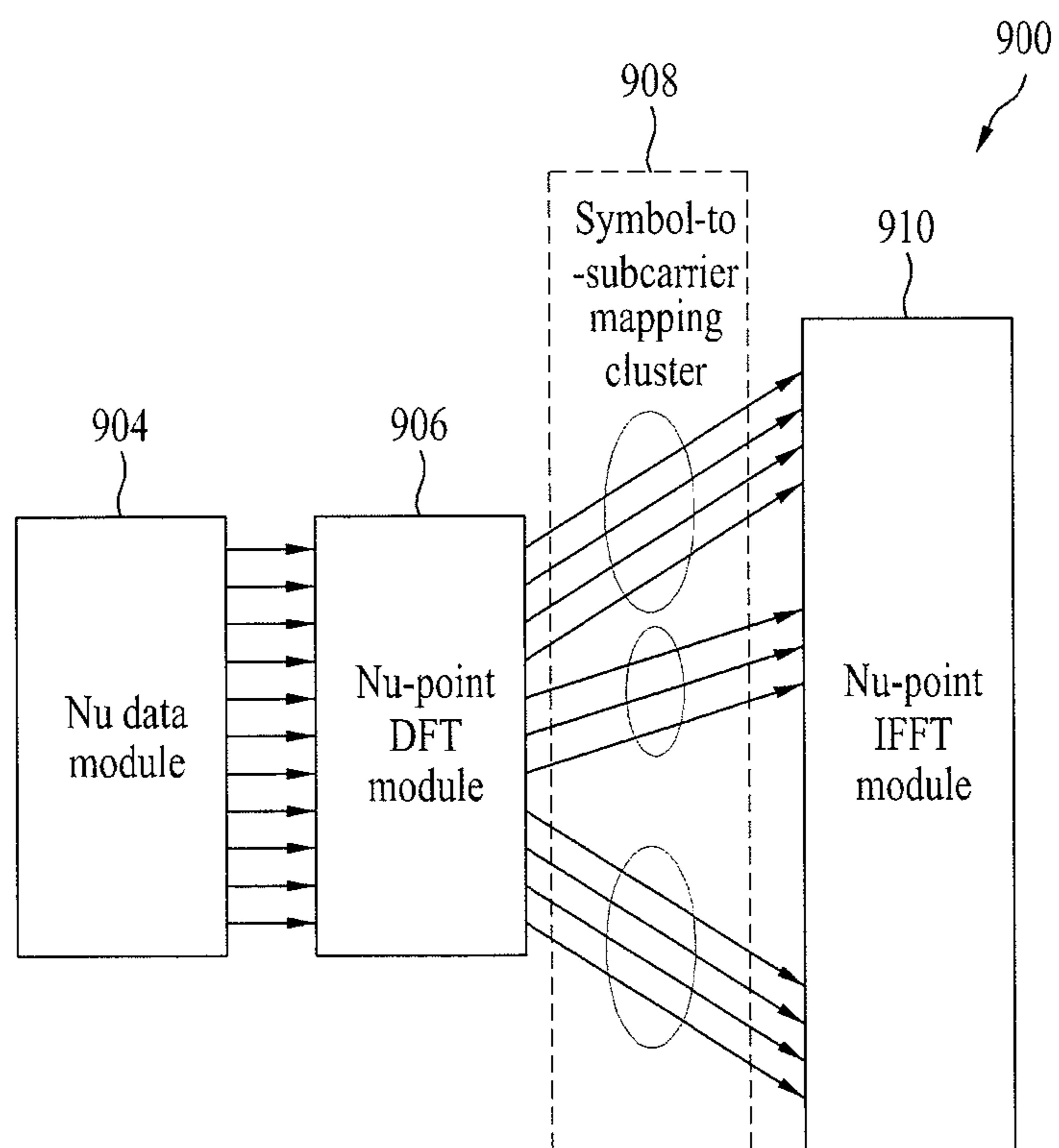
Clustered DFT-s-OFDMA
