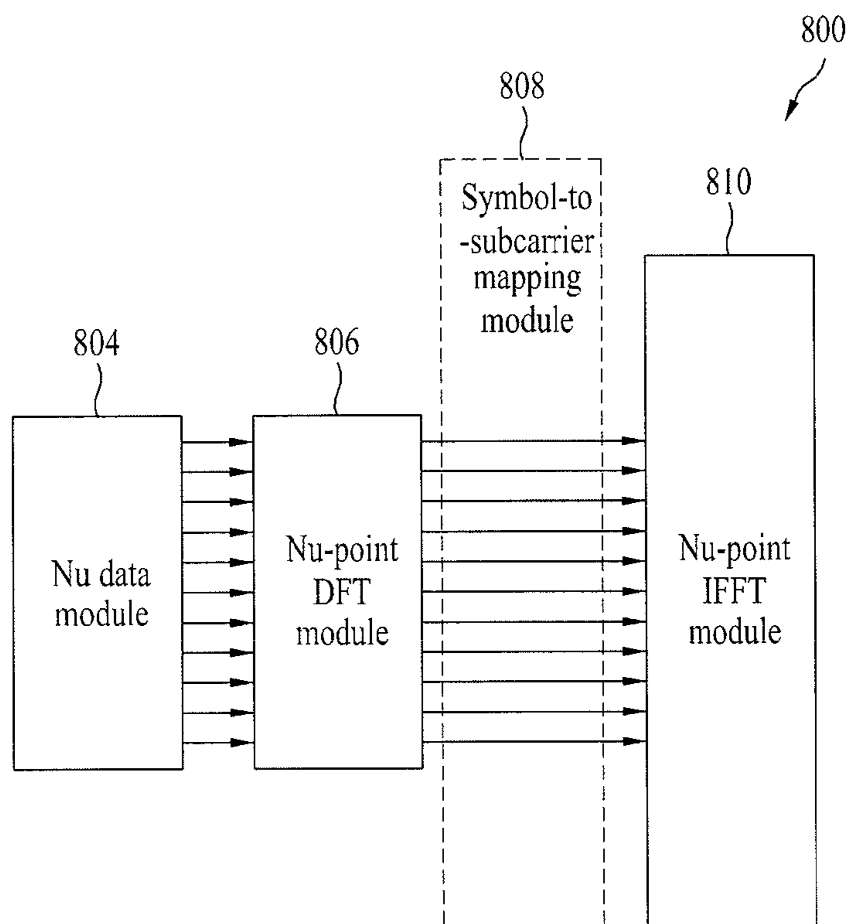
Localized DFT-s-OFDMA
