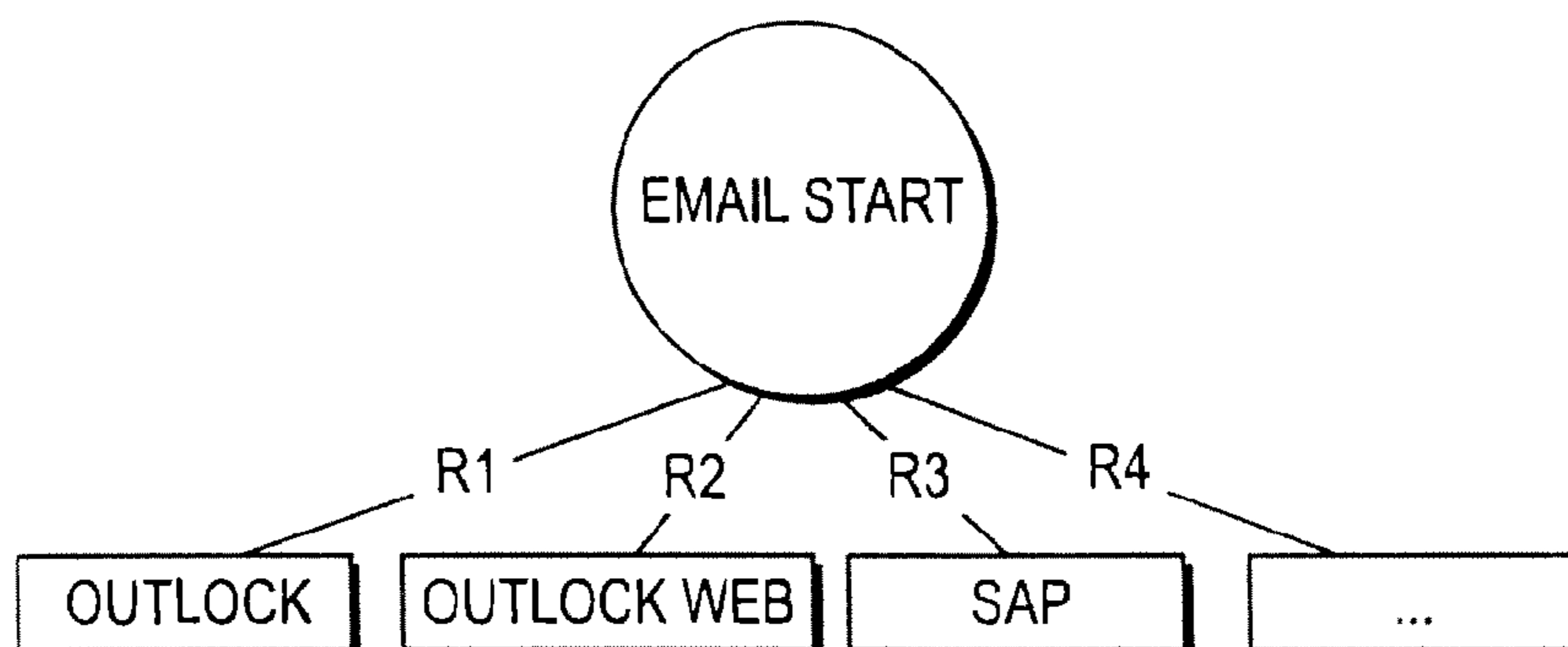
EMISSION PROBABILITIES EXAMPLE 1
