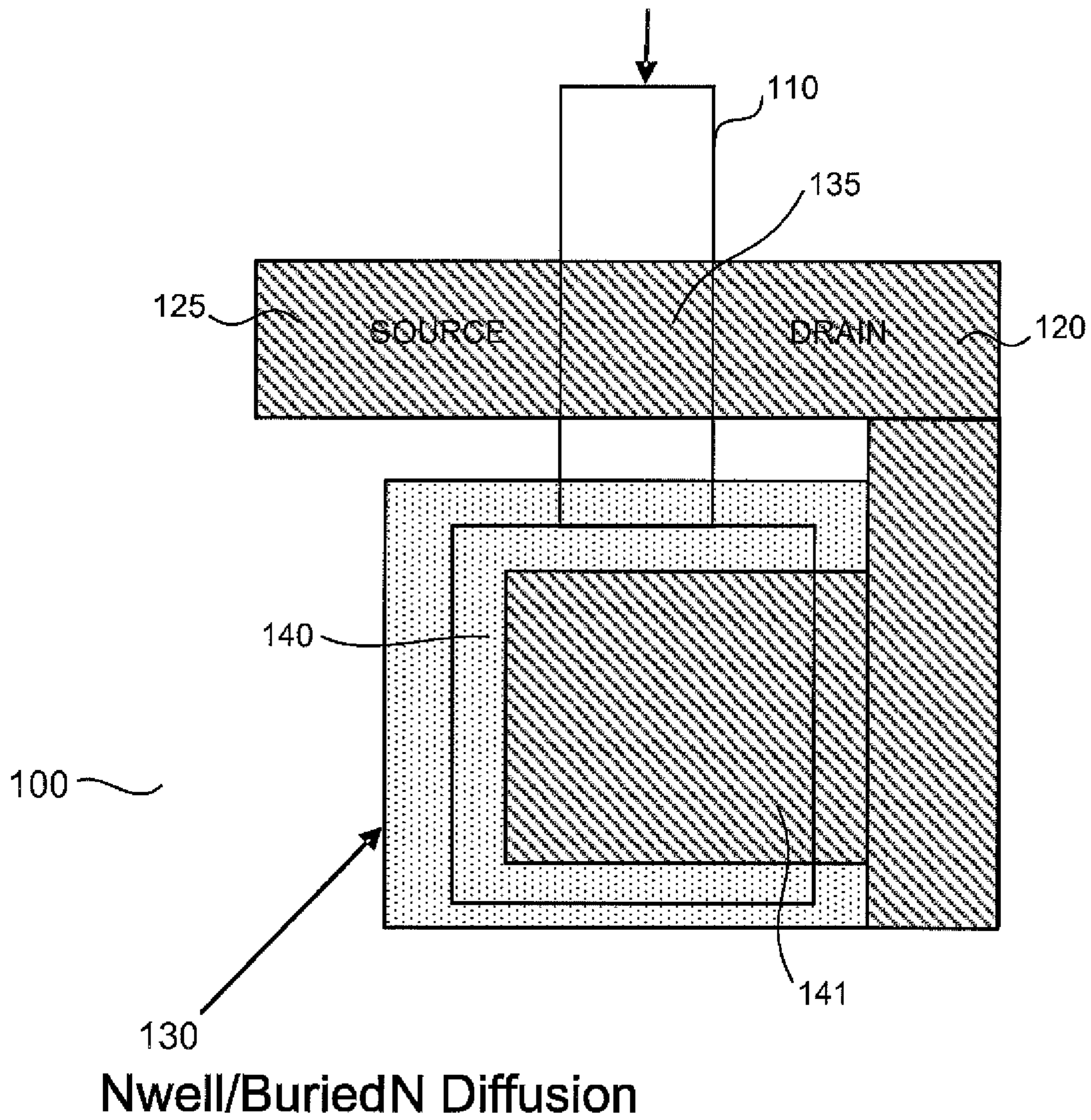
FIG. 1 Floating Gate
