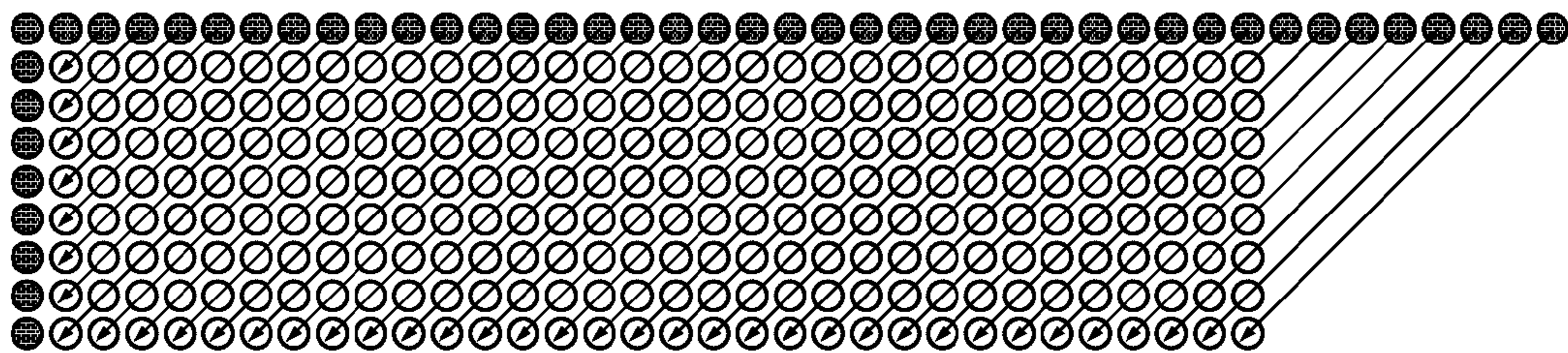
Prediction mode 3
