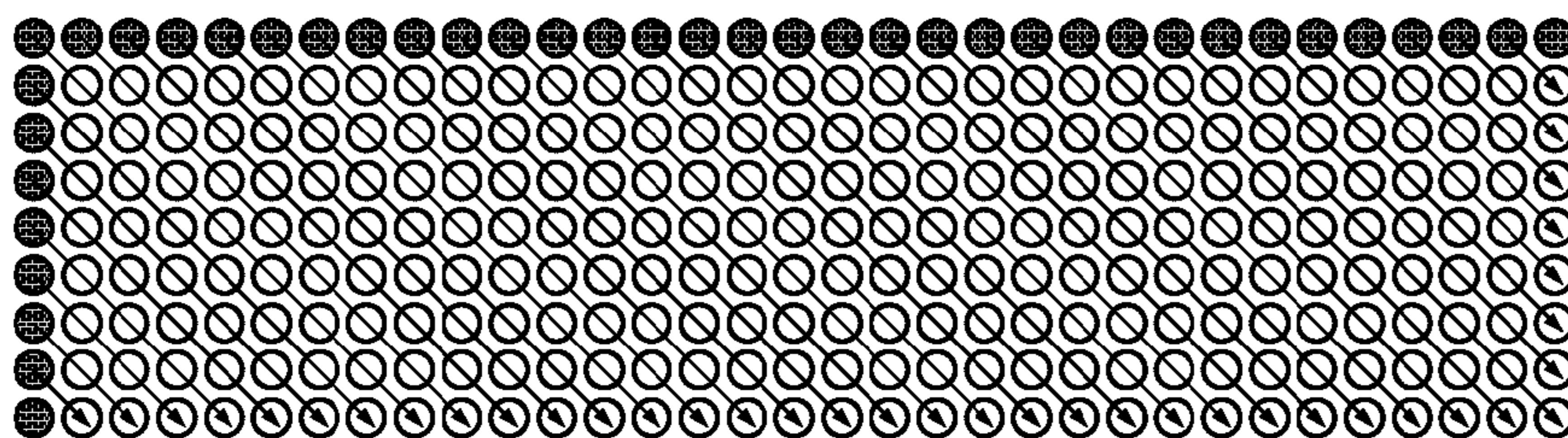
Prediction mode 4
