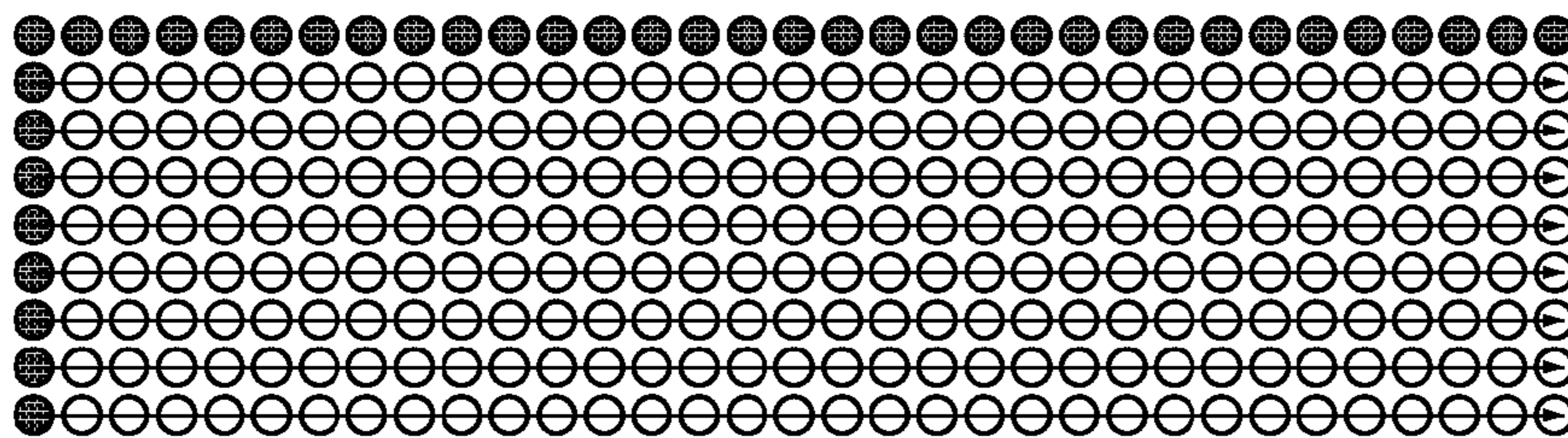
Prediction mode 1
