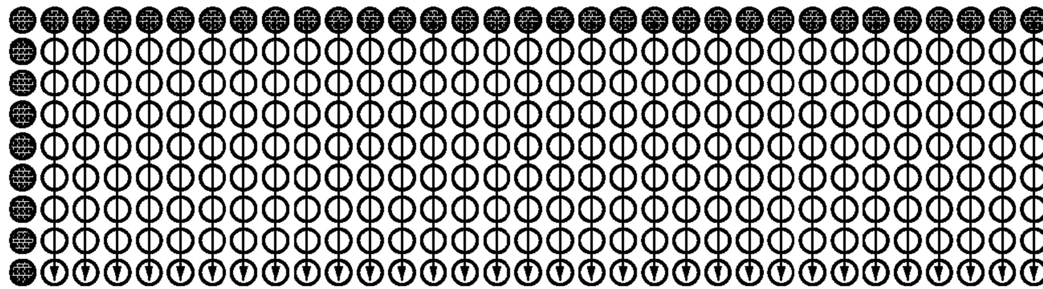
Prediction mode 0
