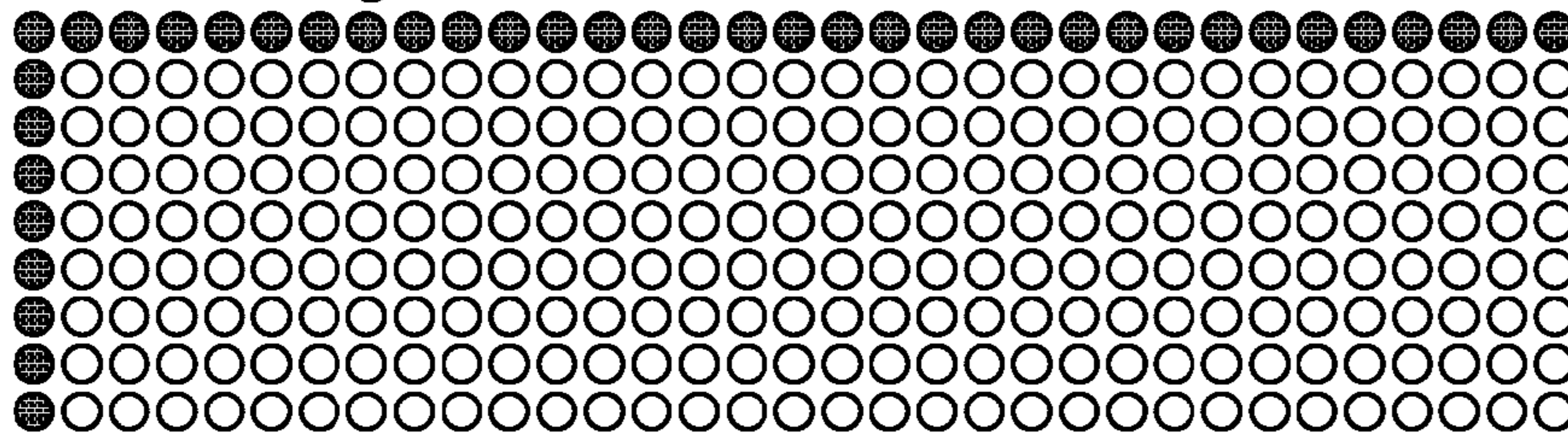
Prediction mode 2
