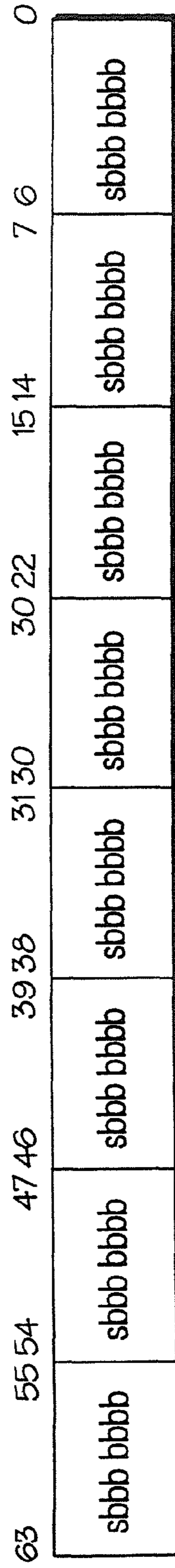
Signed Packed Byte In-register Representation 511
