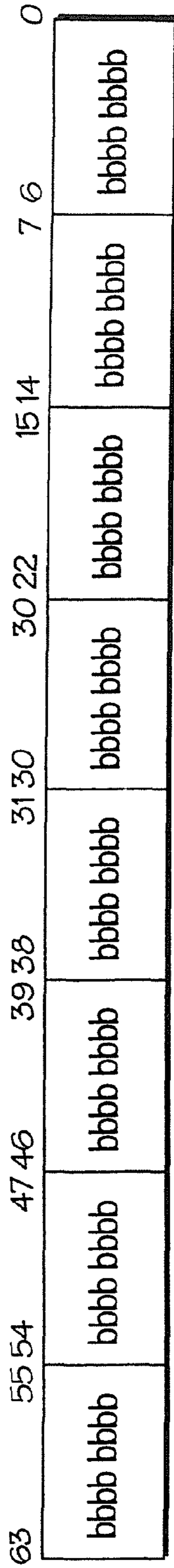
Unsigned Packed Byte In-register Representation 510
