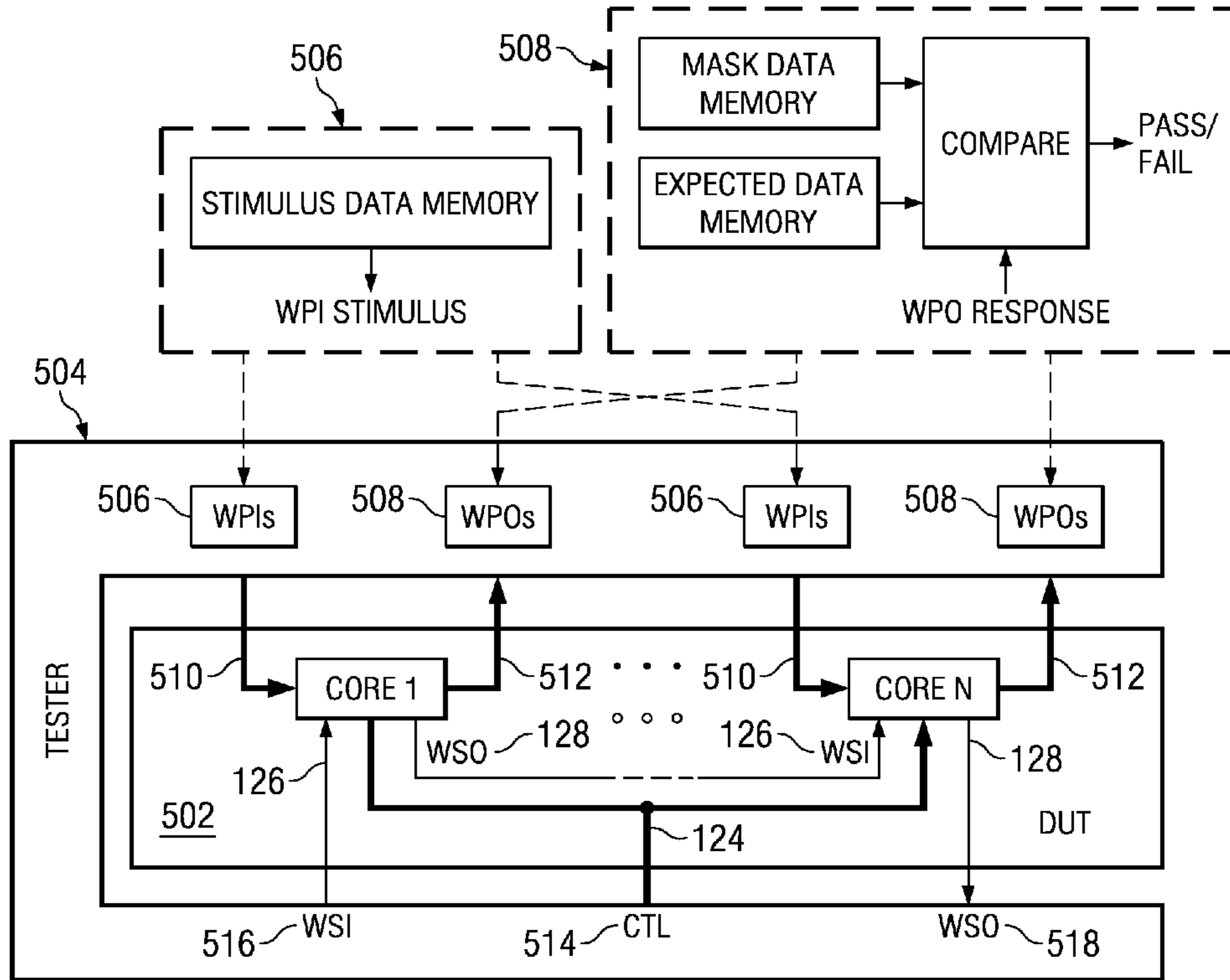
FIG. 5 (PRIOR ART)
