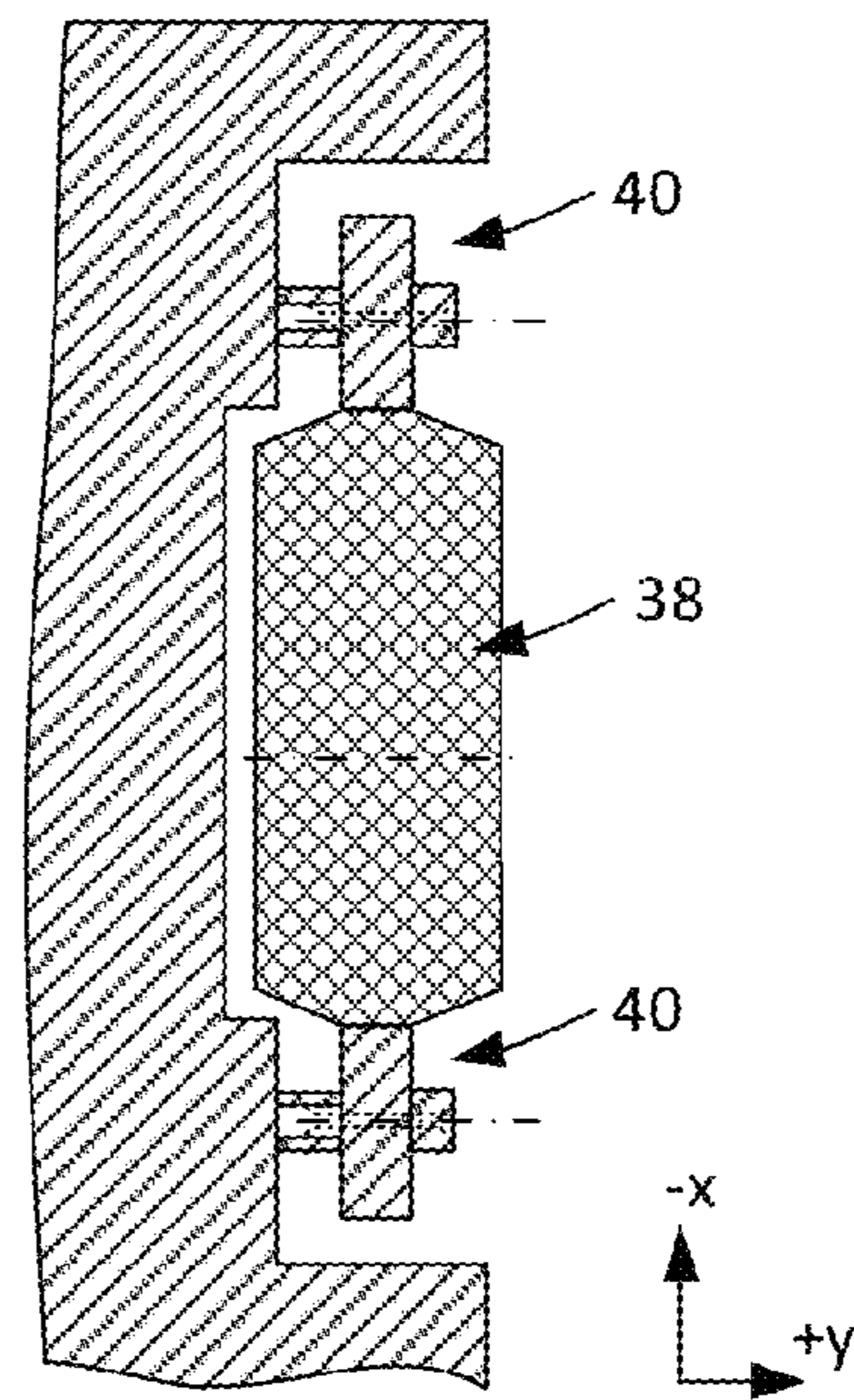
Cross-Section A-A
