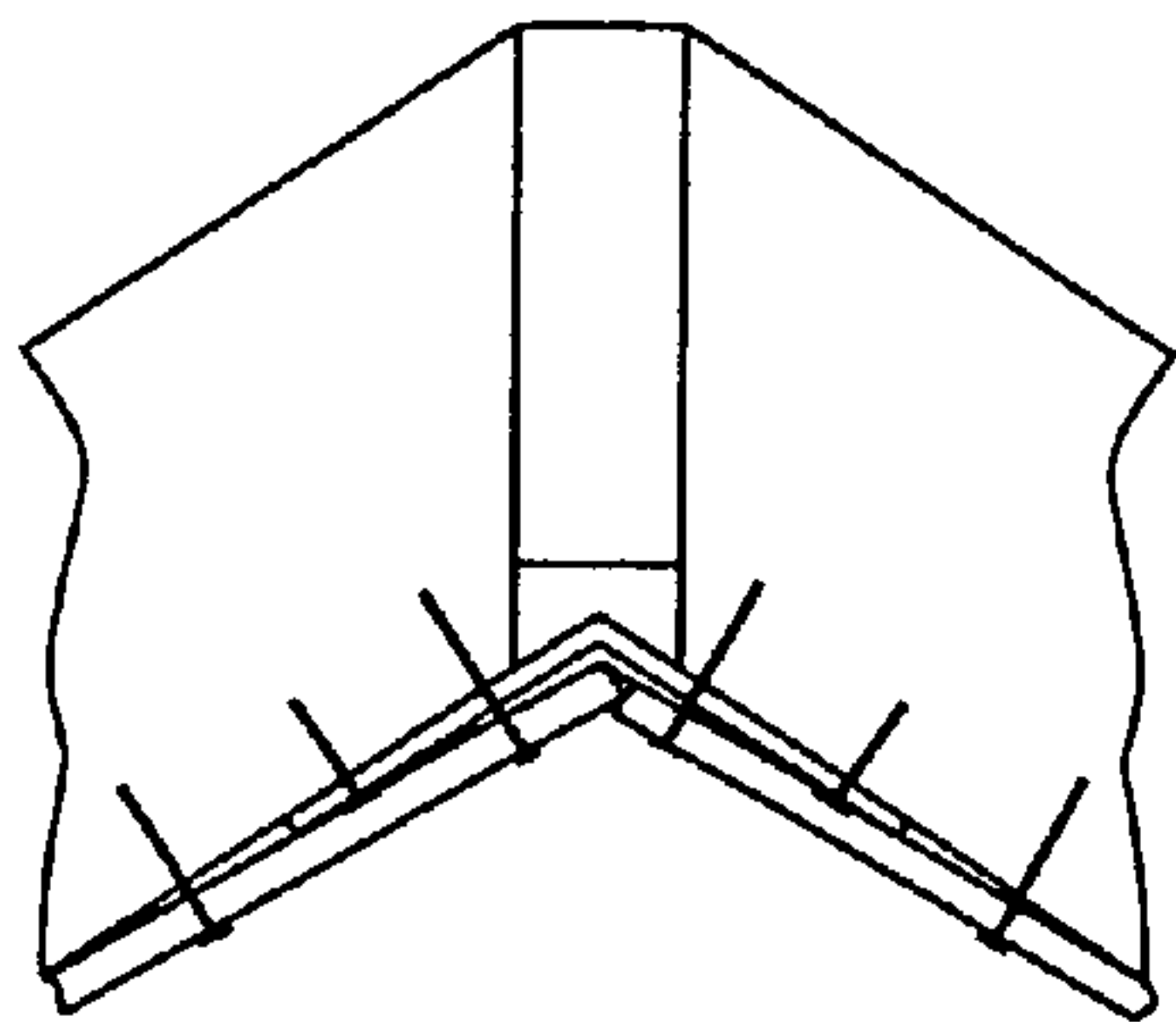
FASTEN WALLBOARD TO RAFTERS PAST EDGES OF HINGED METAL CONNECTOR
