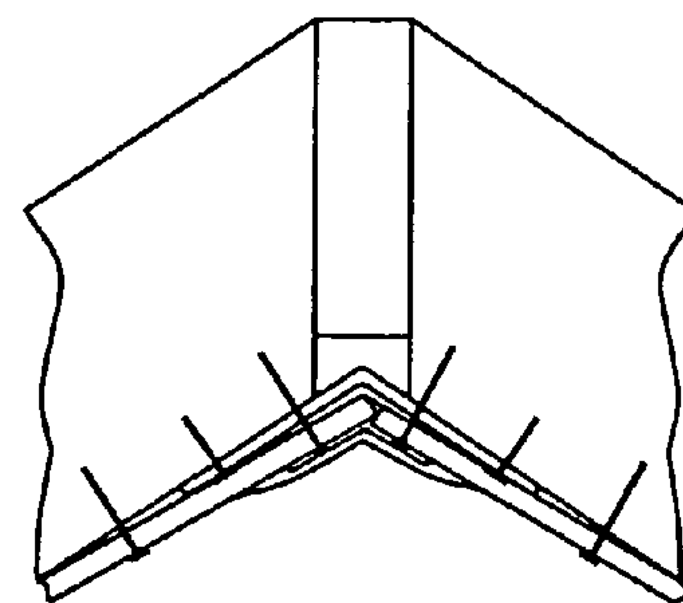
APPLY CONVENTIONAL DRYWALL TAPE AND DRYWALL COMPOUND OVER ROOM SIDE OF JOINT AND FINISH
