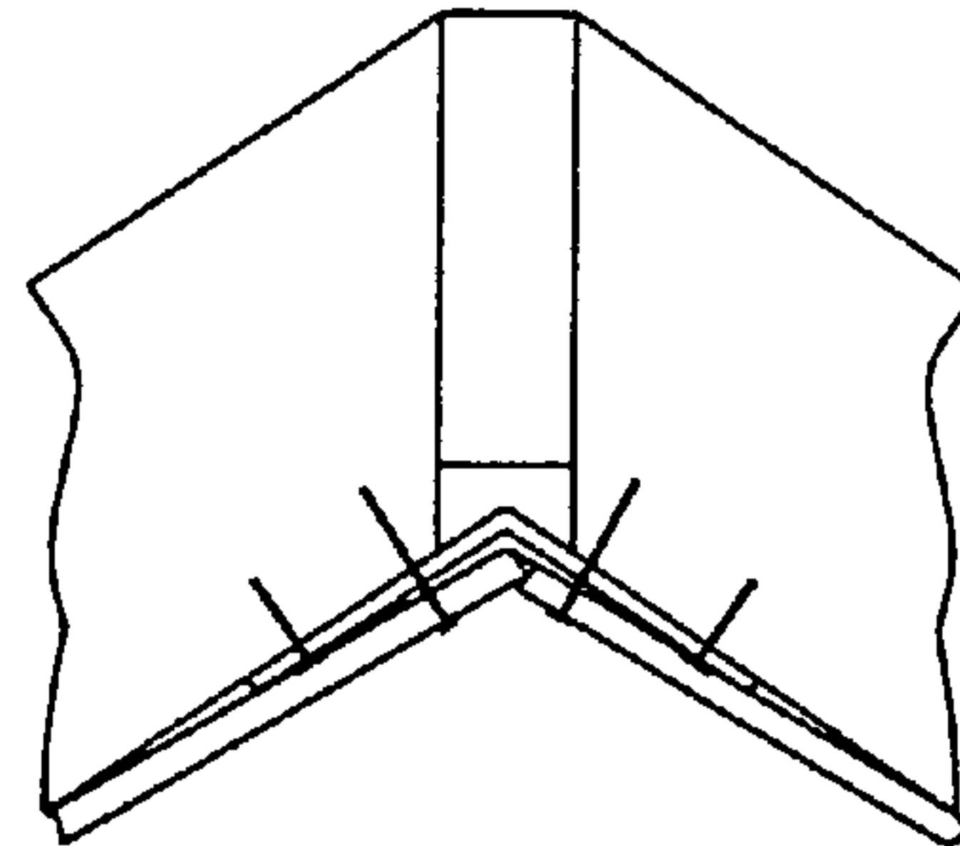
FASTEN WALLBOARD TO CONNECTOR ONLY ADJACENT TO RIDGE BOARD
