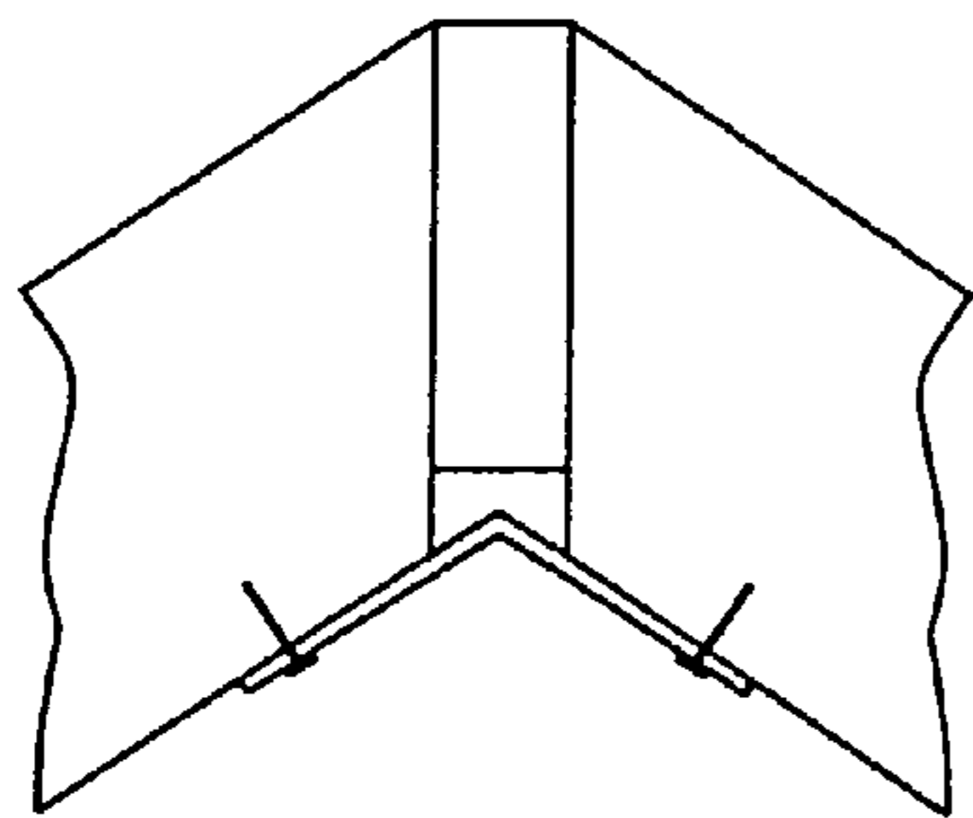
FASTEN CONNECTOR TABS TO RAFTERS AND ALIGN EDGES OF WINGS INTO STRAIGHT LINE
