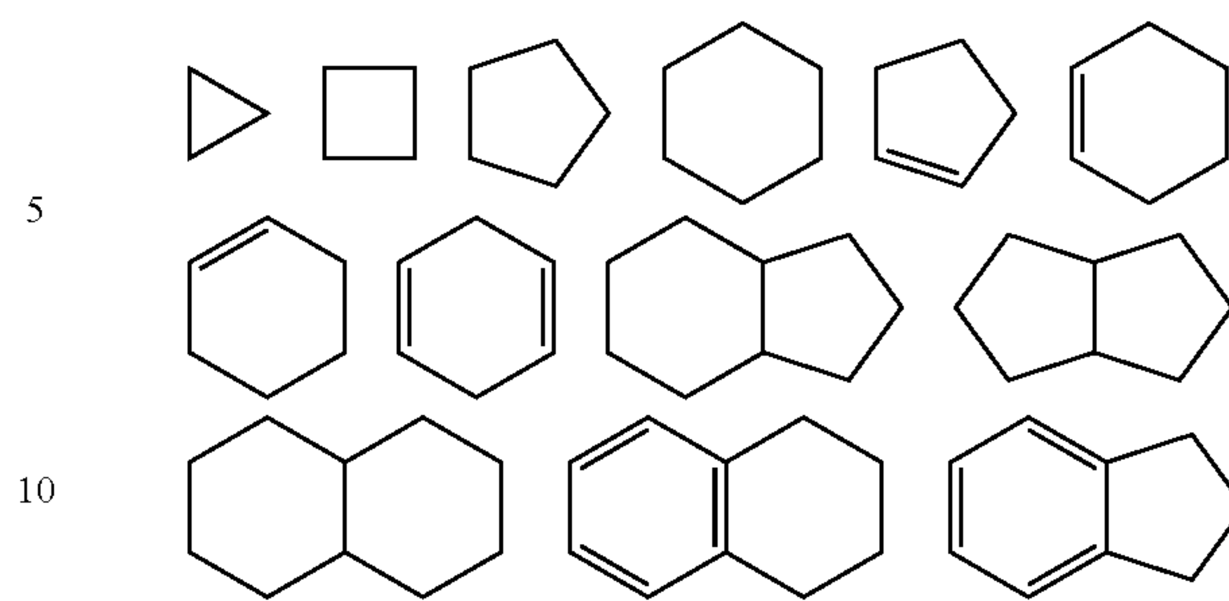
Formula I
