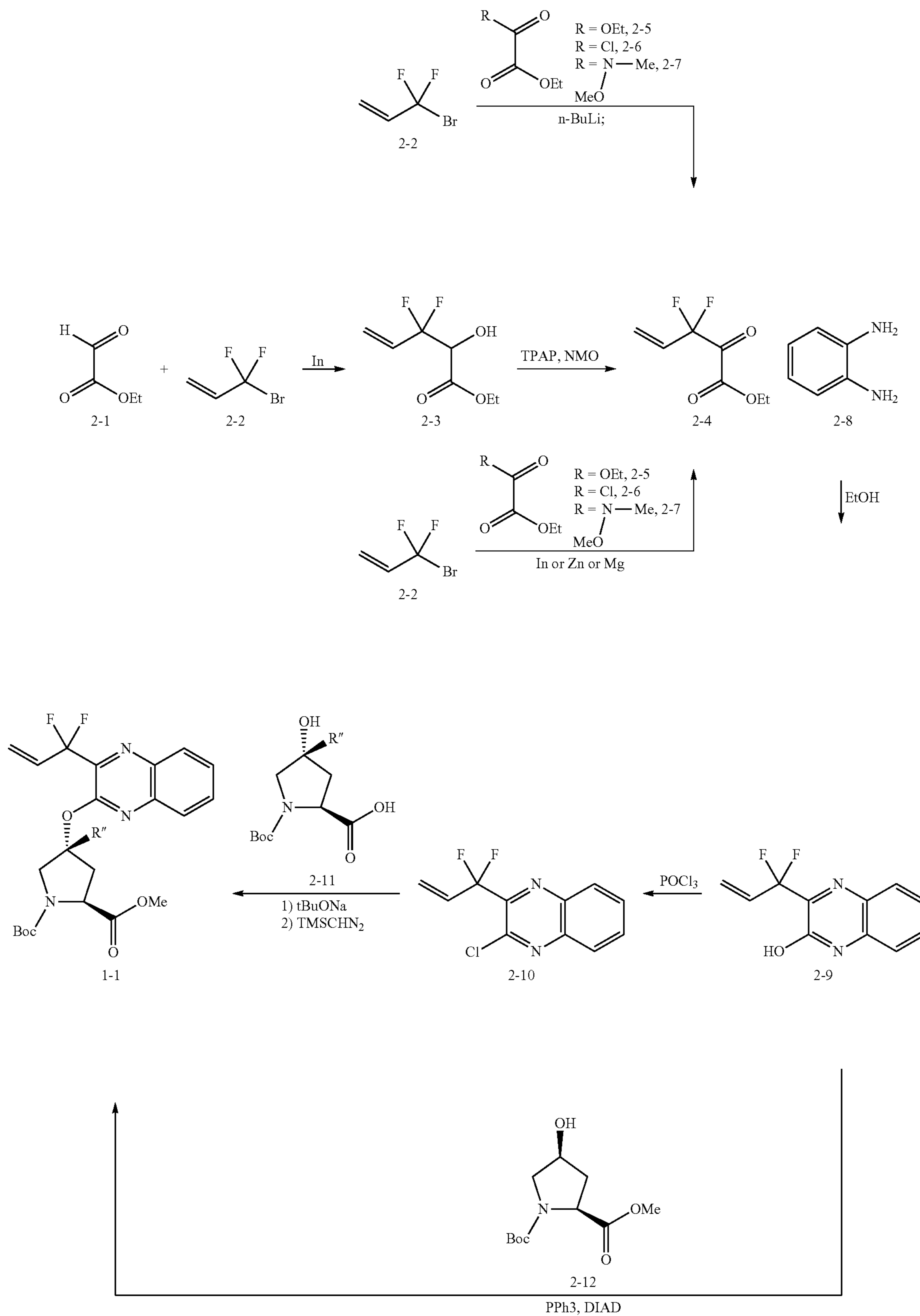
Scheme 2
