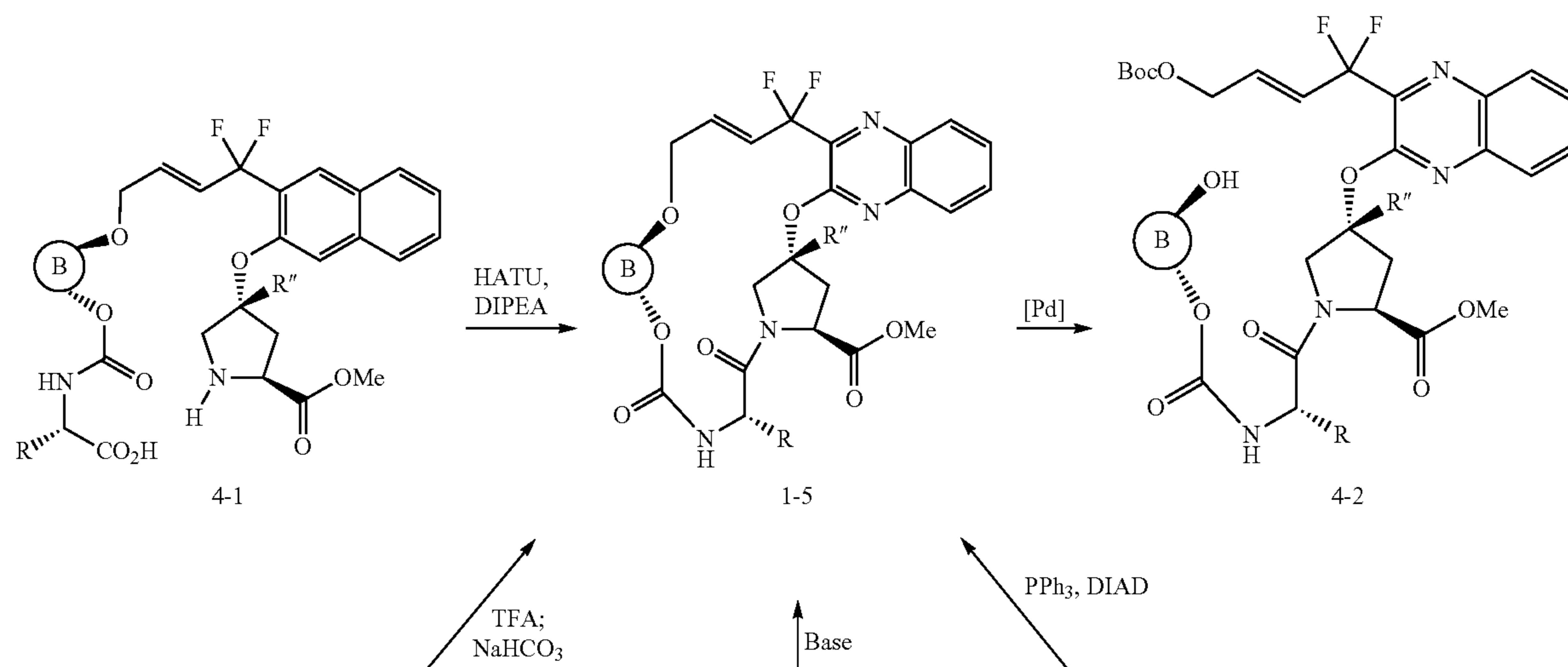
Scheme 4
