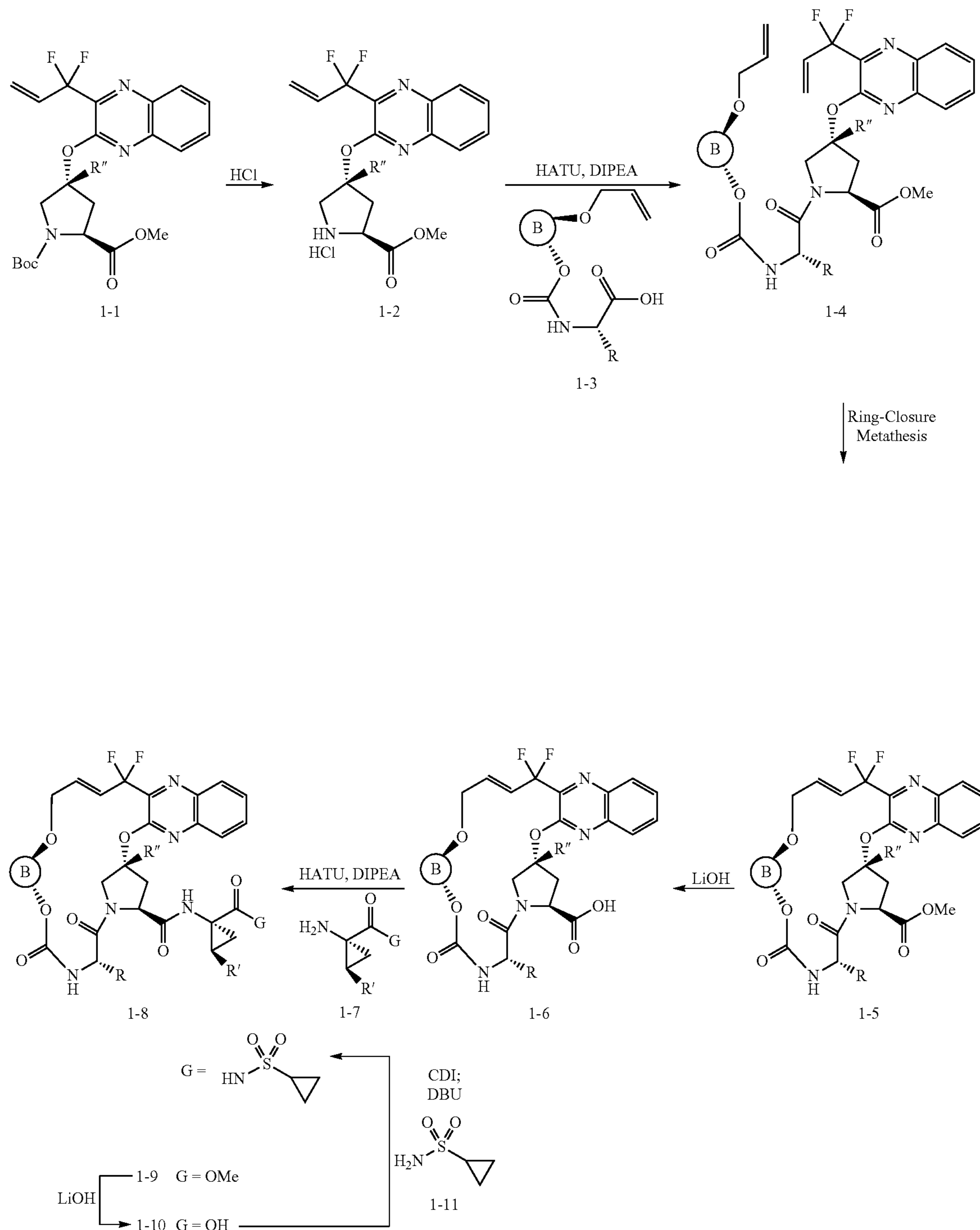
Scheme 1
