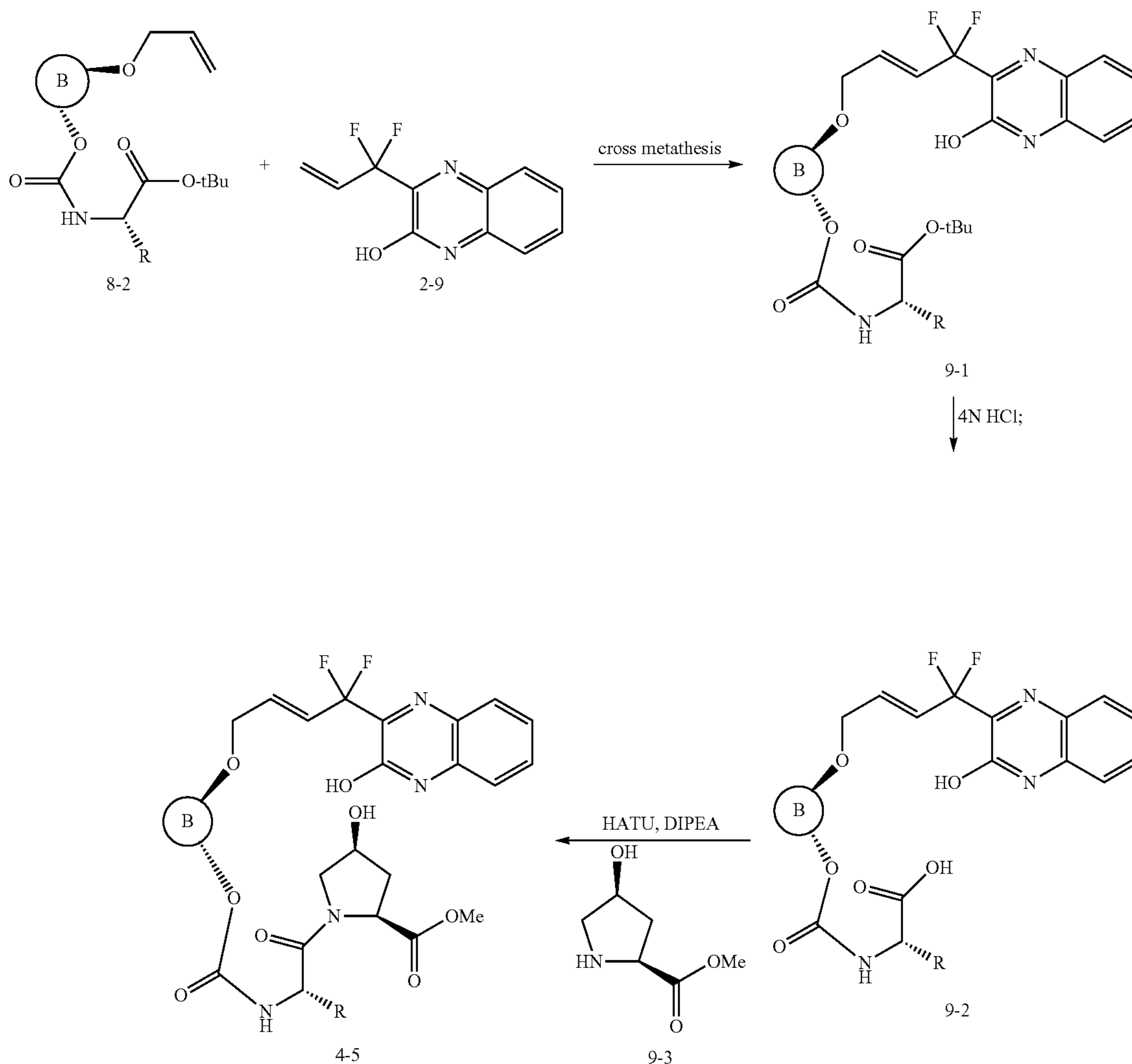
Scheme 9
