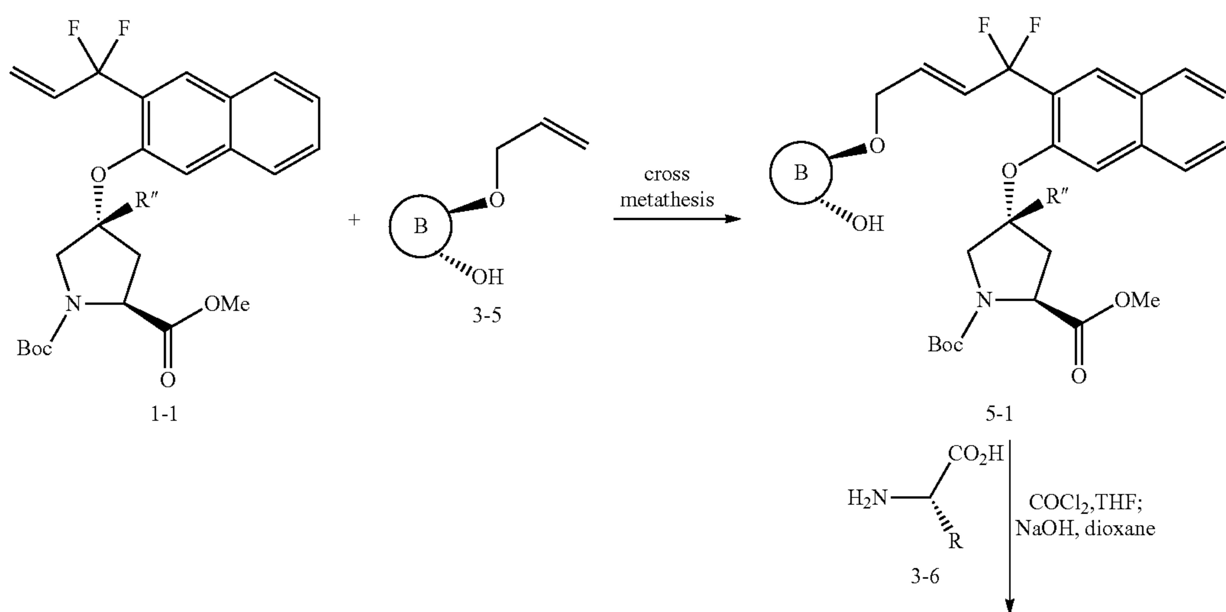
Scheme 5
