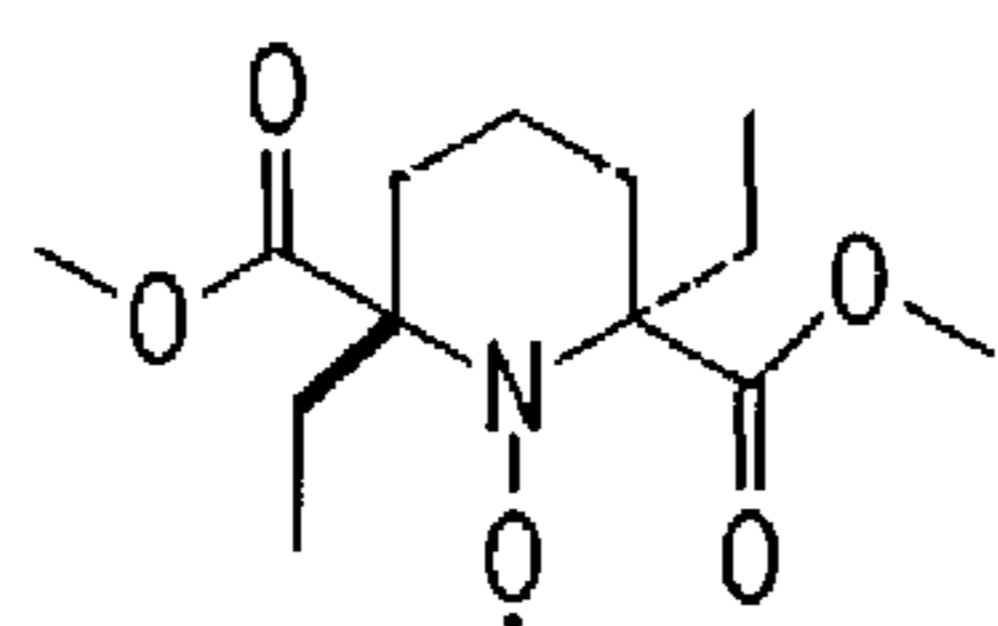
G1, LogP=2.0
