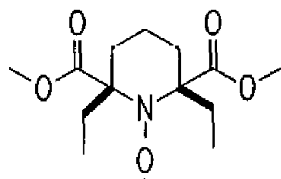
G2, LogP=2.5
