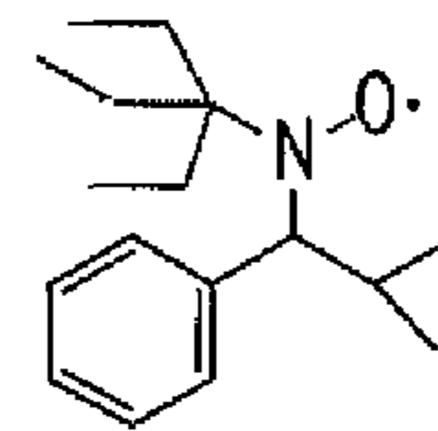
G4, LogP=5.4
