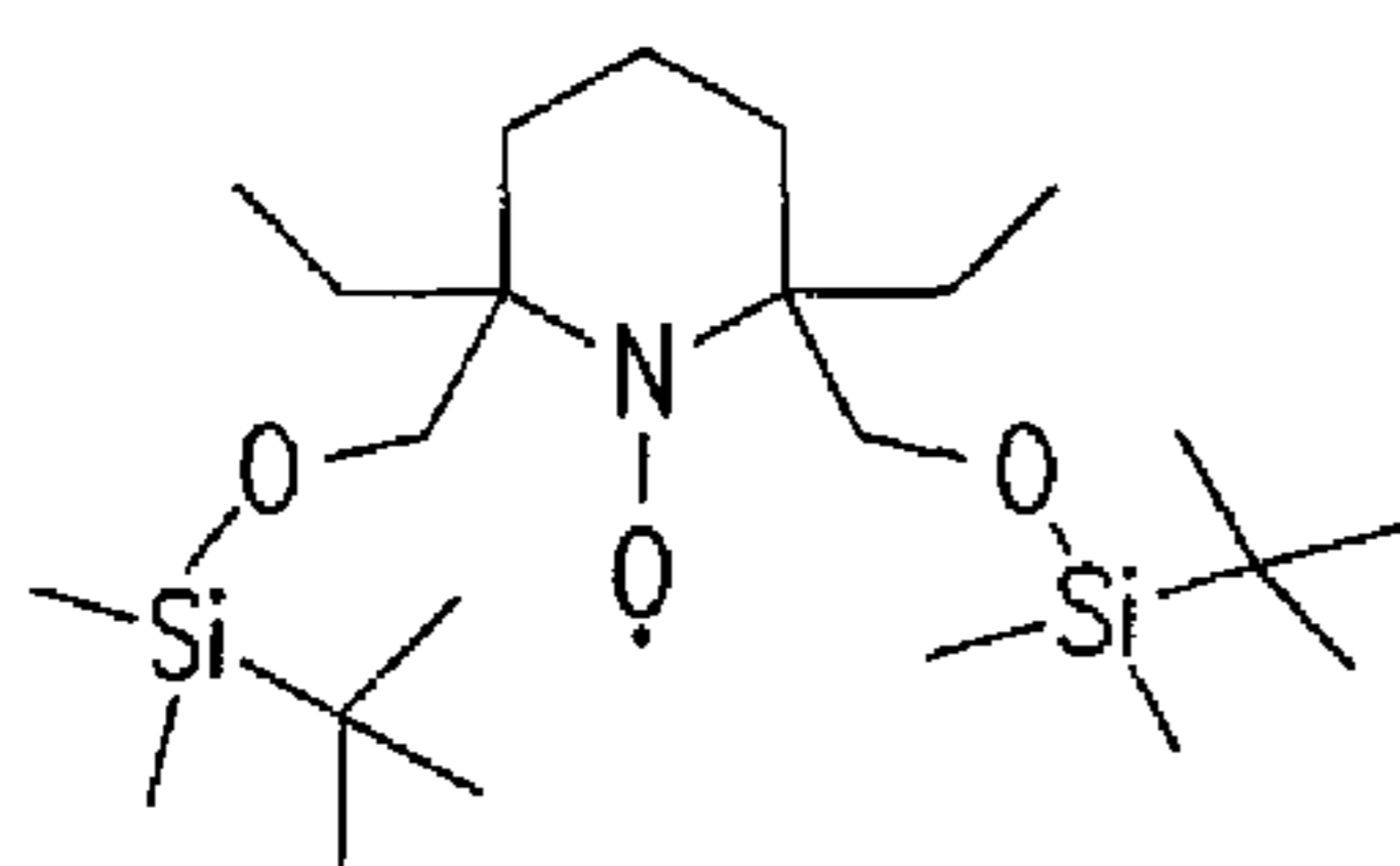
G5, LogP=8.2
