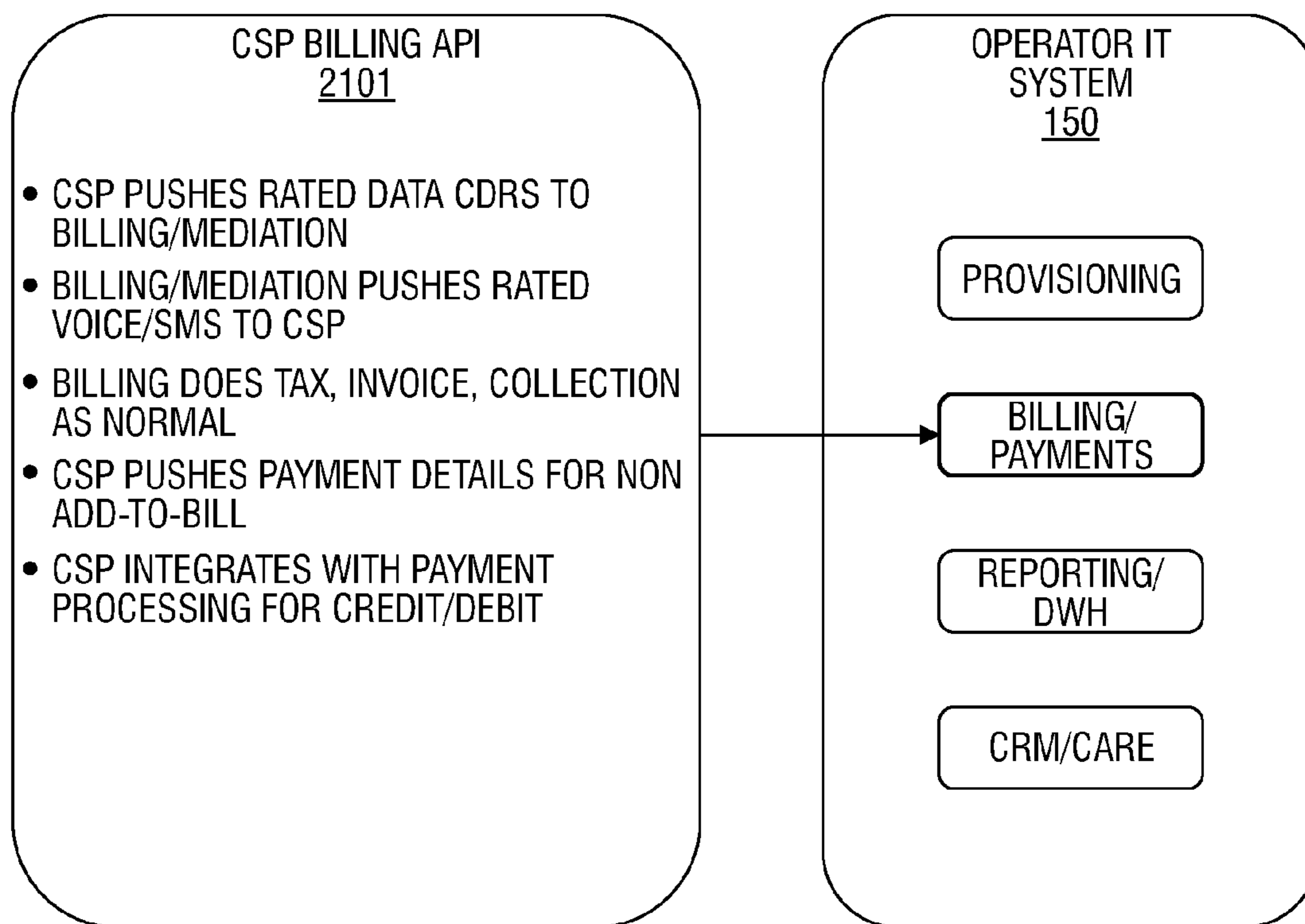
BILLING INTEGRATION
