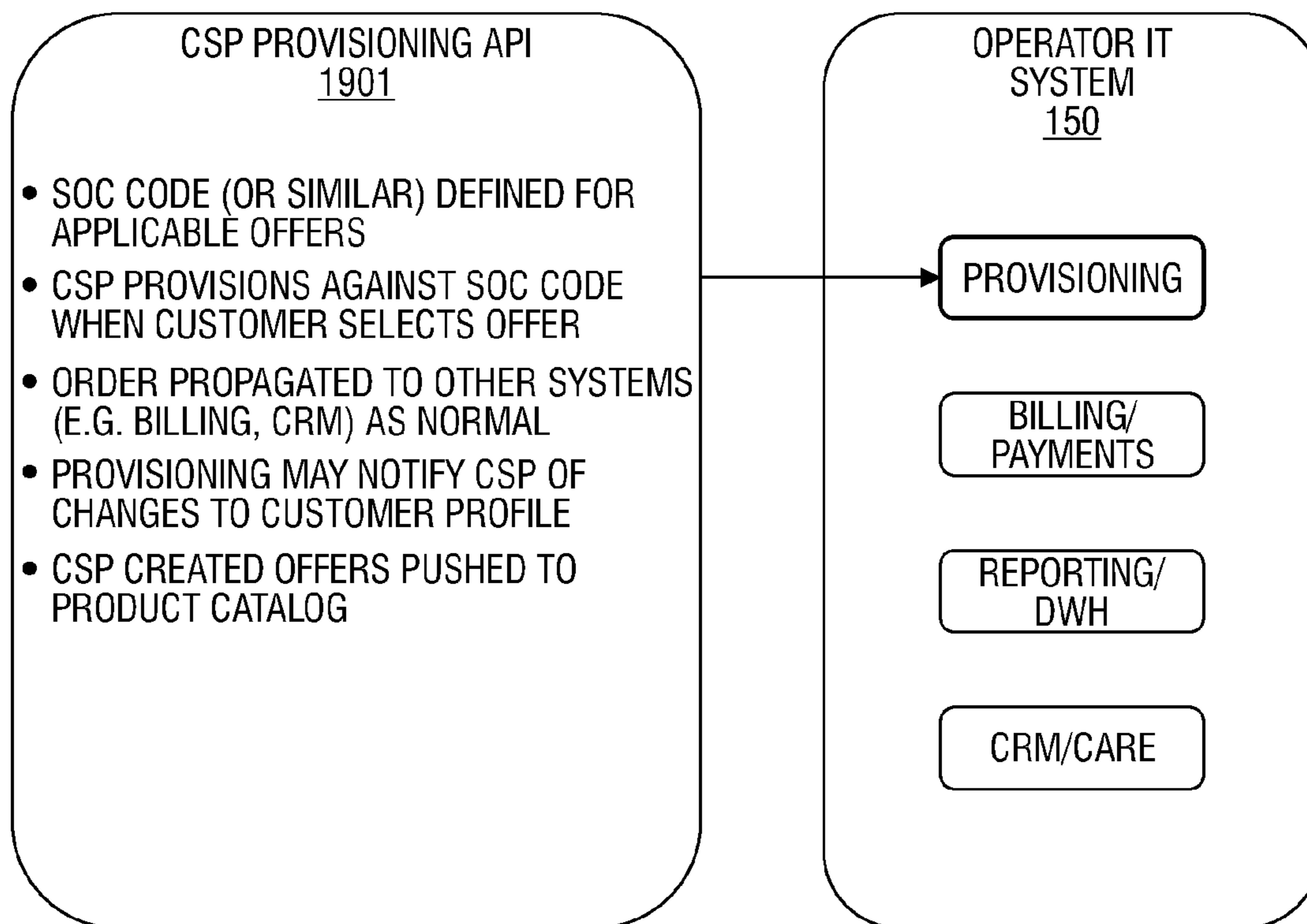
PROVISIONING INTEGRATION
