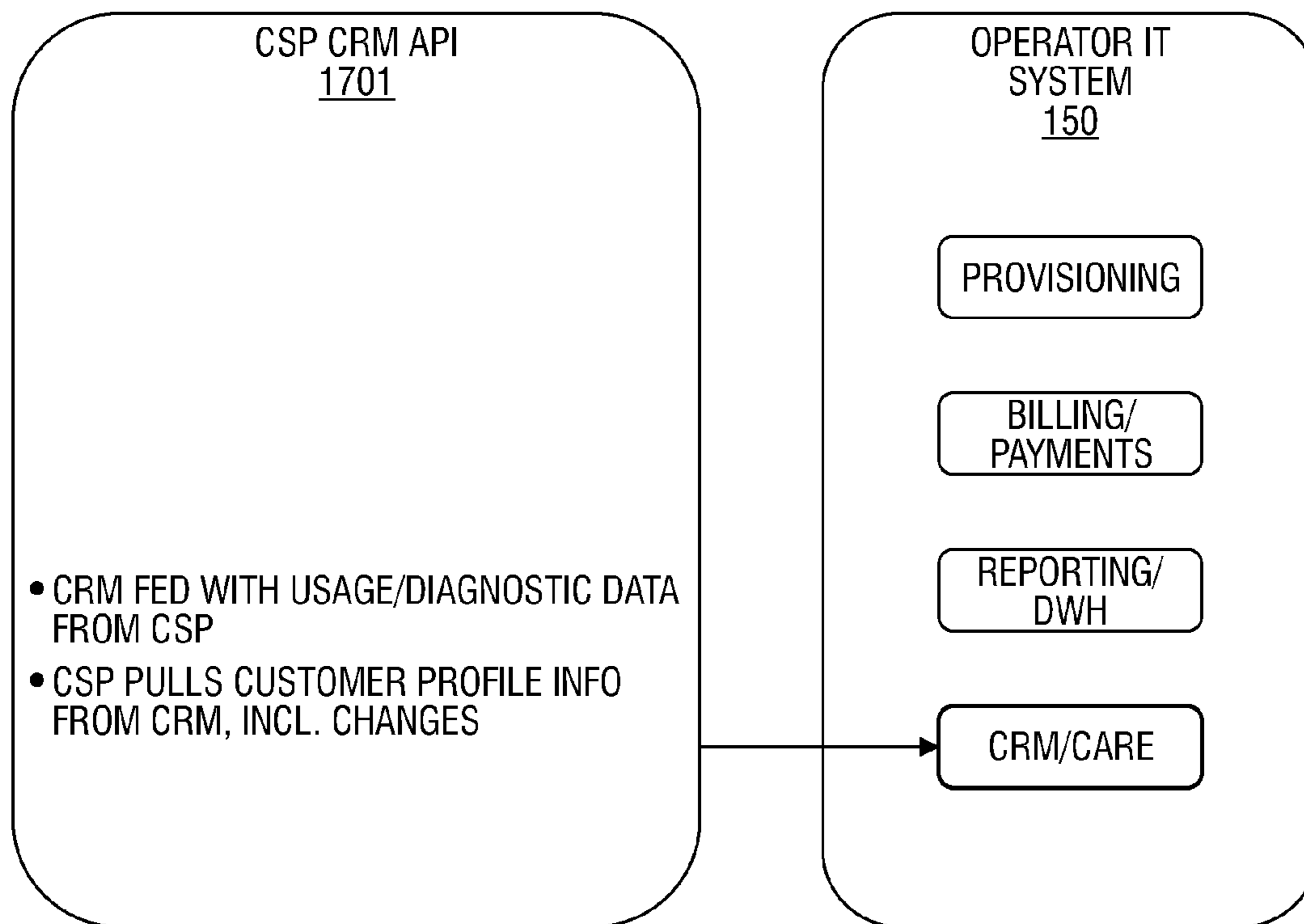
CRM INTEGRATION
