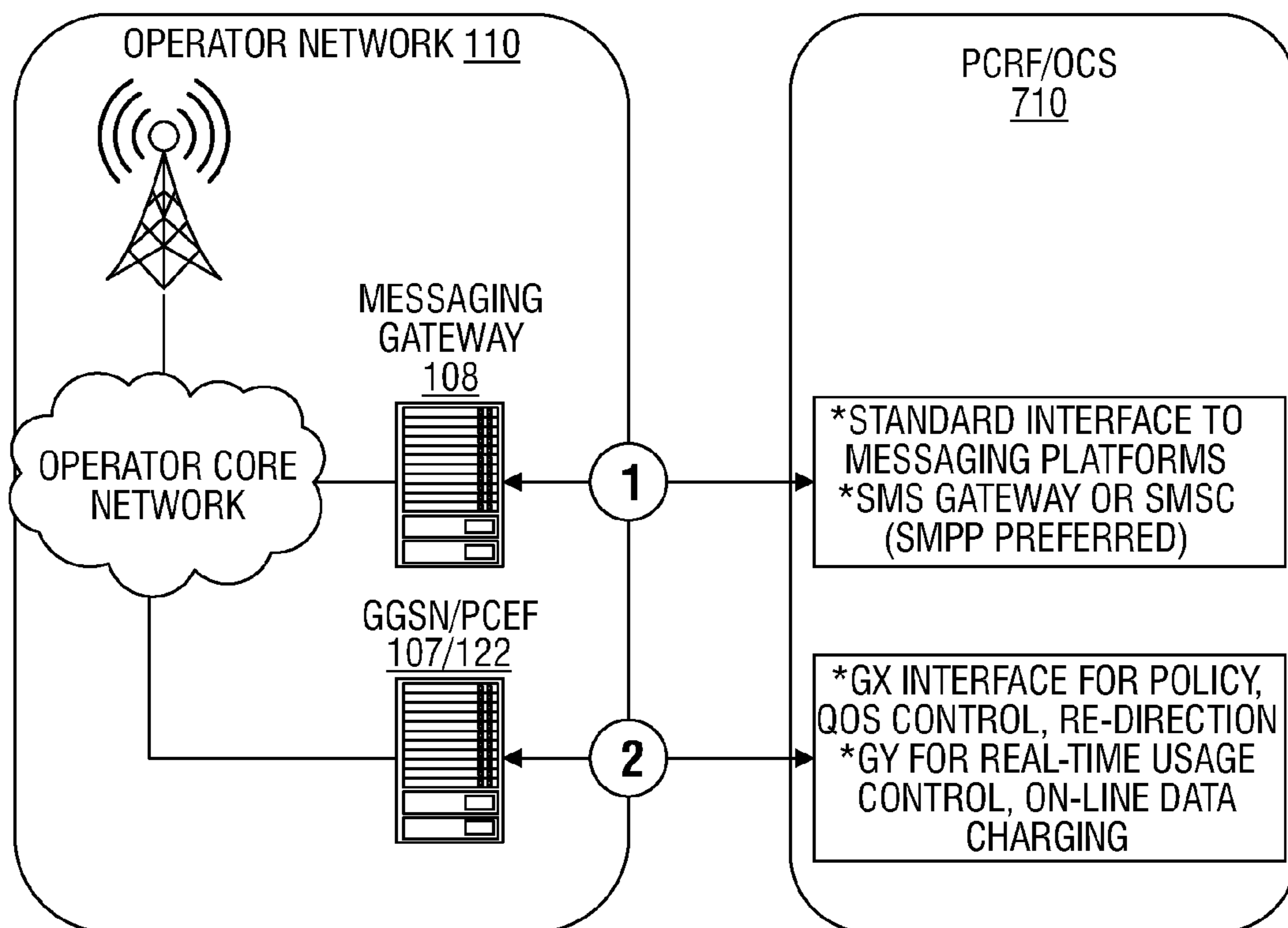
NETWORK INTEGRATION
