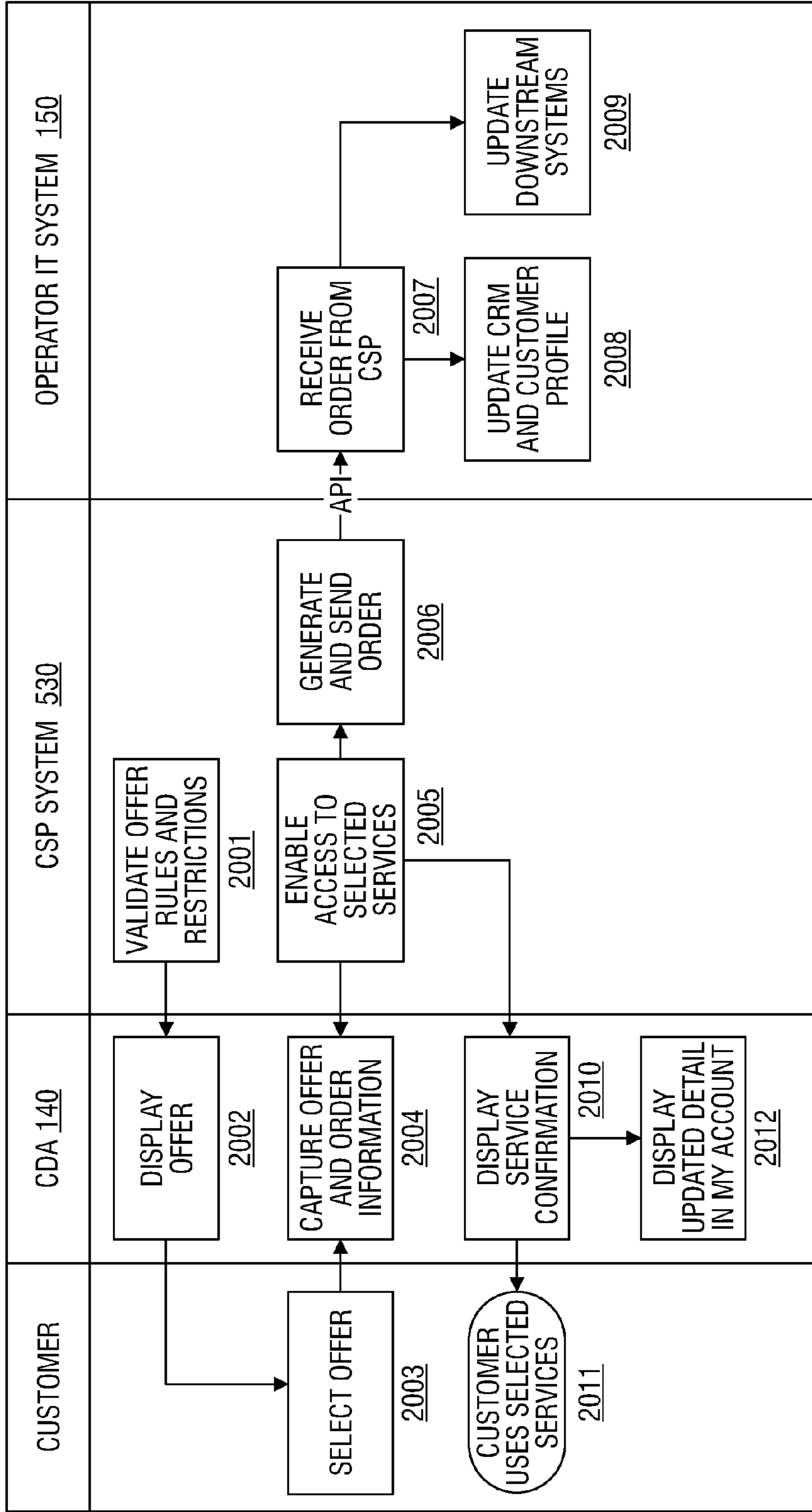
PROVISIONING INTEGRATION
