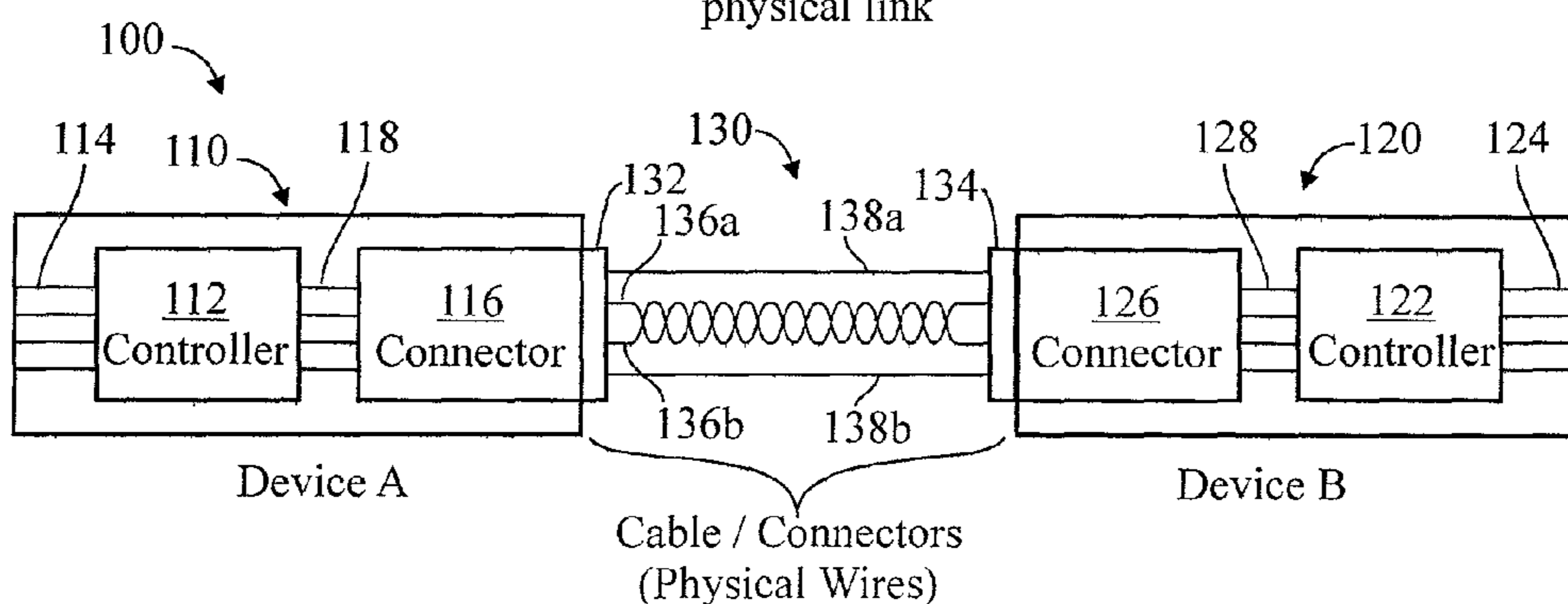
FIG. 1 physical link
