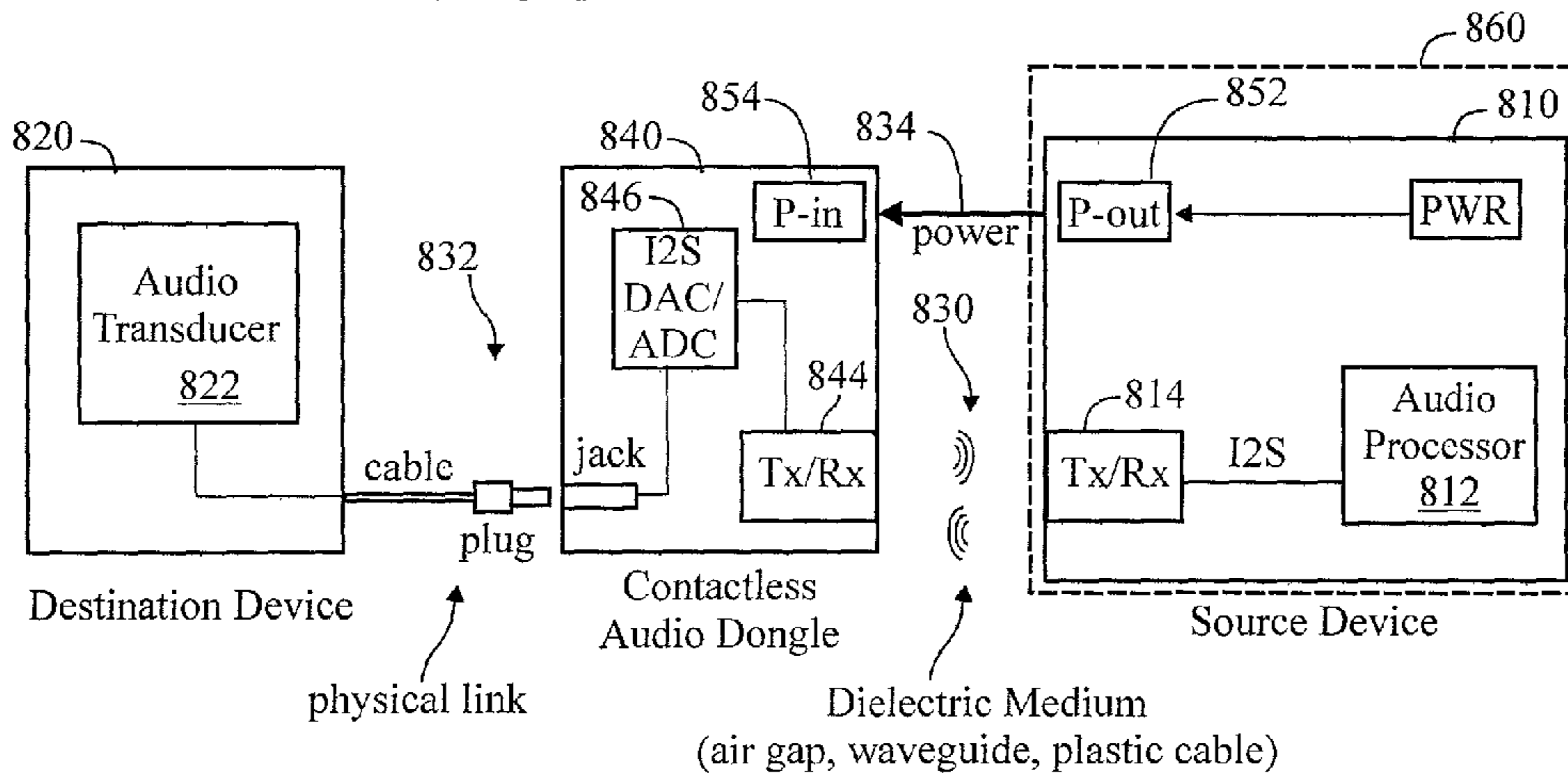
Contactless Audio Dongle and Jack (Dongle powered by Source)
