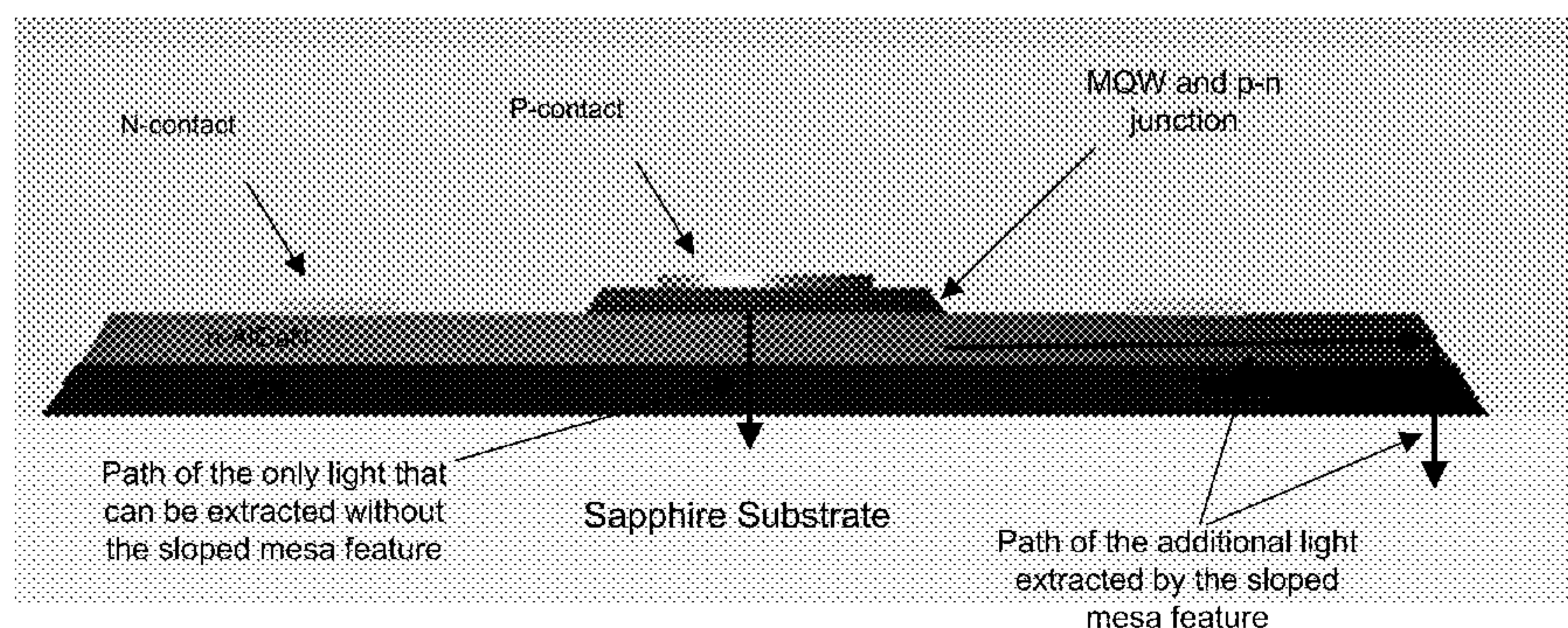
Device Cross-section
