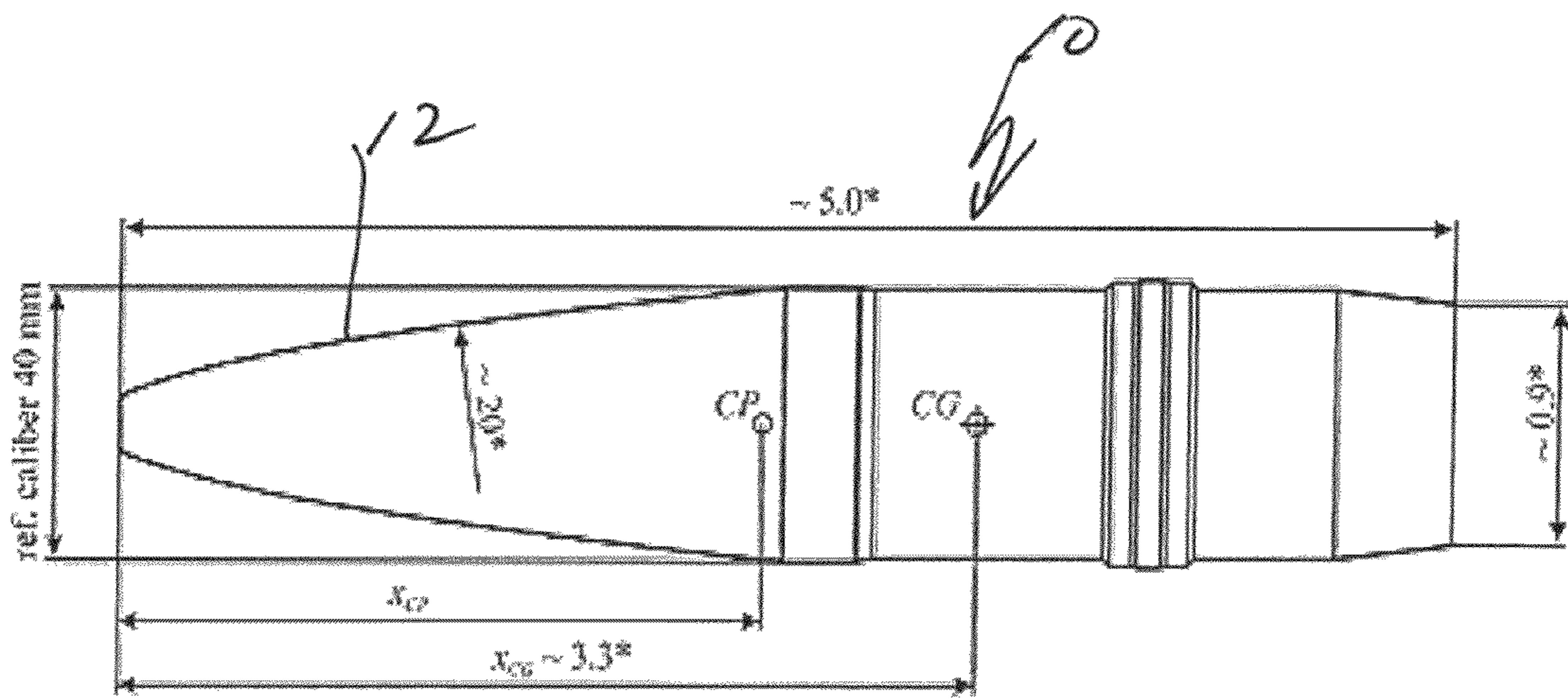
Fig. 1. Model of spin stabilized projectile
