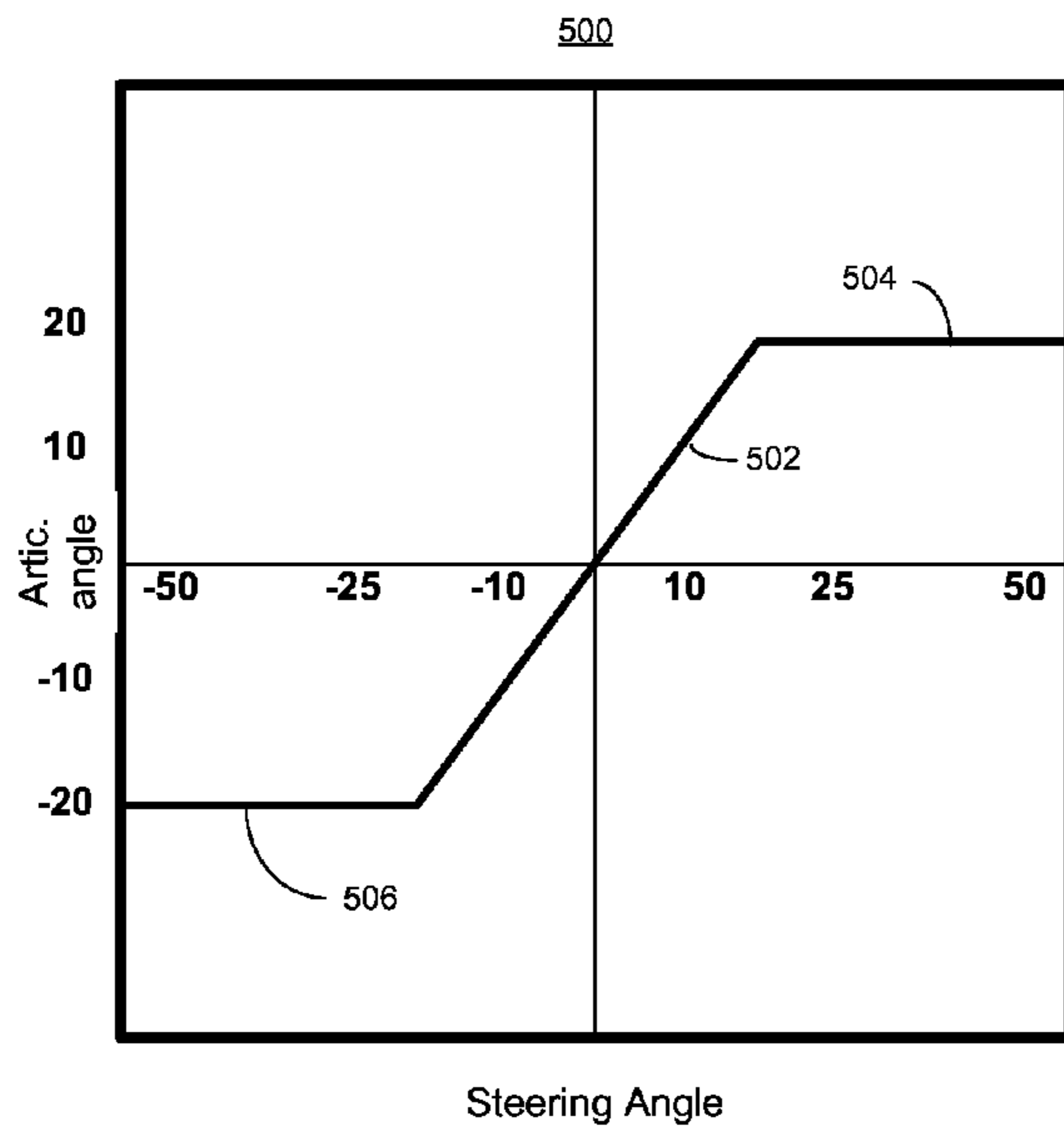
Fig. 11 Prior art
