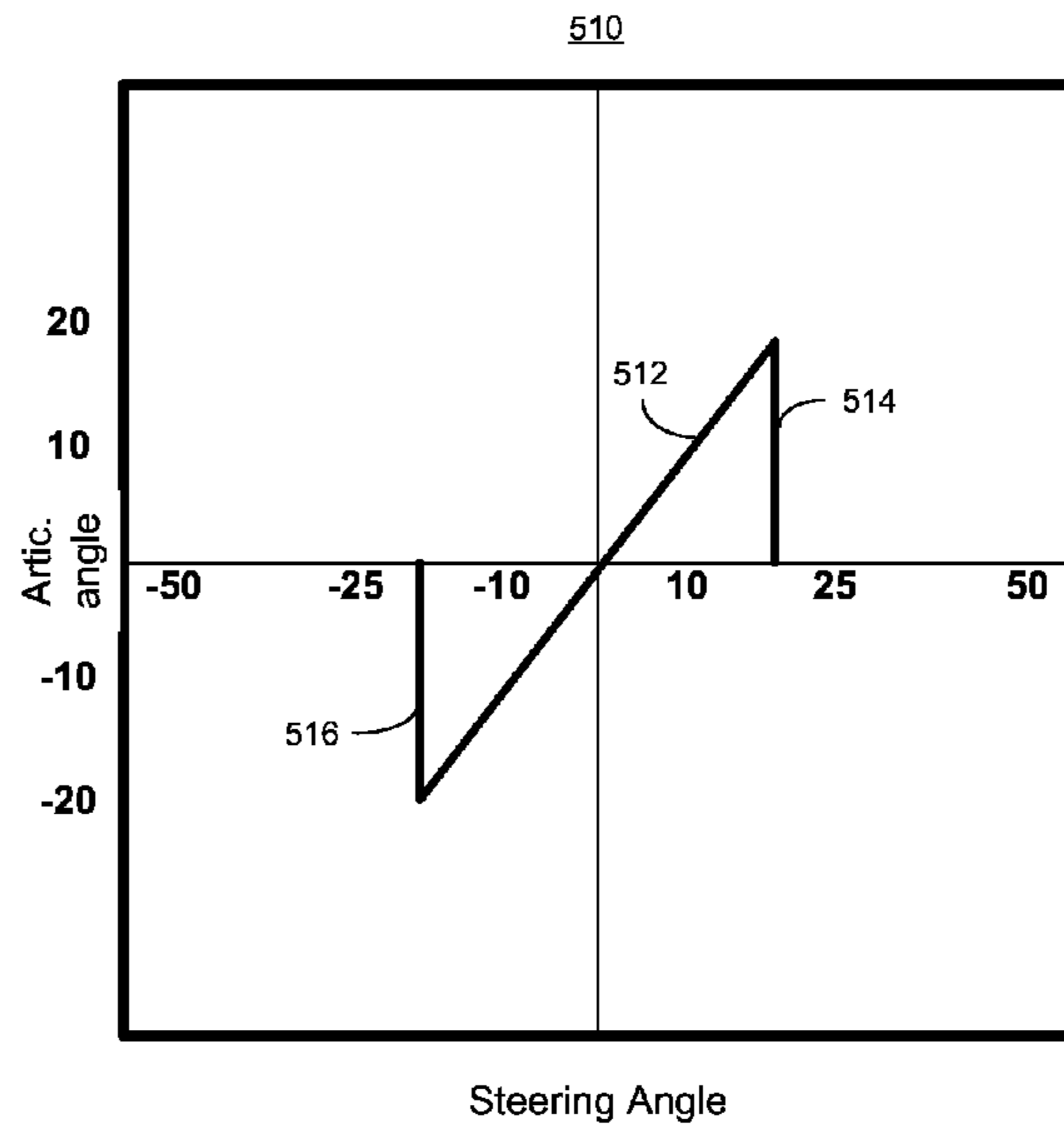
Fig. 12 Prior art
