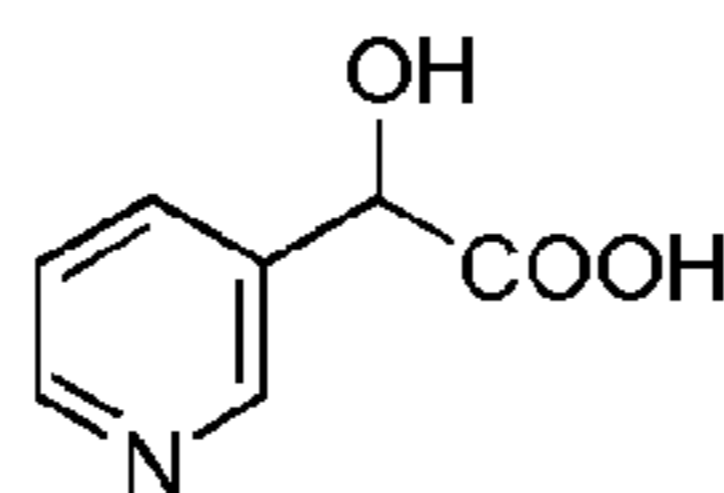
3-pyridyl glycolic acid
