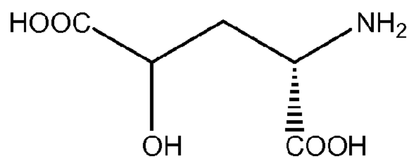
L-gamma-hydroxy glutamate
