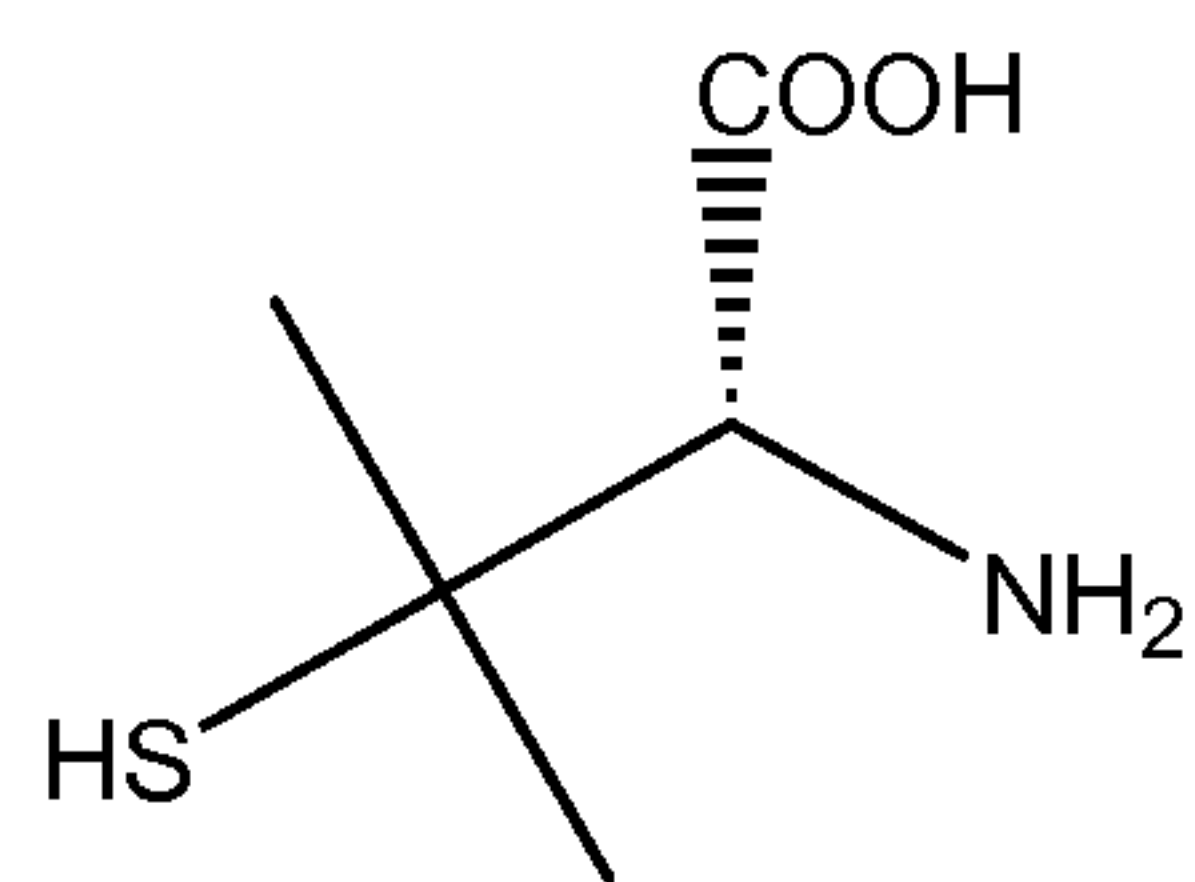
Cuprimine/Depen
