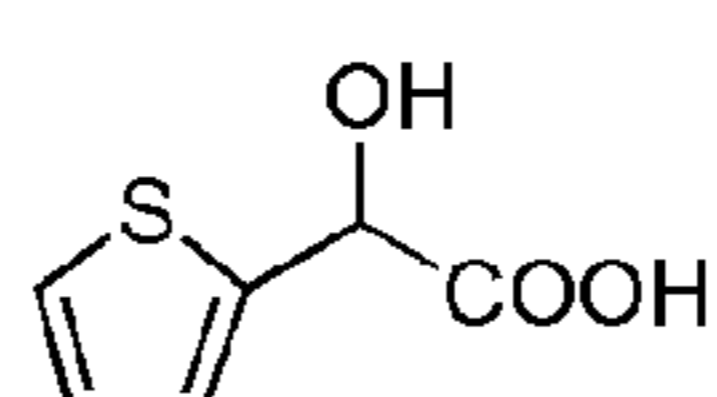
2-thienyl glycolic acid
