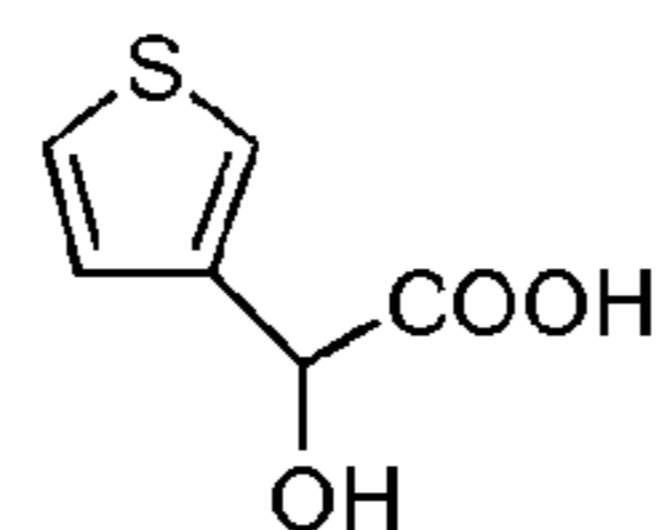
3-thienyl glycolic acid
