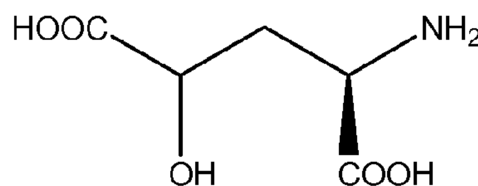
D-gamma-hydroxy glutamate
