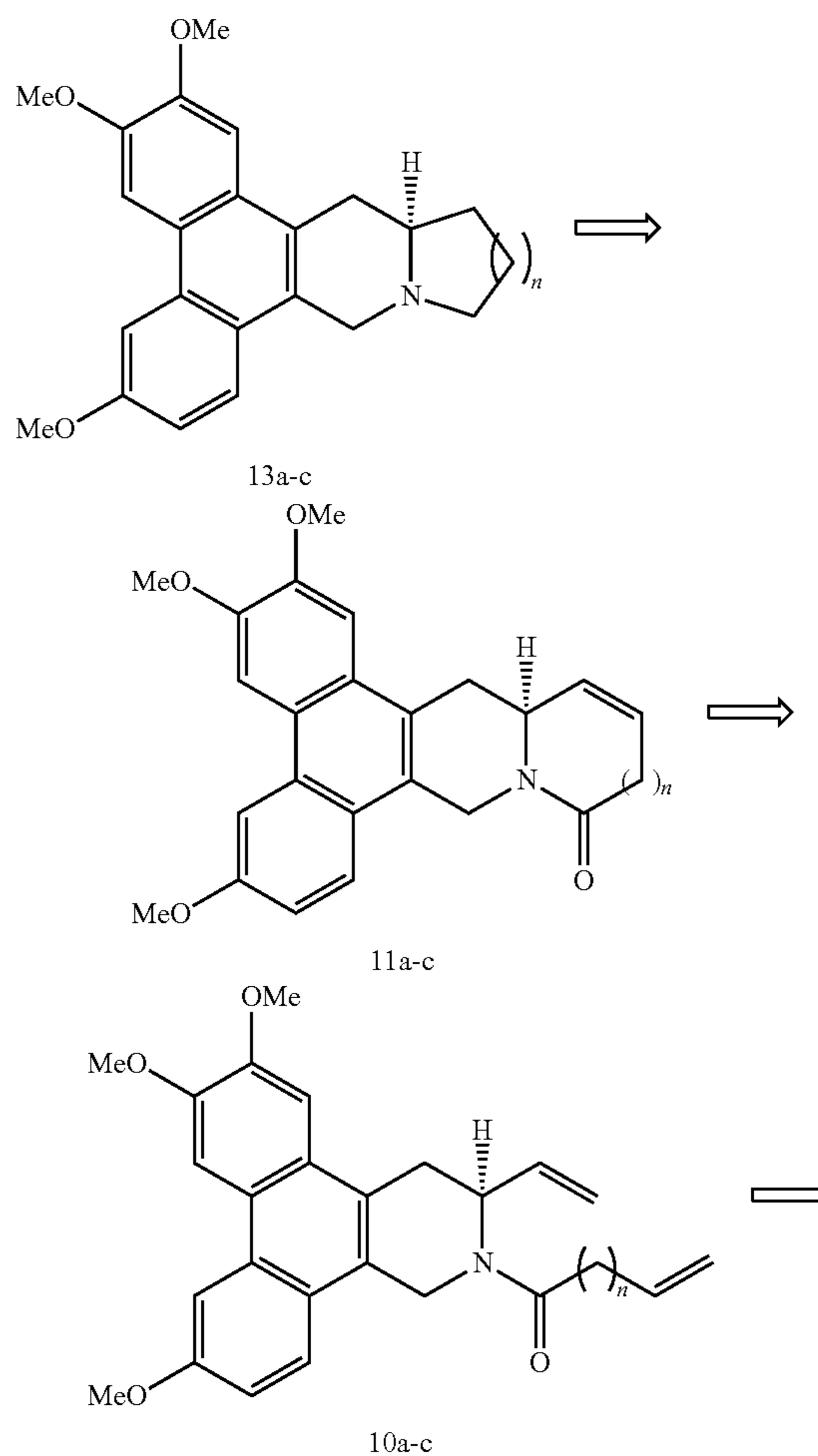
Scheme 1 Retrosynthesis of antofine and its analogs
